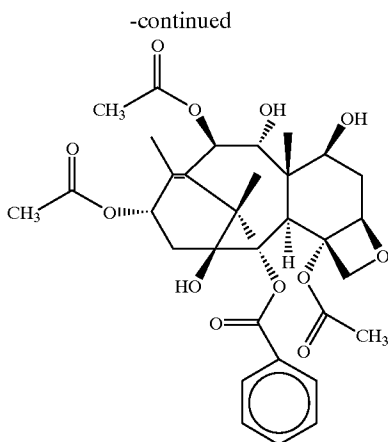
13-acetyl-9-dihydrobaccatin III
