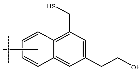
2-(4-(mercaptomethyl)naphthalen-2-yl)ethanol
