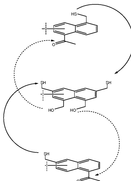
1-(6-(mercaptomethyl)naphthalen-1-yl)ethanone
