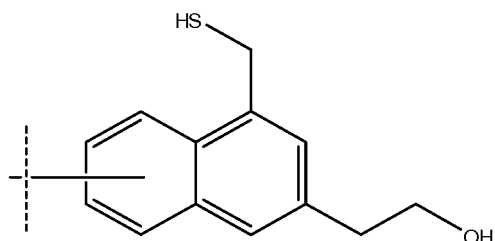
2-(4-(mercaptomethyl)naphthalen-2-yl)ethanol
