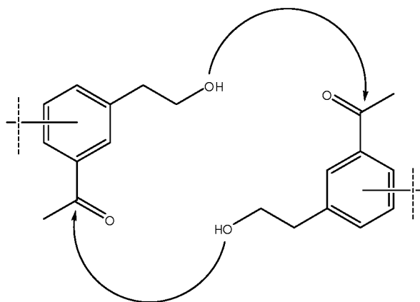
1-(3-(2-hydroxyethyl)phenyl)ethanone
