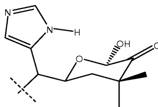
(2R)-2-hydroxy-3-oxo-4-((1H-imidazol-5-yl)methyl)-6,6-dimethylcyclohexanone
