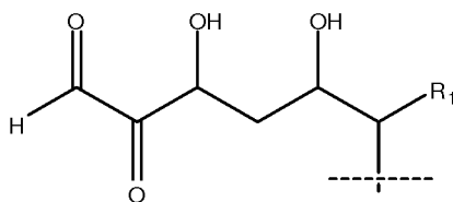
3,5-dihydroxy-2-oxohexanal derivative
