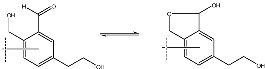
5-(2-hydroxyethyl)-2-(hydroxymethyl)benzaldehyde
