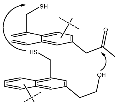
2-(4-(mercaptomethyl)naphthalen-2-yl)ethanol
