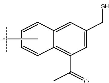
1-(3-(mercaptomethyl)naphthalen-1-yl)ethanone
