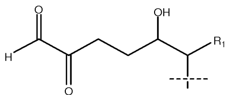
5-hydroxy-2-oxohexanal Derivative
