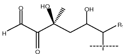
(3S)-3,5-dihydroxy-3-methyl-2-oxohexanal Derivative
