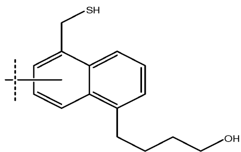
4-(5-(mercaptomethyl)naphthalen-1-yl)butan-1-ol
