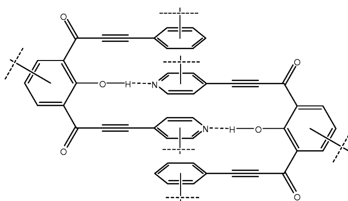
1-(2-hydroxy-3-(3-(pyridin-4-yl)propioloyl)phenyl)-3-phenylprop-2-yn-1-one
