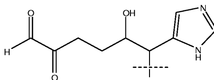
5-hydroxy-6-(1H-imidazol-5-yl)-2-oxohexanal
