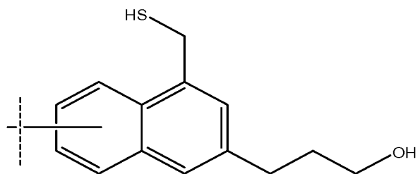
3-(4-(mercaptomethyl)naphthalen-2-yl)propan-1-ol
