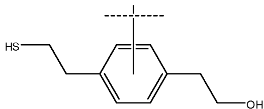
2-(4-(2-mercaptoethyl)phenyl)ethanol
