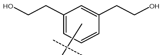
2,2'-(1,3-phenylene)diethanol
