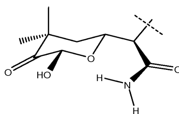
(2S)-2-hydroxy-3-oxo-4-(2-acetamido)-6,6-dimethylcyclohexanone
