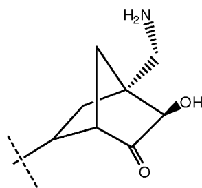
(3R,4S)-4-(aminomethyl)-3-hydroxybicyclo[2.2.1]heptan-2-one
