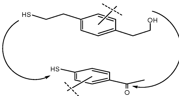
1-(4-mercaptophenyl)ethanone
