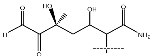
(5S)-3,5-dihydroxy-5-methyl-6,7-dioxoheptanamide
