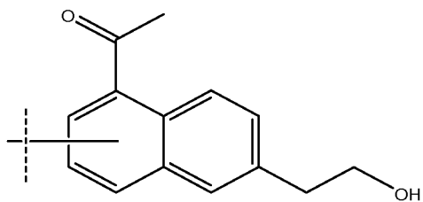
1-(6-(2-hydroxyethyl)naphthalen-1-yl)ethanone
