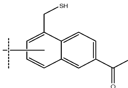
1-(5-(mercaptomethyl)naphthalen-2-yl)ethanone
