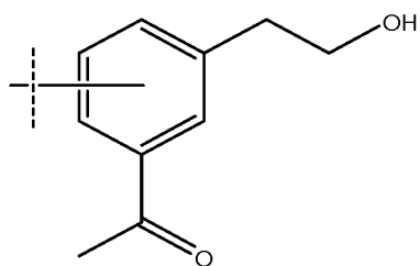
1-(3-(2-hydroxyethyl)phenyl)ethanone
