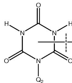
1,3,5-triazinane-2,4,6-trione Monomer 2
