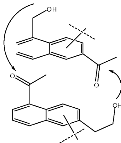
1-(6-(2-hydroxyethyl)naphthalen-1-yl)ethanone
