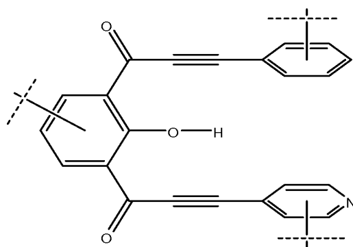
1-(2-hydroxy-3-(3-(pyridin-4-yl)propioloyl)phenyl)-3-phenylprop-2-yn-1-one
