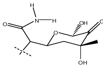
(2R,6R)-2,6-dihydroxy-3-oxo-6-methyl-4-(2-acetamido)-cyclohexanone
