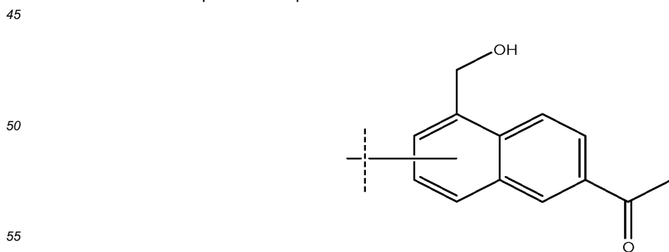
1-(5-(hydroxymethyl)naphthalen-2-yl)ethanone
