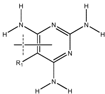
2,4,6-triaminopyrimidine
