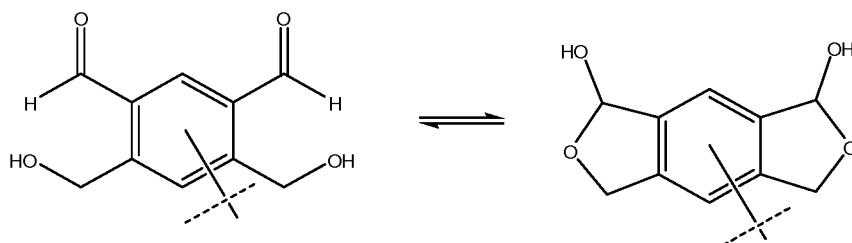
4,6-bis(hydroxymethyl)isophthalaldehyde
