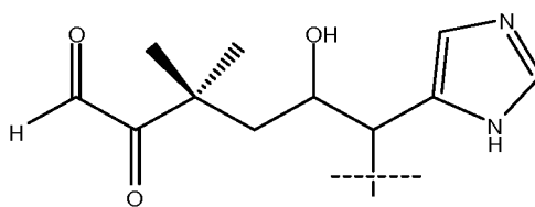
5-hydroxy-6-((1H-imidazol-5-yl)methyl)-3,3-dimethyl-2-oxohexanal
