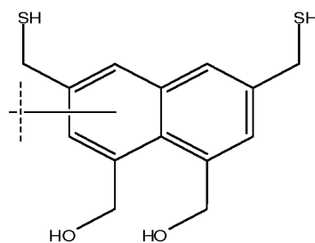
(3,6-bis(mercaptomethyl)naphthalene-1,8-diyl)dimethanol
