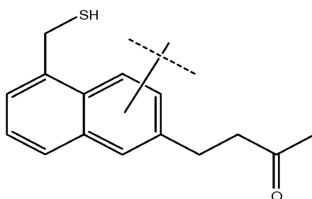
4-(5-(mercaptomethyl)naphthalen-2-yl)butan-2-one
