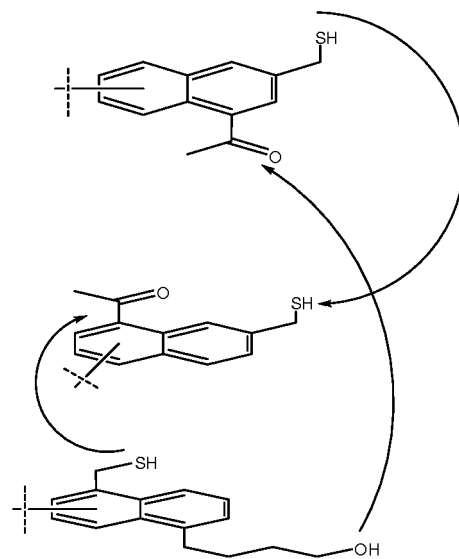
4-(5-(mercaptomethyl)naphthalen-1-yl)butan-1-ol
