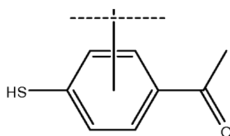
1-(4-mercaptophenyl)ethanone
