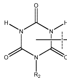
1,3,5-triazine-2,4,6-trione
