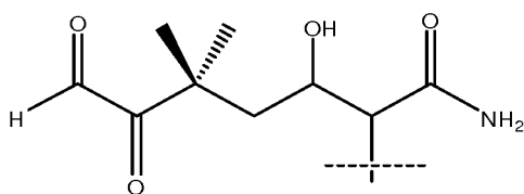
3-hydroxy-5,5-dimethyl-6,7-dioxoheptanamide
