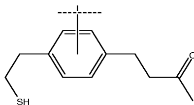
4-(4-(2-mercaptoethyl)phenyl)butan-2-one
