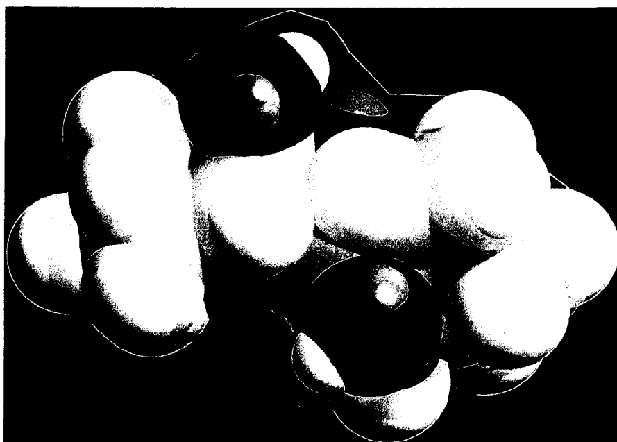
2-hydroxycyclohexanone dimer
