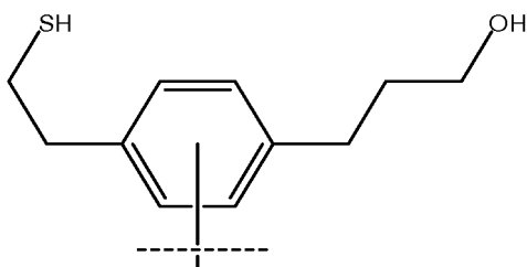
3-(4-(2-mercaptoethyl)phenyl)propan-1-ol
