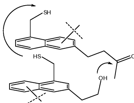
2-(4-(mercaptomethyl)naphthalen-2-yl)ethanol
