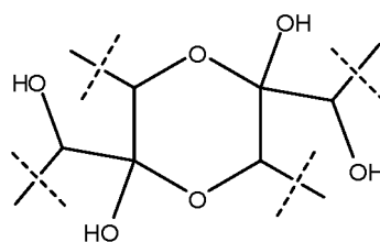
1,3-Dihydroxyacetone dimer
