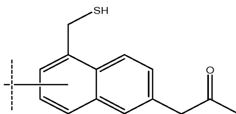
1-(5-(mercaptomethyl)naphthalen-2-yl)propan-2-one
