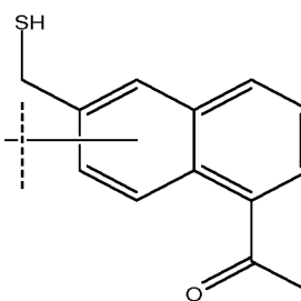
1-(6-(mercaptomethyl)naphthalen-1-yl)ethanone
