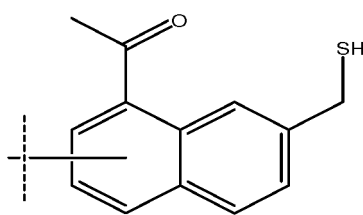
1-(7-(mercaptomethyl)naphthalen-1-yl)ethanone
