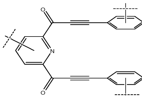
1,1'-(pyridine-2,6-diyl)bis(3-phenylprop-2-yn-1-one)
