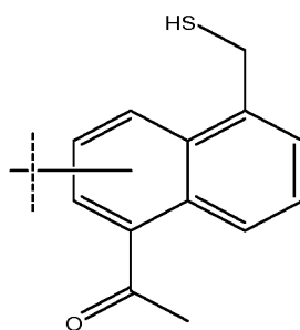
1-(5-(mercaptomethyl)naphthalen-1-yl)ethanone
