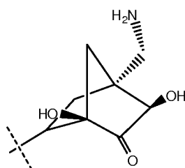
(1S,3R,4S)-4-(aminomethyl)-1,3-dihydroxybicyclo[2.2.1]heptan-2-one
