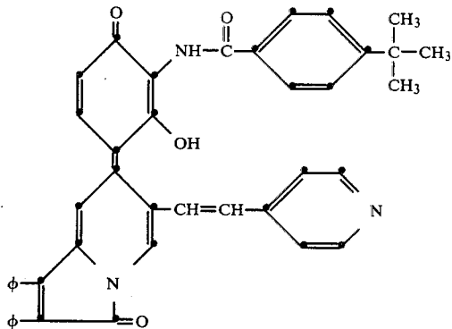
7-[3-(4-tert-butylbenzamido)-2-hydroxy-4-oxo-1-phenylidene]-2,3-diphenyl-6-(3-hydroxypropyl)-1(7H)-indolizine
