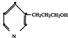
P-30 4-Cyanopyridine:
