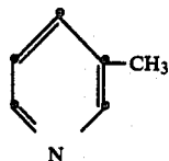
P-27 3-Cyanomethylpyridine (also known as 3-Pyridylacetonitrile):
