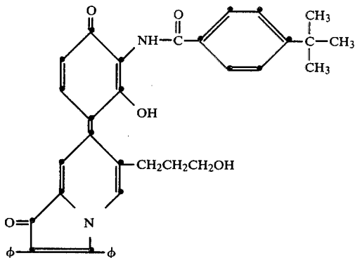
7-[3-(4-tert-butylbenzamido)-2-hydroxy-4-oxo-1-phenylidene]-2,3-diphenyl-6-(3-hydroxypropyl)-1(7H)-indolizine
