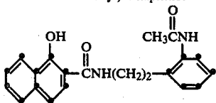
C-13 2-(4-tert-butylbenzamido-resorcinol
