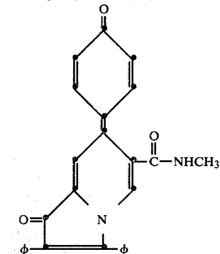
2,3-diphenyl-6-methoxycarbonyl-7-(4-oxo-1-phenylidene)-1(7H)-indolizone
