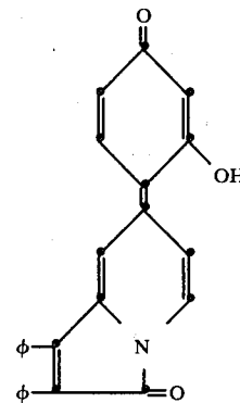
1,2-diphenyl-7-(4-oxo-2-hydroxy-1-phenylidene)-3(7H)-indolizine
