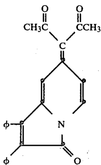
7-(dibenzoylmethylidene)-2,3-diphenyl-
