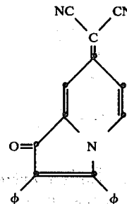
7-(1-cyano-1-phenylmethylidene)-1,2-diphenyl-3(7H)-indolizine
