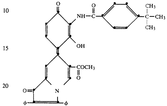
5 7-[3-(4-tert-butylbenzamido)-2-hydroxy-4-oxo-1-phenylidene]-6-carbomethoxy-2,3-diphenyl-1(7H)-indolizine
