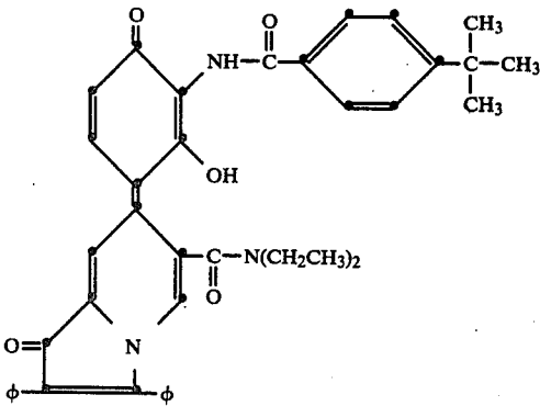
7-[3-(4-tert-butylbenzamido)-2-hydroxy-4-oxo-1-phenylidene]-6-diethylcarbonyl-2,3-diphenyl-1(7H)-indolizinone
