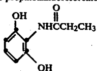
C-17 2-propinoamidoresorcinol
