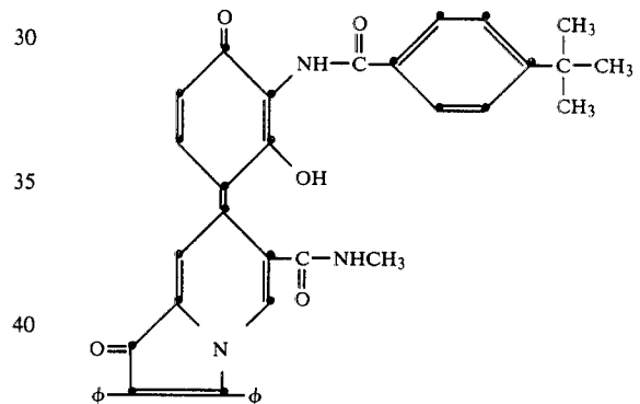
25 7-[3-(4-tert-butylbenzamido)-2-hydroxy-4-oxo-1-phenylidene]-2,3-diphenyl-6-methyl-carbamyl-1(7H)-indolizine
