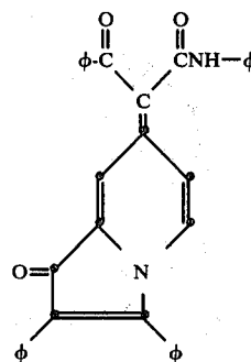
6-cyano-7-(diacetylmethylidene)-2,3-diphenyl-1(7H)-indolizine
