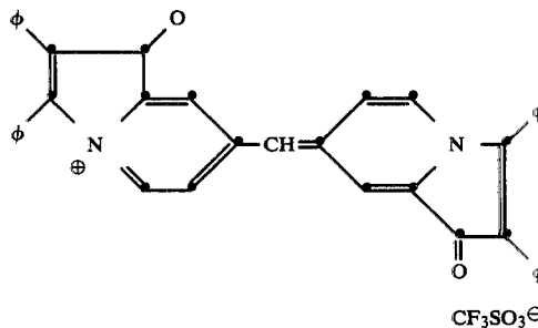
2,3-diphenyl-7-[(2,6-diphenyl-4-thio- pyranilydene)methyl]-1-indolizinium trifluoromethane sulfonate
