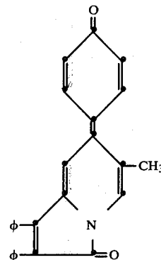
2,3-diphenyl-6-formyl-7-(4-oxo-1-phenylidene)-1(7H)-indolizine
