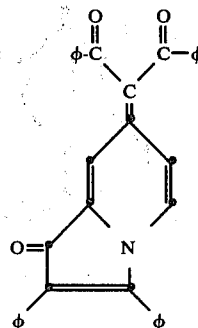
7-(anilincarbonyl benzoylmethylidene)-2,3-diphenyl-1(7H)-indolizine
