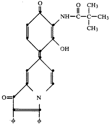
7-[3-(4-tert-butylbenzamido)-2-hydroxy-4-oxo-1-phenylidene]-1,2-diphenyl-6-[2-(4-pyridyl)-1-ethenyl]-3(7H)-indolizine
