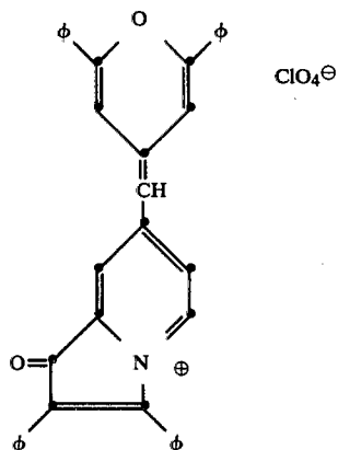
2,3-diphenyl-7-[(2,3-diphenyl-7-1(7H)- indolizinonylidene)methyl]-1-indoli- zinonium trifluoromethane sulfonate
