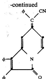
7-(1-aminocarbonyl-1-phenylmethylidene)- 2,3-diphenyl-1(7H)-indolizinone
