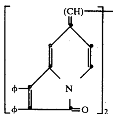
1,4-bis[7-(1,2-diphenyl-3(7H)-indolizinonylidene)]-2,5-cyclohexadiene
