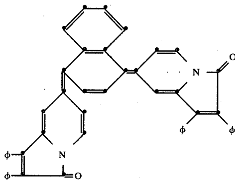
7,7'-bis[1,2-di-n-propyl-3(7H)-indolizinonylidene]
