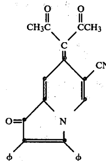
7-(dicyanomethylidene)-2,3-diphenyl-1(7H)-indolizine
