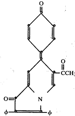
6-benzyl-1,2-diphenyl-7-(4-oxo-1-phenylidene)-3(7H)-indolizinone
