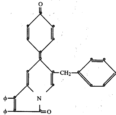
6-chloro-1,2-diphenyl-7-(4-oxo-1-phenylidene)-3(7H)-indolizinone
