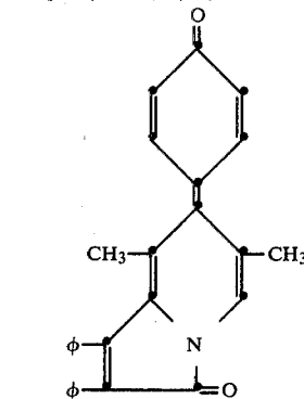
2,3-diphenyl-6-methylaminocarbonyl-7-(4-oxo-1-phenylidene)-1(7H)-indolizone
