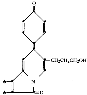
1,2-diphenyl-6-ethoxycarbonylmethyl-7-(4-oxo-1-phenylidene)-3(7H)-indolizone
