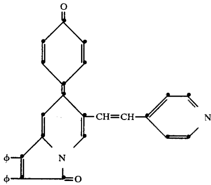
2,3-diphenyl-7-(2-hydroxy-4-oxo-3-pival-amido-1-phenylidene)-1(7H)-indolizine
