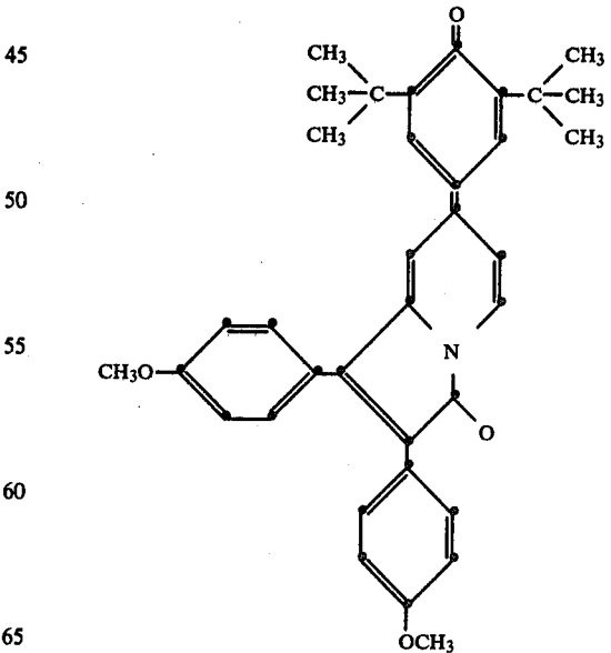
7-[3,5-di-tert-butyl-4-oxo-1-phenylidene]-2,3-di-n-propyl-1(7H)-indolizinone
