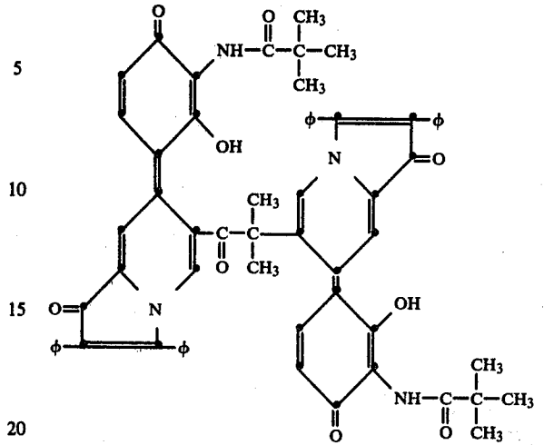
2,3-diphenyl-7-[3-(4-tert-butylbenzamido)-2-hydroxy-4-oxo-1-phenylidene]-1(7H)-indolizinone
