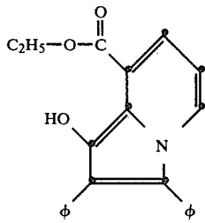
7-carboxy-2,3-diphenyl-1-indolizolinol
