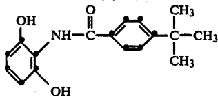
C-14 resorcinol
