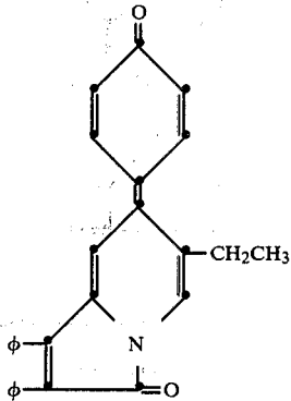
6-cyanomethyl-1,2-diphenyl-7-(4-oxo-1-phenylidene)-3(7H)-indolizone
