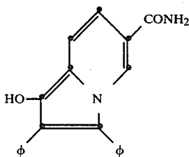
8-carboethoxy-2,3-diphenyl-1-indolizolinol
