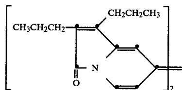
7,7'-bis-[1,2-pentamethylene-3(7H)-indolizinonylidene]
