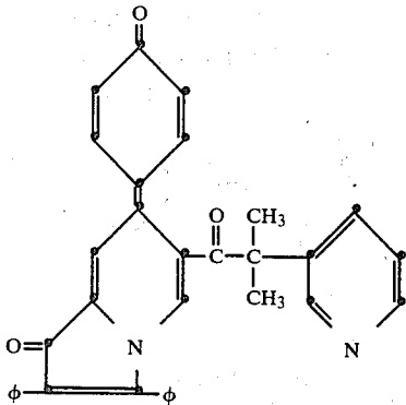
2,3-diphenyl-6-[2-methyl-2-(3-pyridyl)-propionyl]-7-(4-oxo-1-phenylidene)-1(7H)-indolizinone
