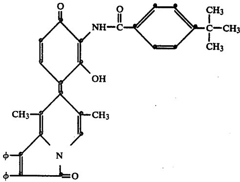
7-[3-(4-tert-butylbenzamido)-2-hydroxy-4-oxo-1-phenylidene]-6-diethylcarbonyl-2,3-diphenyl-1(7H)-indolizinone
