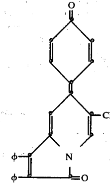
6-cyano-2,3-diphenyl-7-(4-oxo-1-phenylidene)-1(7H)-indolizinone
