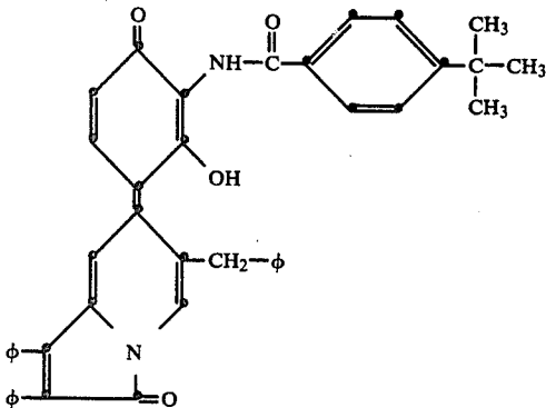
6-benzyl-7-[3-(4-tert-butylbenzamido)-2-hydroxy-4-oxo-1-phenylidene]-1,2-diphenyl-3(7H)-indolizinone
