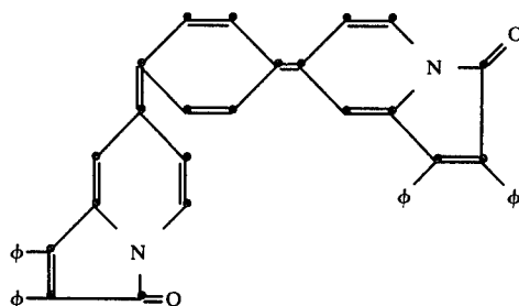
1,4-bis[7-(1,2-diphenyl-3(7H)-indolizinonylidene)]-2,3-benzo-2,5-cyclohexadiene
