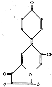
6-(4-azastyryl)-1,2-diphenyl-7-(4-oxo-1-phenylidene)-3(7H)-indolizinone
