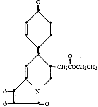
6,8-dimethyl-1,2-diphenyl-7-(4-oxo-1-phenylidene)-3(7H)-indolizone
