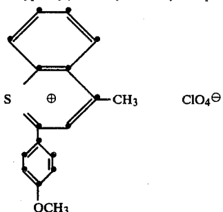
M-8 2-(4-methoxyphenyl)-4-methylthioflavylium perchlorate
