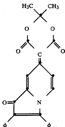
2,3-diphenyl-7-(2,2-dimethyl-4,6-dioxo- 1,3-dioxanylidene)-1(7H)-indolizinone
