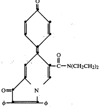
1,2-diphenyl-6-ethyl-7-(4-oxo-1-phenylidene)-3(7H)-indolizone
