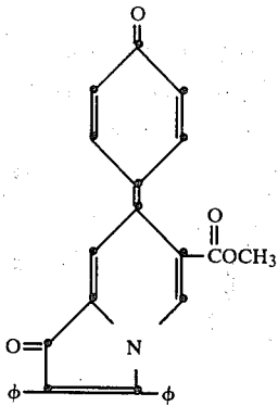
2,3-diphenyl-6-[2-methyl-2-(3-pyridyl)-propionyl]-7-(4-oxo-1-phenylidene)-1(7H)-indolizinone
