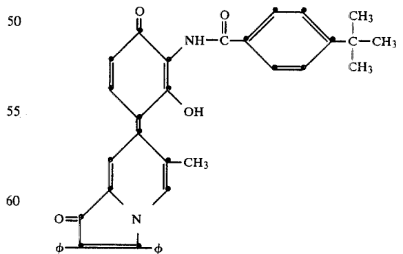
45 7-[3-(4-tert-butylbenzamido)-2-hydroxy-4-oxo-1-phenylidene]-2,3-diphenyl-6-methyl-1(7H)-indolizine
