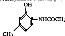
2-[α-(4'-tert.-amylphenoxy)-butyrylamino]-5-methyl-1-phenol
