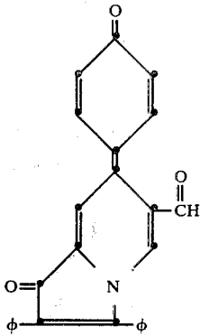
6-diethylaminocarbonyl-2,3-diphenyl-(4-oxo-1-phenylidene)-1(7H)-indolizone
