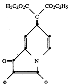
2,3-diphenyl-7-(2,2-dimethyl-4,6-dioxo- 1,3-dioxanylidene)-1(7H)-indolizinone
