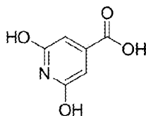
citrazinic acid
