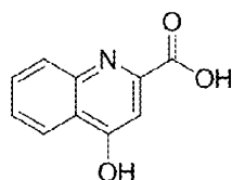
kynurenic acid
