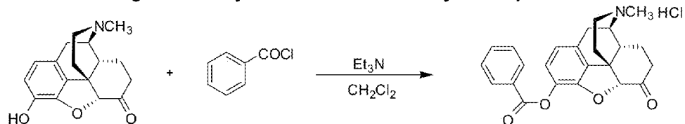
Figure 21D: Synthesis of 3,6-di-aspirin-hydromorphone:
