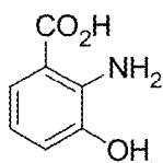
3-hydroxyanthranilic acid
