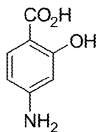
4-aminosalicylic acid
