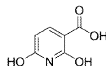
2,6-dihydroxynicotinic acid
