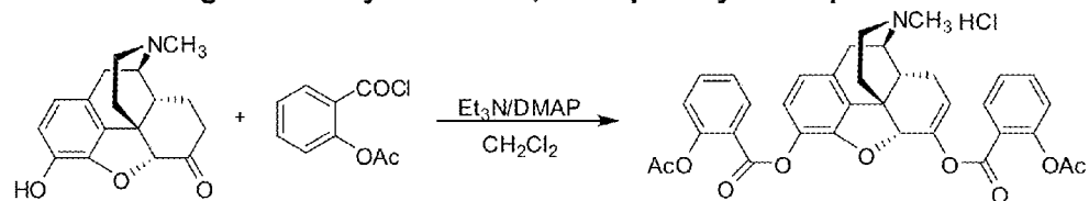
Figure 21D: Synthesis of 3,6-di-aspirin-hydromorphone:
