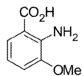
3-methoxyanthranilic acid
