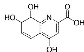
7,8-dihydro-7,8-dihydroxykynurenic acid
