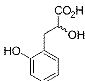
2-hydroxyphenyl- lactic acid
