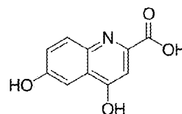
6-hydroxy-kynurenic acid
