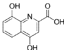
xanthurenic acid
