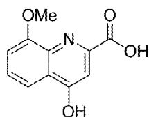
8-methoxykynurenic acid
