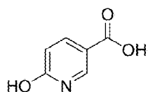
6-hydroxynicotinic acid
