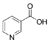
nicotinic acid
