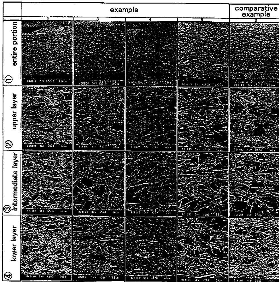
SEM photograph of cross section
