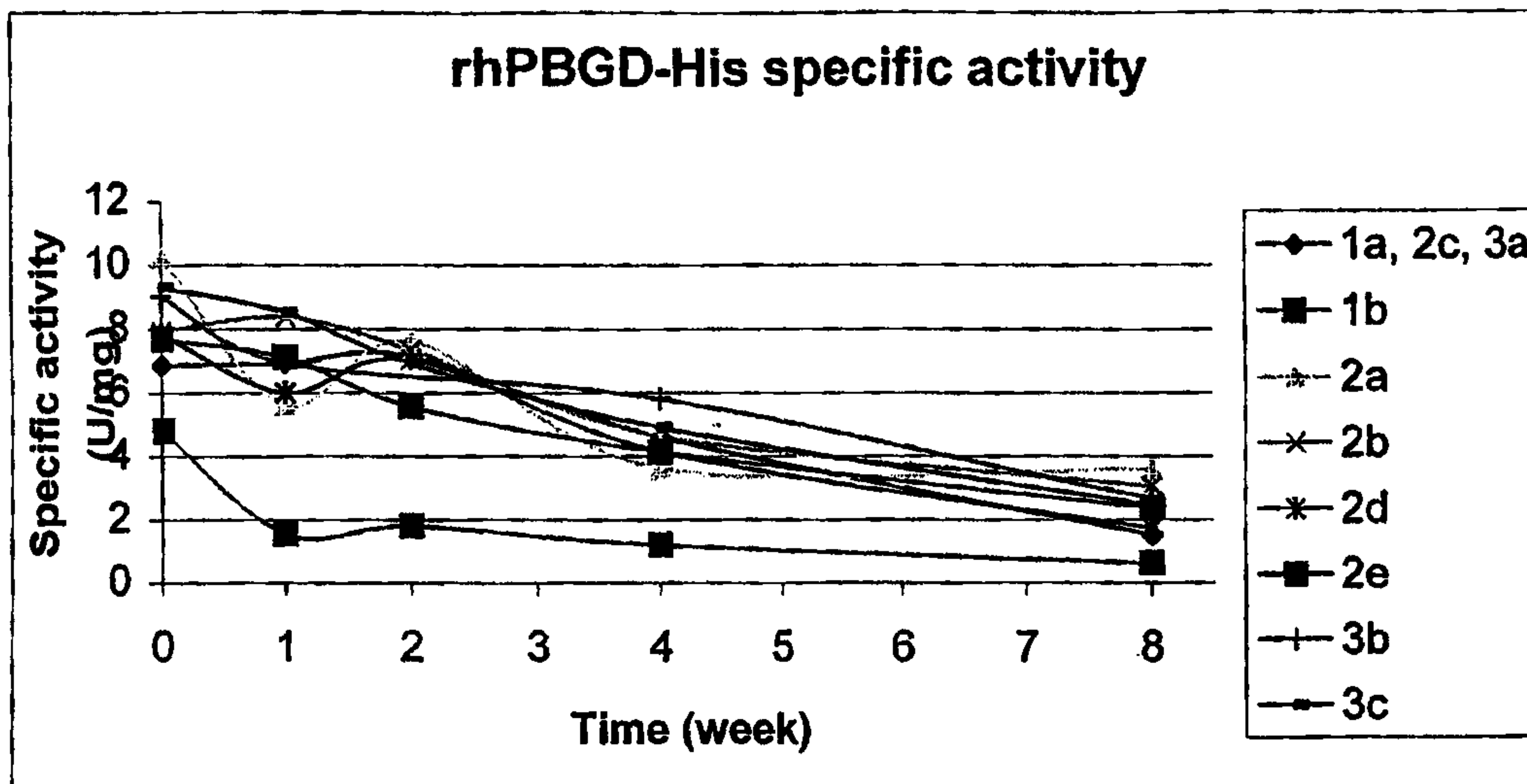
Figure 46. Enzyme specific activity measured during 8 weeks at 40°C. The activity was measured using the enzyme activity assay and the protein concentration was measured using HPLC.
