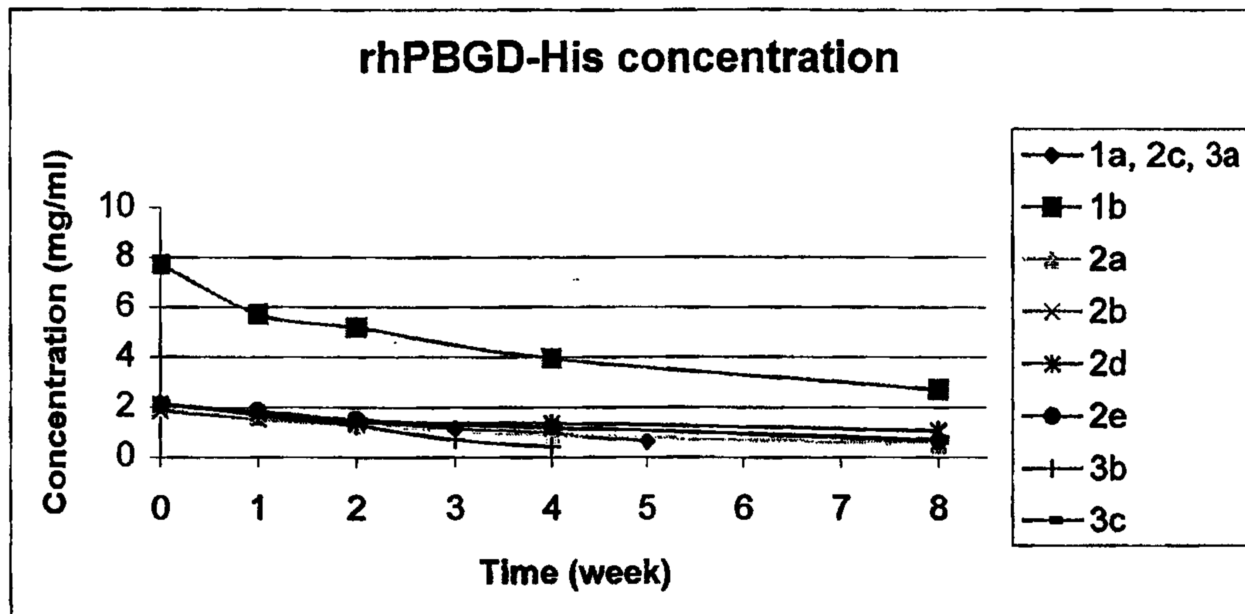
Figure 44. Enzyme concentration over 8 weeks at 40°C measured by HPLC. A decrease from 2 mg/ml to 0,5 mg/ml and 8 mg/ml to 2,5 was detected.
