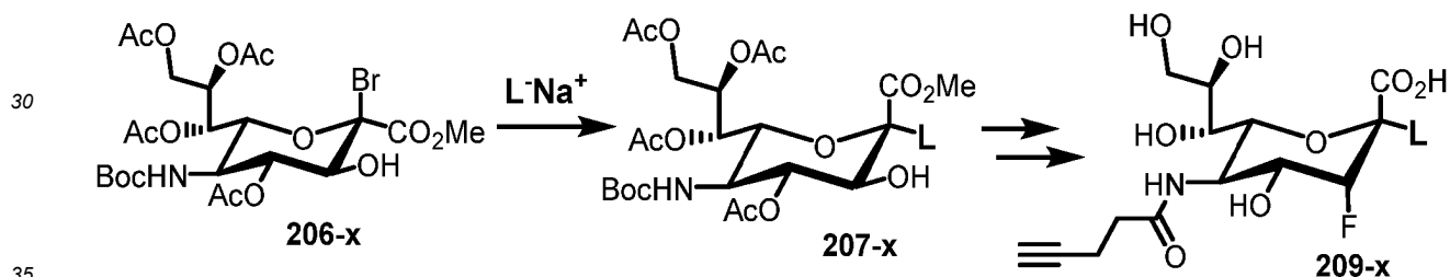
Scheme 700. Chemical synthesis of variants of the variants of compound 209 by selection of leaving group salt L^-Na^+ .
