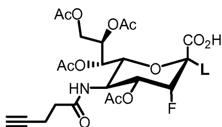
Formula (V);
