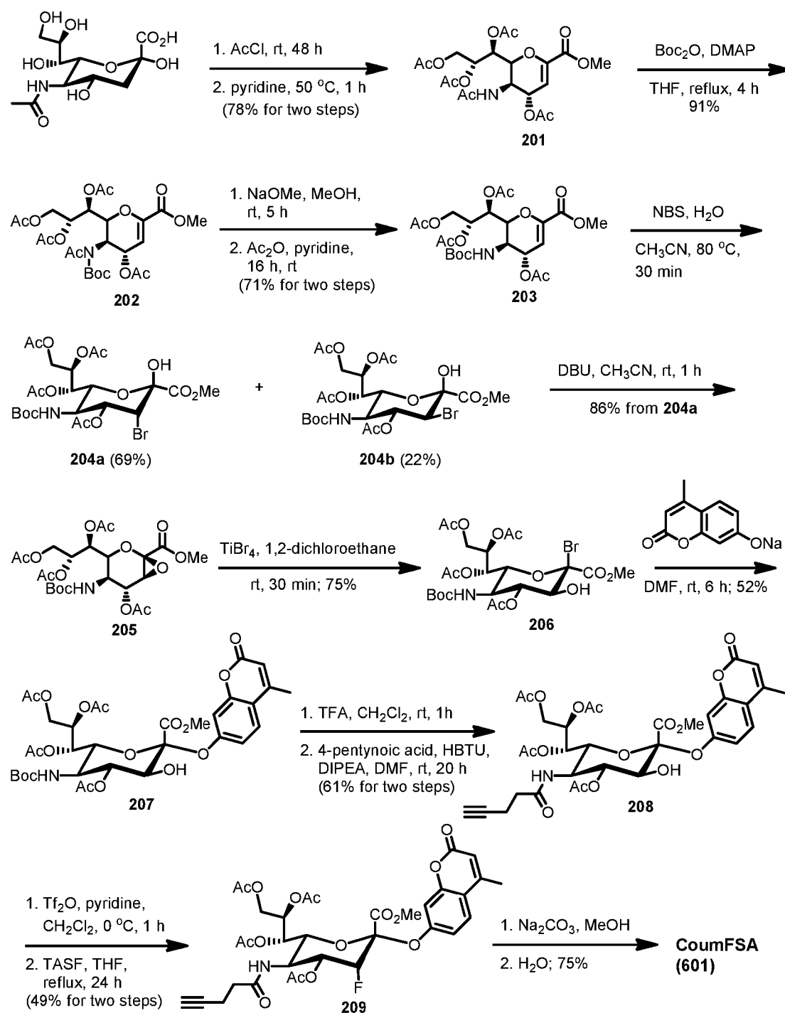
Scheme 500. Chemical synthesis of CoumFSA.
