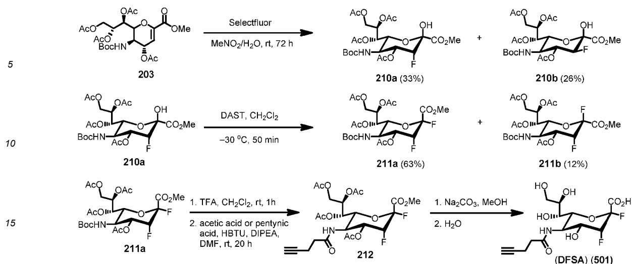
Scheme 600. Chemical synthesis of DFSA (501).
