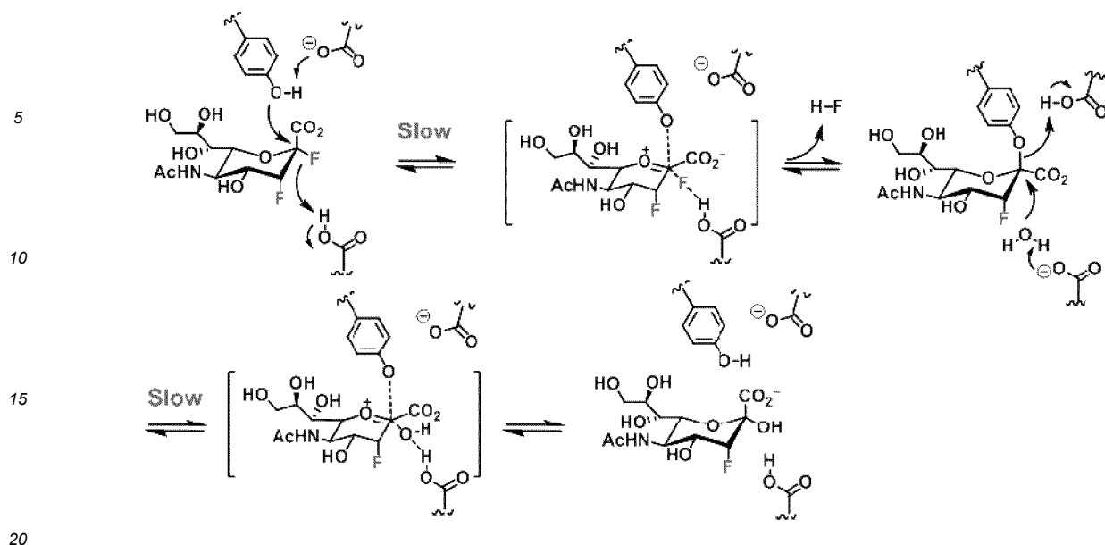
[0127] Figure 13. Mechanism and Transition State of Sialidase Enzymes acting on substrates.
