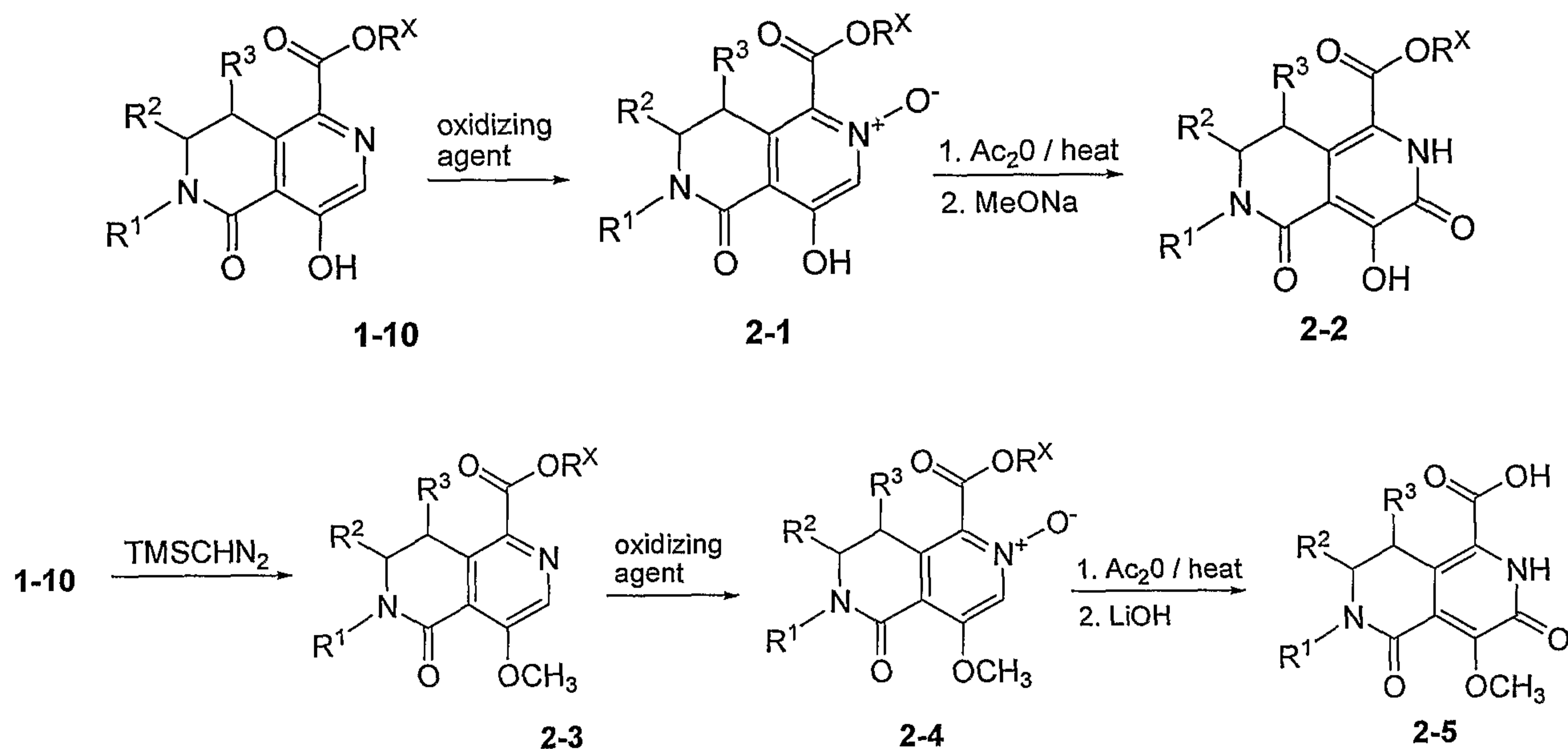
SCHEME 2
