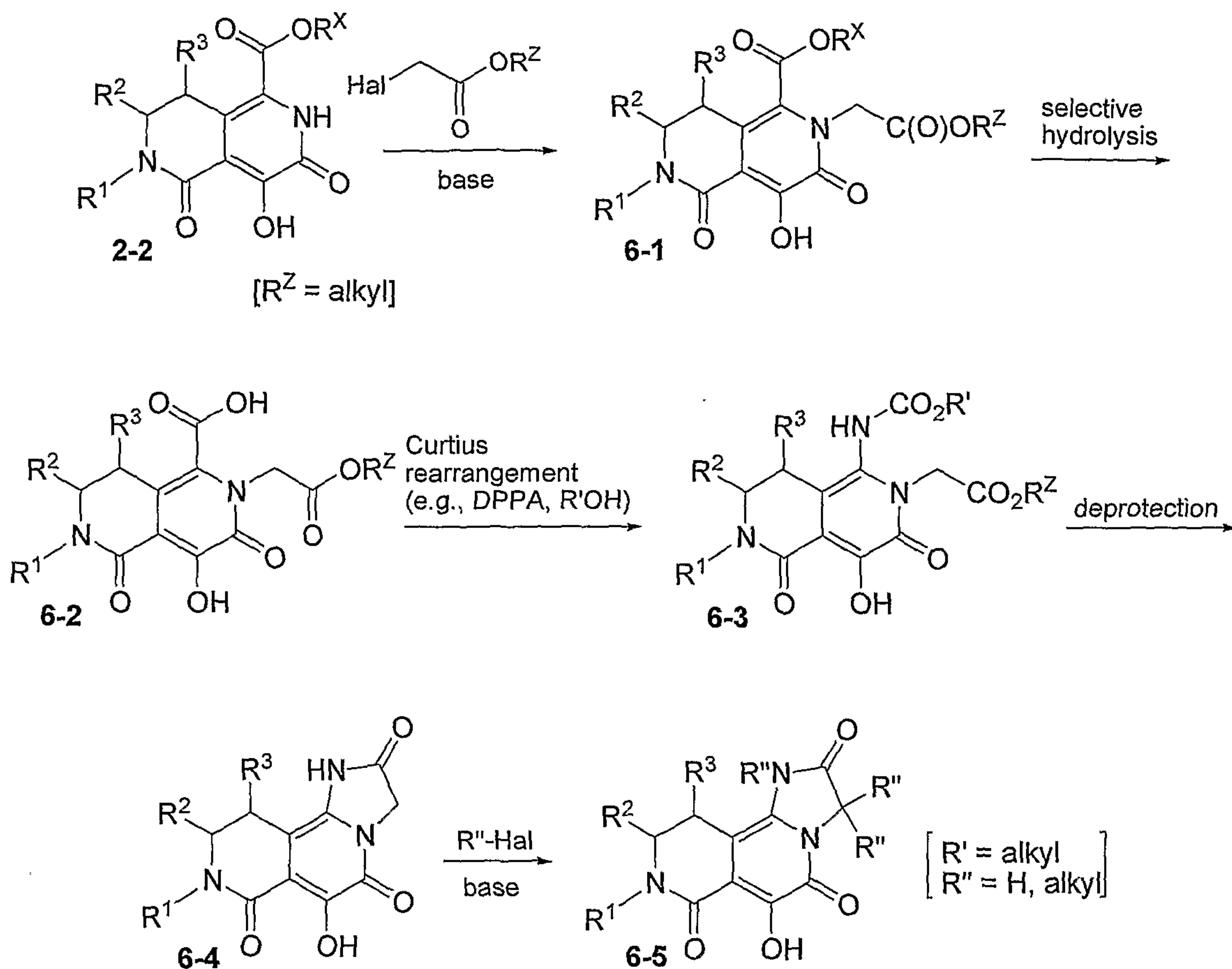
SCHEME 6
