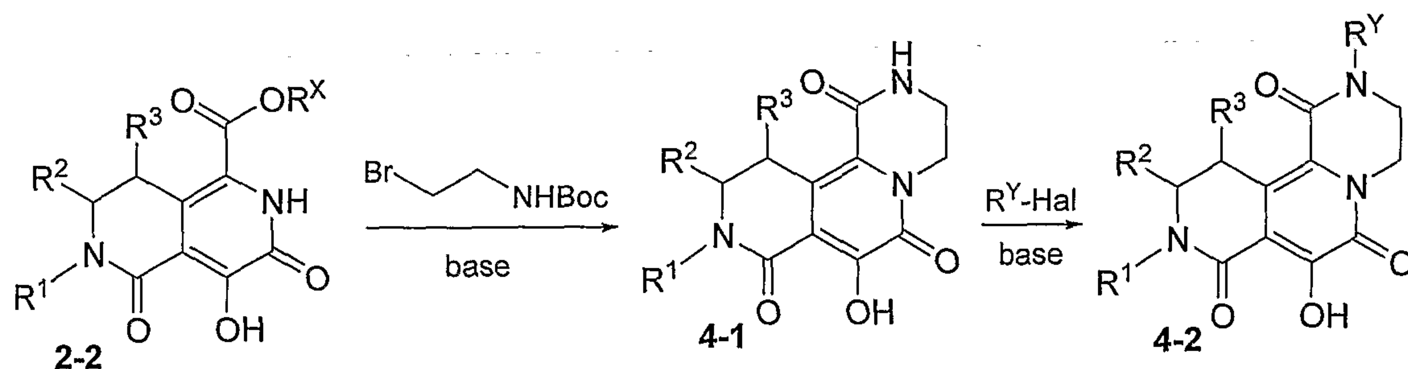
SCHEME 4
