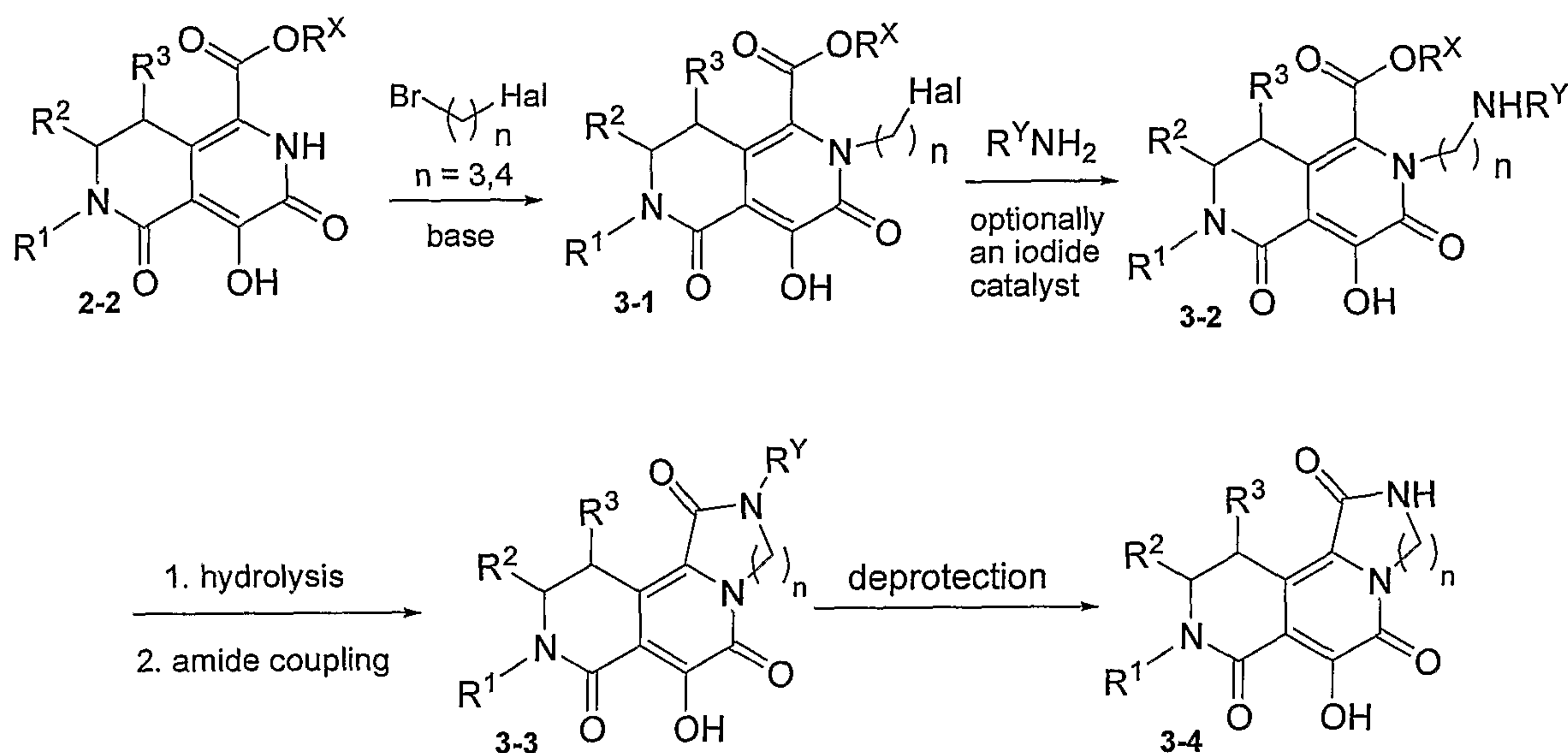
SCHEME 3
