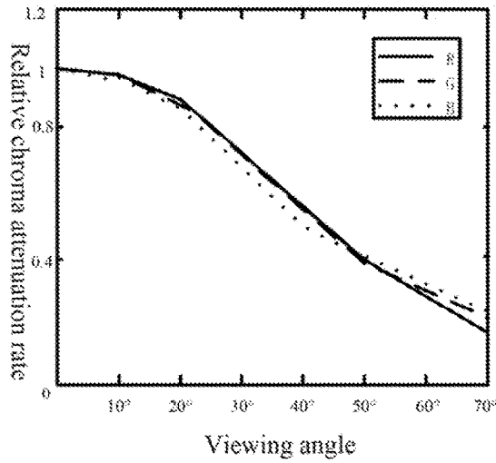
FIG. 4 (Prior art)
