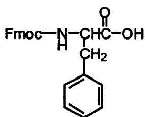
Fmoc-L-Phe-OH
