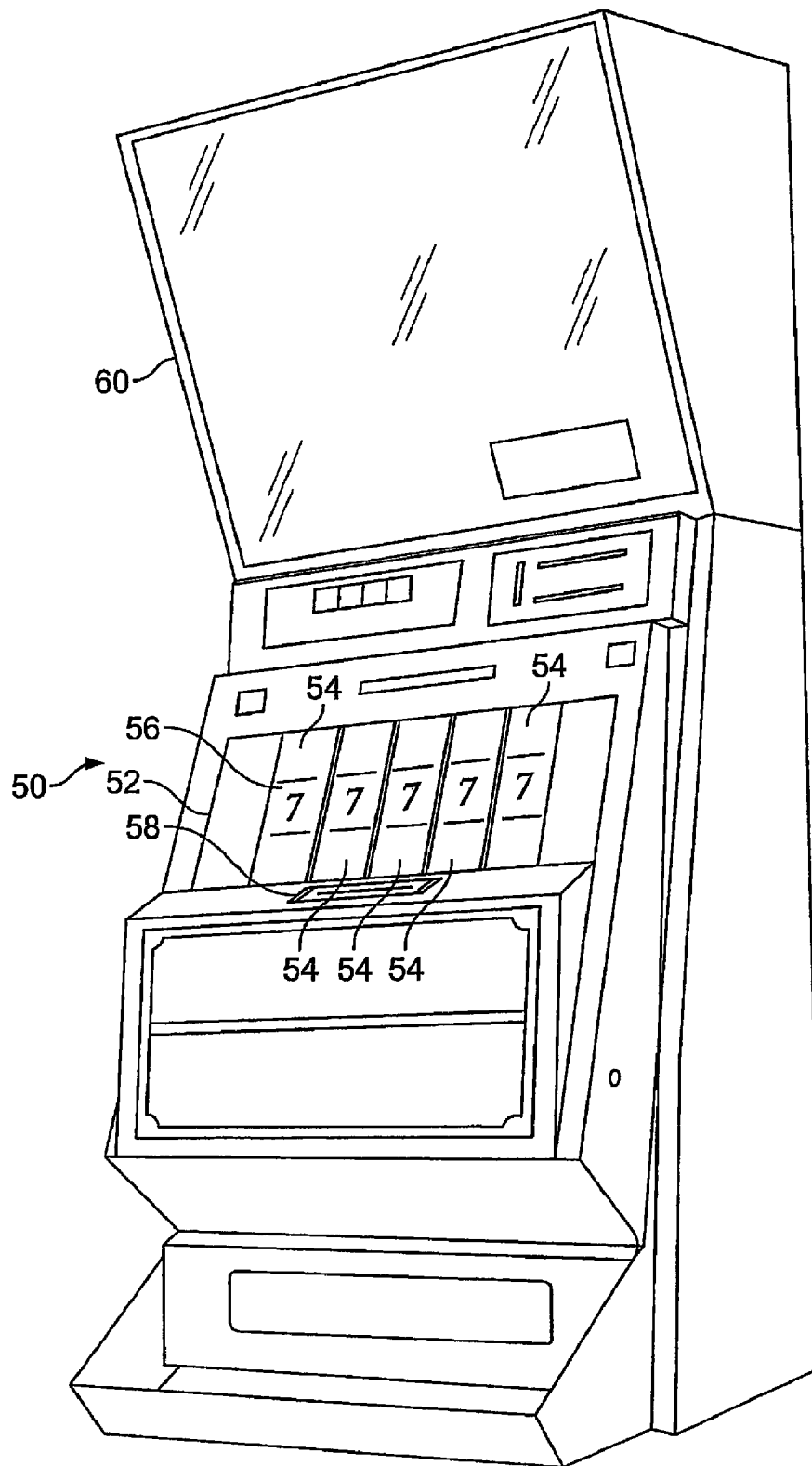
FIG. 2 (Prior Art)
