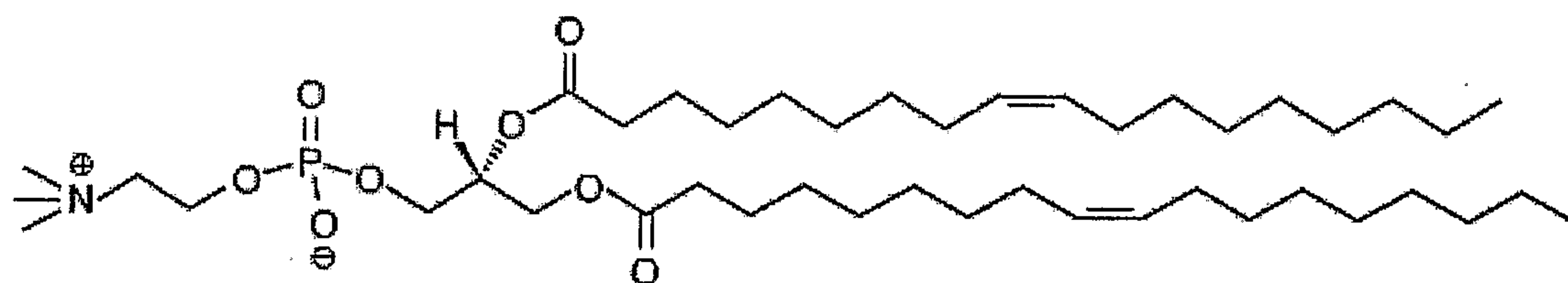
1,2-Dioleoyl-sn-Glycero-3-Phosphocholine (DOPC)
