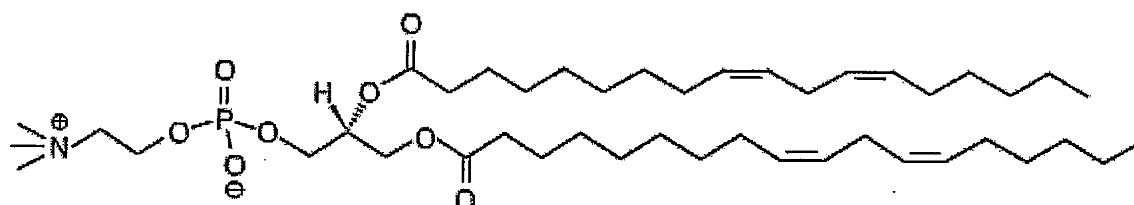
1,2-Linoleoyl-sn-Glycero-3-Phosphocholine
