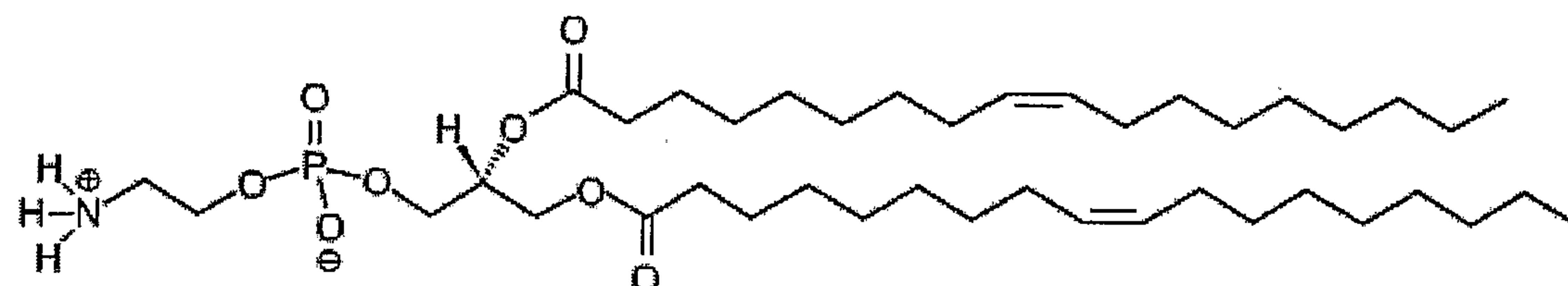
1,2-Dioleoyl-sn-Glycero-3-Phosphoethanolamine (DOPE)
