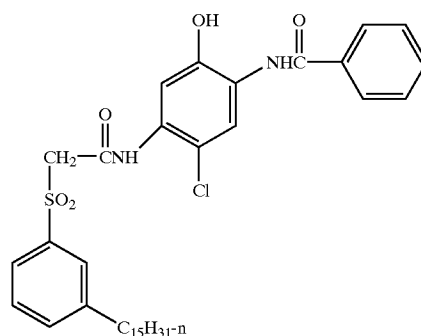
Compounds of formula (III)
