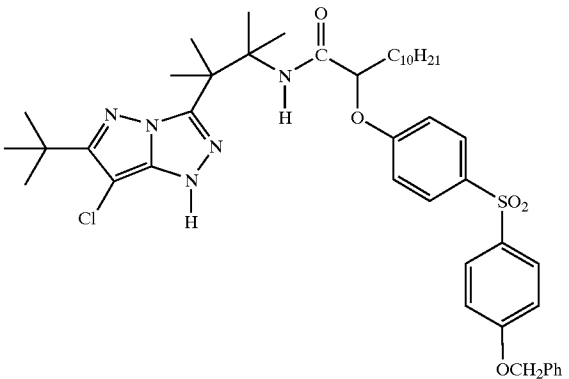
Coupler MC-1
