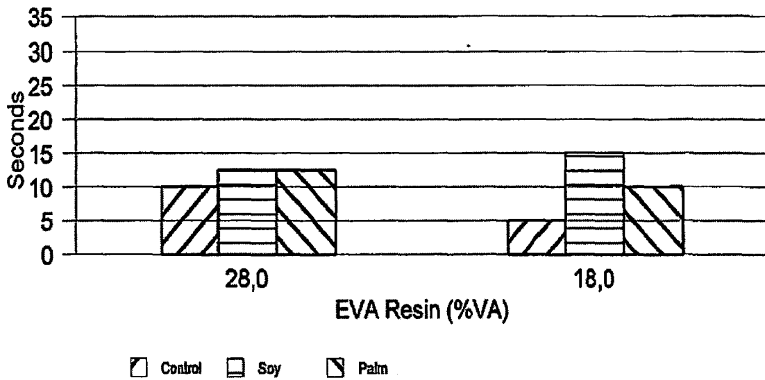
FIG. 2 Open Time (sec) ASTM D-4497
