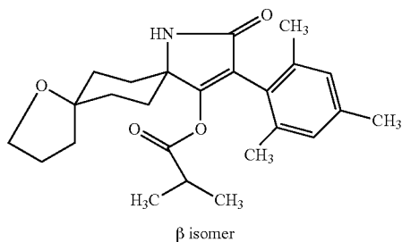
Example I-1-b-1
