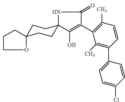
\alpha isomer
