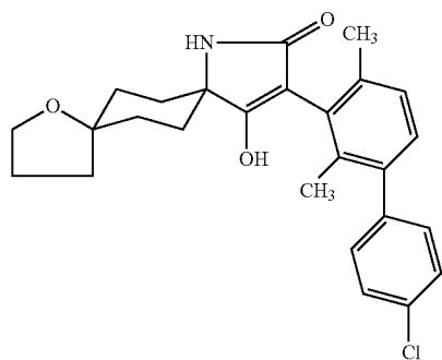
\beta isomer
