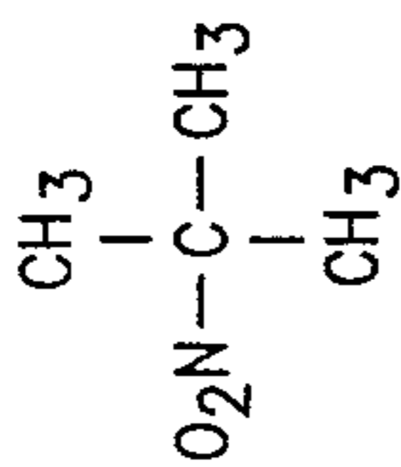
2-Methyl-2-nitropropane
