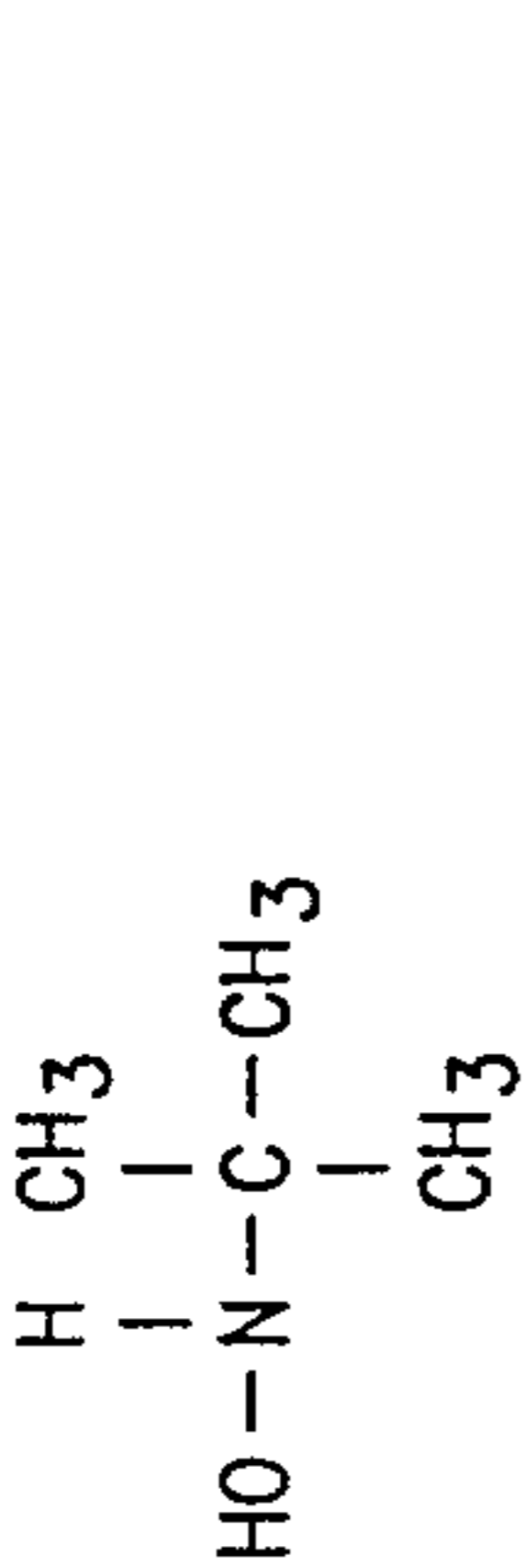
t -Butylhydroxylamine
