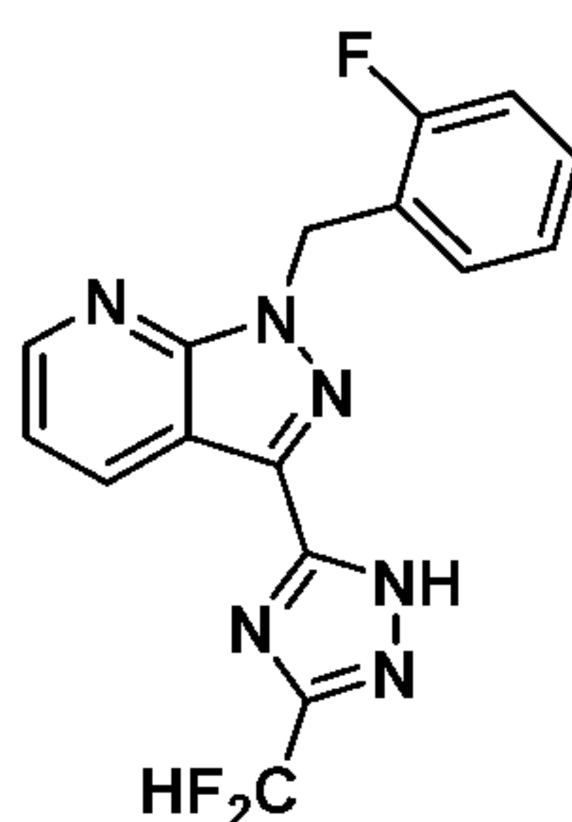
Compound I-20
