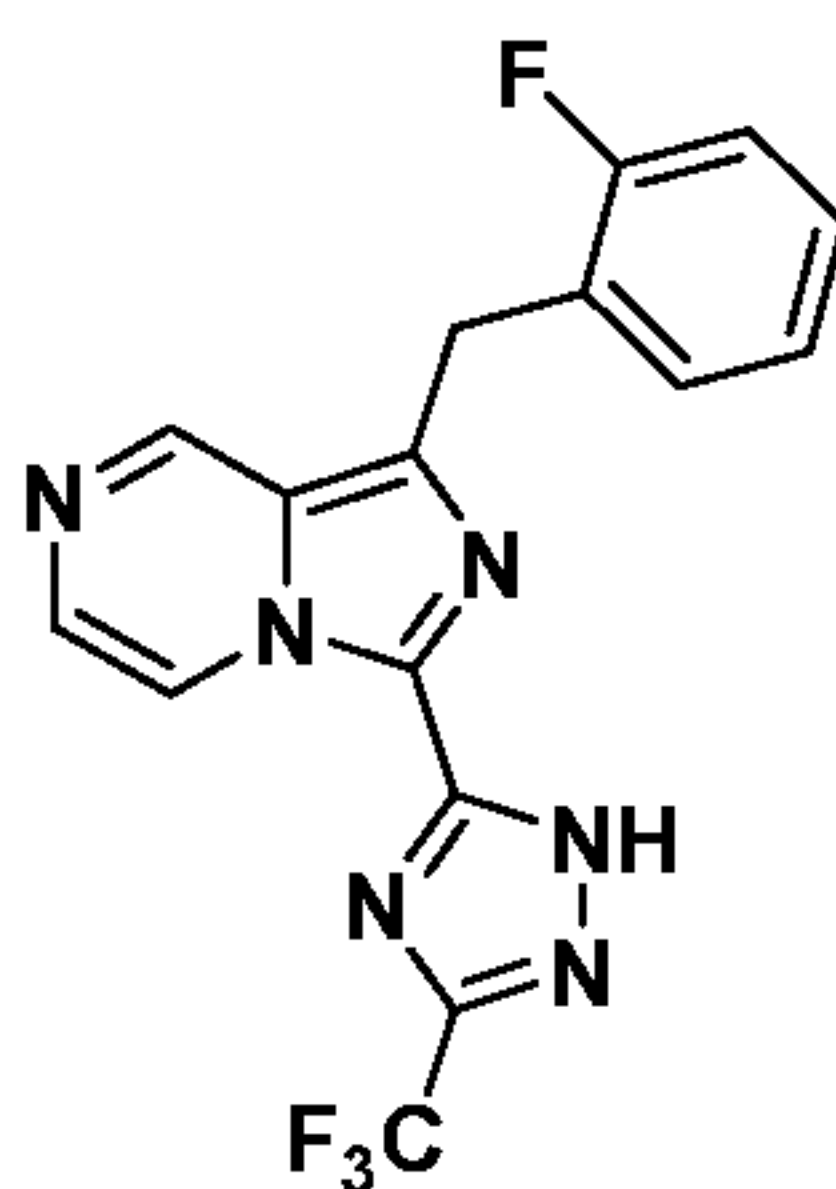
Compound I-44
