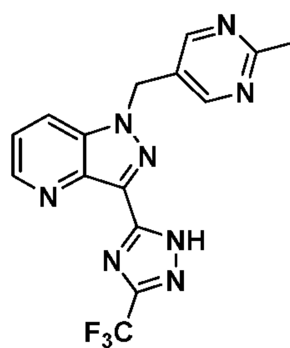
Compound I-38
