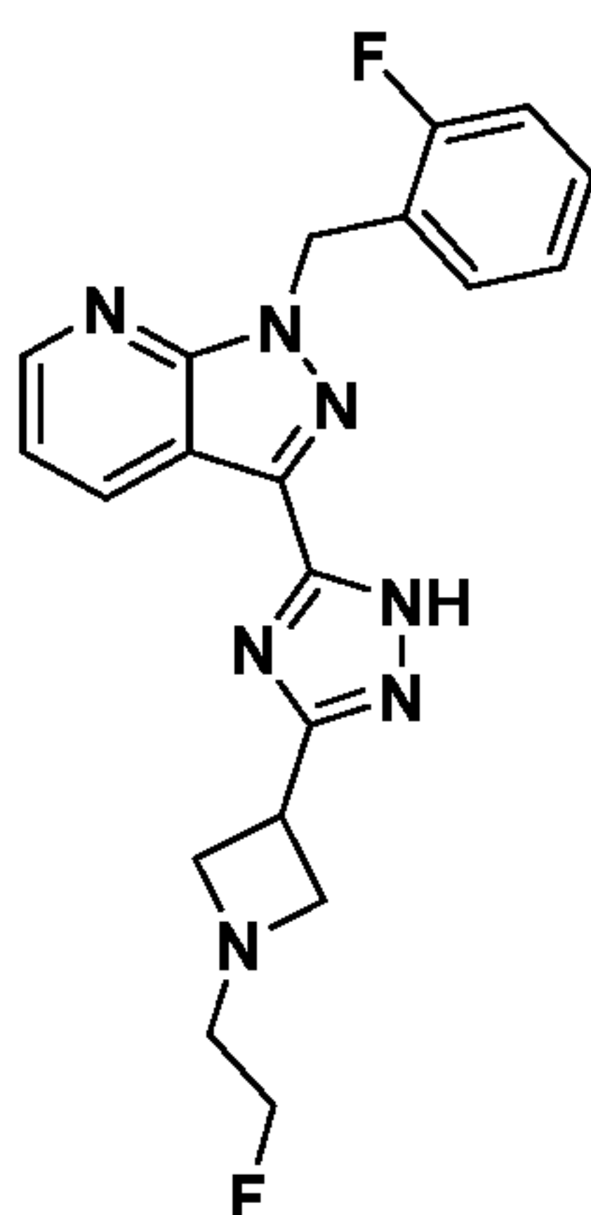
Compound I-97
