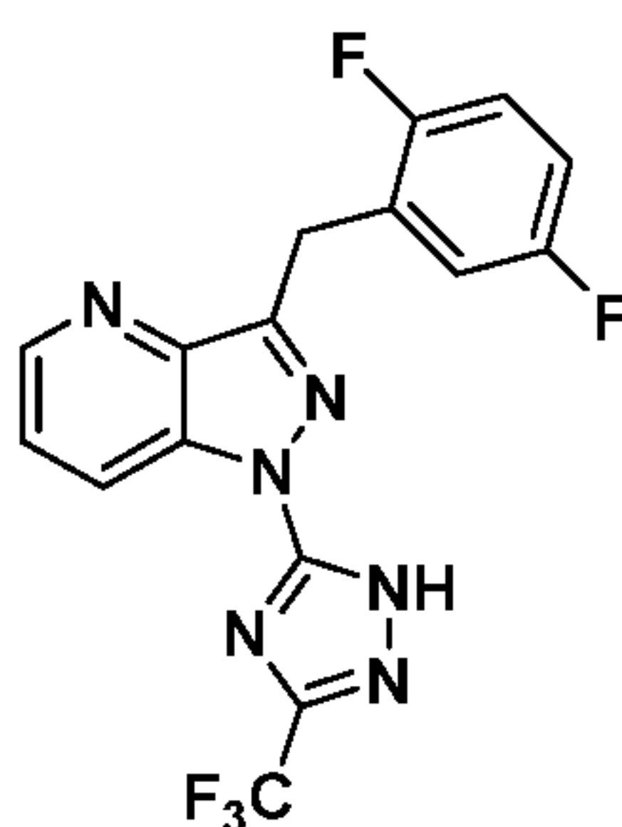
Compound I-130
