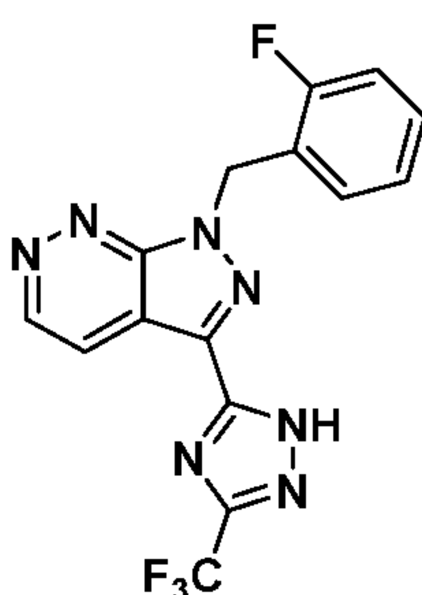
Compound I-100
