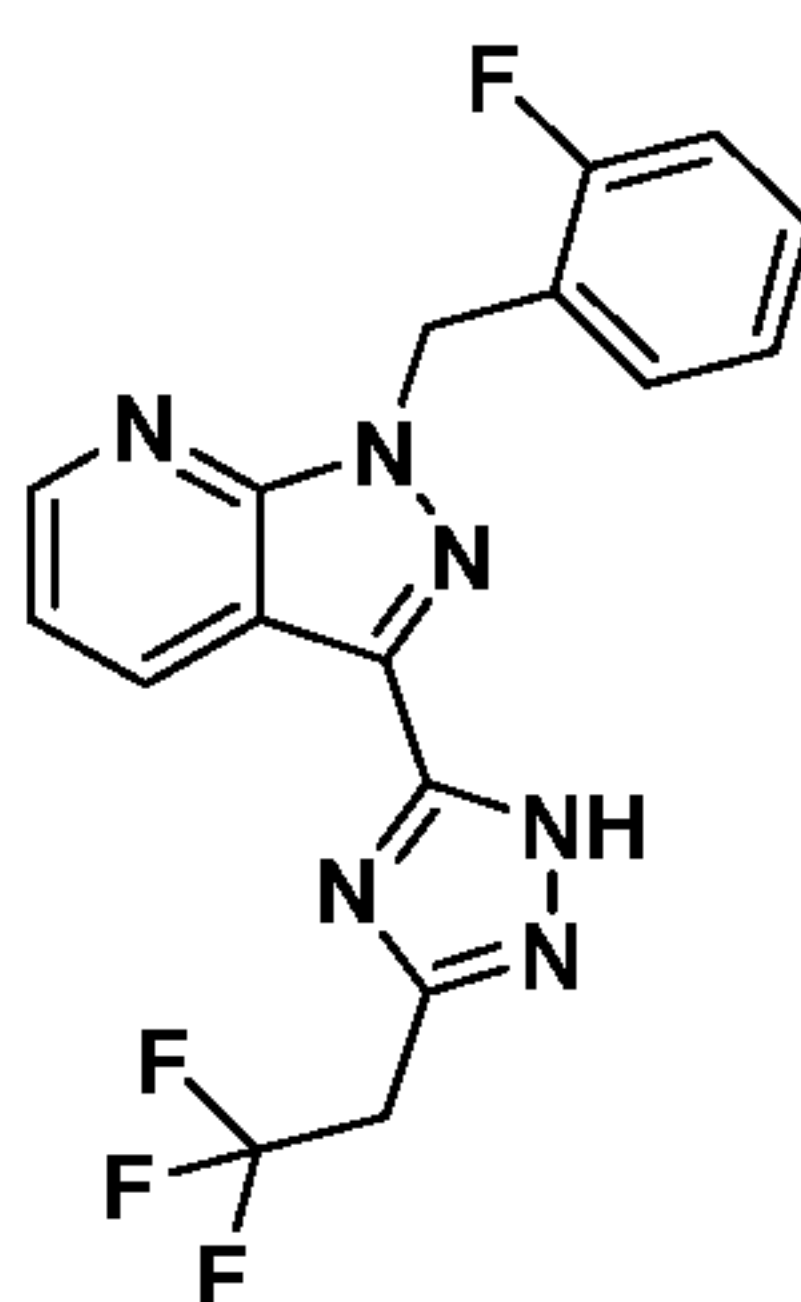
Compound I-26
