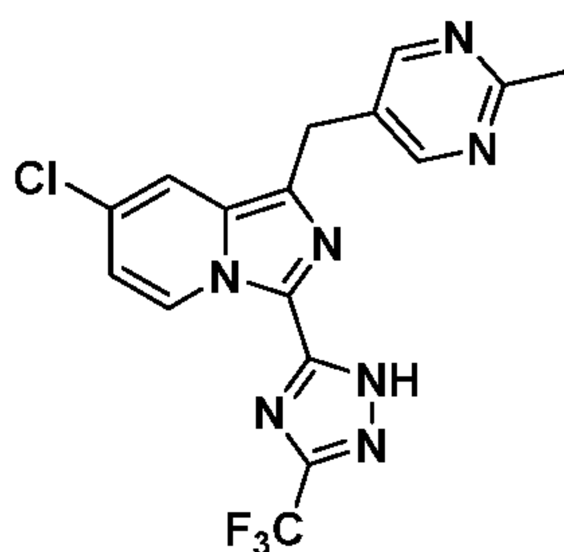
Compound I-29
