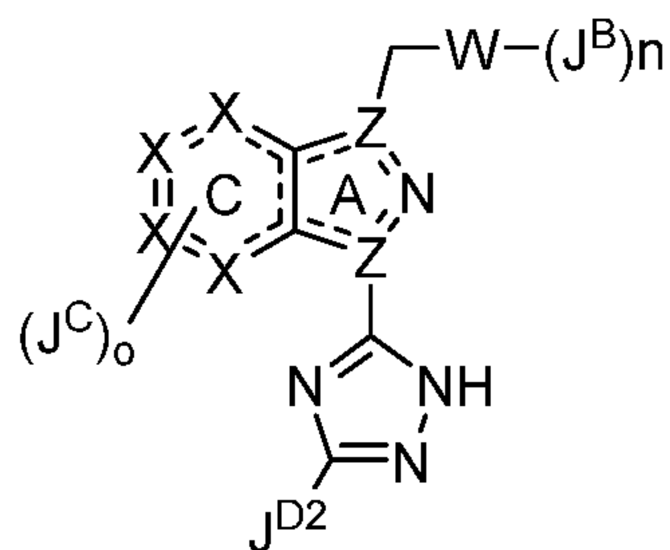
Formula IIA
