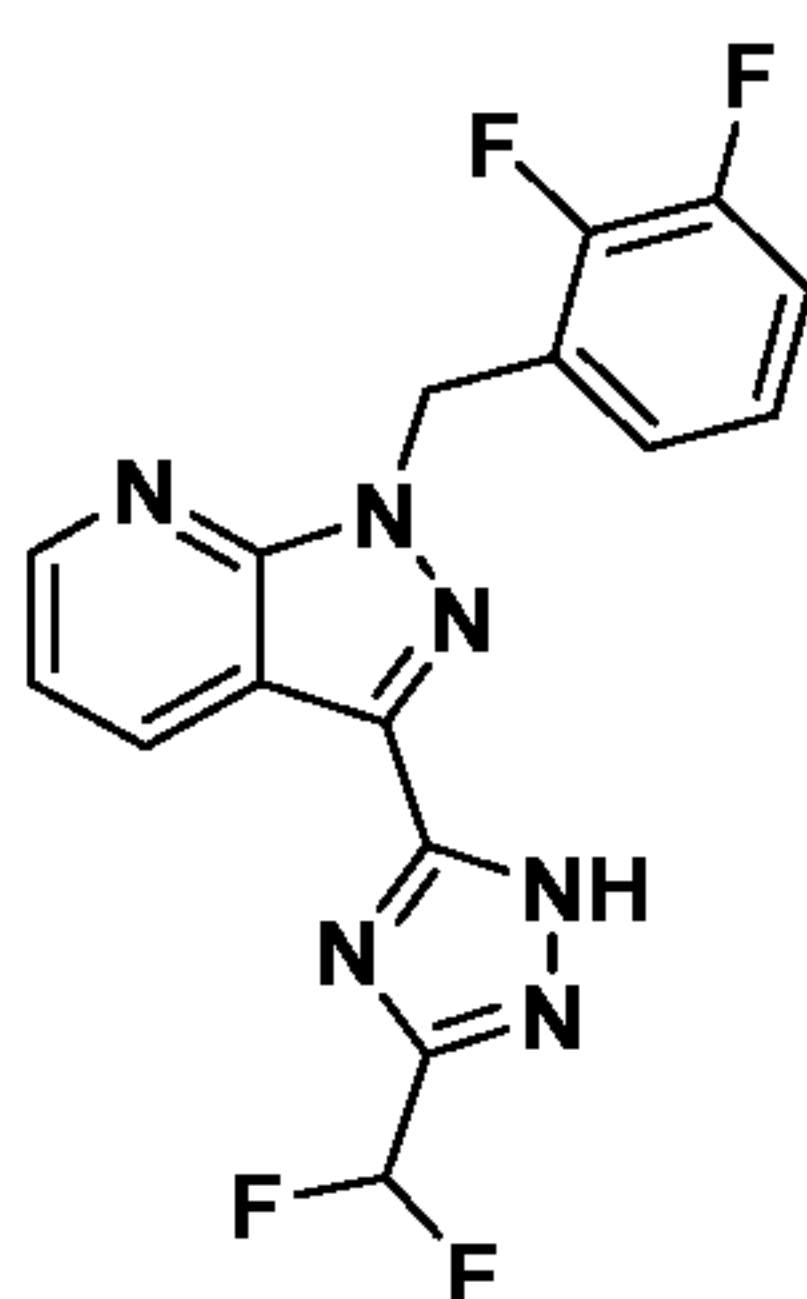
Compound I-67
