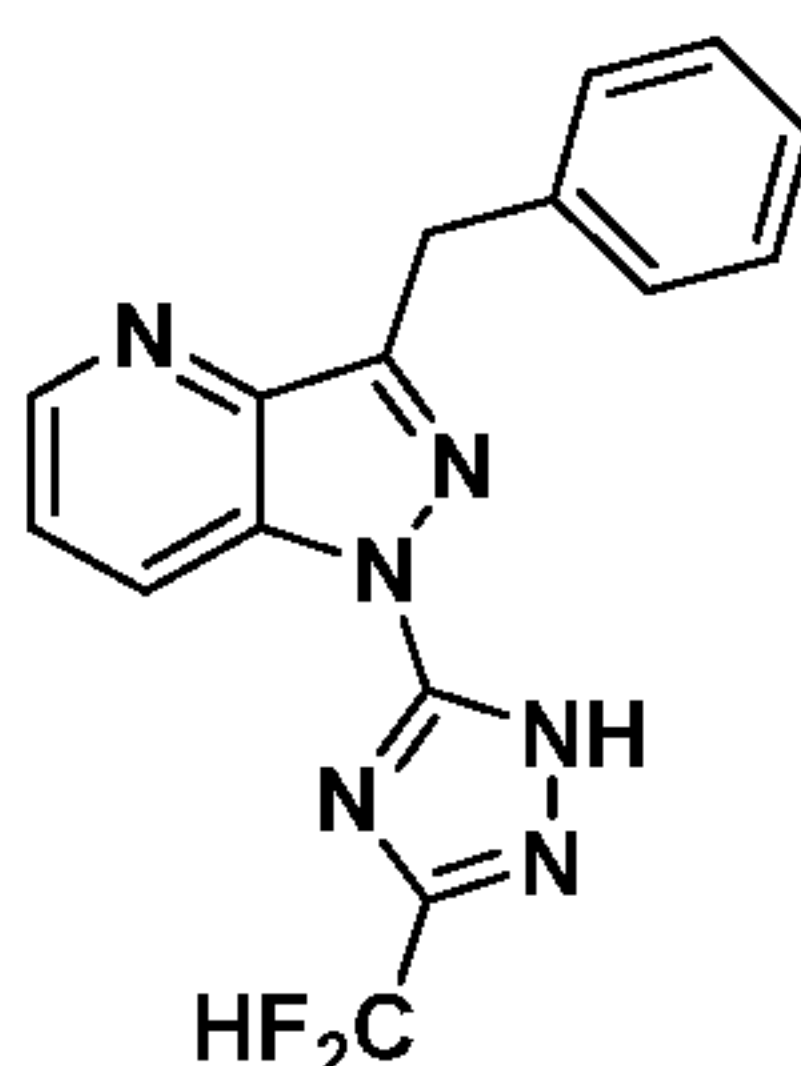
Compound I-129
