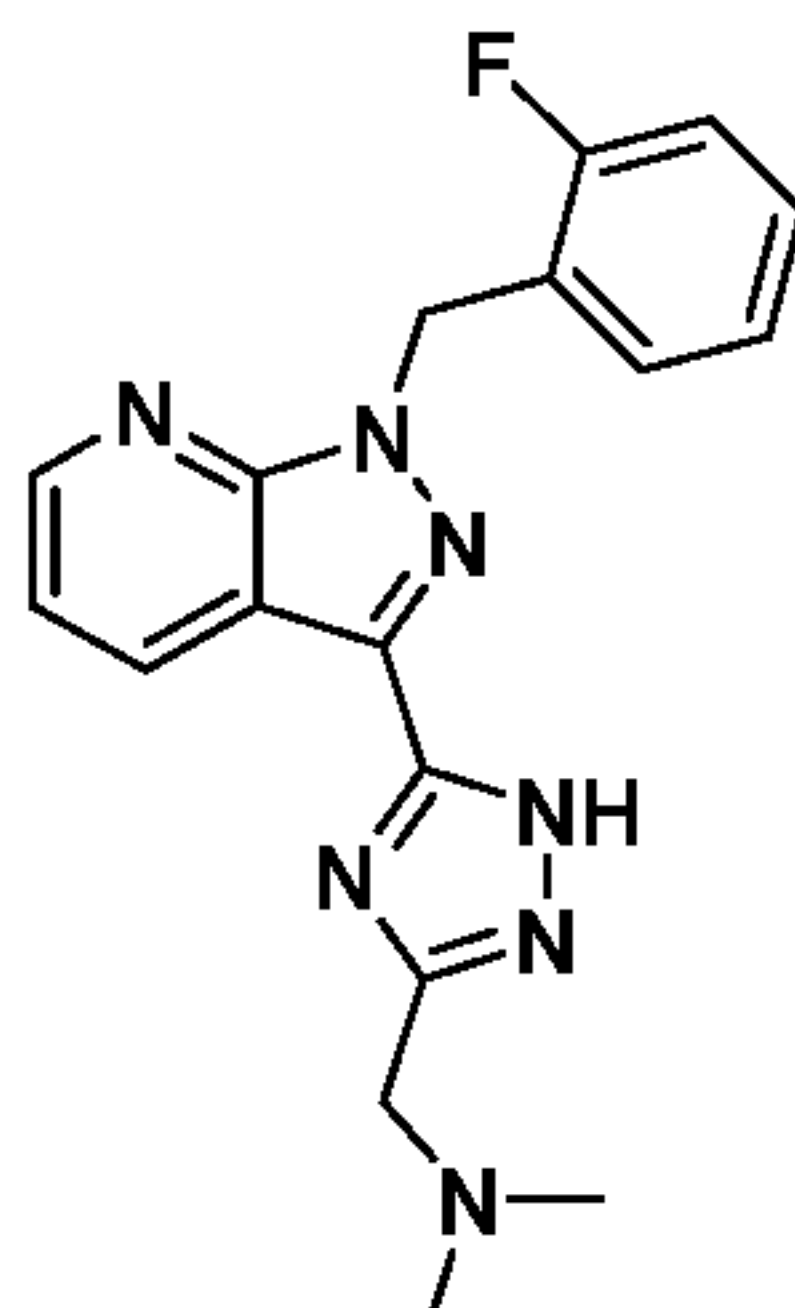
Compound I-106
