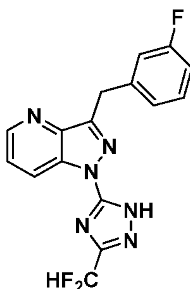
Compound I-122
