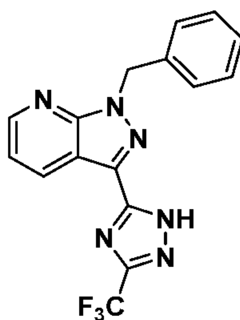
Compound I-49
