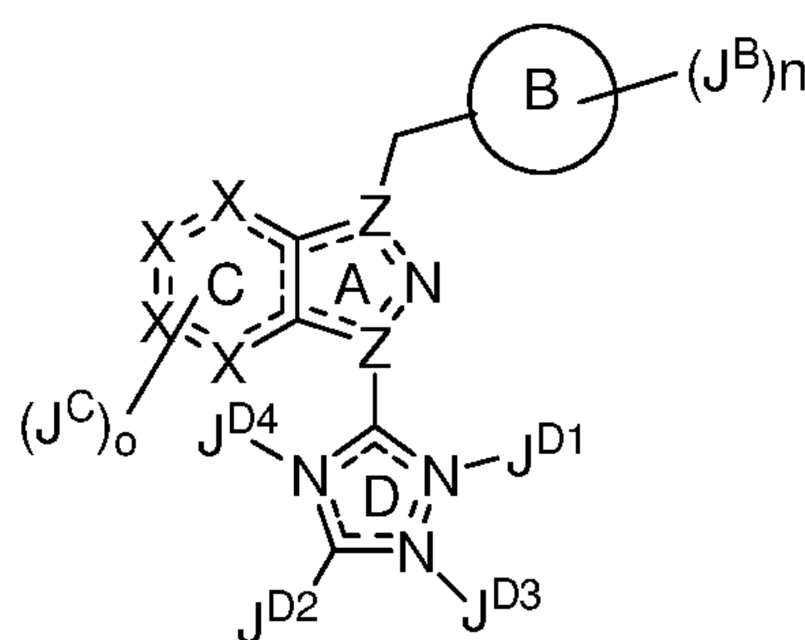
Formula IV.
