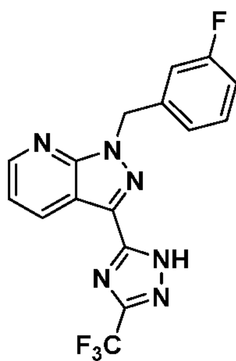
Compound I-52
