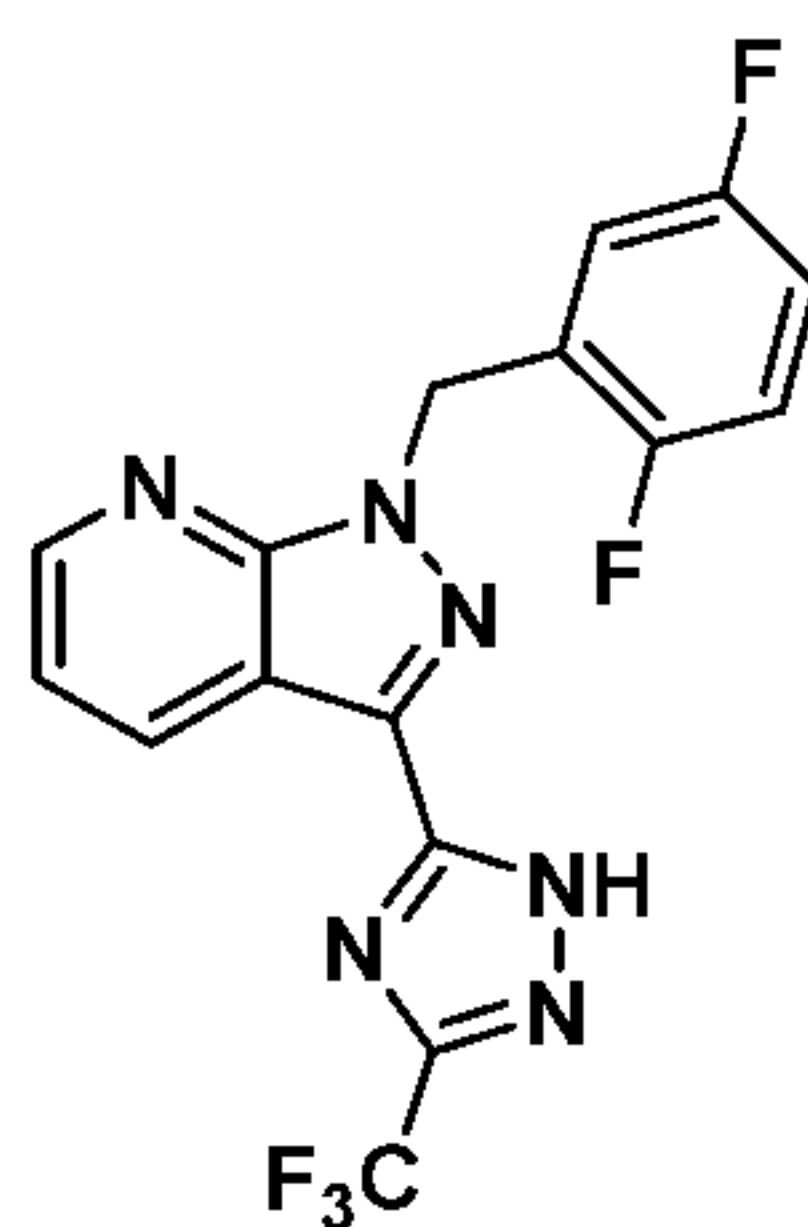
Compound I-14
