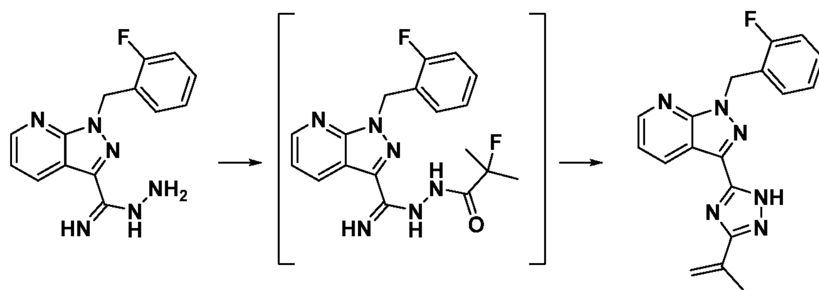
Compound I-55
