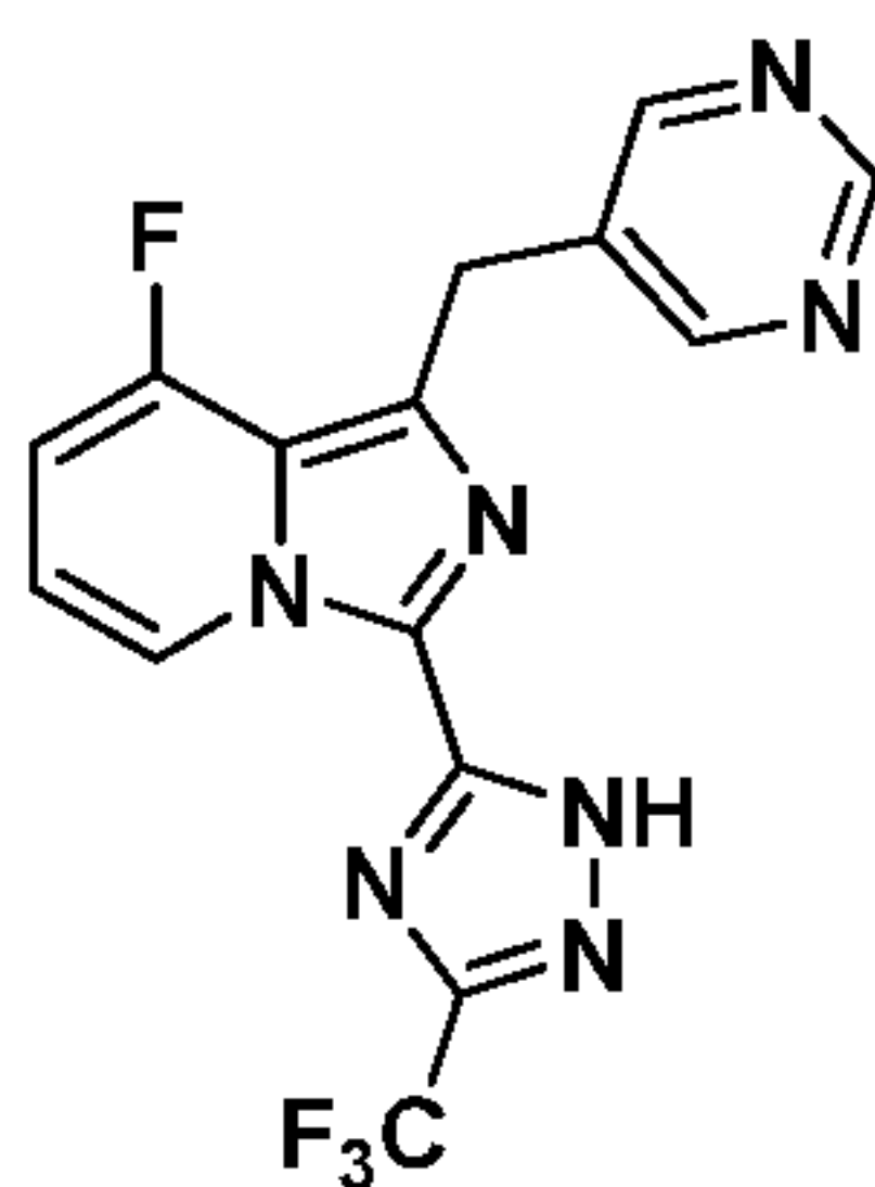
Compound I-15
