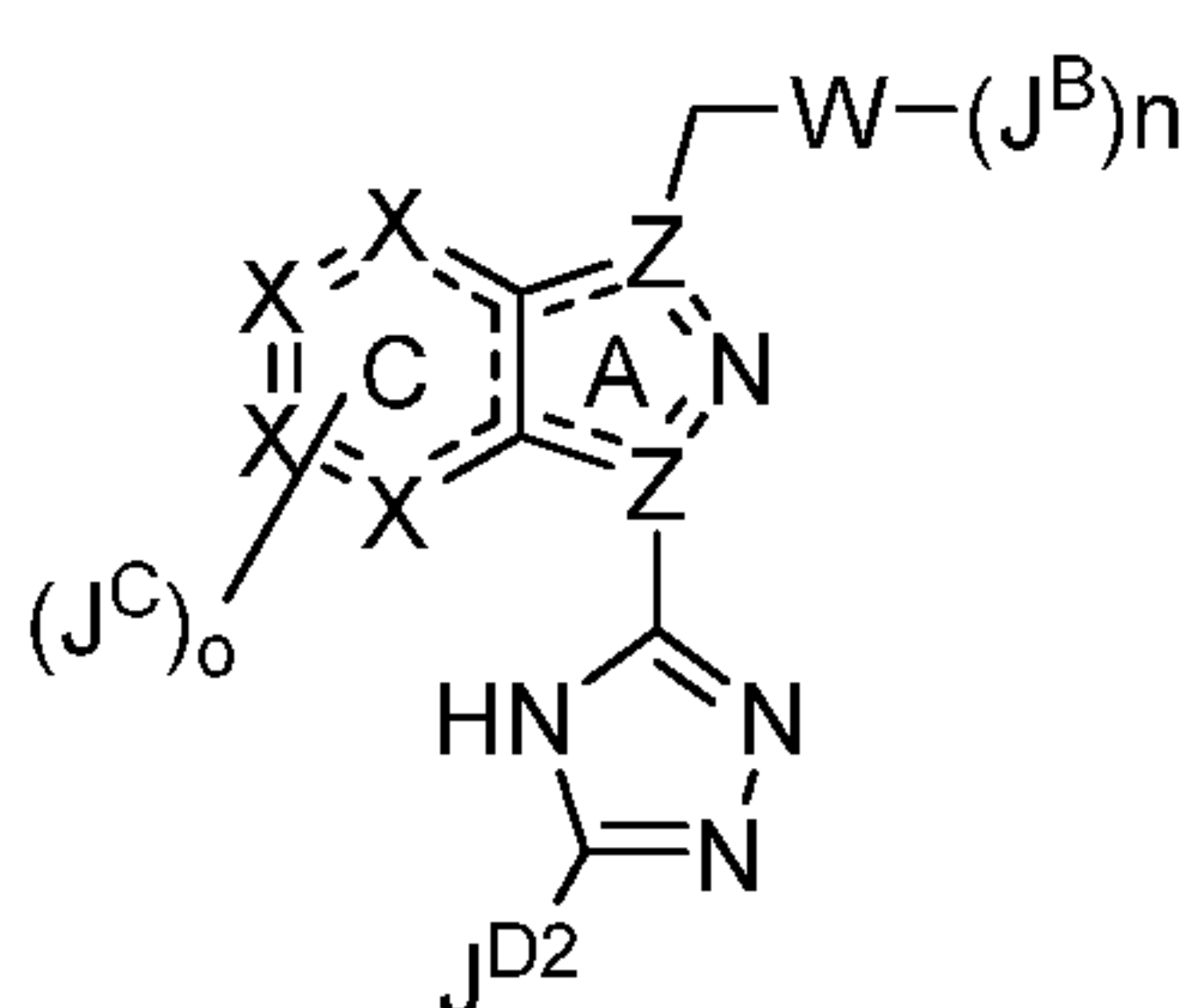
Formula IIB
