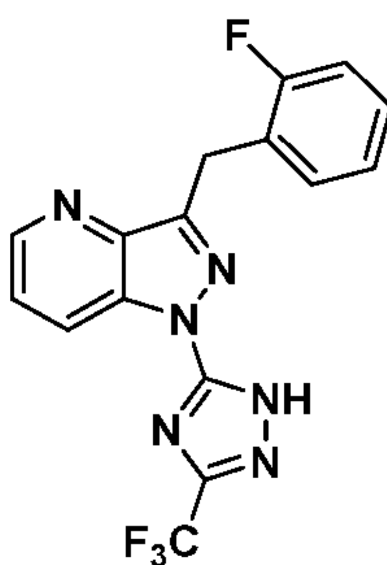
Compound I-31
