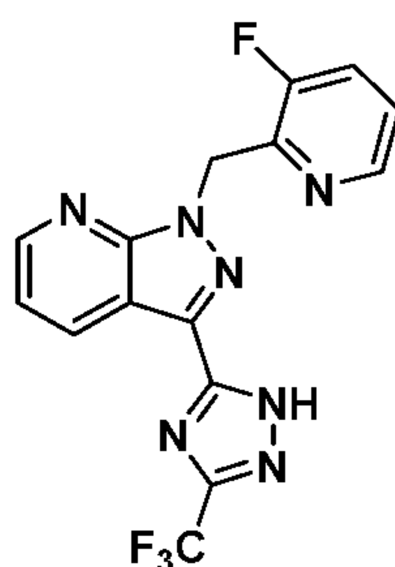
Compound I-13
