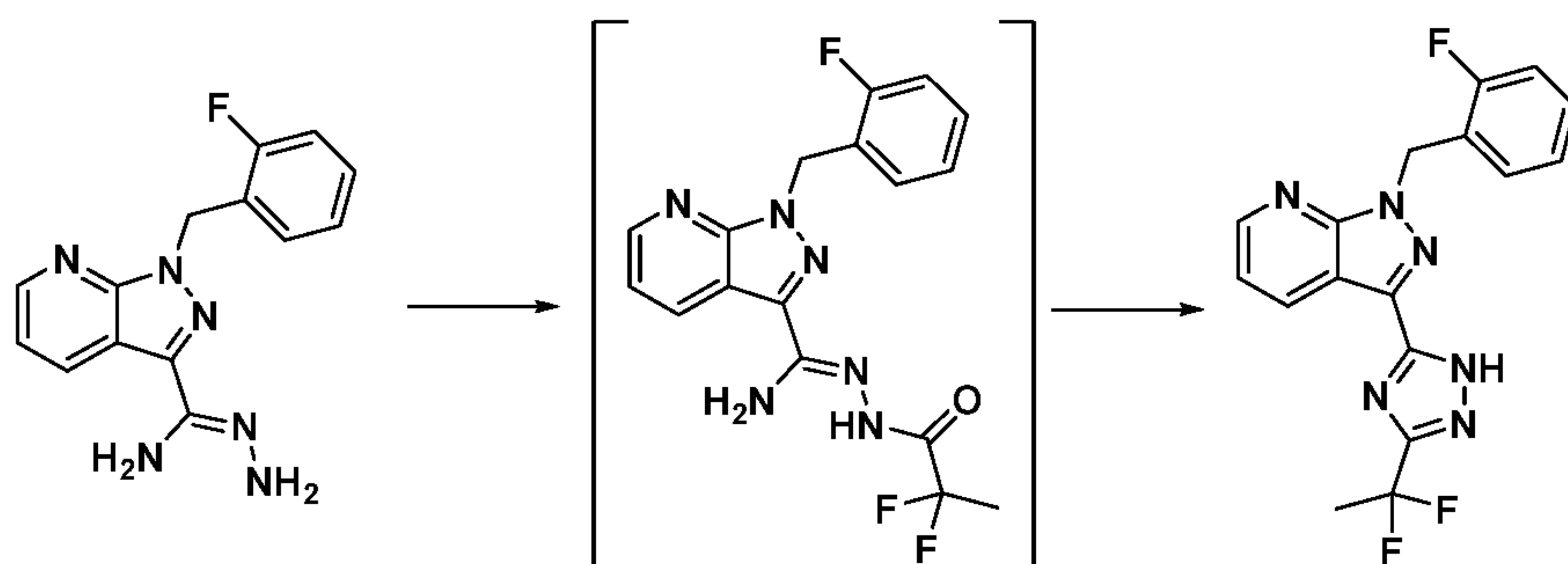
Compound I-36
