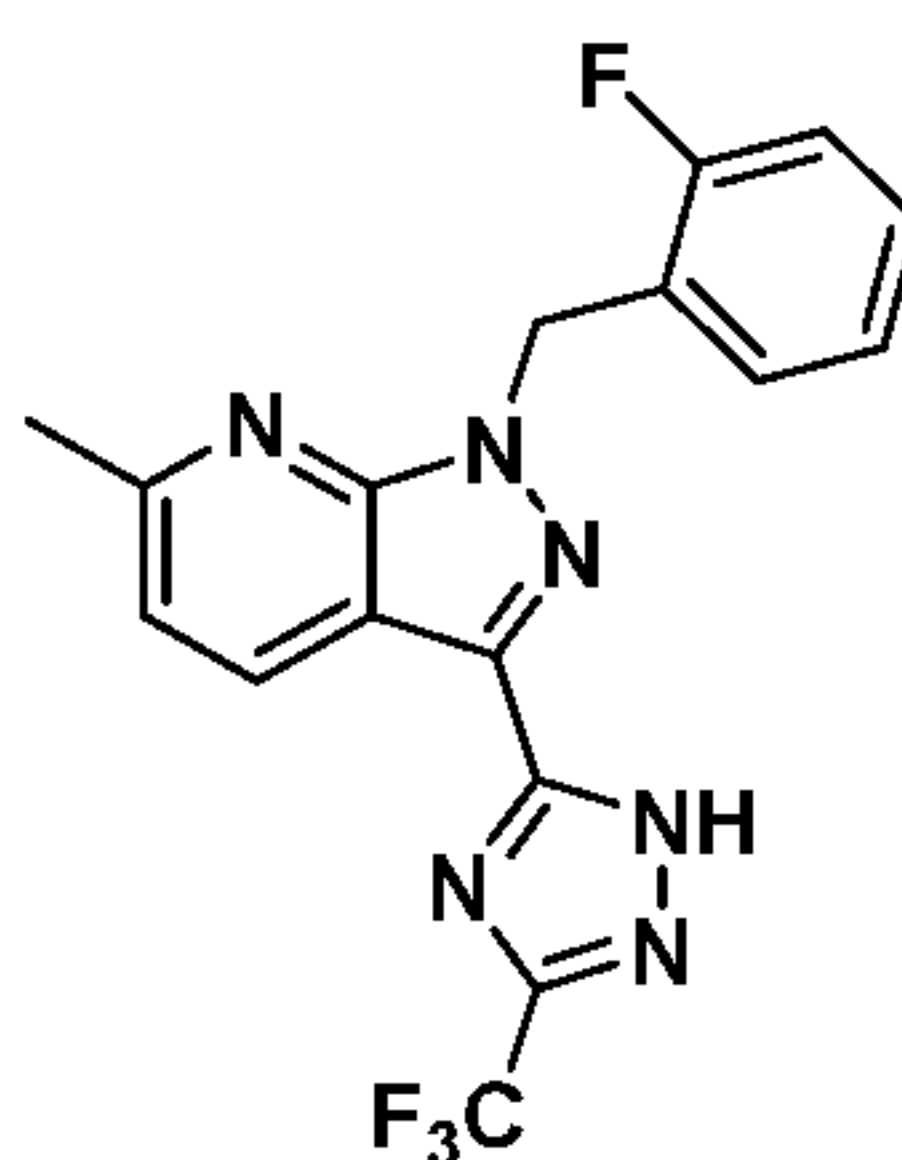
Compound I-50
