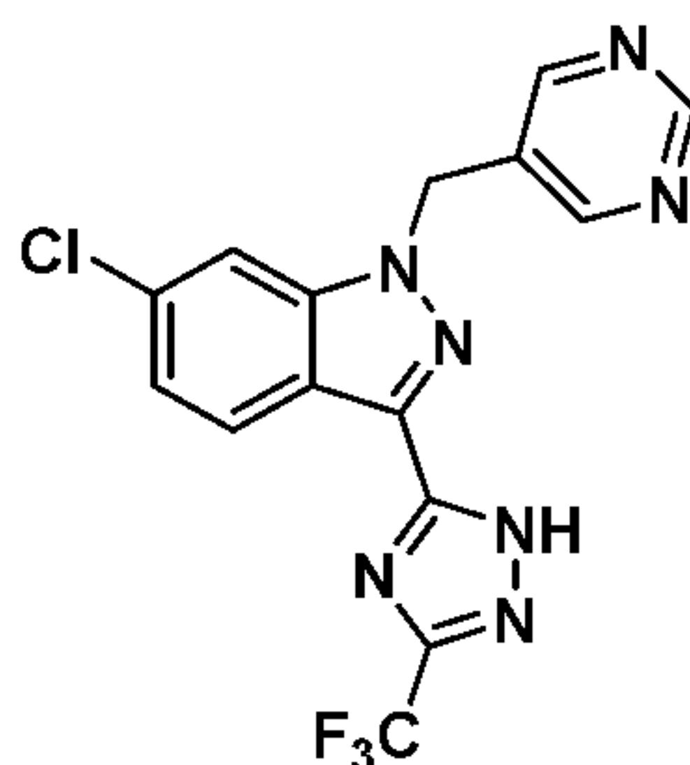
Compound I-16
