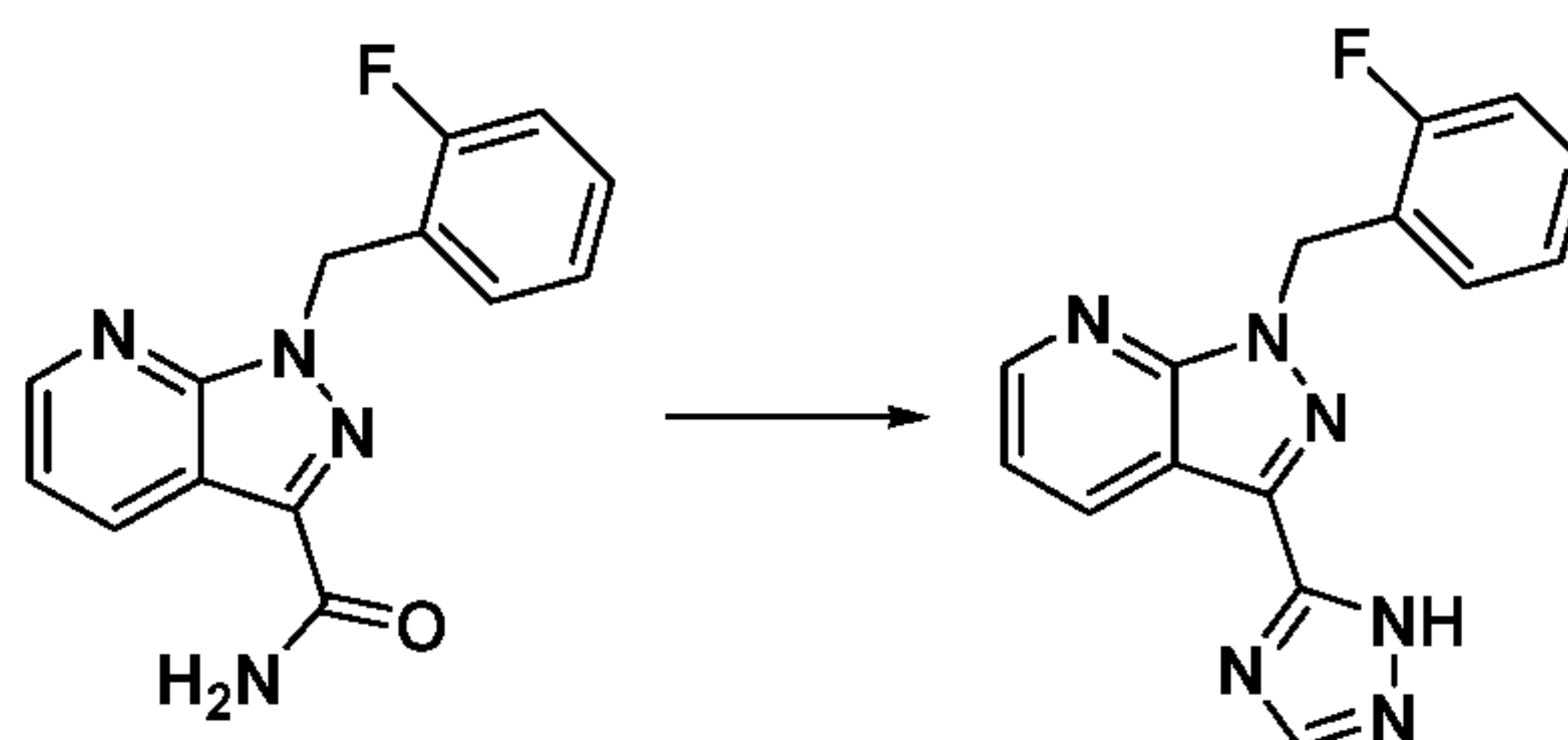
Compound I-25
