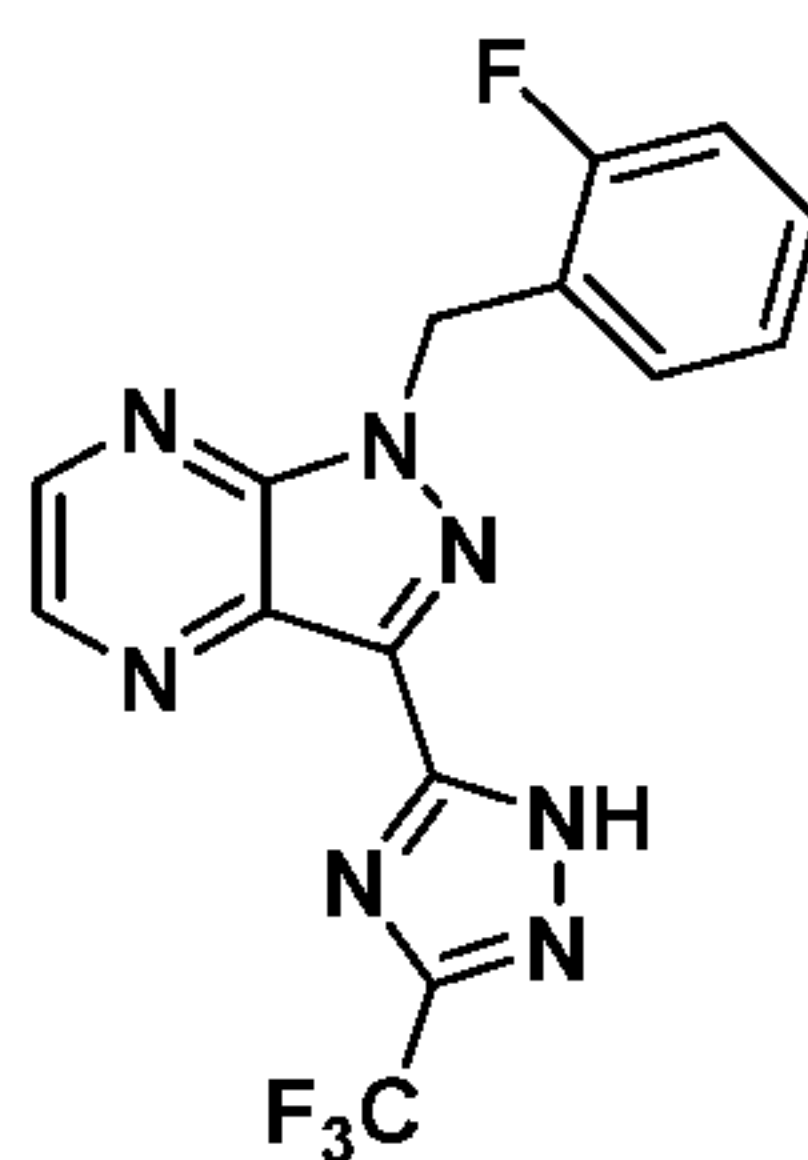
Compound I-98
