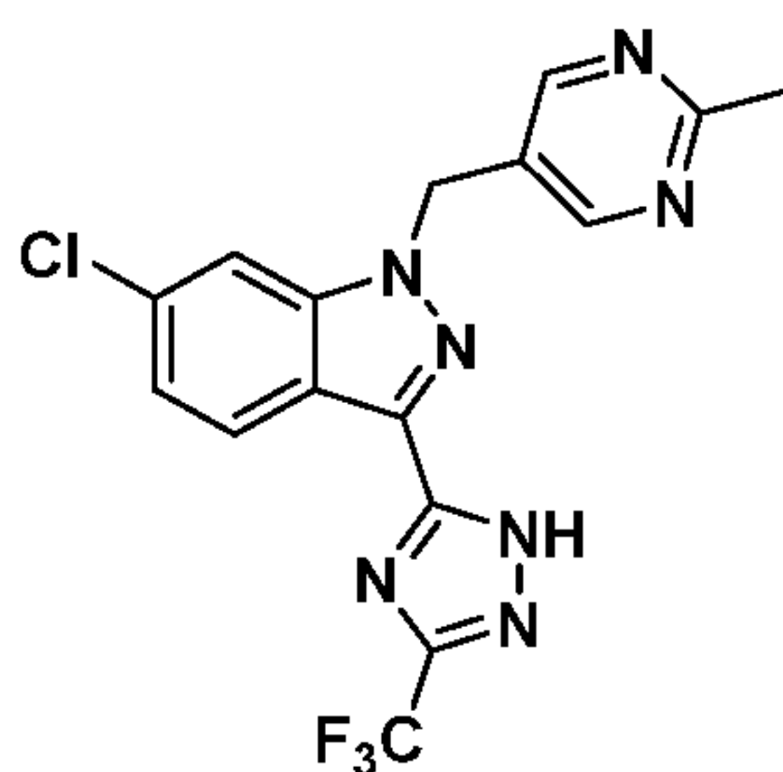
Compound I-22
