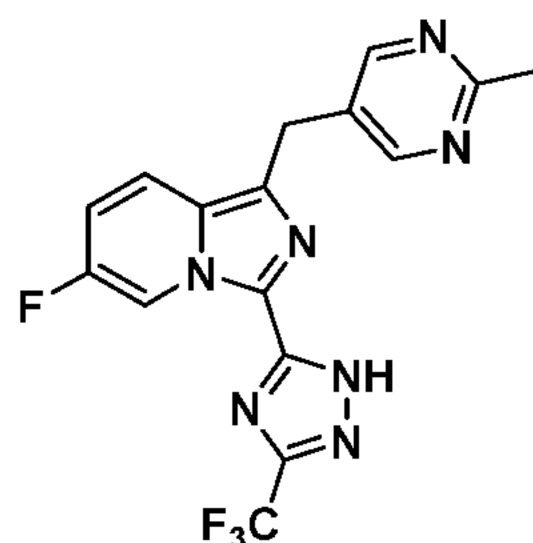
Compound I-23
