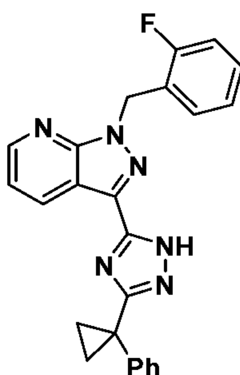
Compound I-81
