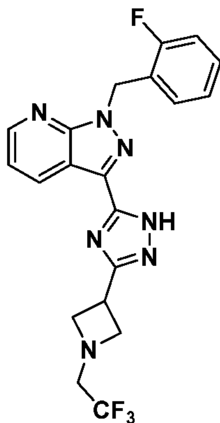
Compound I-95
