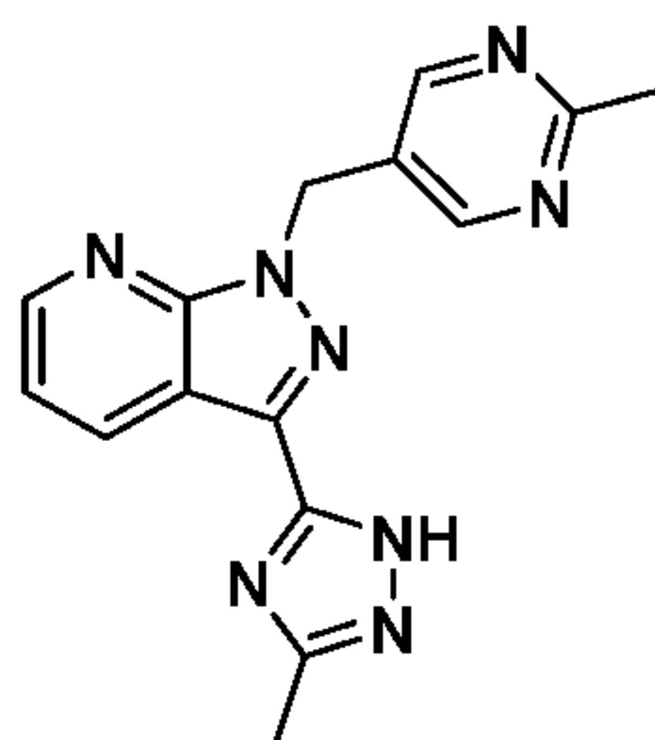
Compound I-113
