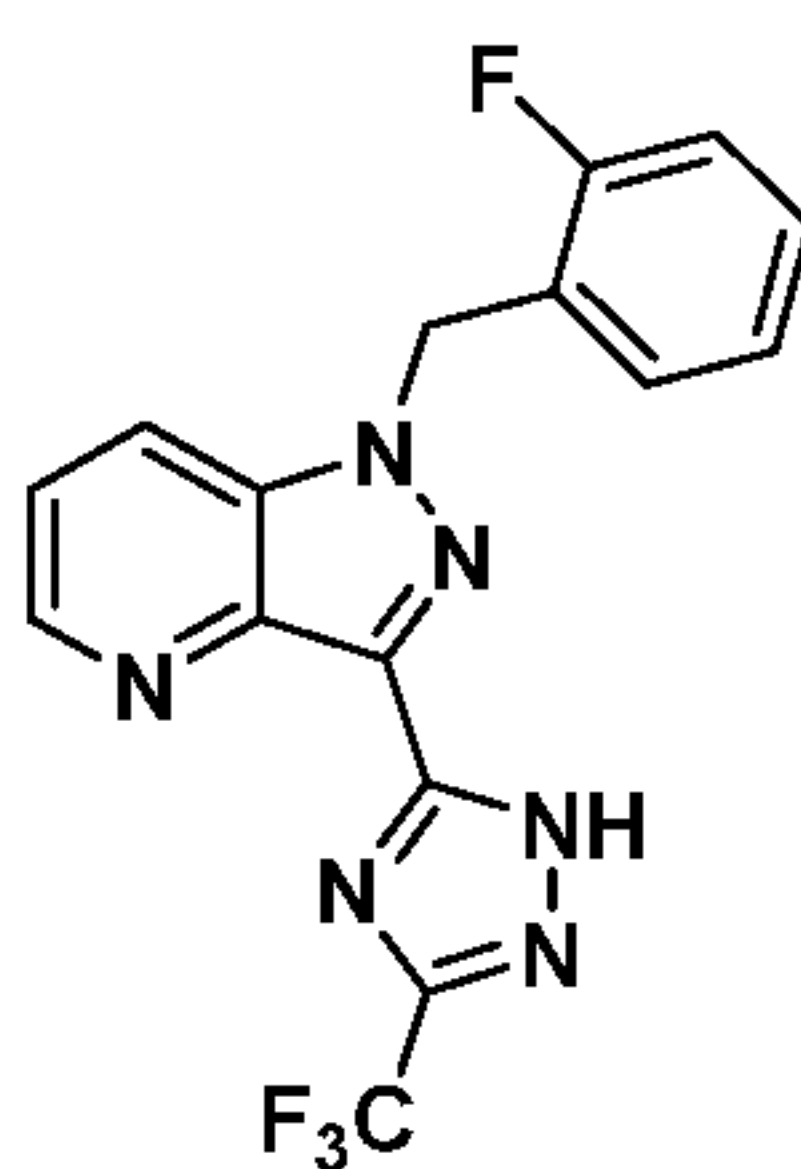
Compound I-35
