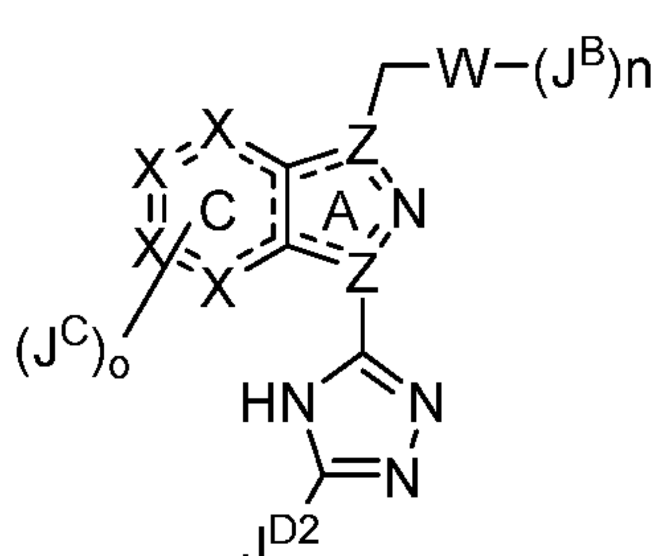
Formula IIB
