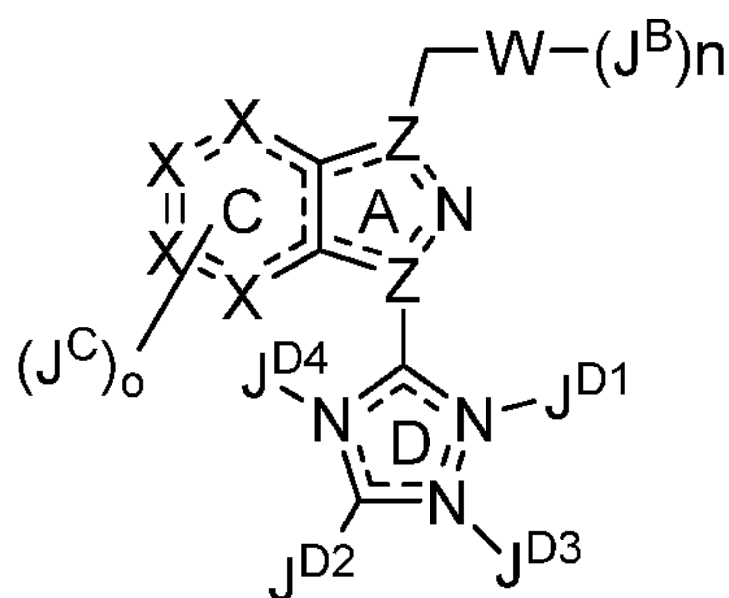
Formula I
