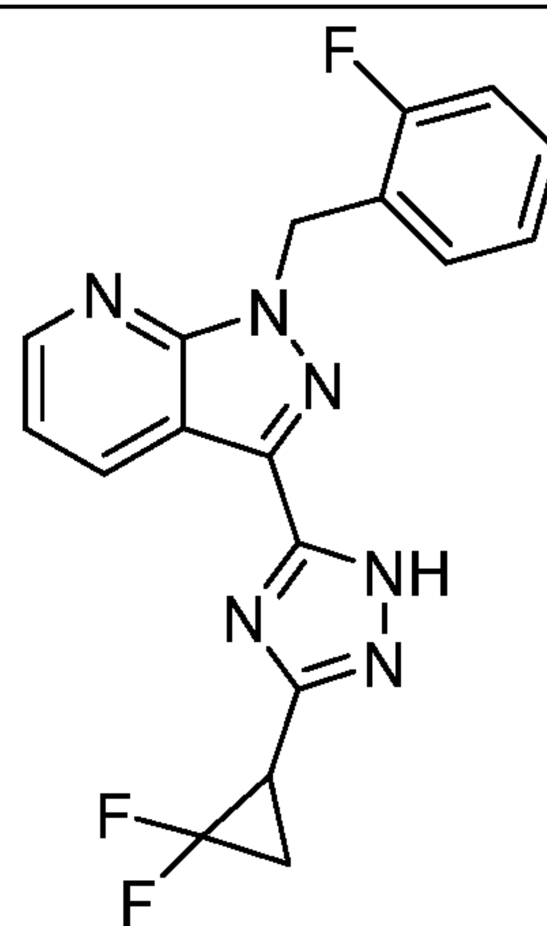
I-96
