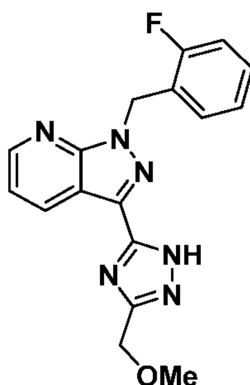
Compound I-112
