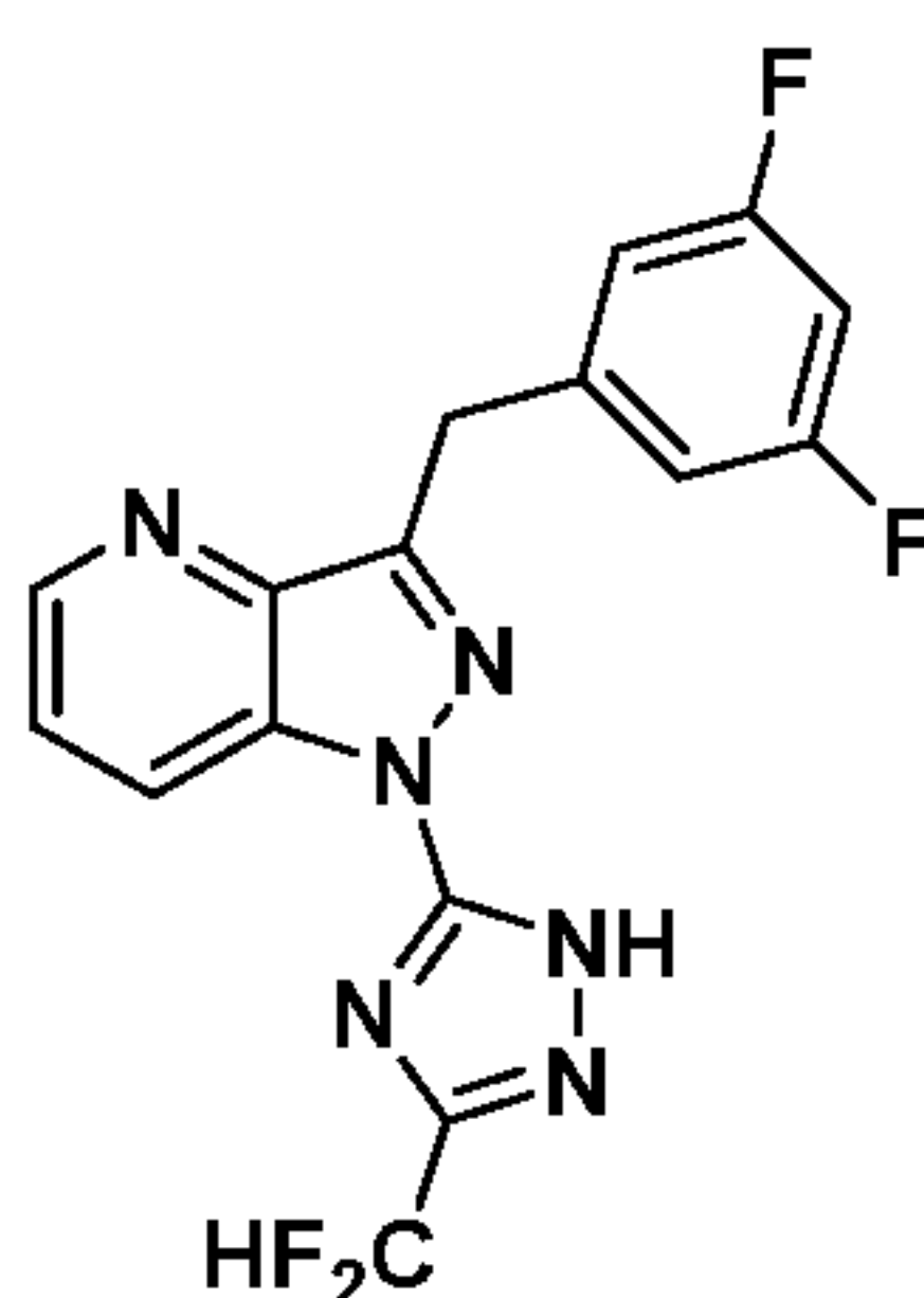
Compound I-123
