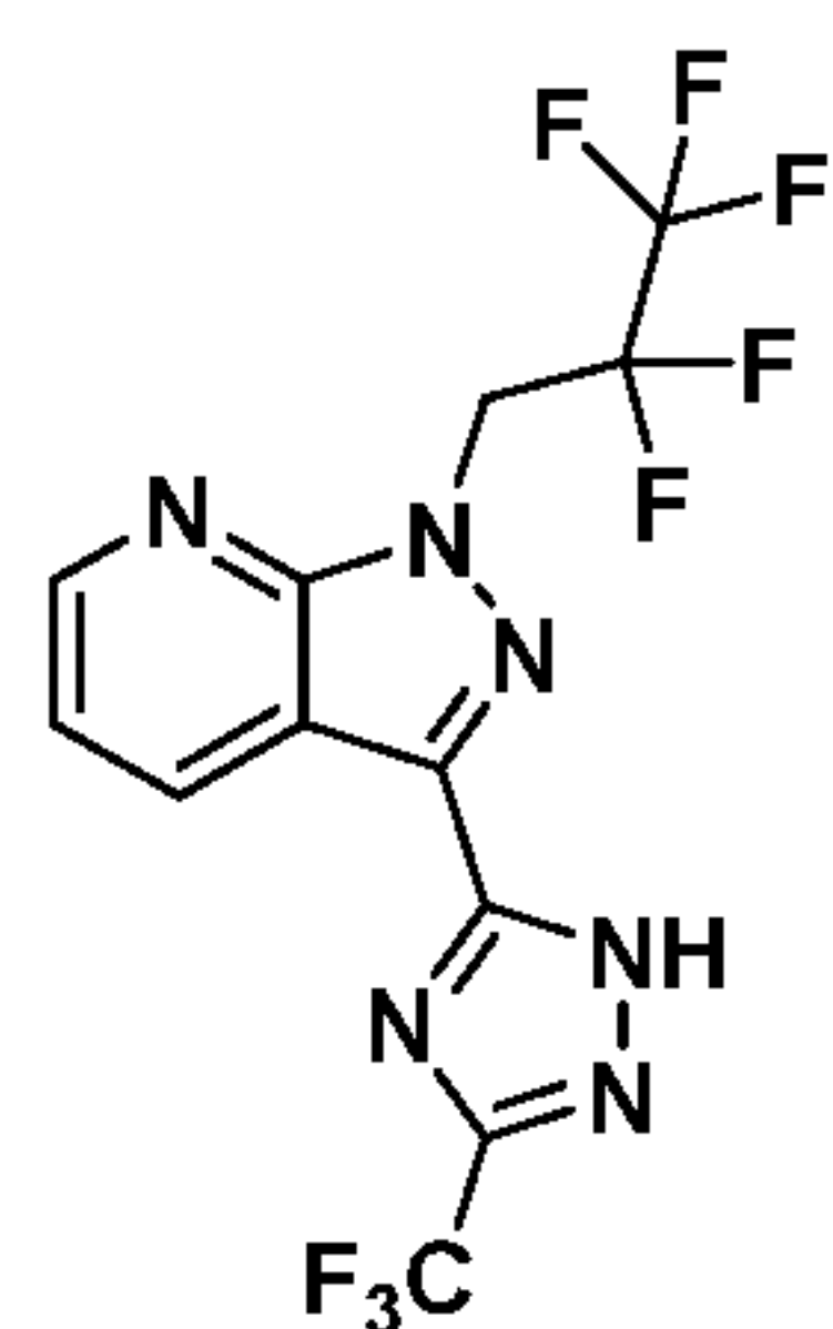
Compound I-19
