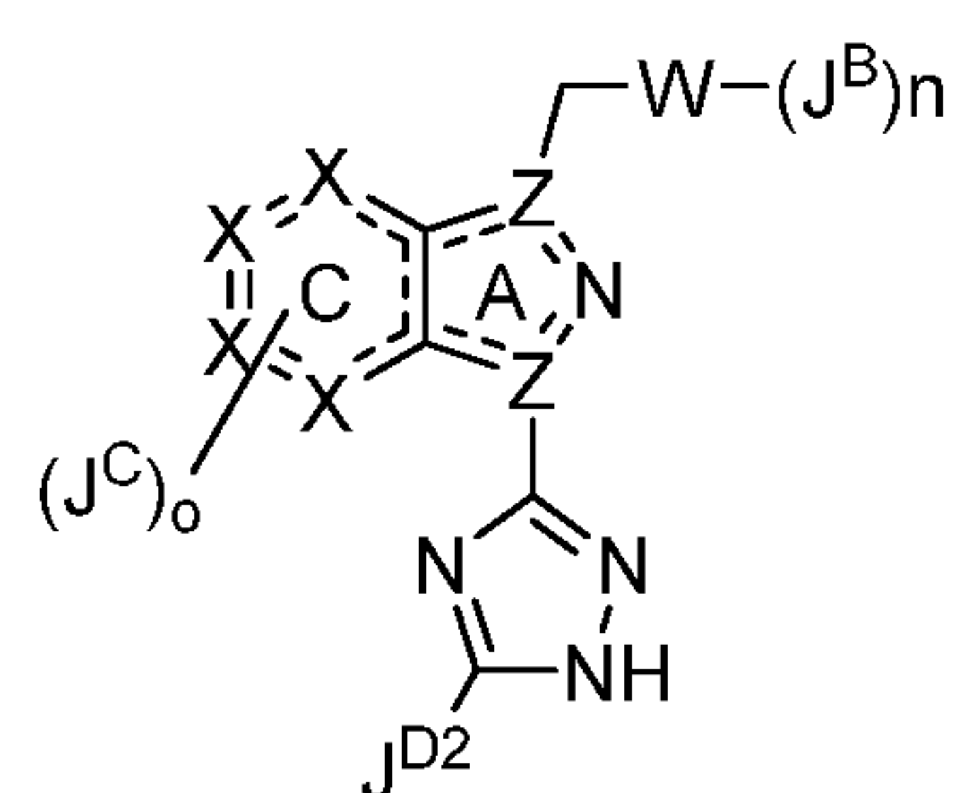
Formula IIC
