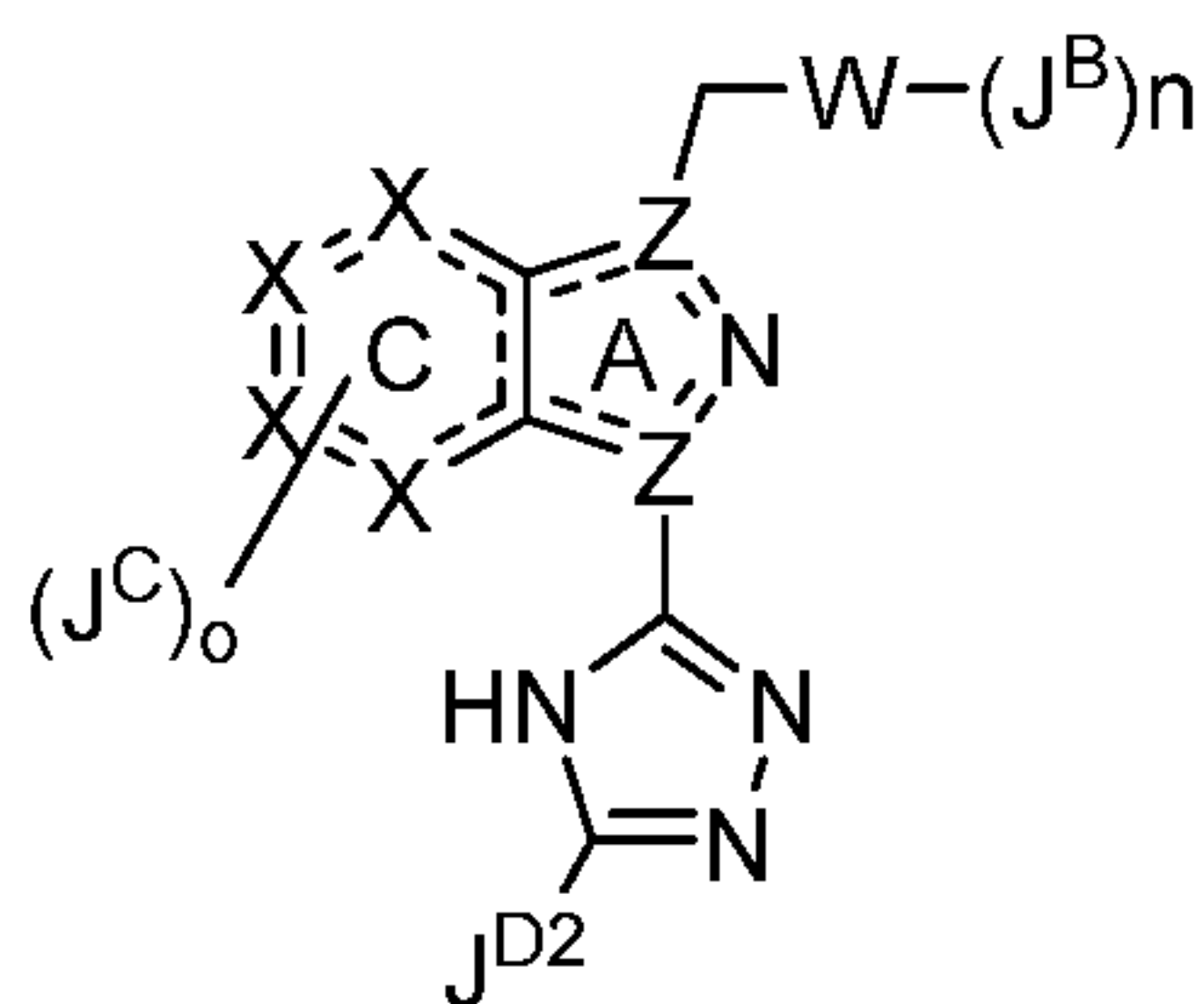
Formula IIB
