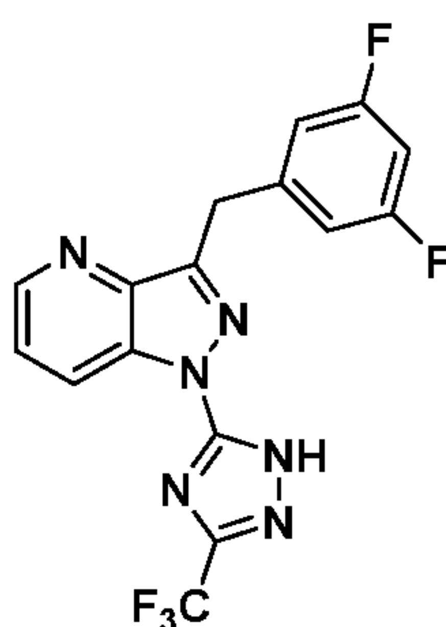
Compound I-121
