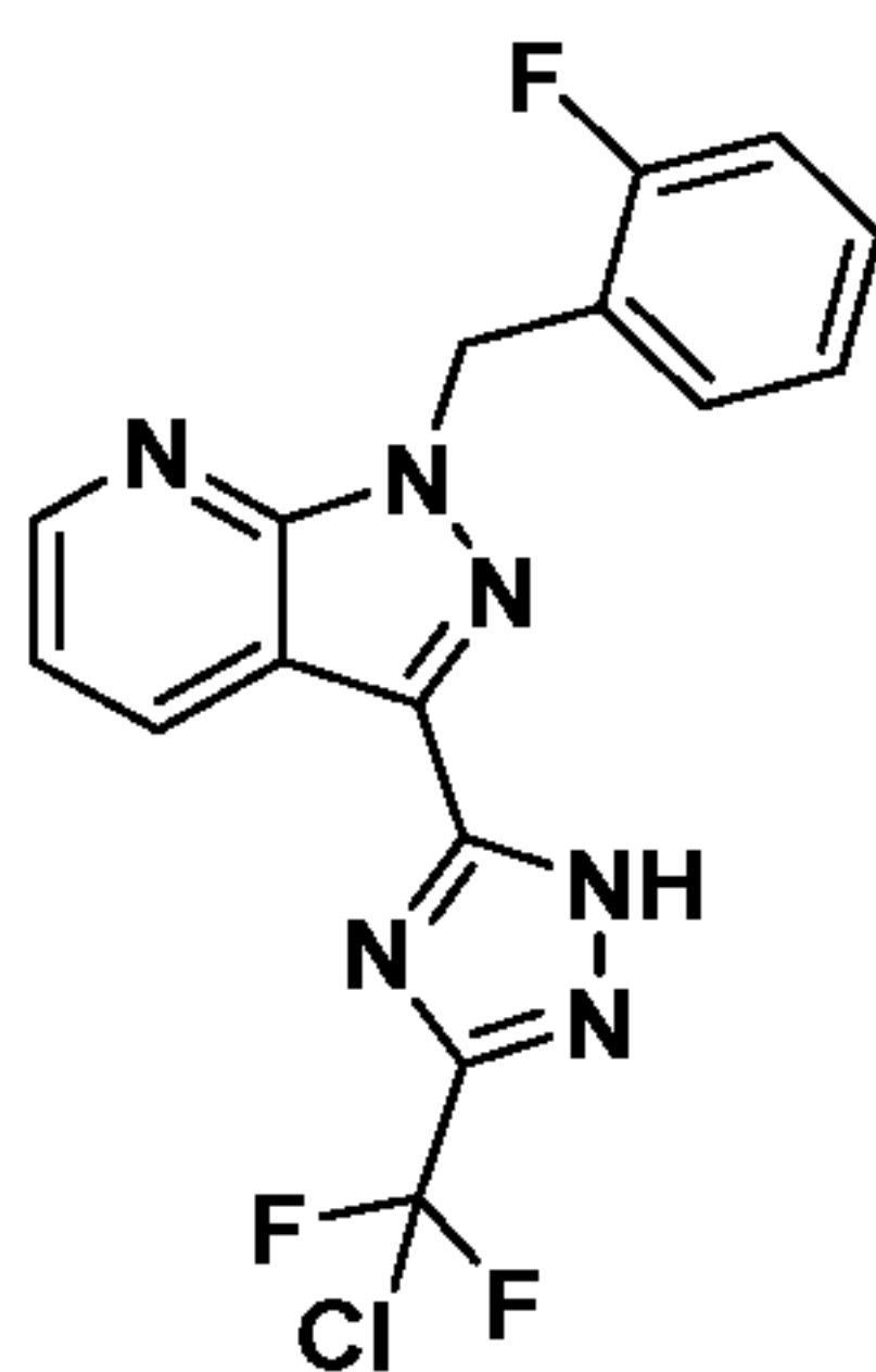
Compound I-65
