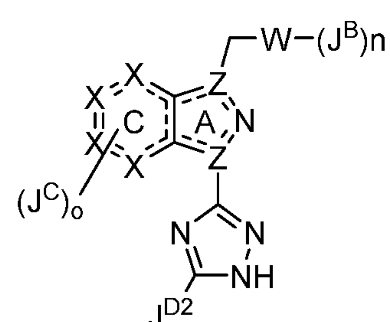
Formula IIC
