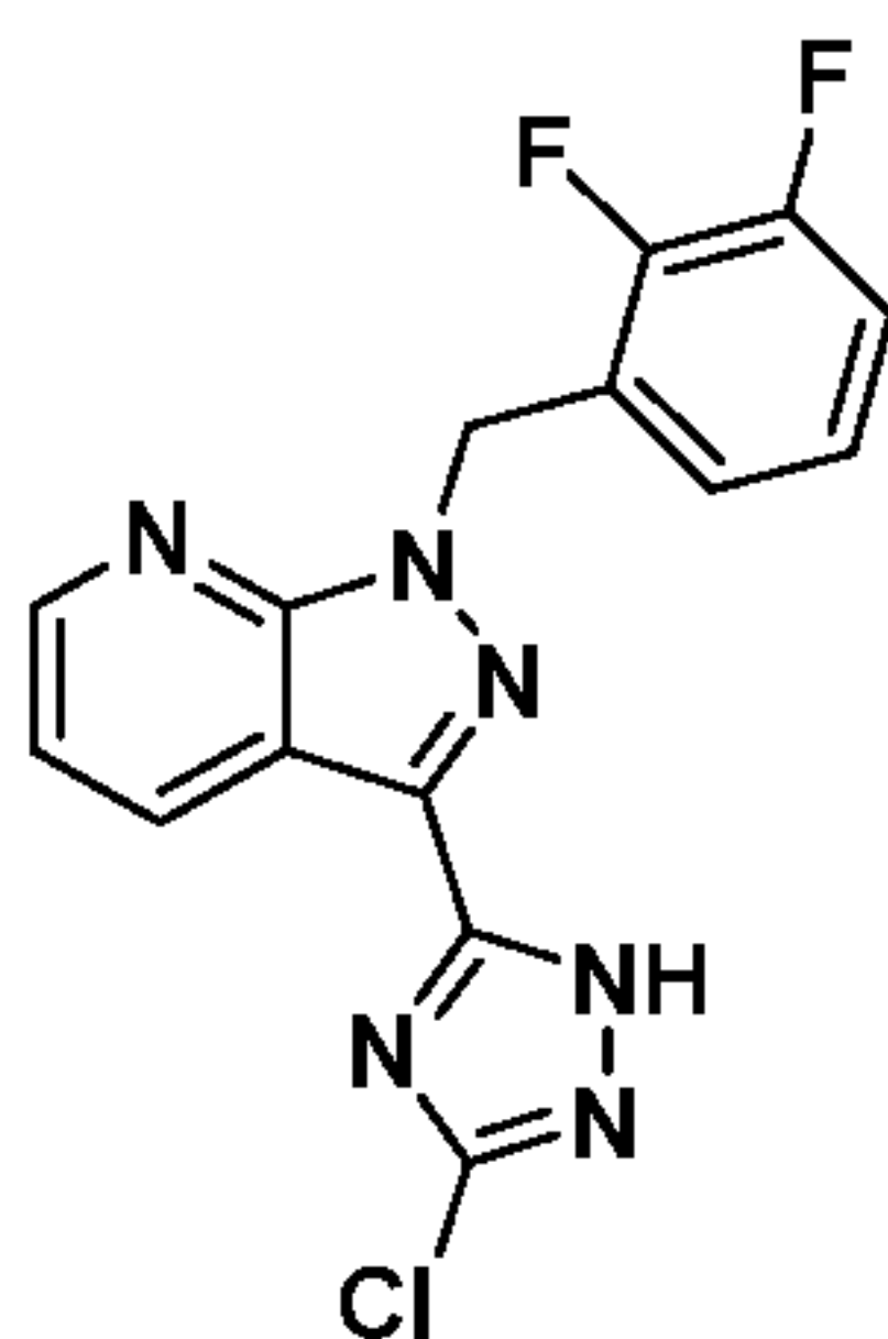
Compound I-86
