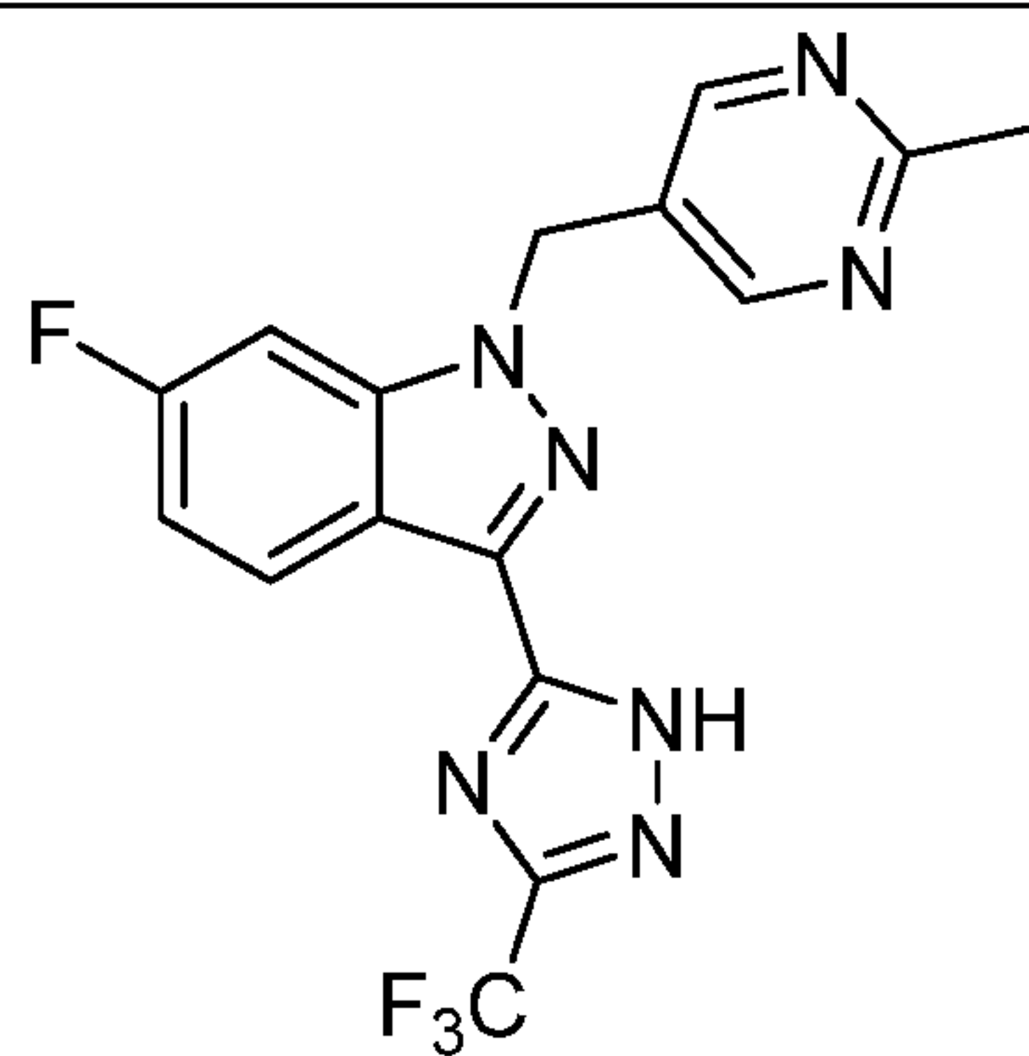
I-61
