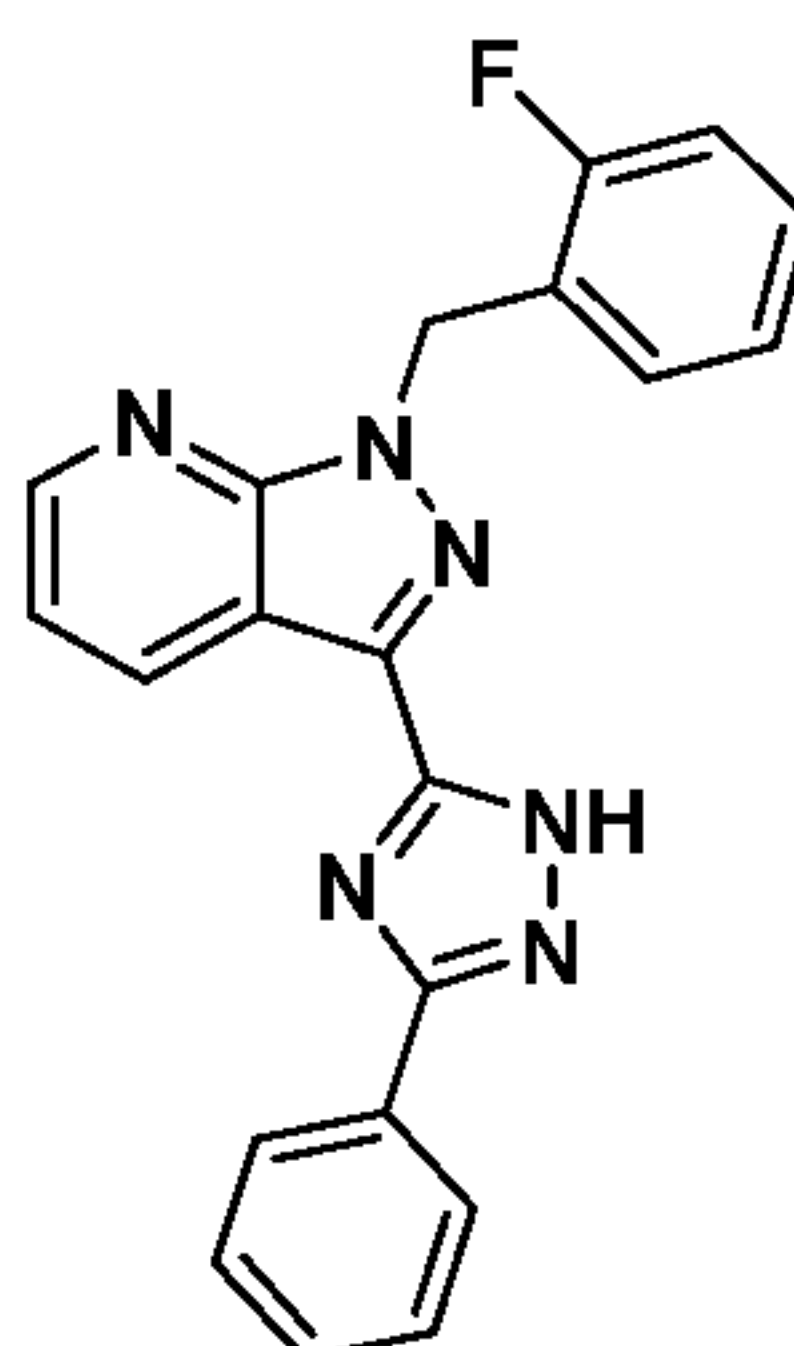
Compound I-39
