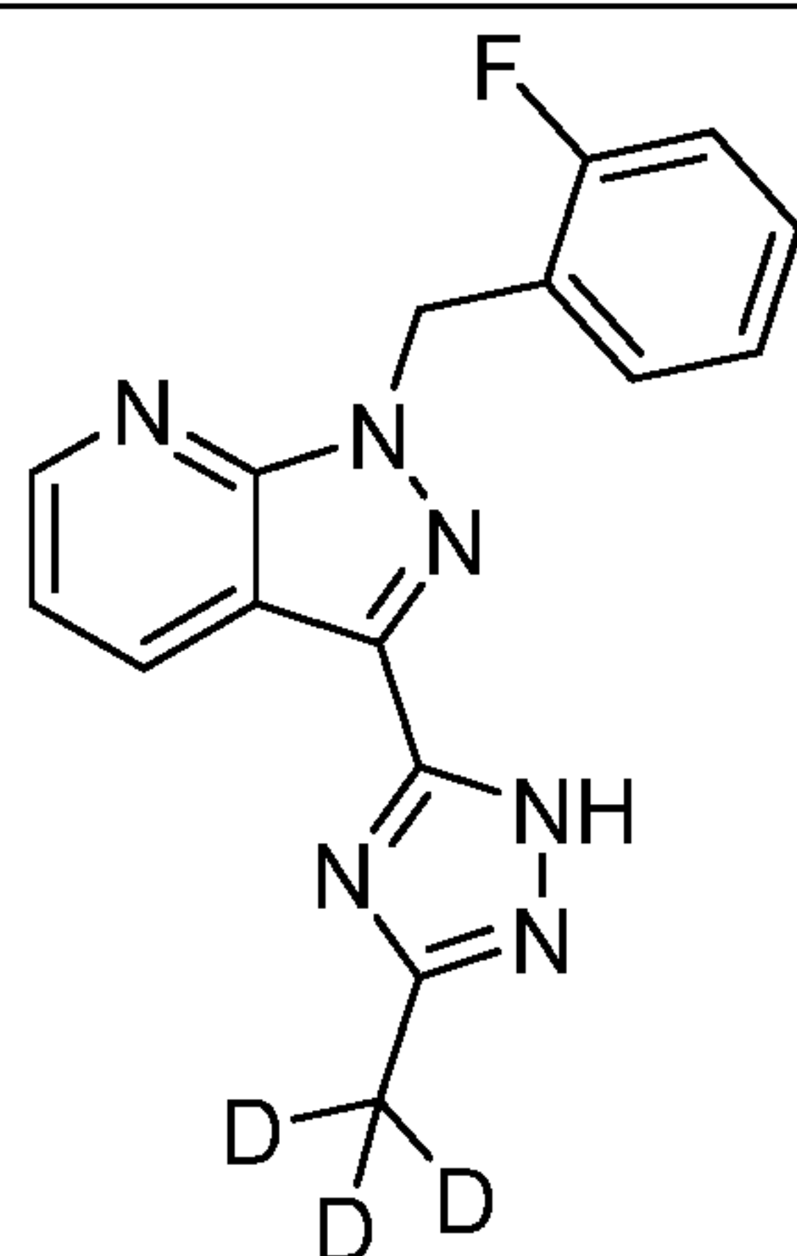
I-91
