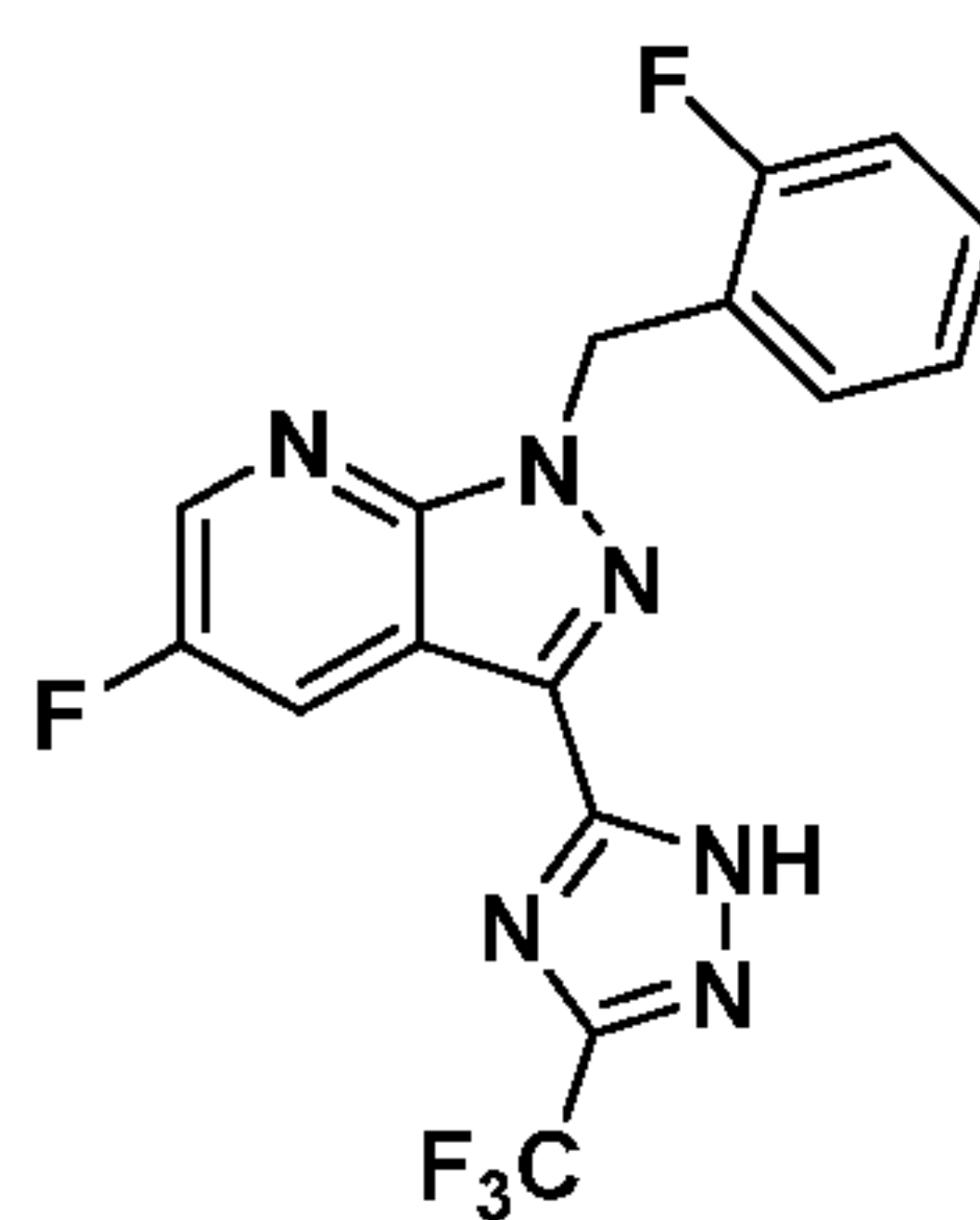
Compound I-8
