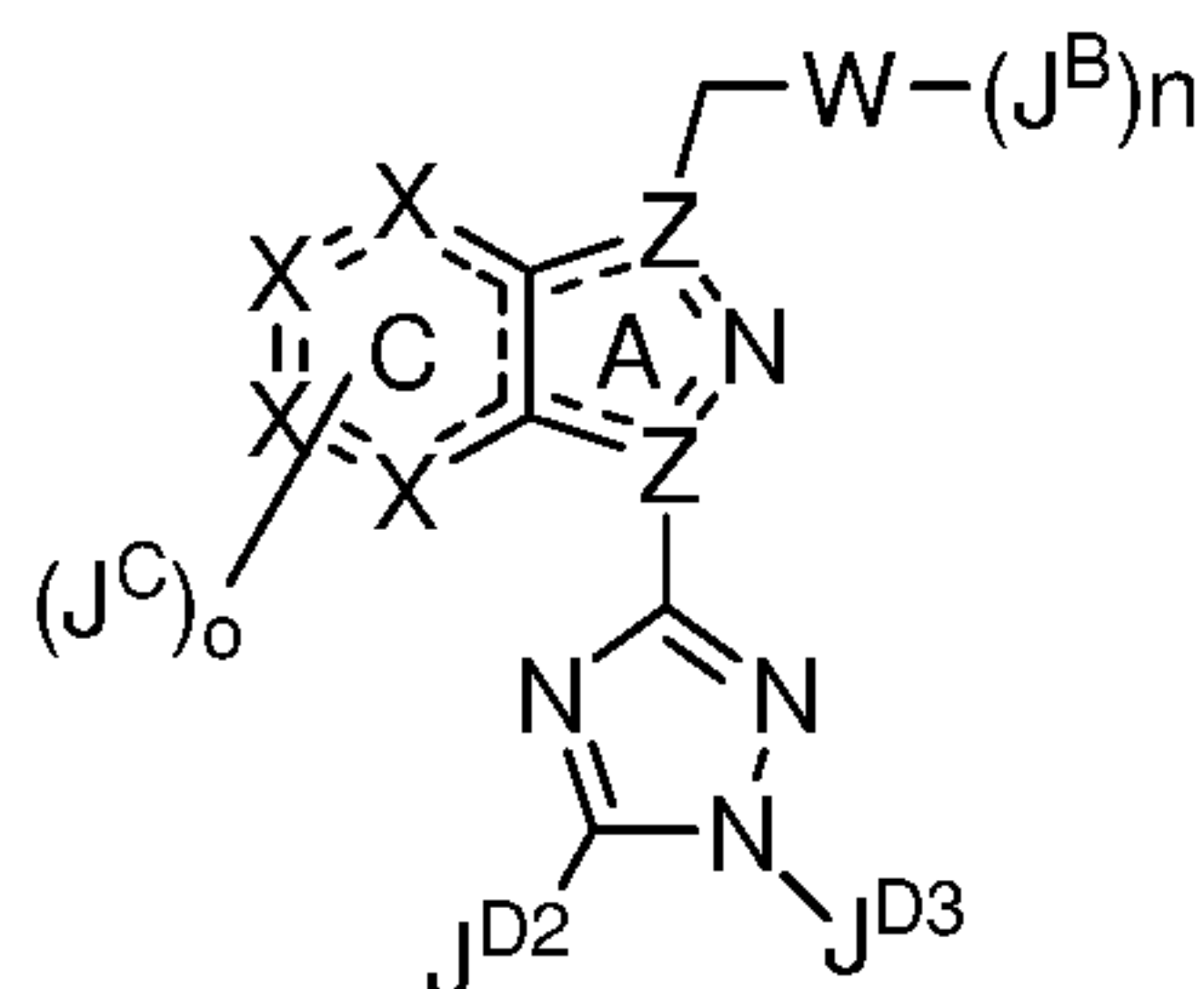
Formula III;
