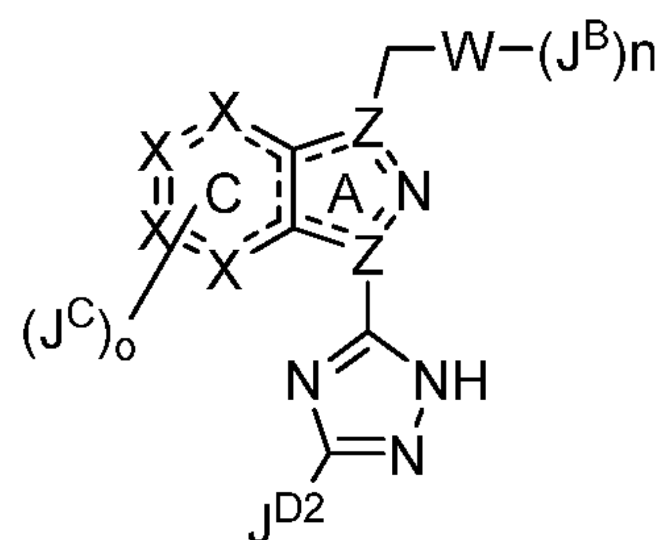
Formula IIA
