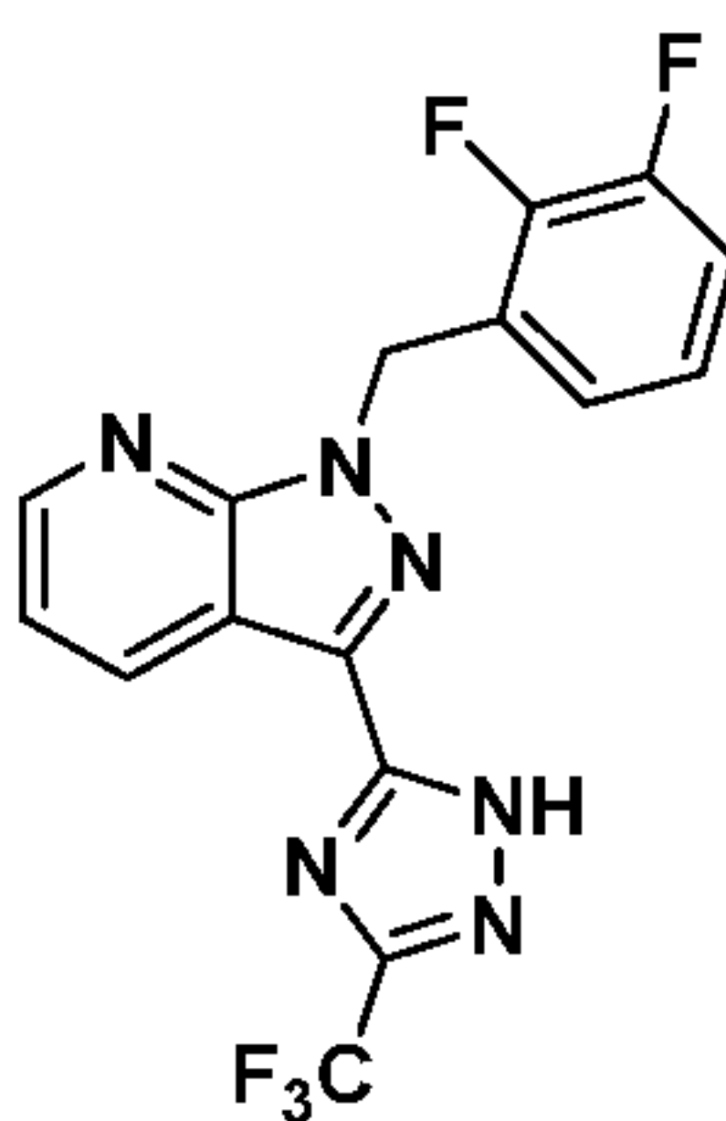
Compound I-48
