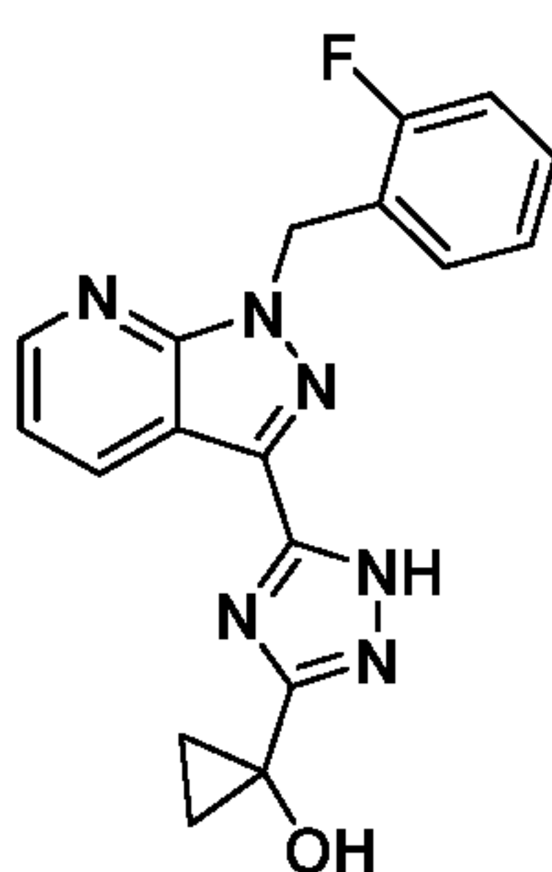
Compound I-104
