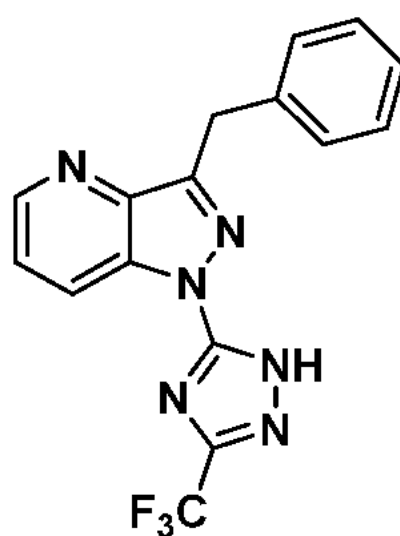
Compound I-128
