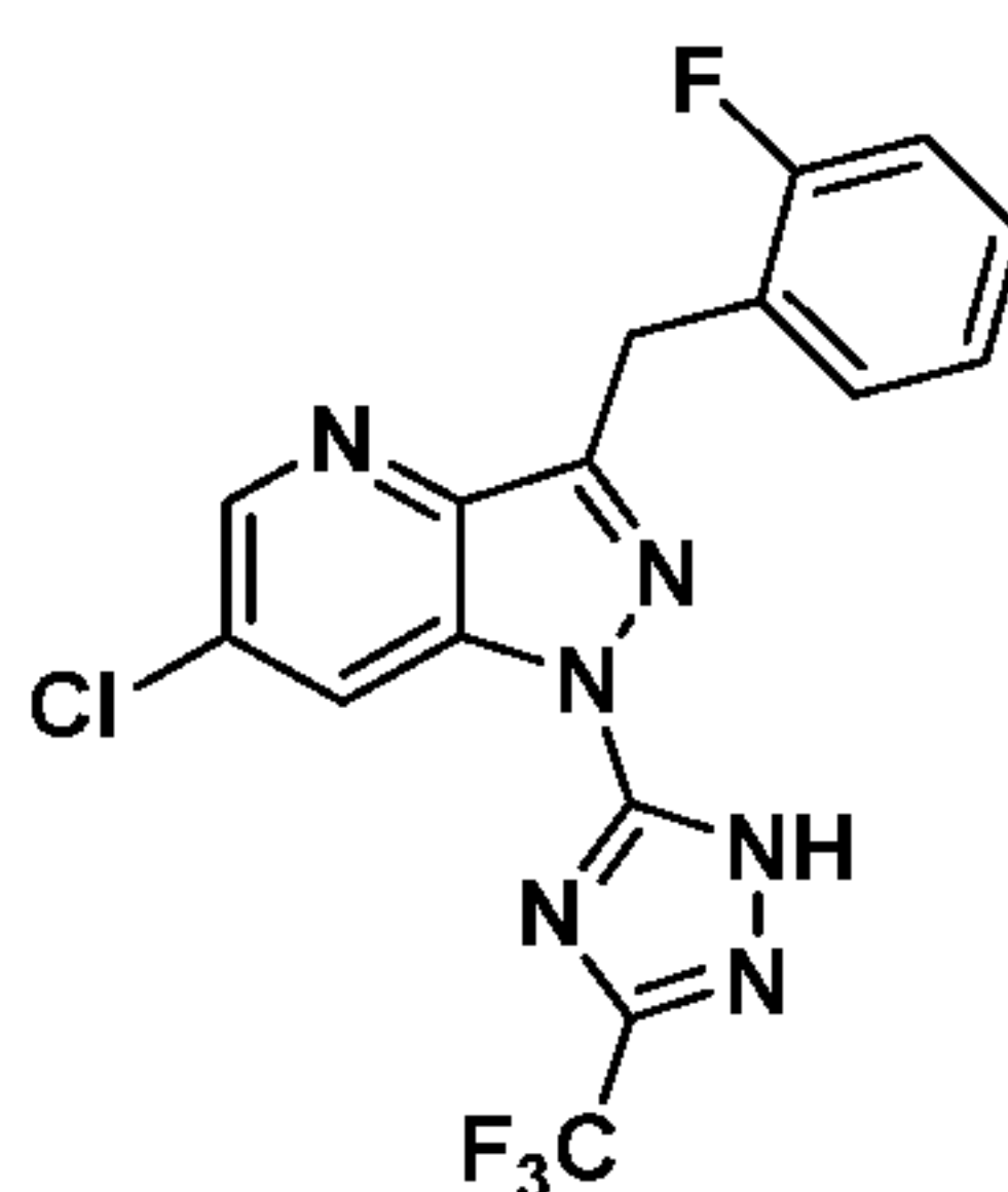
Compound I-30
