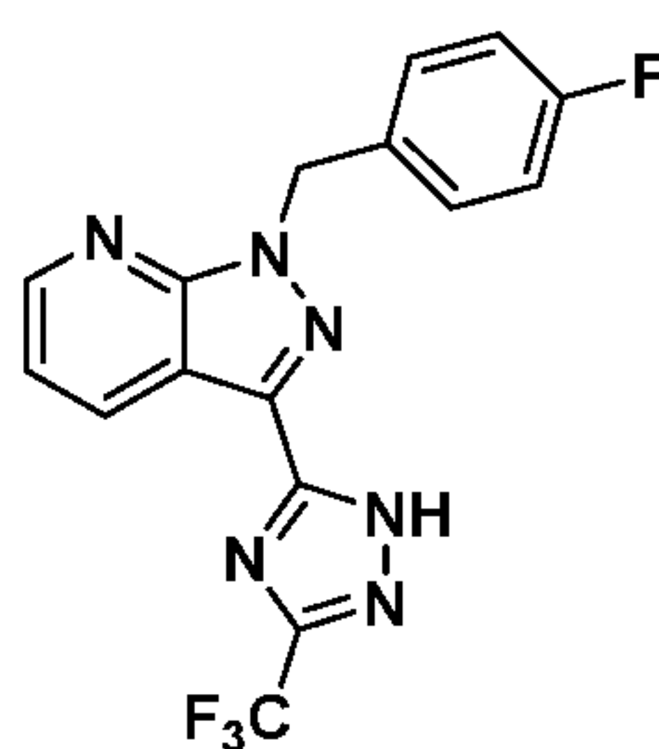
Compound I-53
