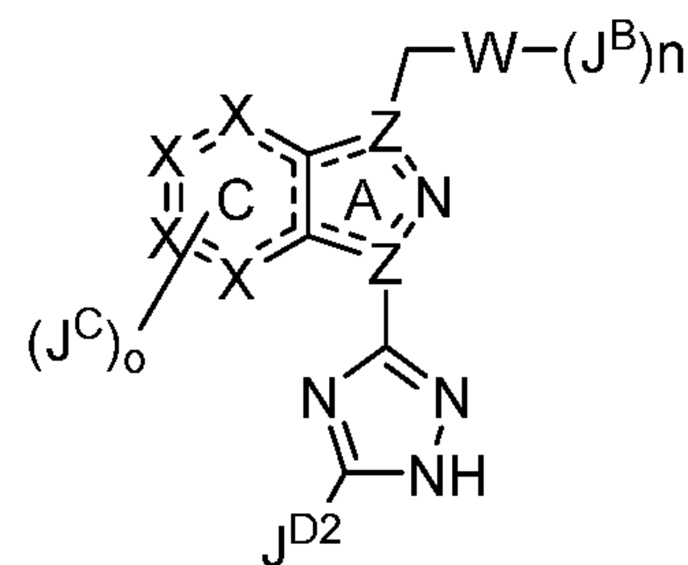
Formula IIC
