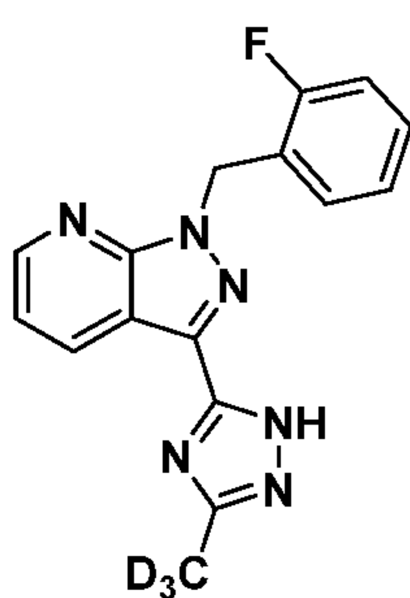
Compound I-91
