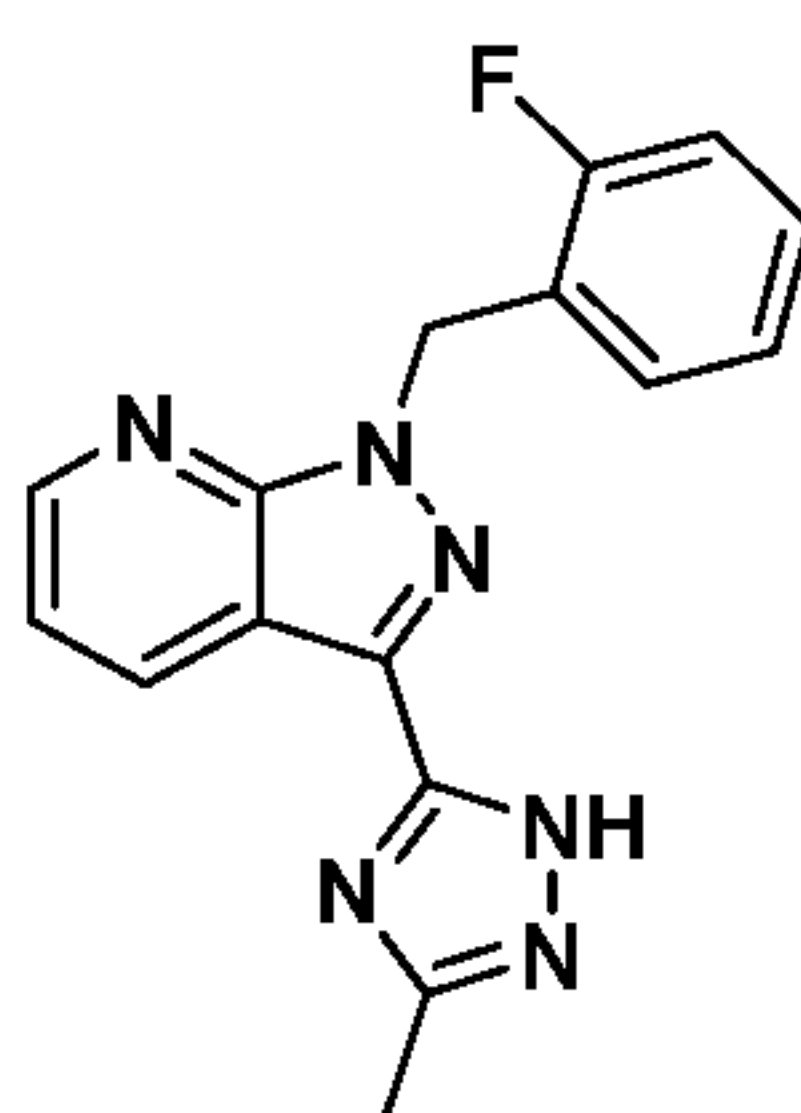
Compound I-60
