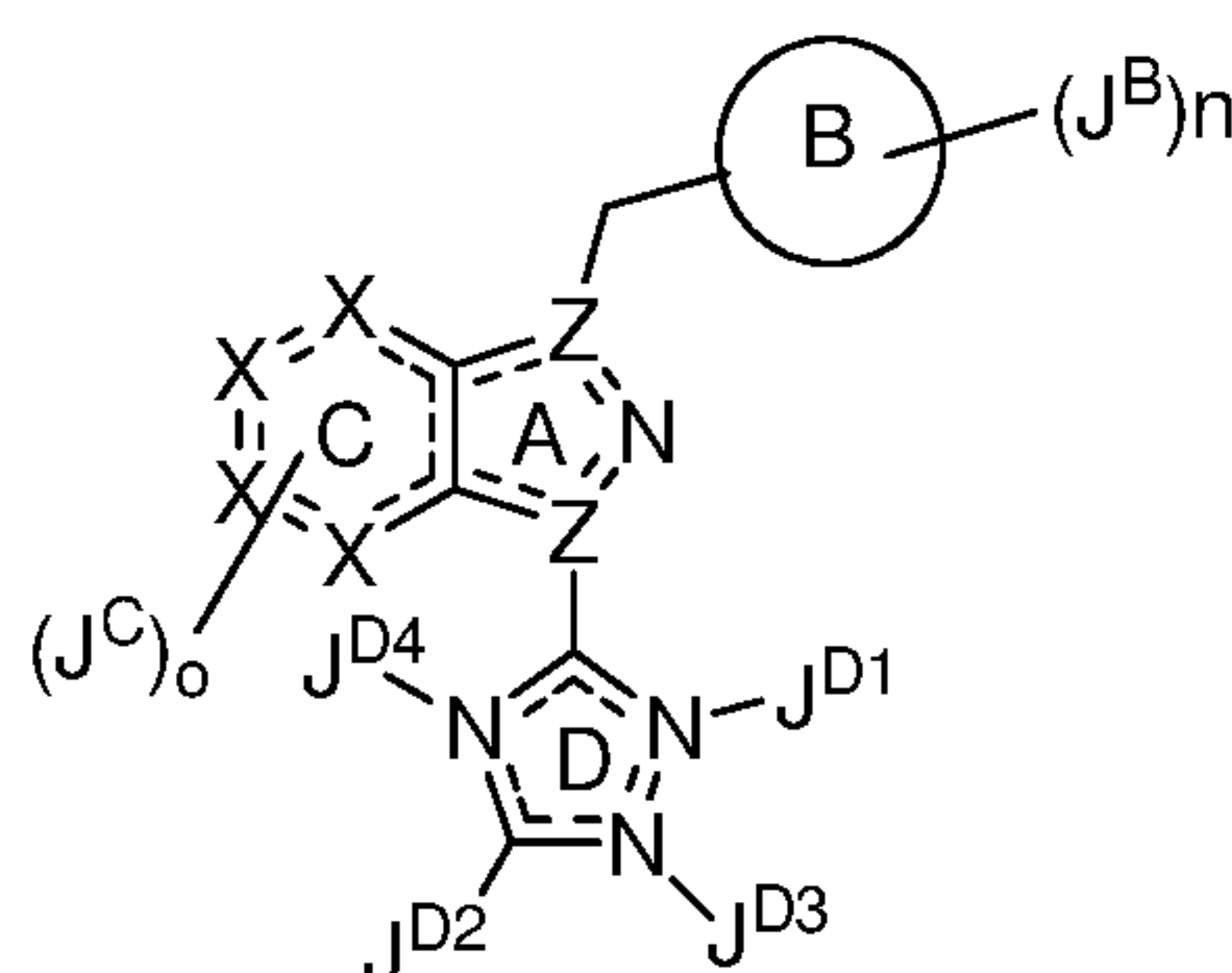
Formula IV.
