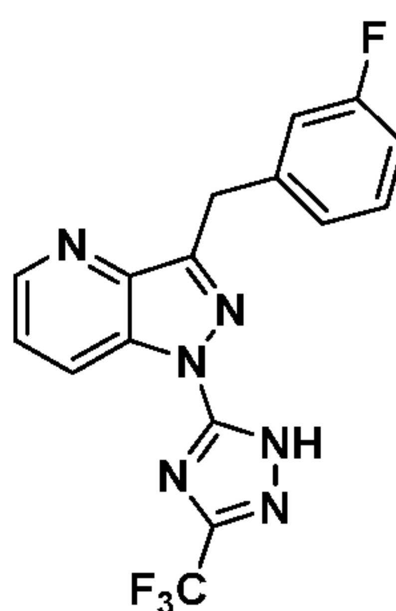
Compound I-120
