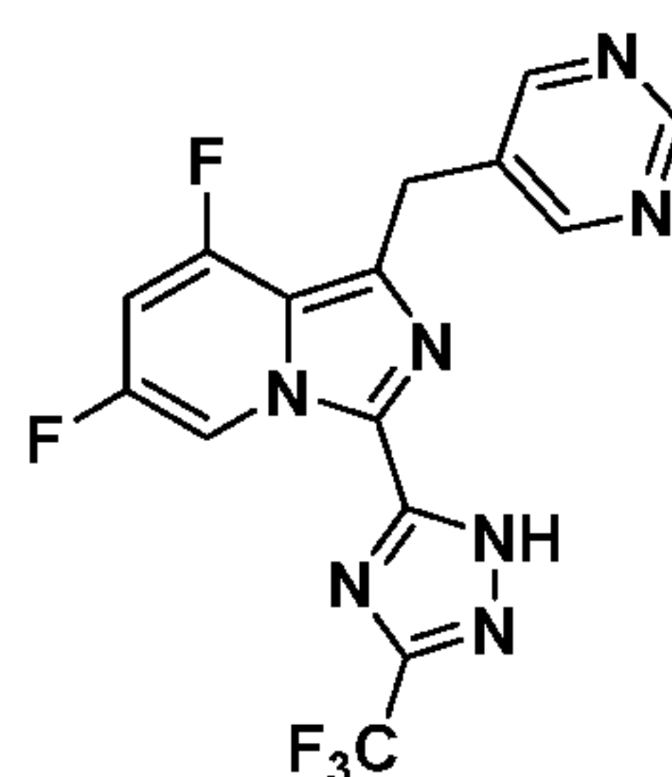
Compound I-28
