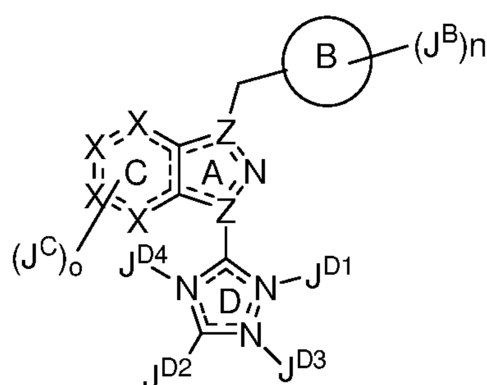
Formula IV.
