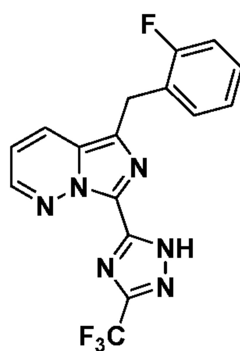
Compound I-24
