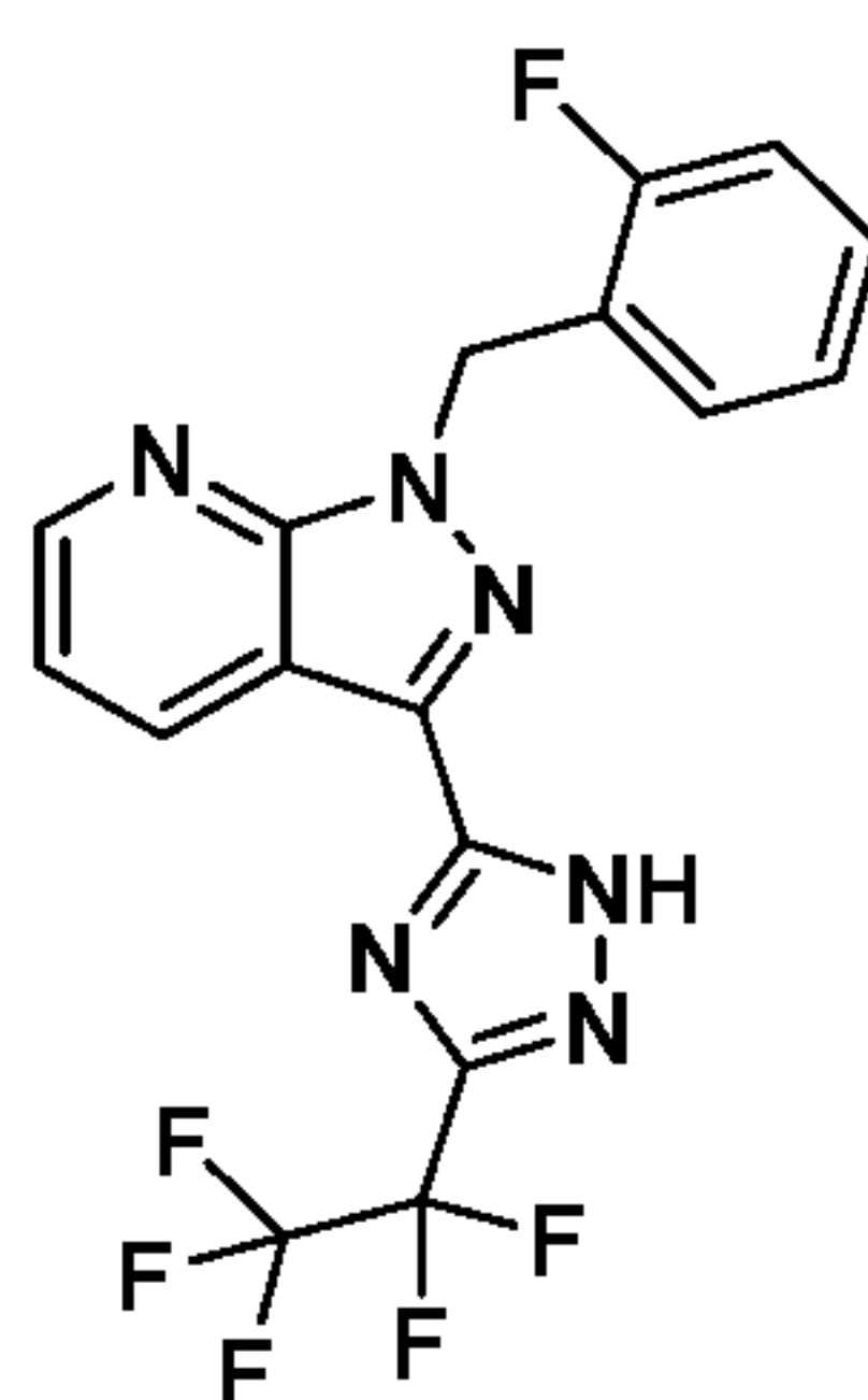
Compound I-21
