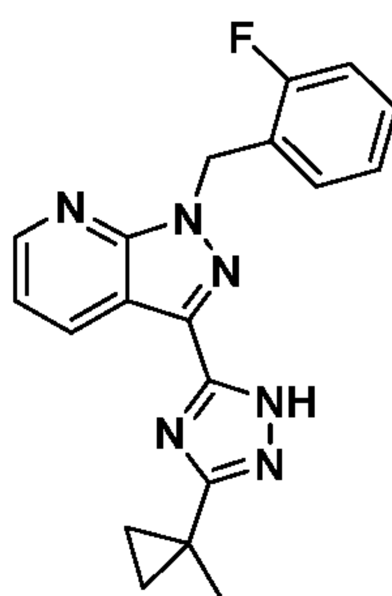
Compound I-63
