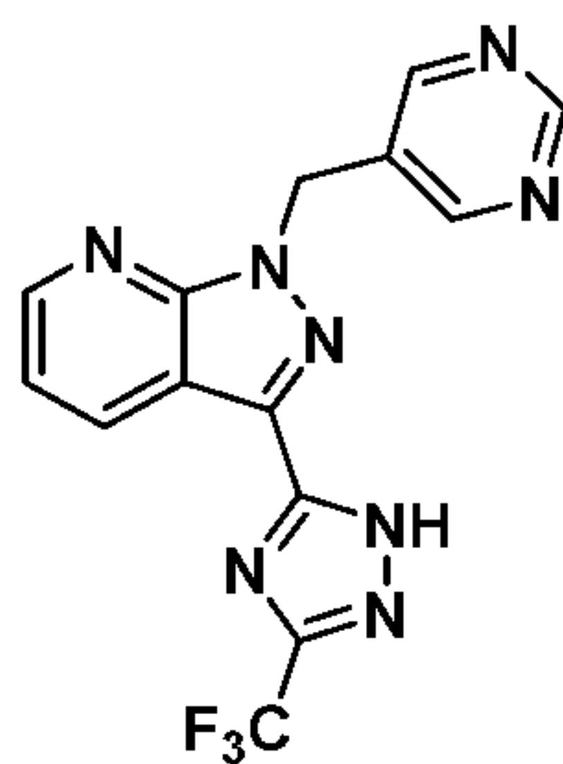
Compound I-4
