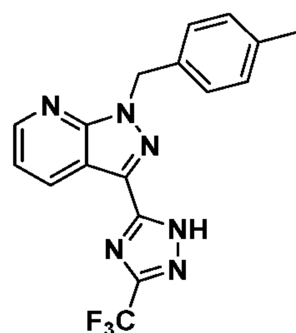
Compound I-54
