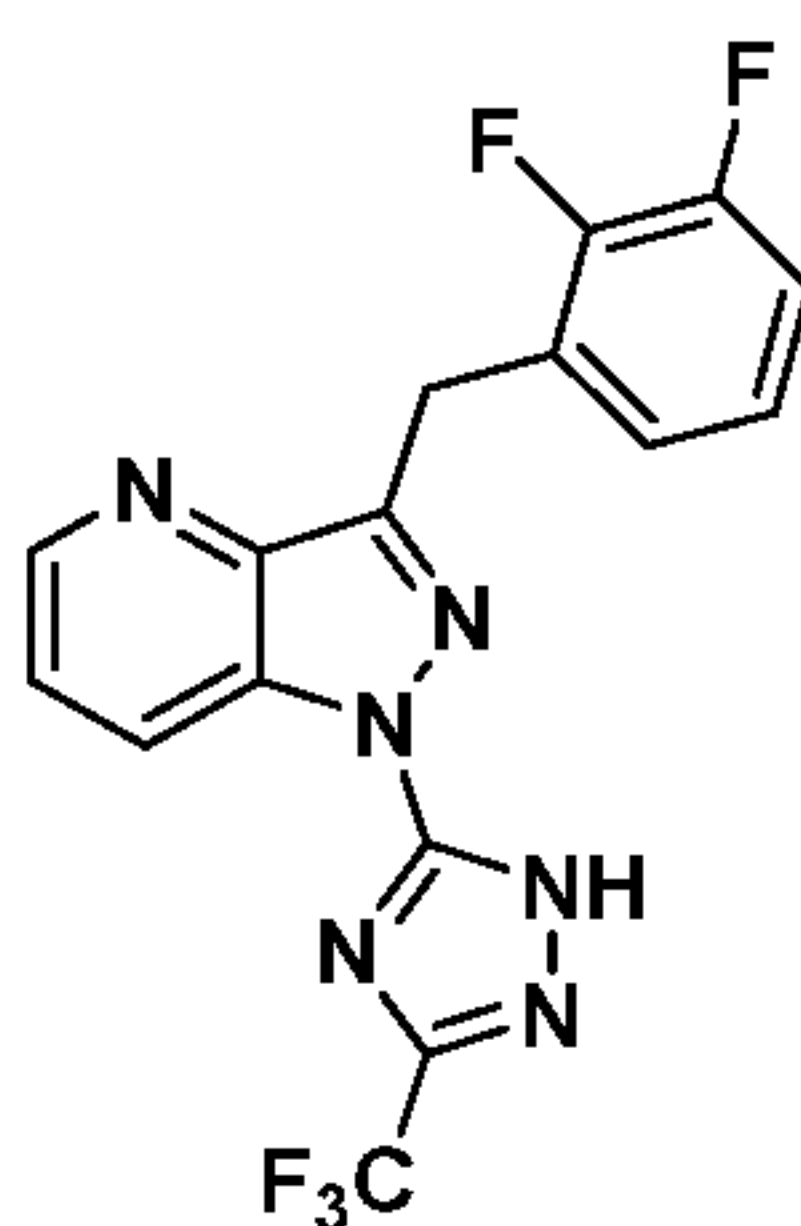
Compound I-105
