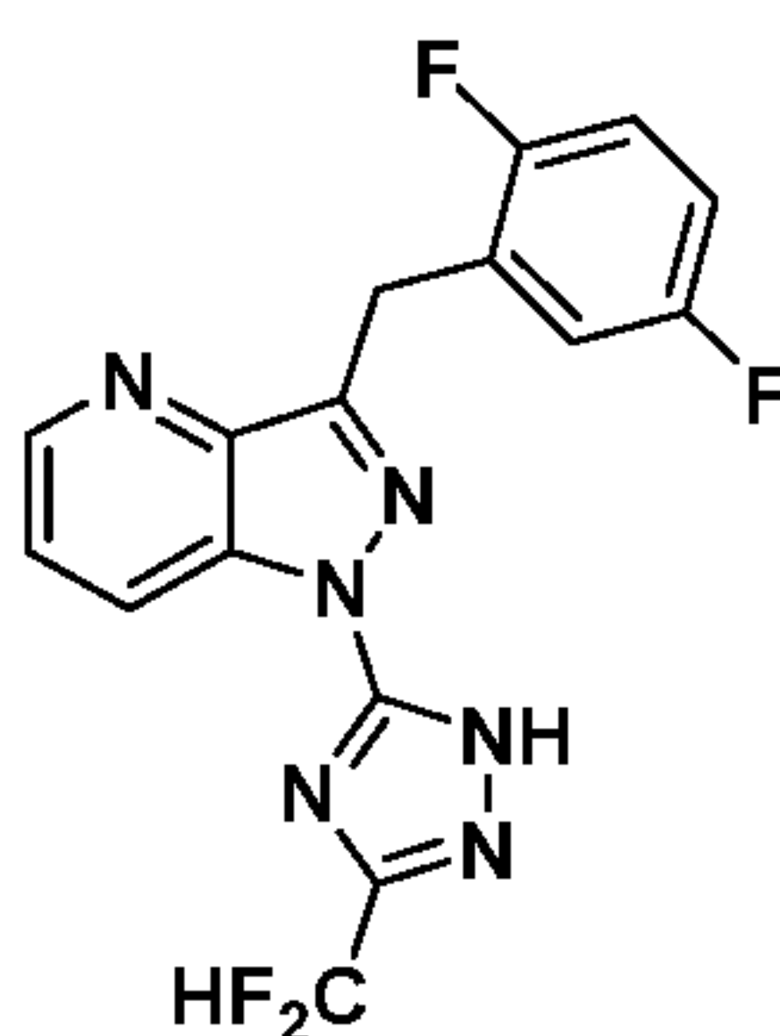
Compound I-131
