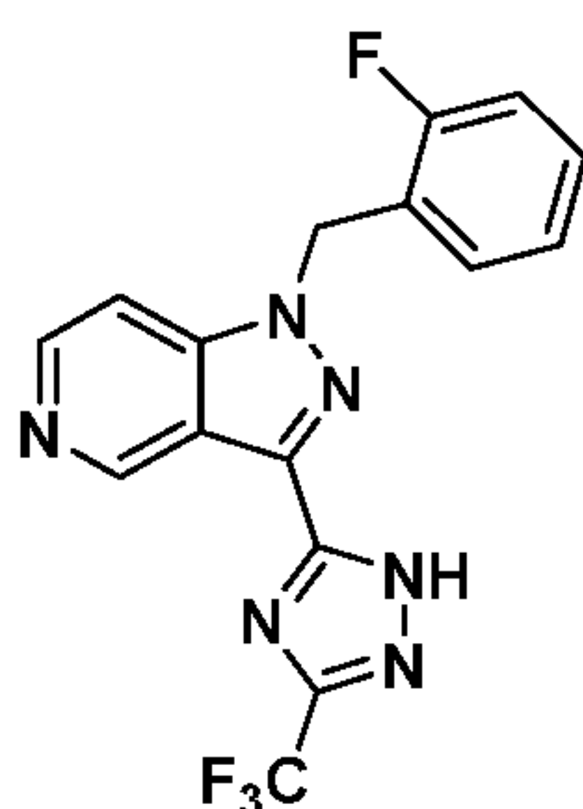
Compound I-43
