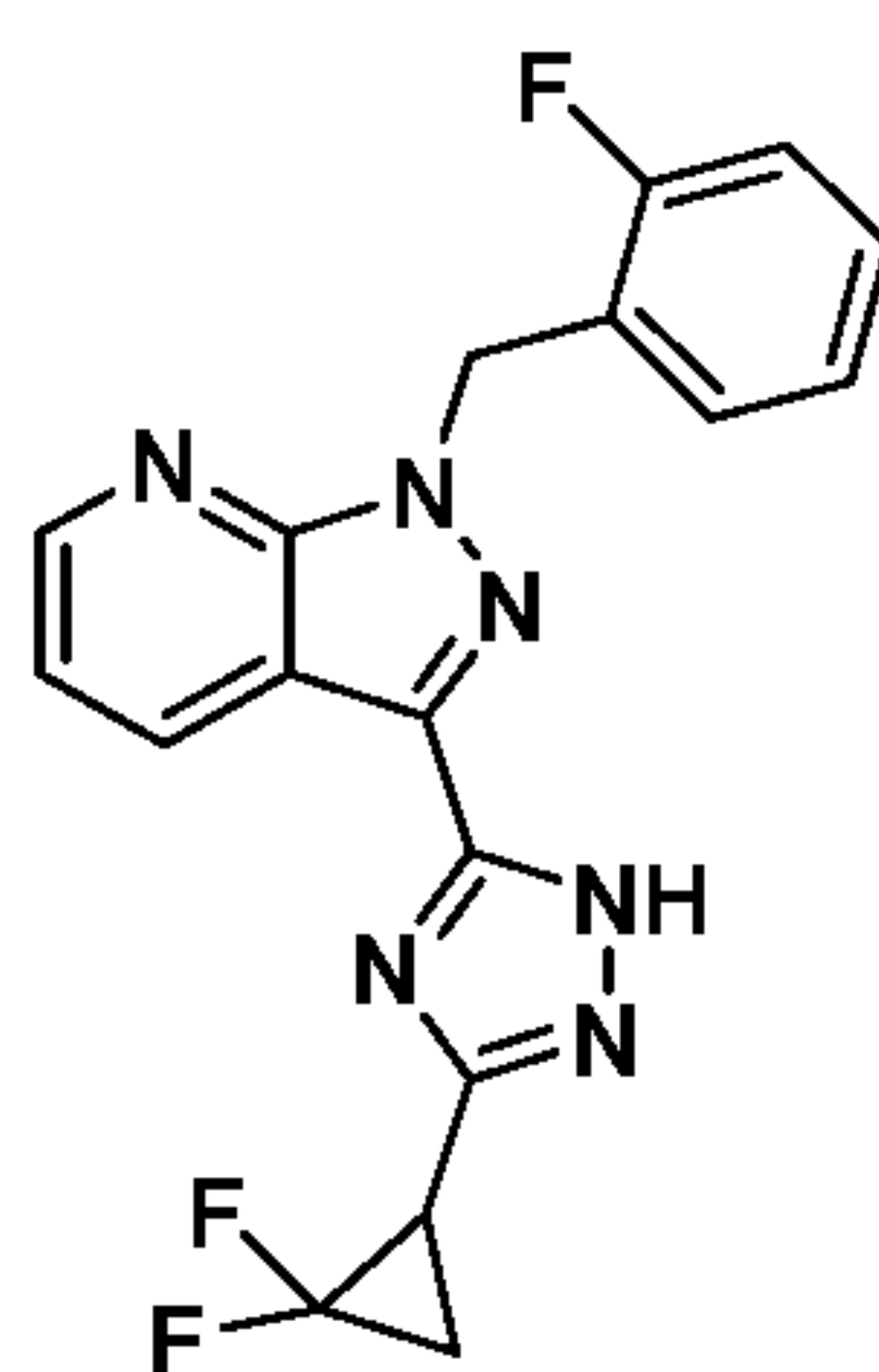
Compound I-96
