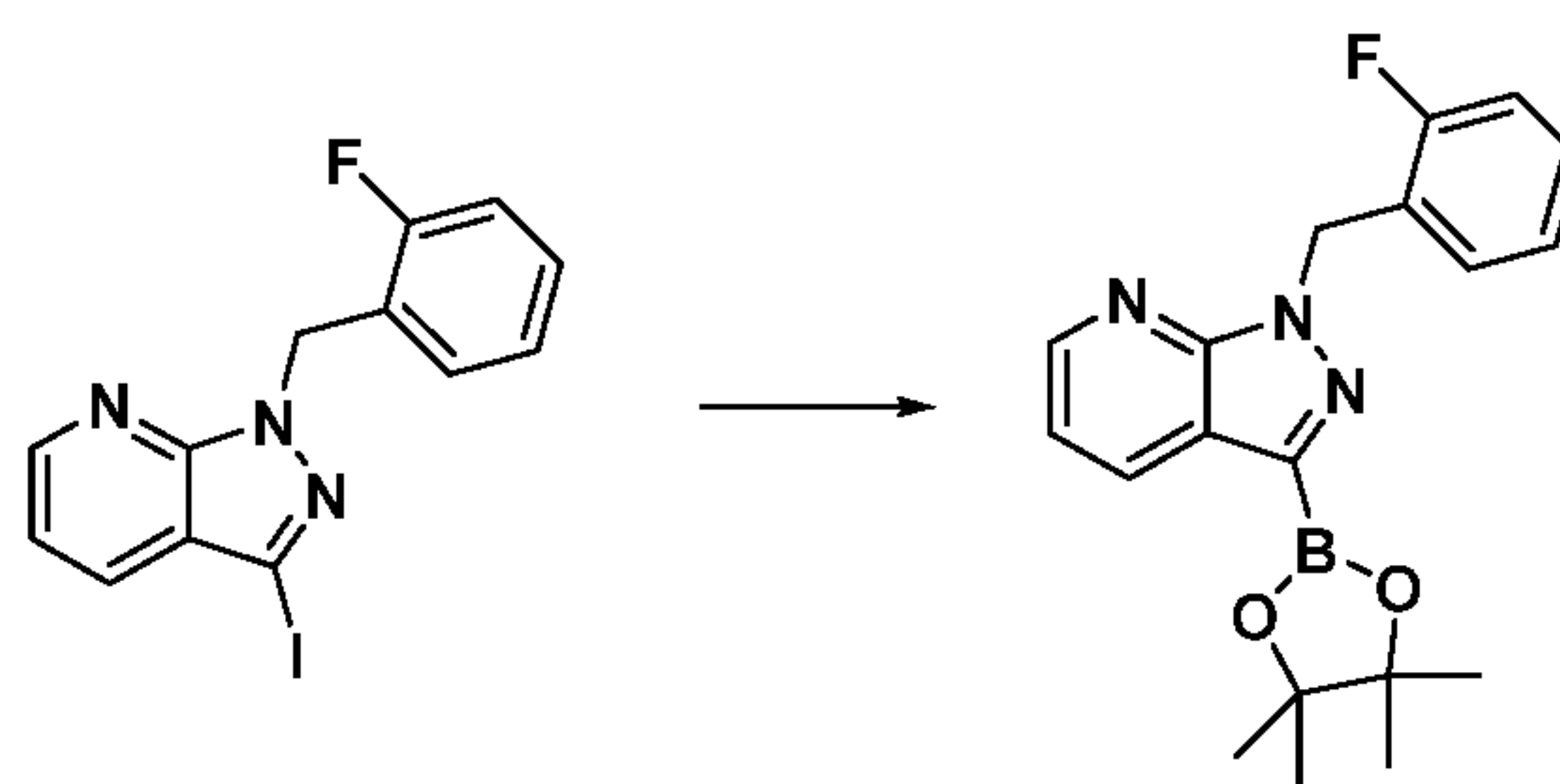
Intermediate 10
