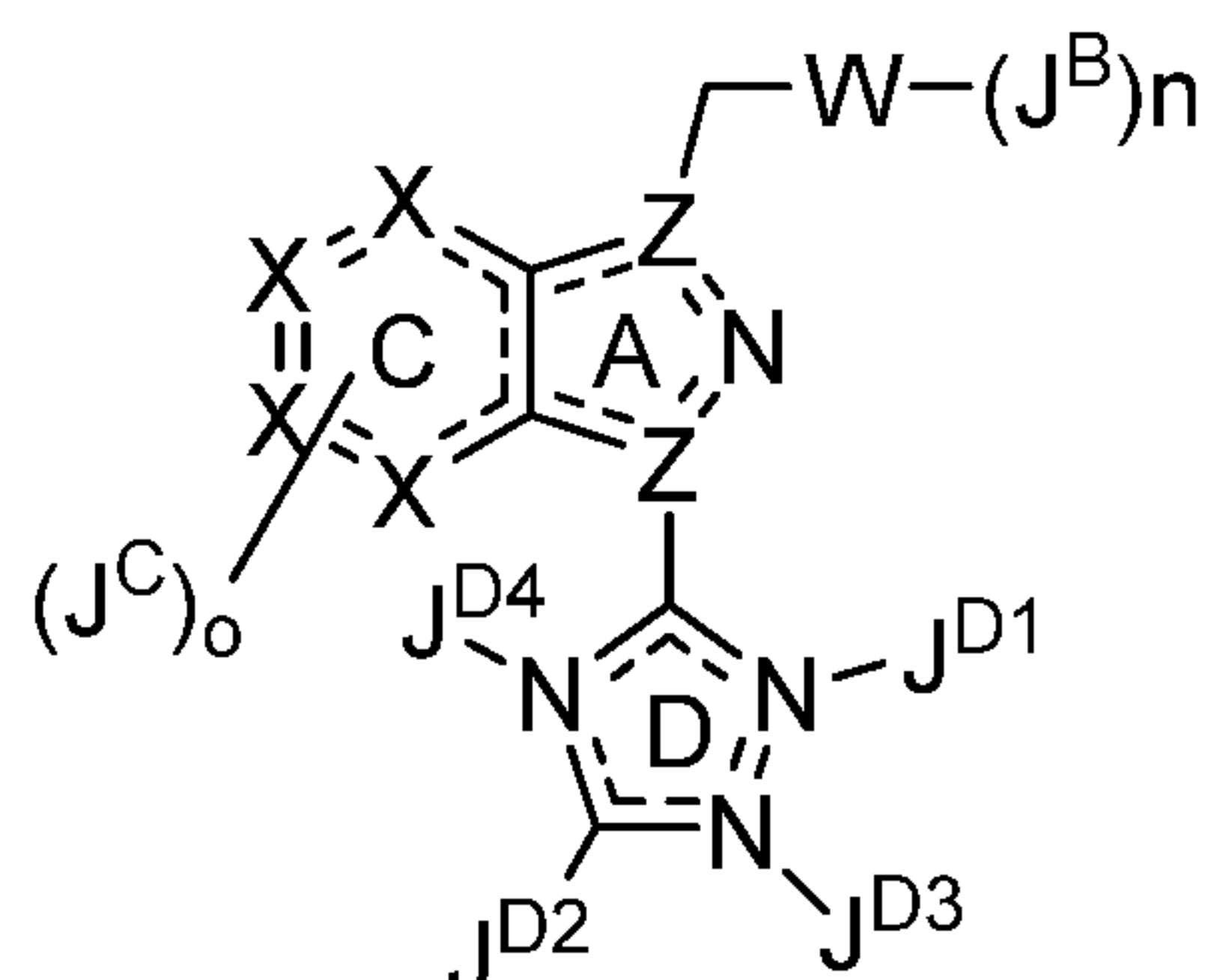
Formula I
