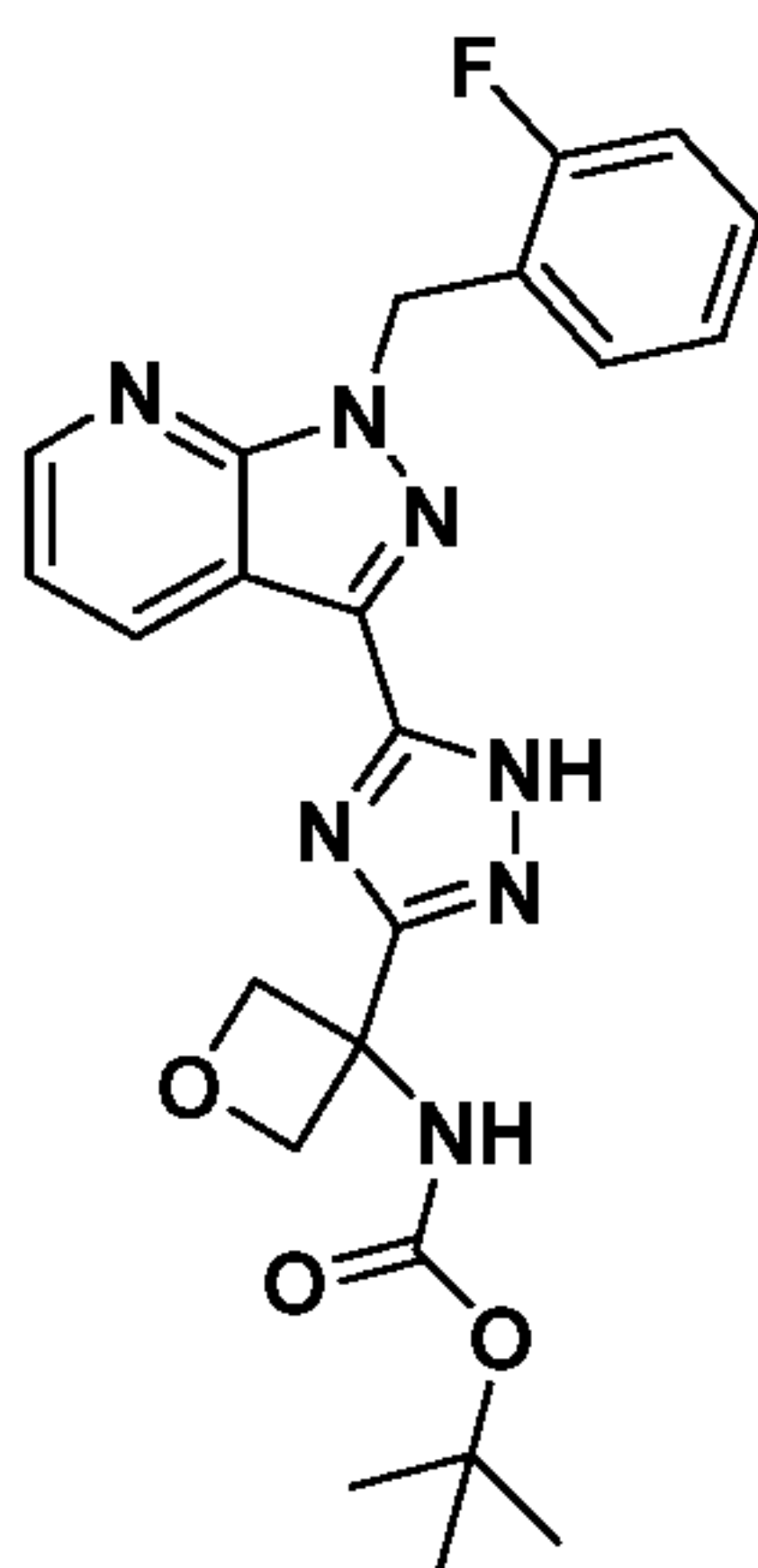
Compound I-76
