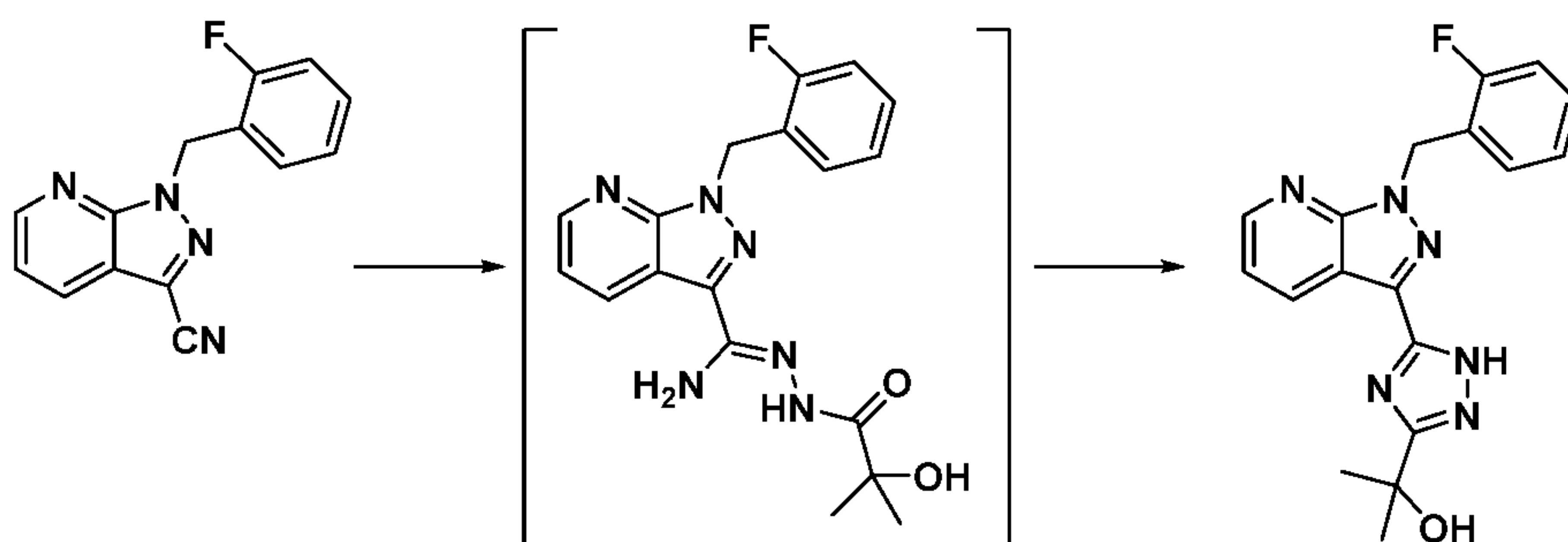
Compound I-94
