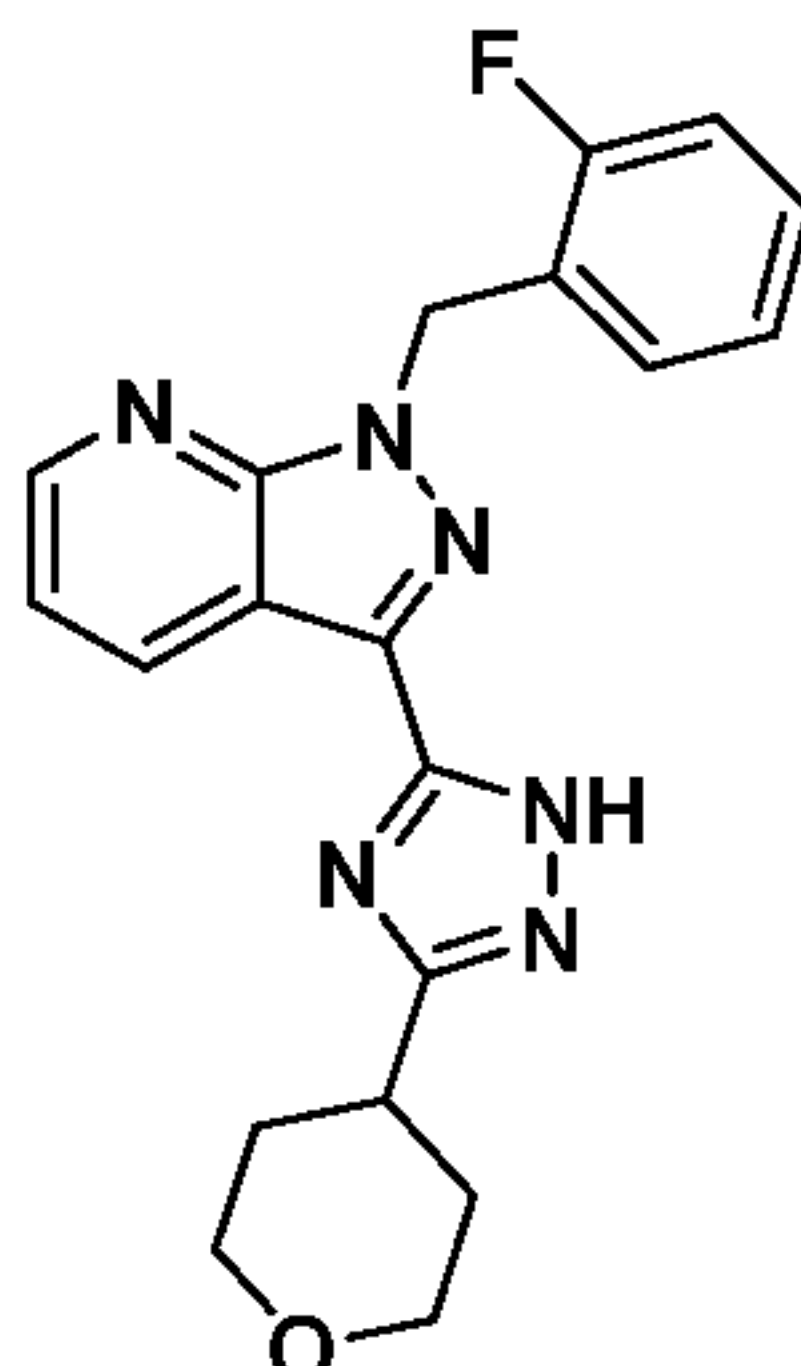
Compound I-78
