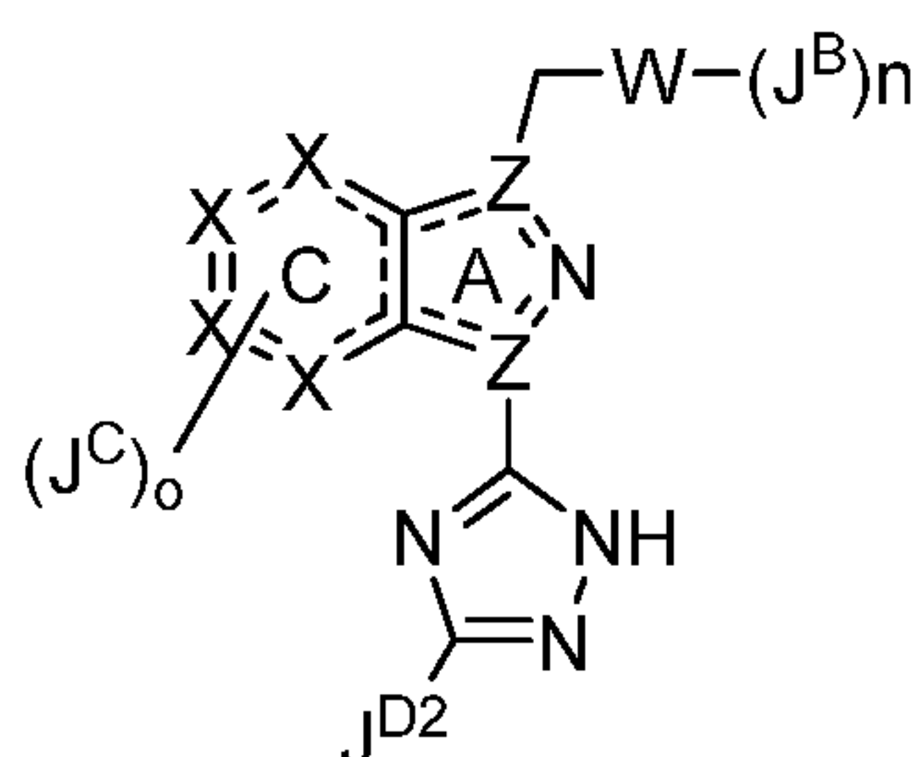
Formula IIA
