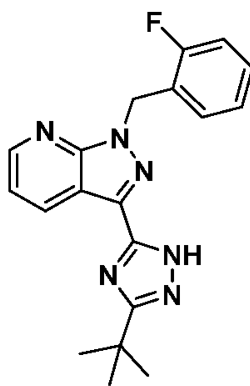
Compound I-37
