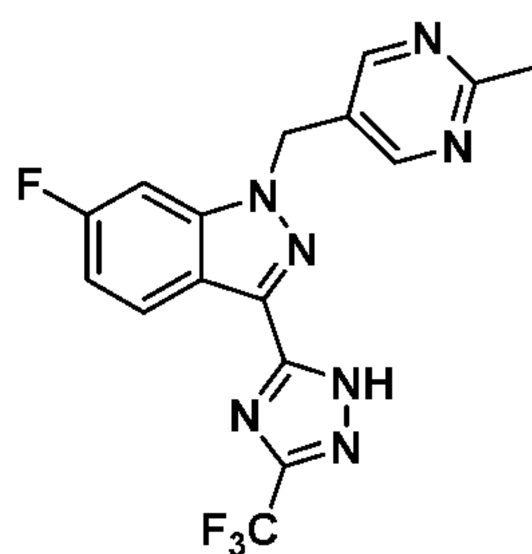
Compound I-61
