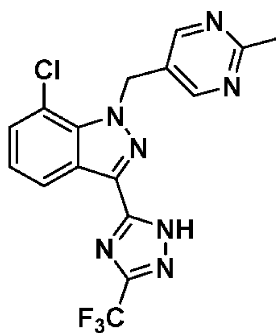
Compound I-46
