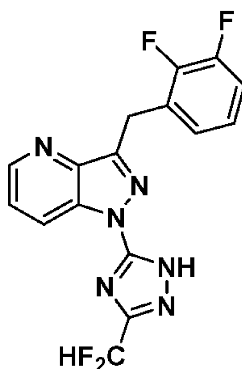
Compound I-127
