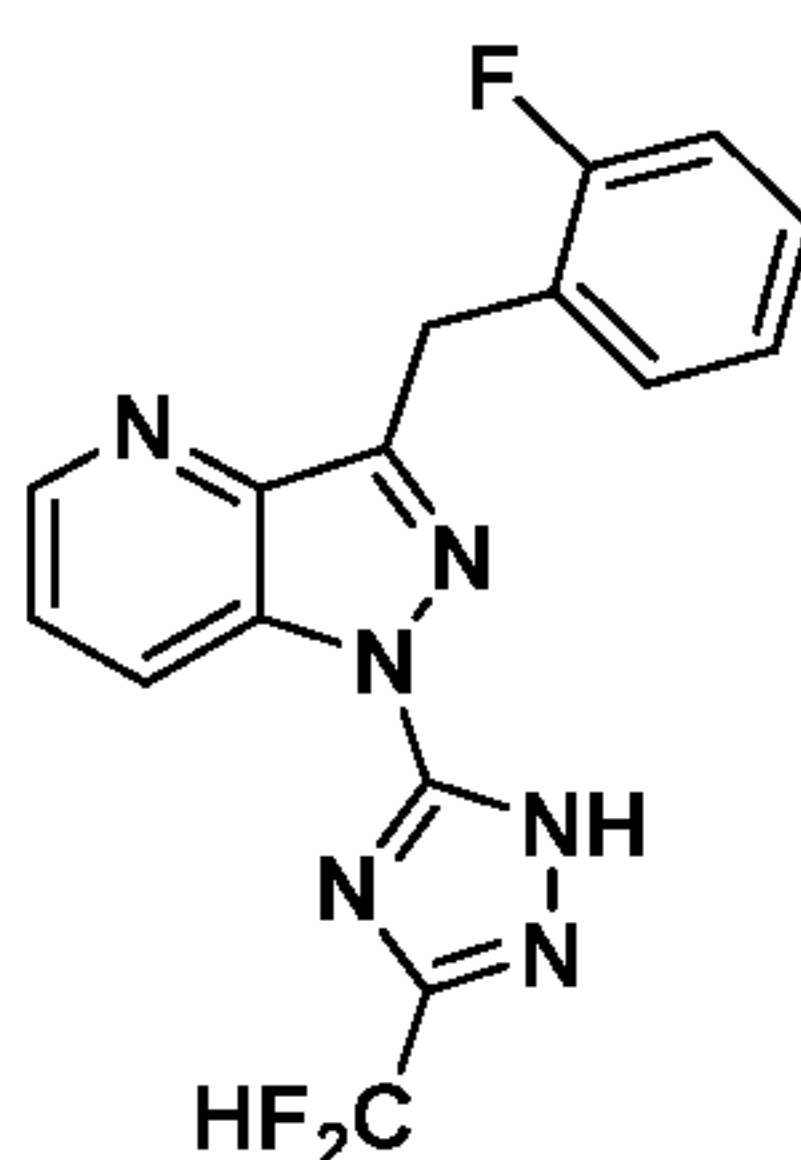
Compound I-101
