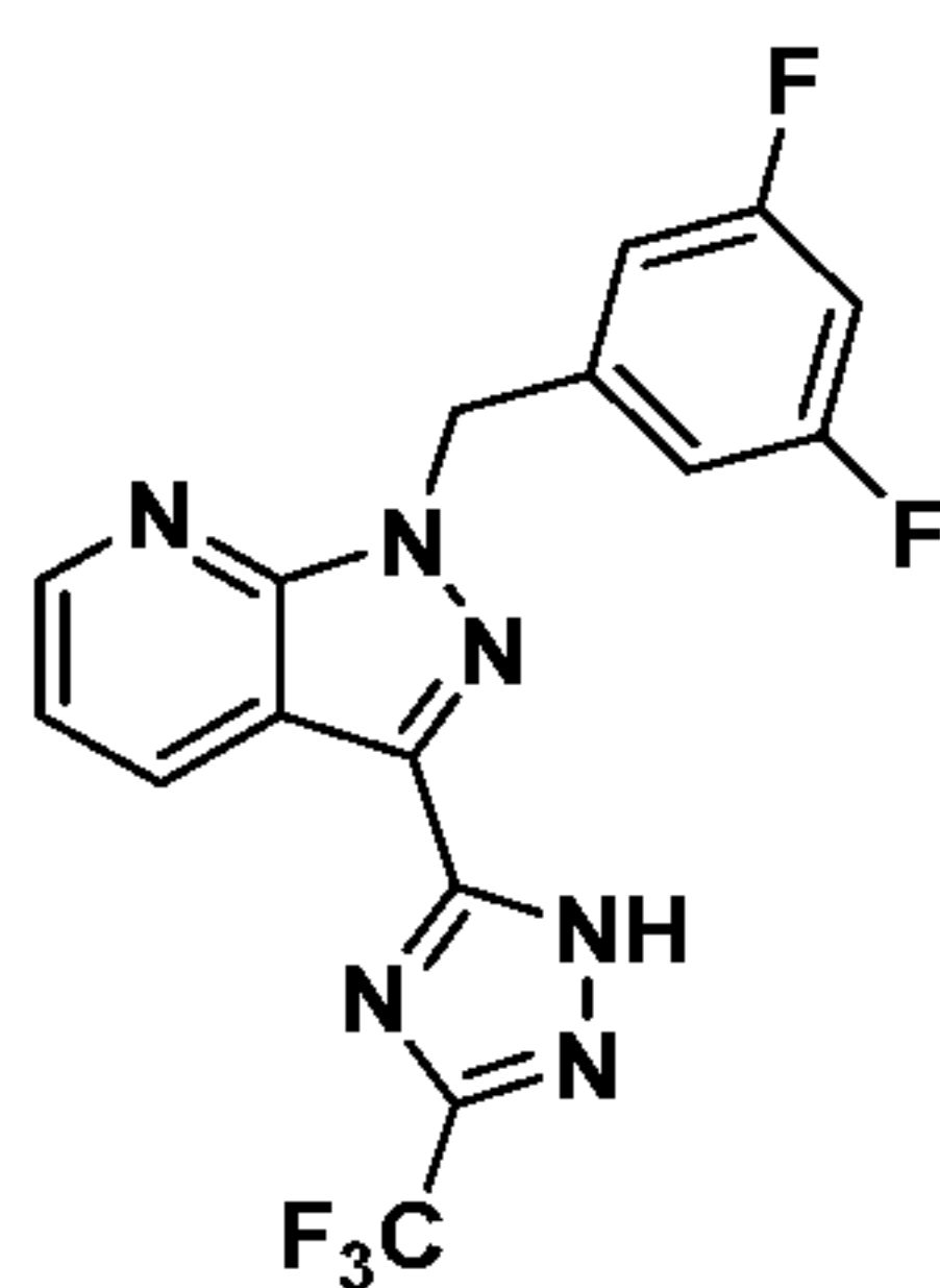
Compound I-51
