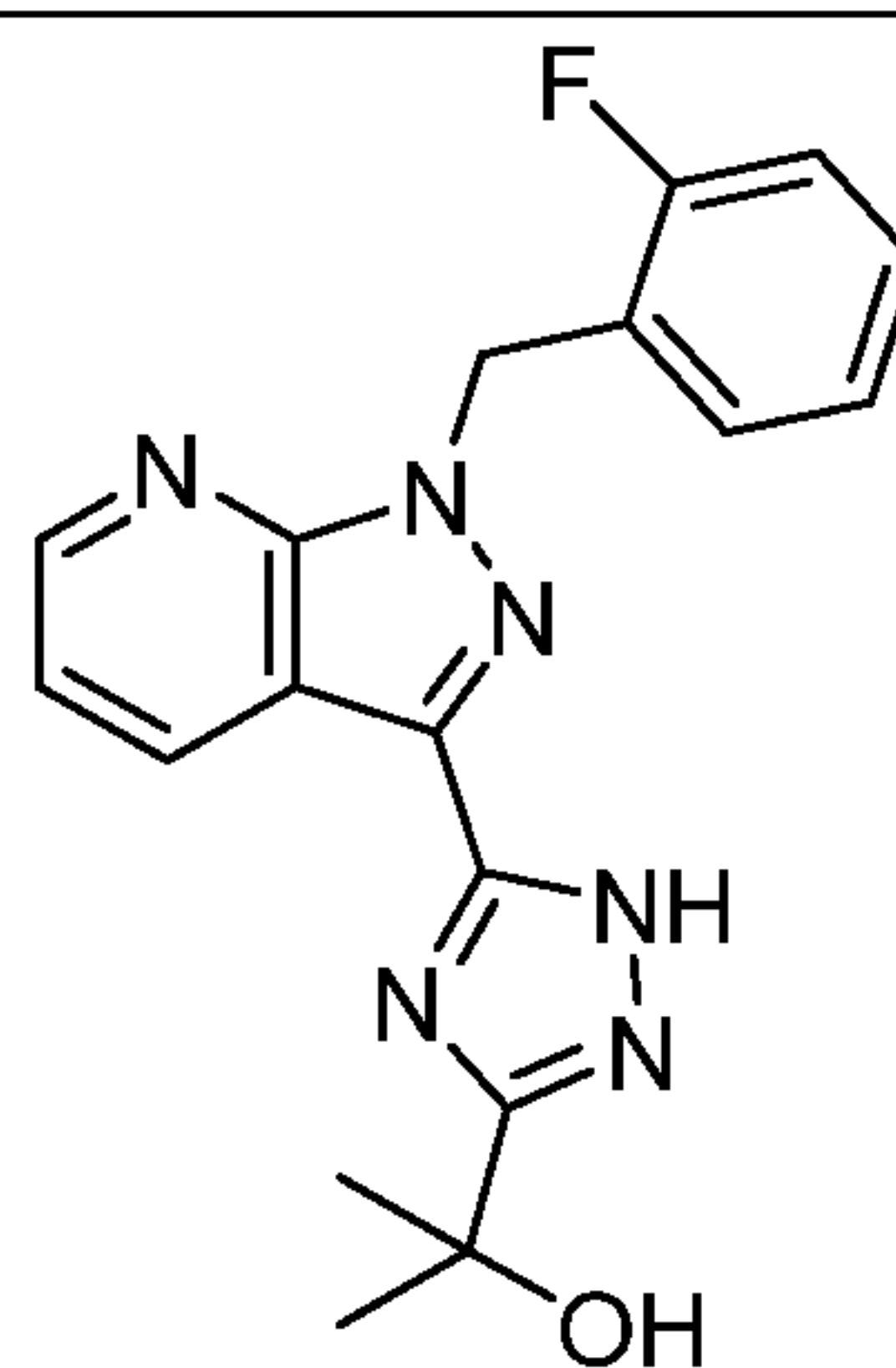
I-94
