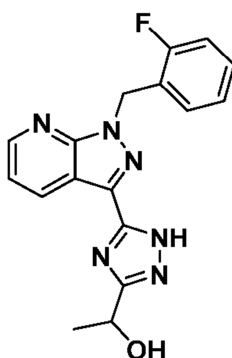
Compound I-107
