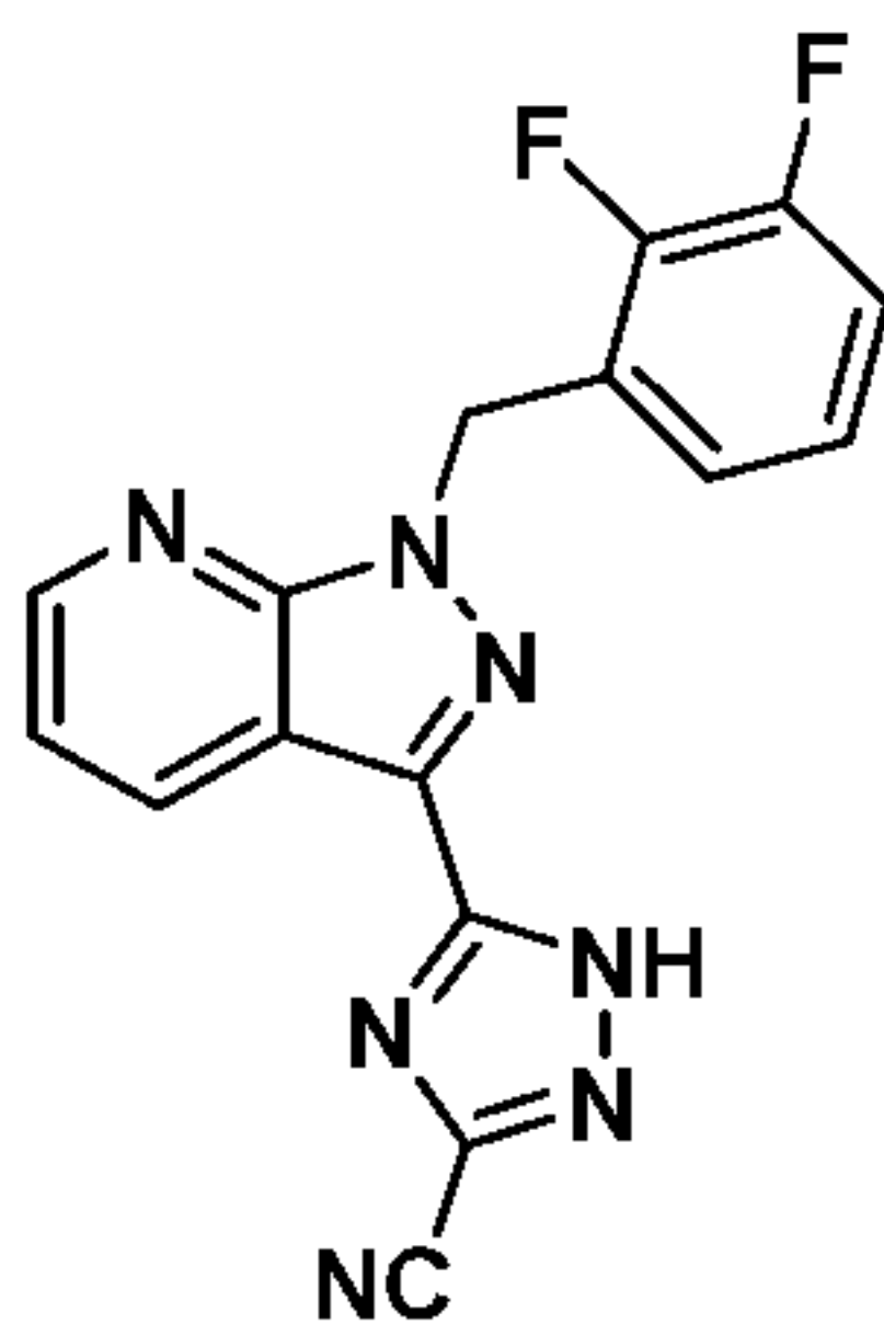
Compound I-92
