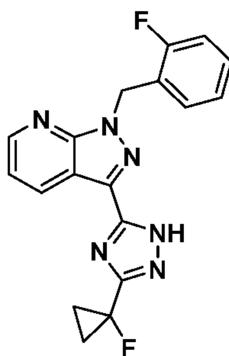
Compound I-80
