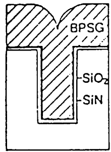
1 BPSG deposition
