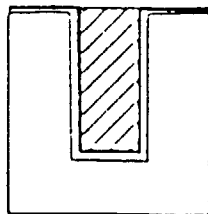
3 BPSG etchback
