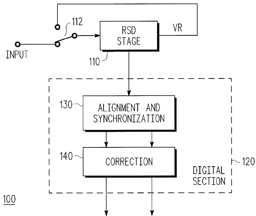
FIG. 1 (CONVENTIONAL)
