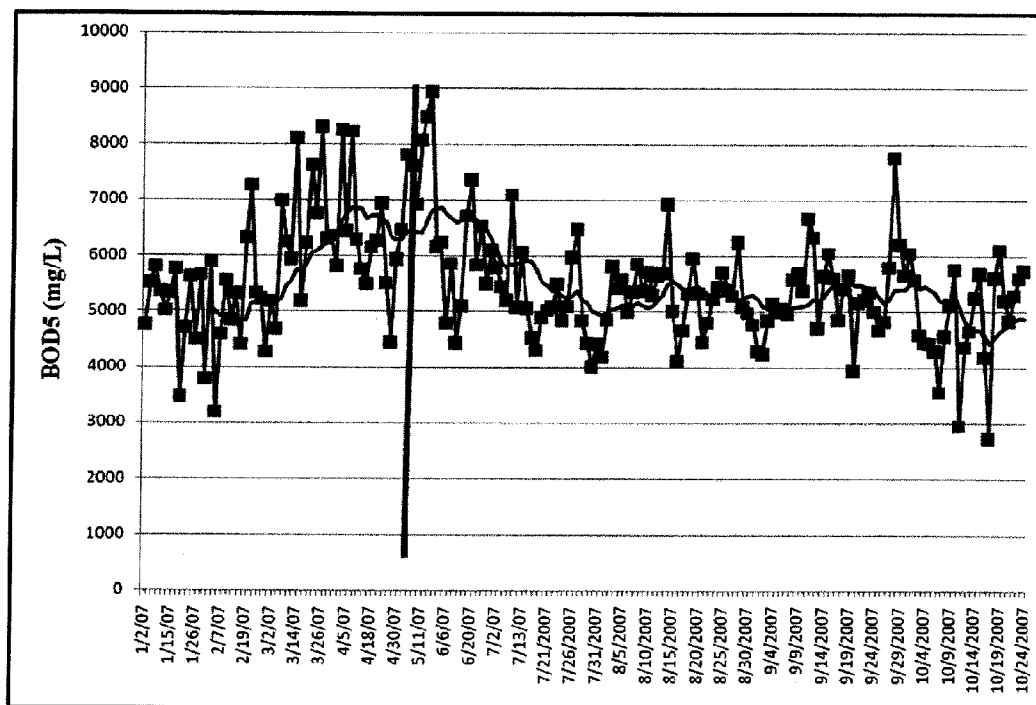
Reduction of Effluent BOD 5
