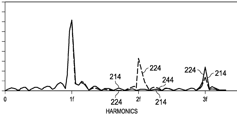
FIG. 1C (PRIOR ART)
