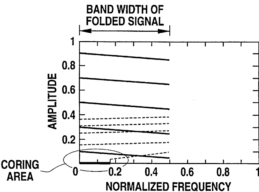
ADAPTIVE DEEMPHASIS OF FOLDED HIGH LUMA
