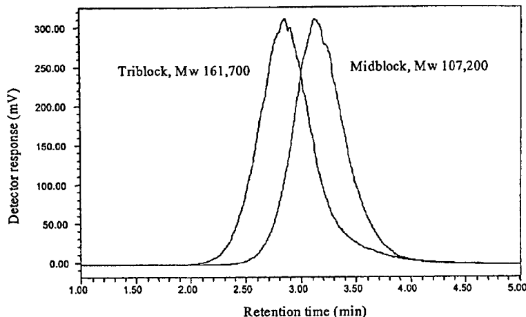
SEC traces of midblock and triblock polymers
