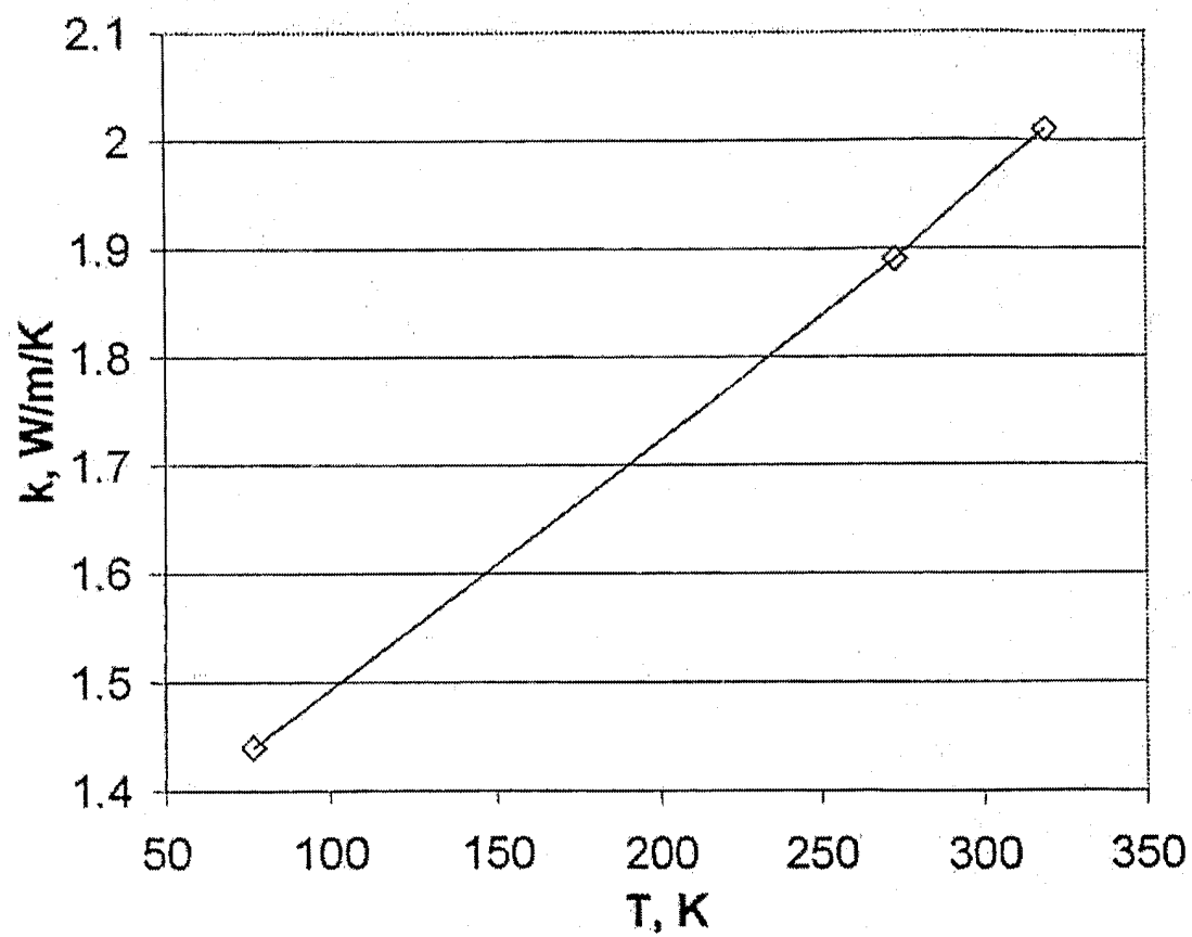
Figure 4. Thermal conductivity of termination dielectric material.
