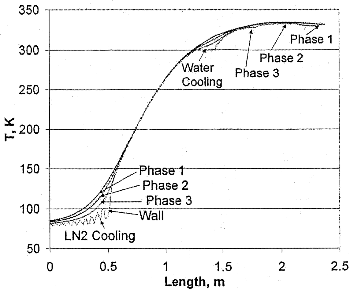
Figure 5. ANSYS predicted temperature profiles in the termination.
