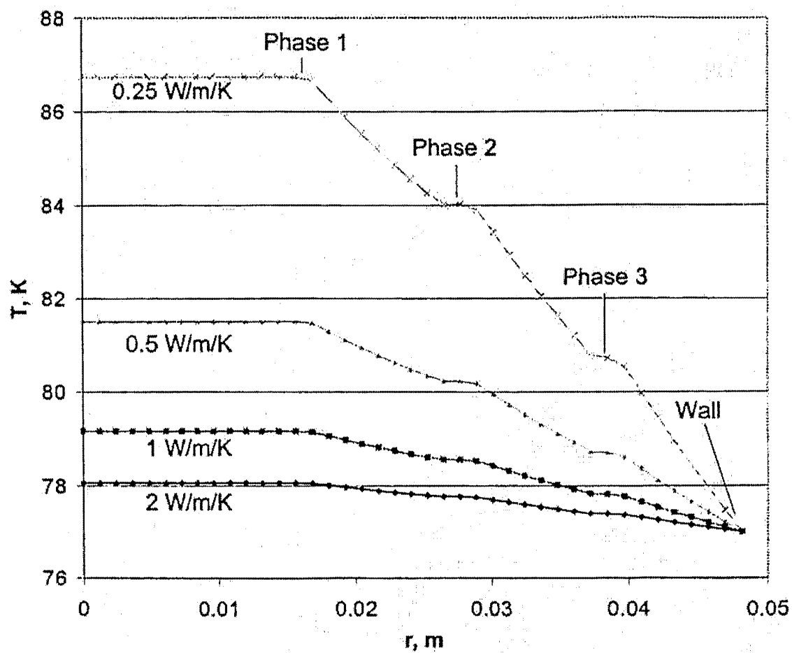
Fig. 3. Radial temperature profile of the tri-axial termination.
