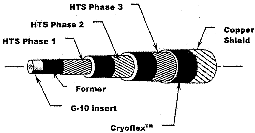
Fig. 2. Schematic of the tri-axial cable.
