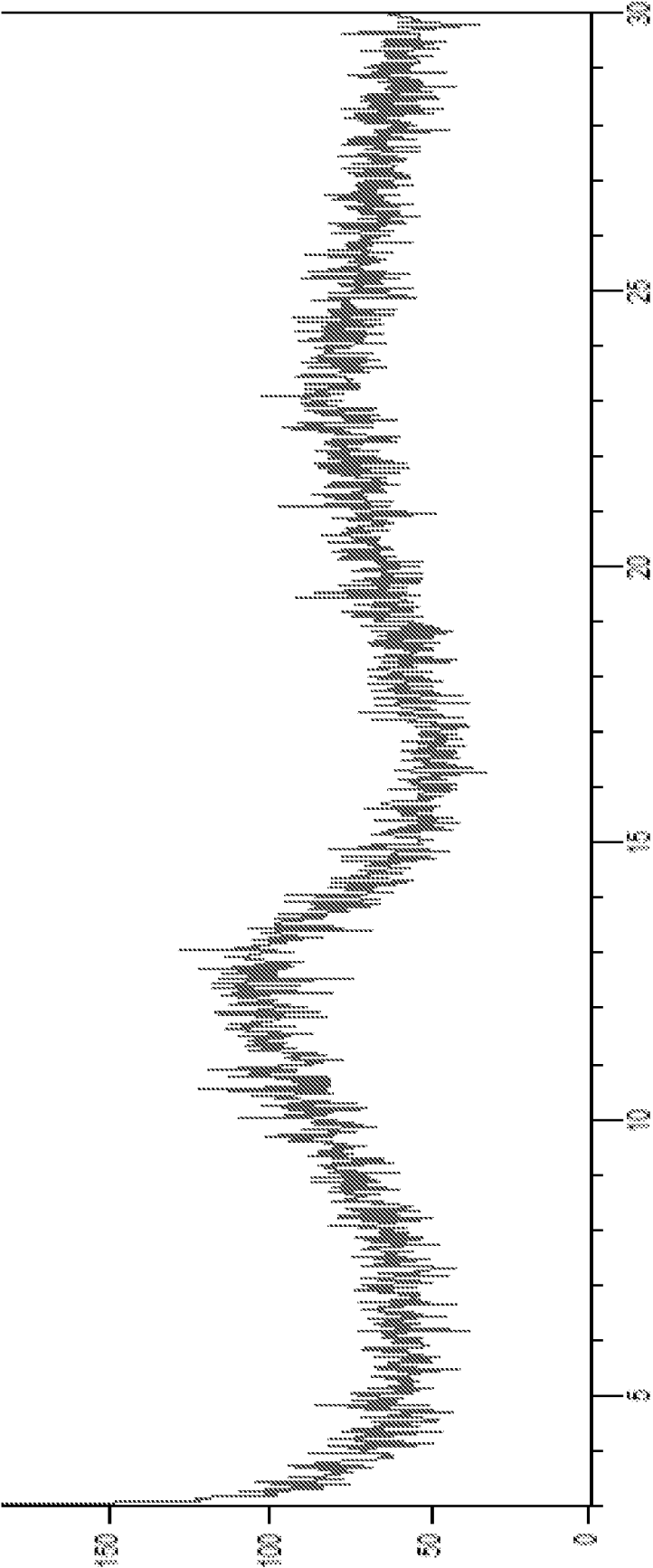
Position [° 2theta]
