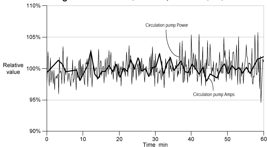
Fig.1 Power and Amps on slurry circulation pump
