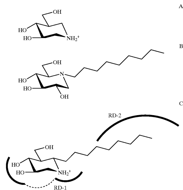
1(A) Isifagomine or hydroxy-piperidine; 1(B) N-nonyl 1-deoxynojirimycin; 1(C) 6-C-nonyl hydroxypiperidine, RD-1: recognition domain 1; RD-2: recognition domain 2.
