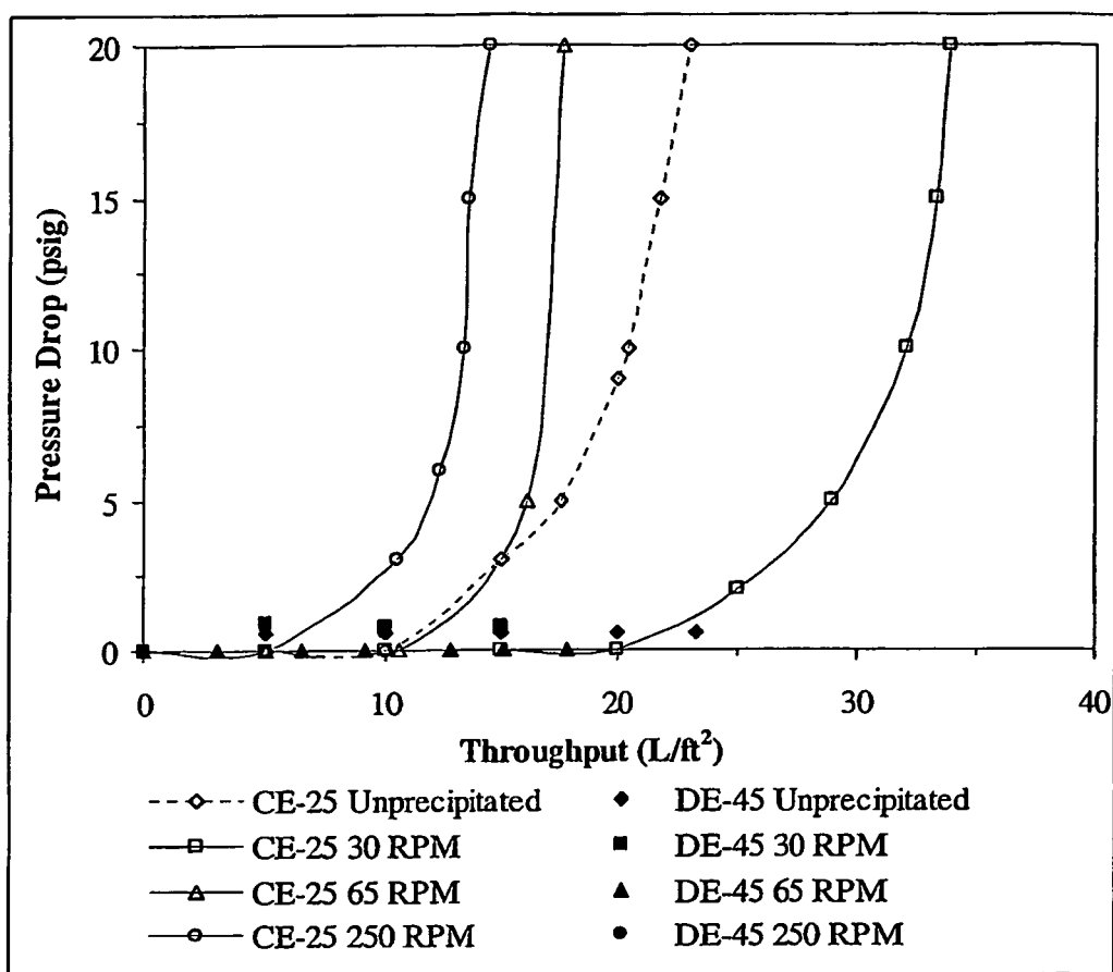
Depth Filtration Capacities for Various Precipitation Conditions
