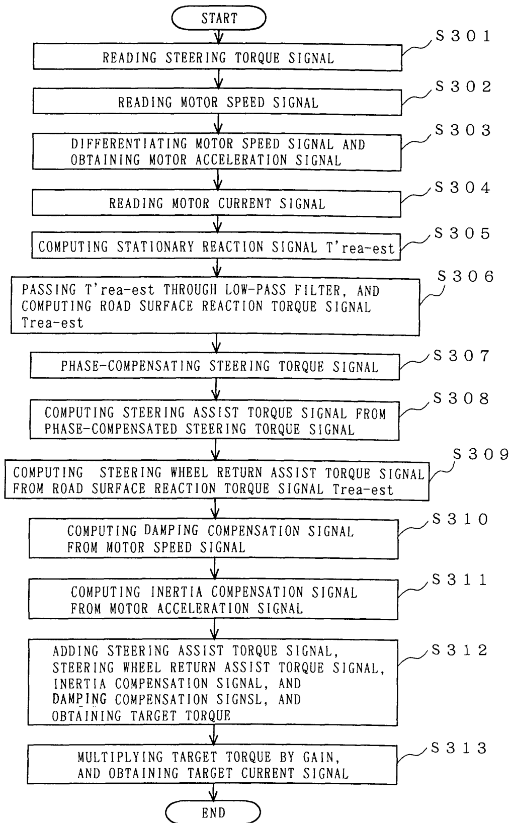
Fig. 11 (PRIOR ART)
