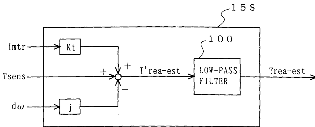
Fig. 12 (PRIOR ART)
