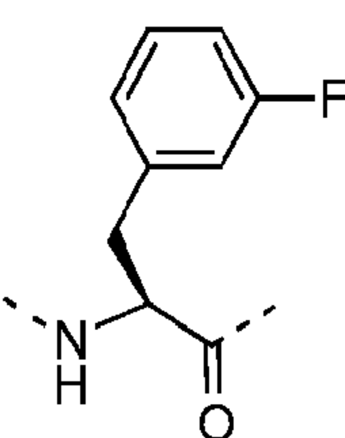
3-fluorophenylalanine (F3F=3ff)
