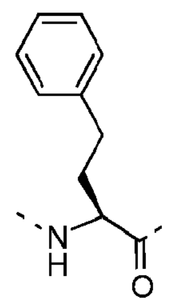
homophenylalanine (hF)
