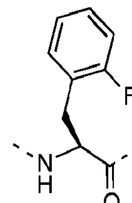
2-fluorophenylalanine (F2F=2ff)
