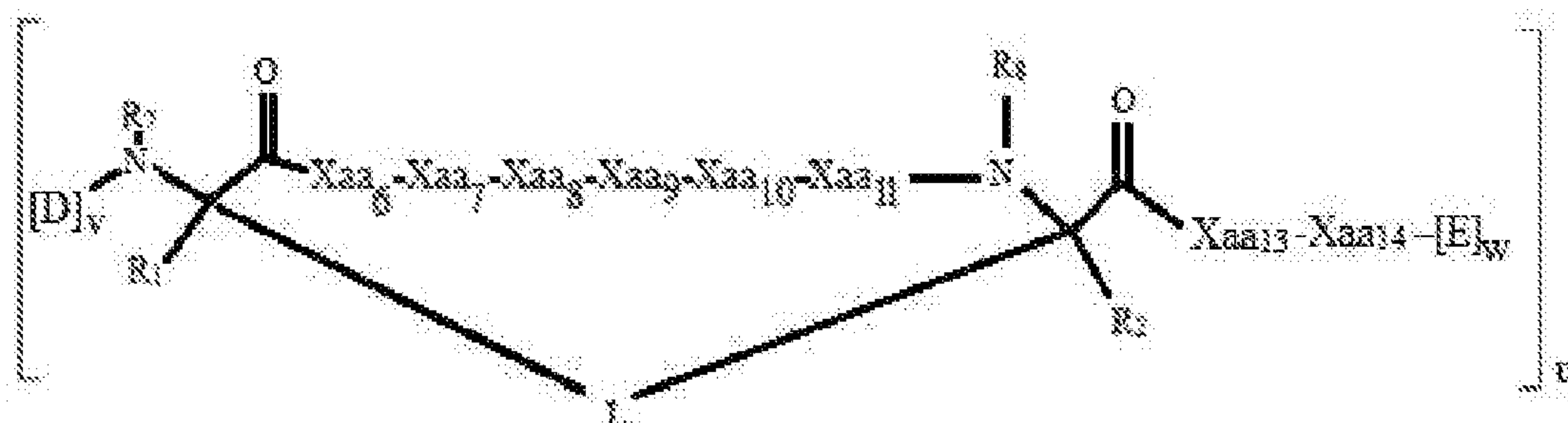
Formula (Ib-1)
