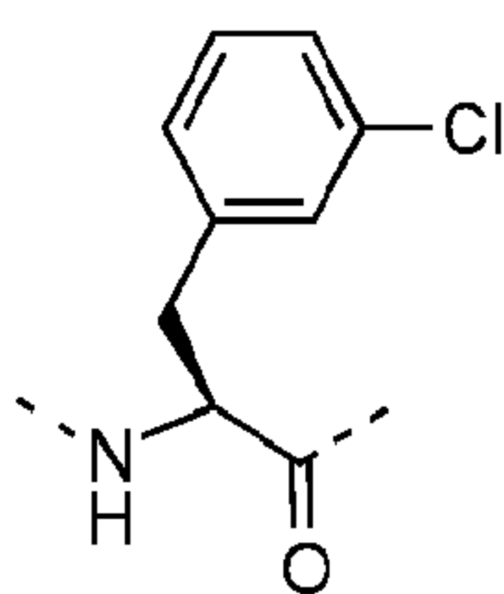
3-chlorophenylalanine (F3Cl=3cf)
