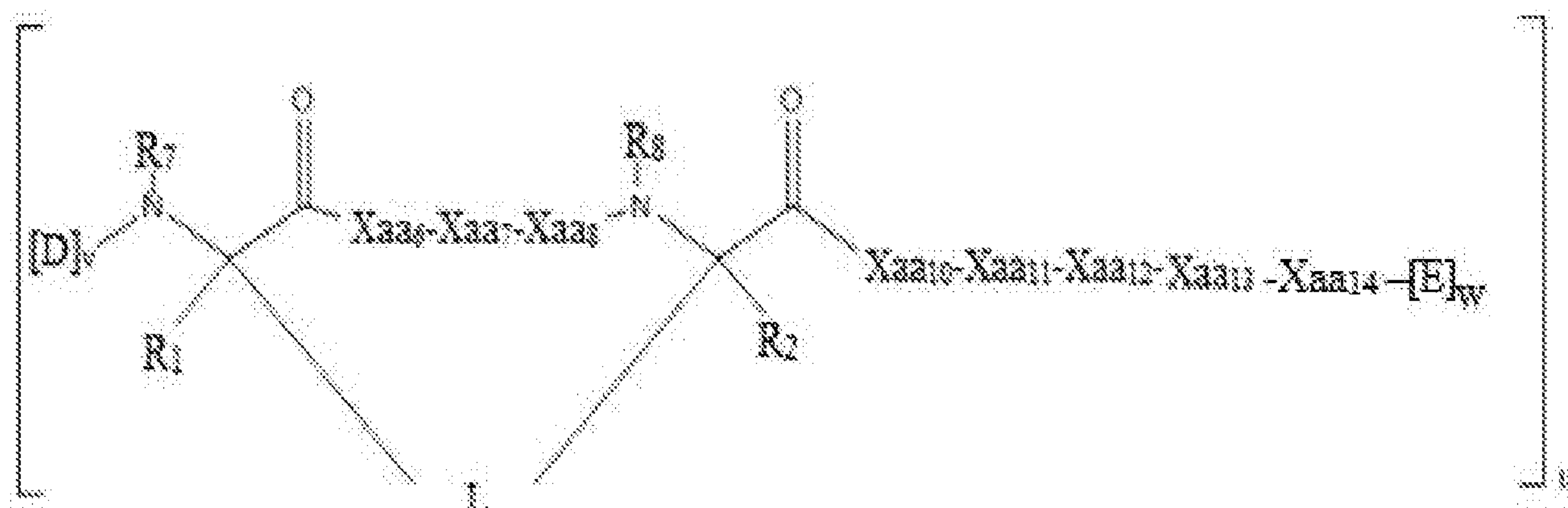
Formula (Ia-1)
