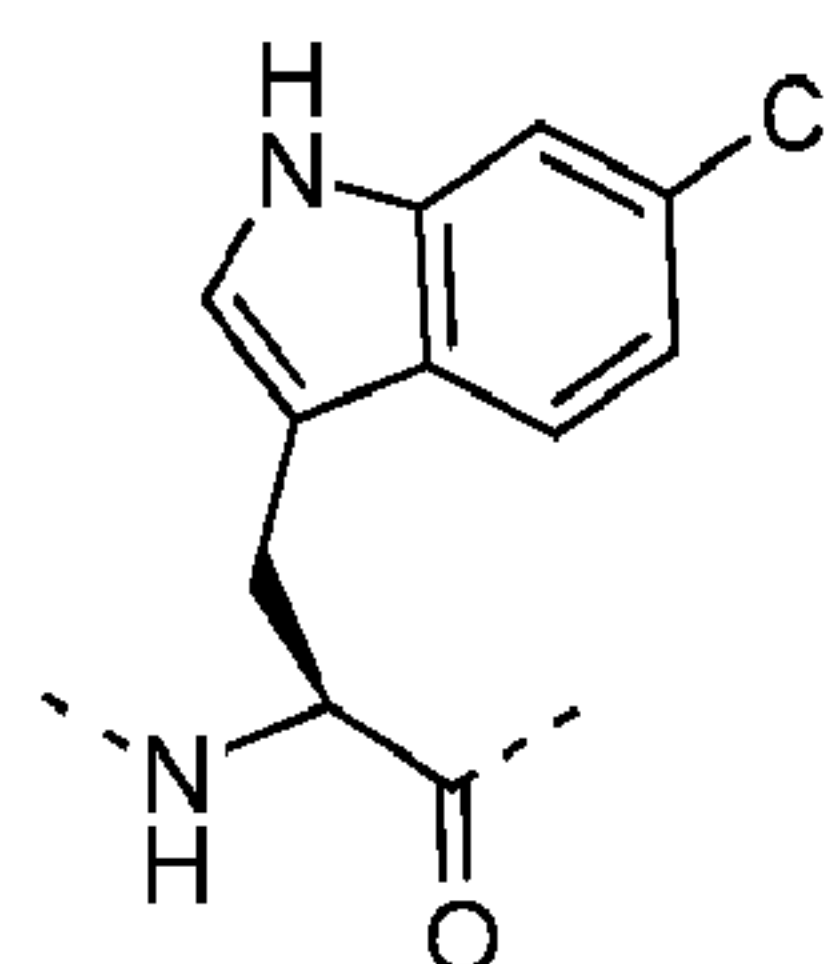
6-chlorotryptophan (6clW)
