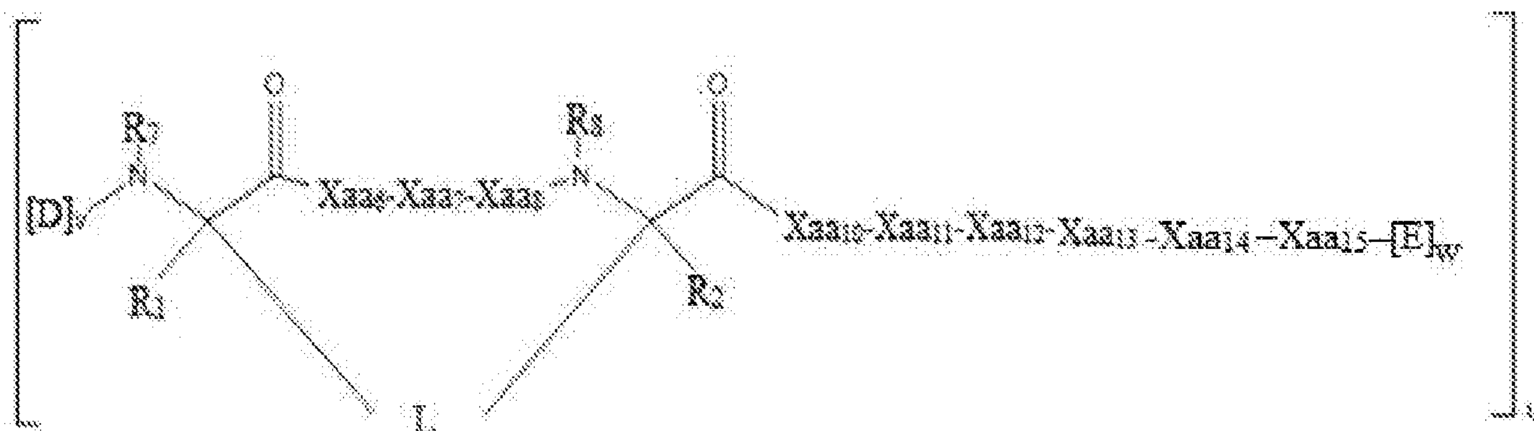
Formula (Ia-2)
