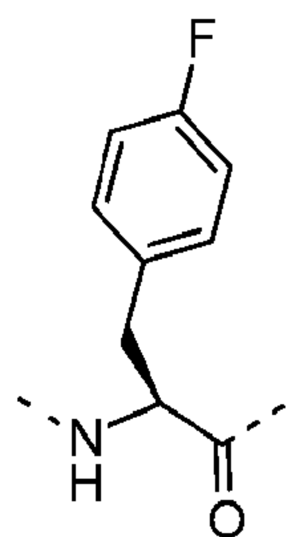
4-fluorophenylalanine (F4F)
