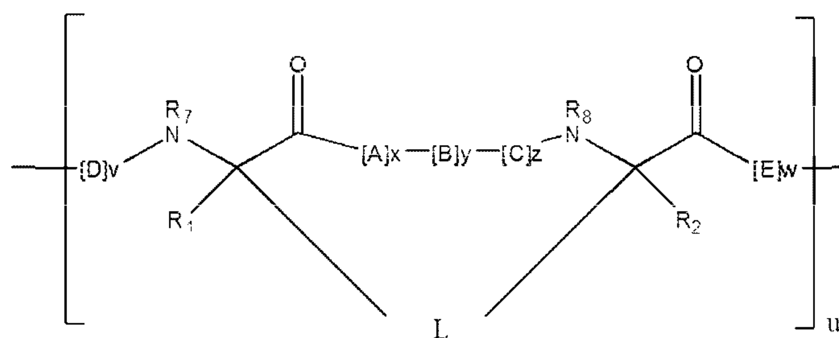
Formula (I)
