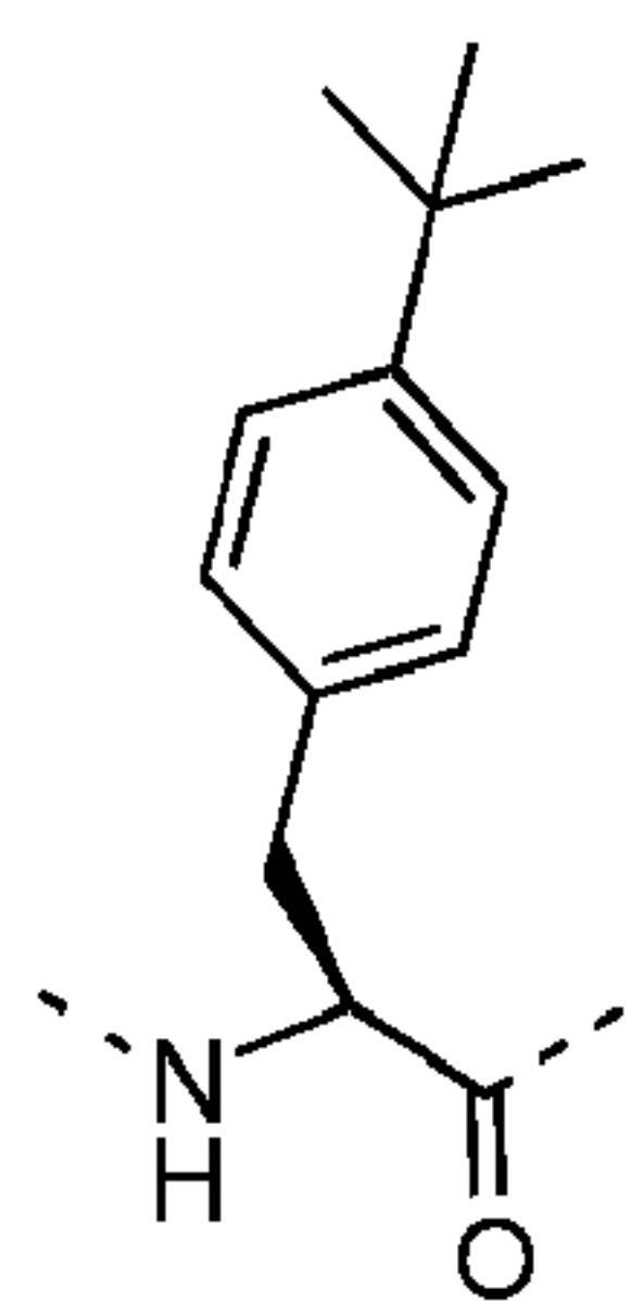
4-t-butylphenylalanine (F4tBu)
