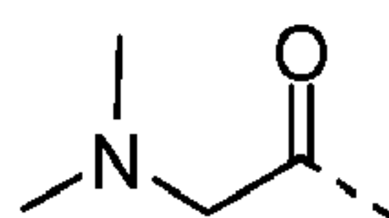
N,N-Dimethylaminoacetyl
