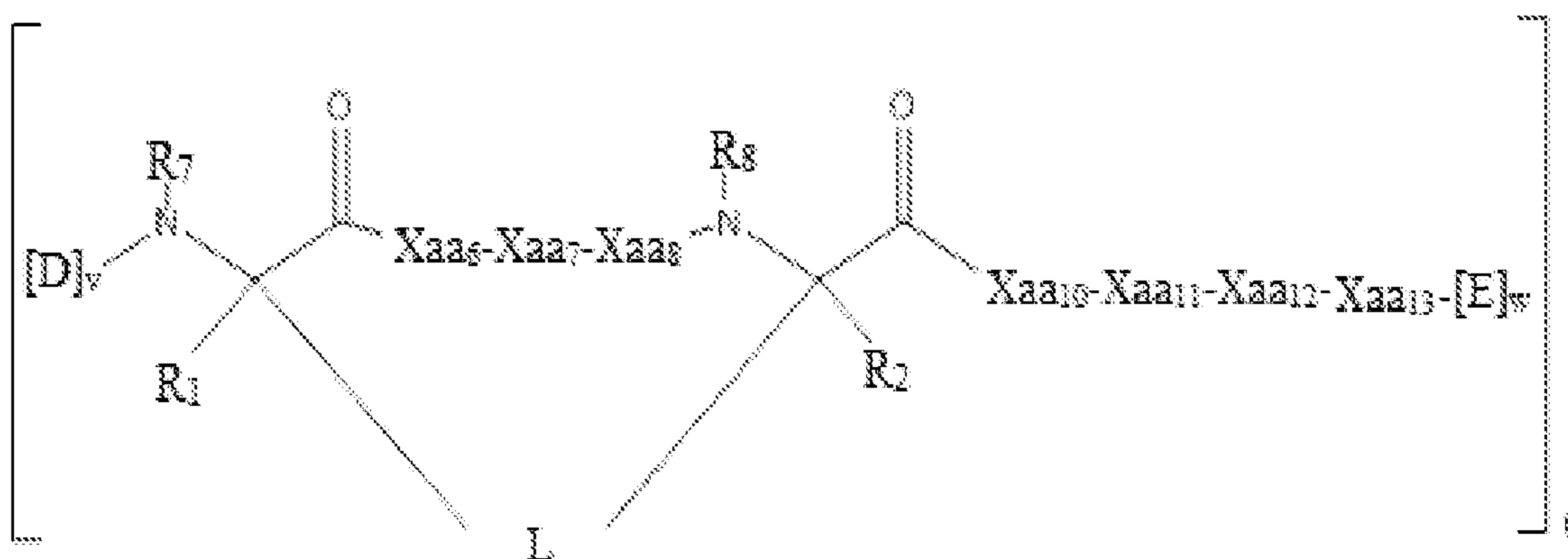
Formula (Ia)
