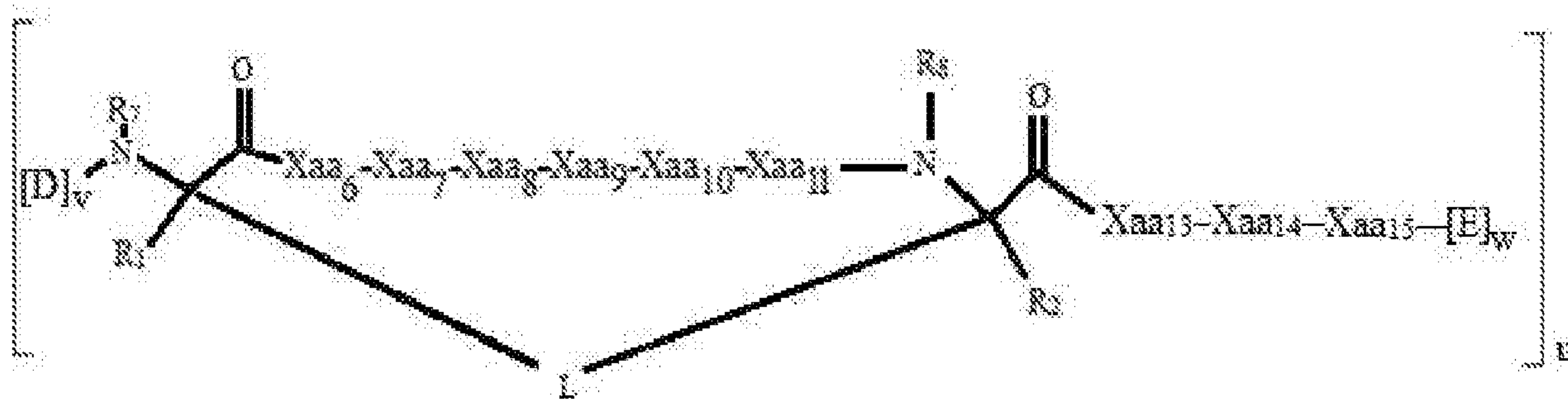
Formula (Ib-2)
