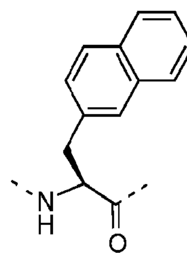
2-Naphthylalanine (2NaI)
