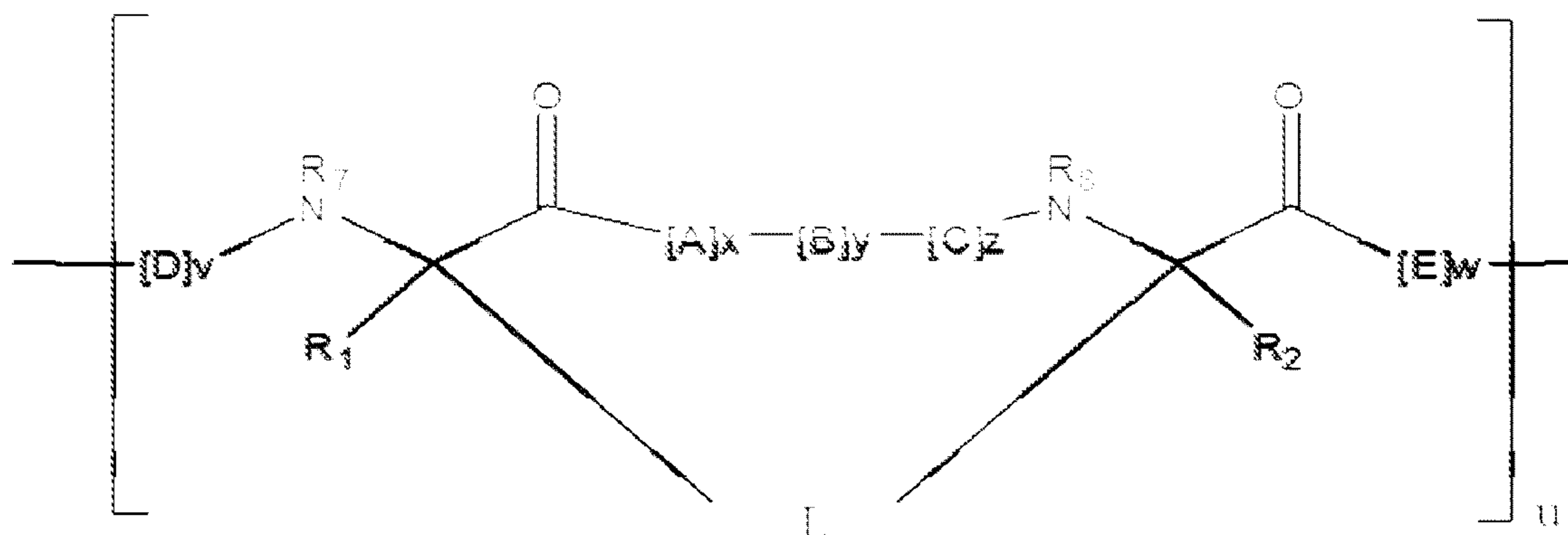
Formula (I)
