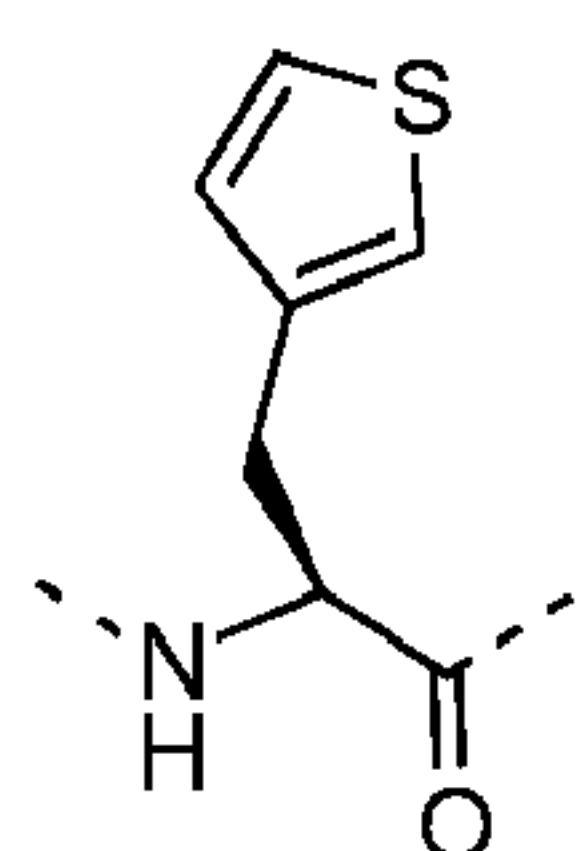
3-thienylalanine (2Thi)
