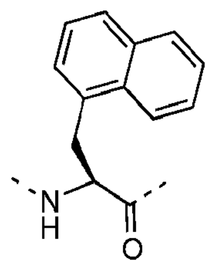
1-Naphthylalanine (1NaI)
