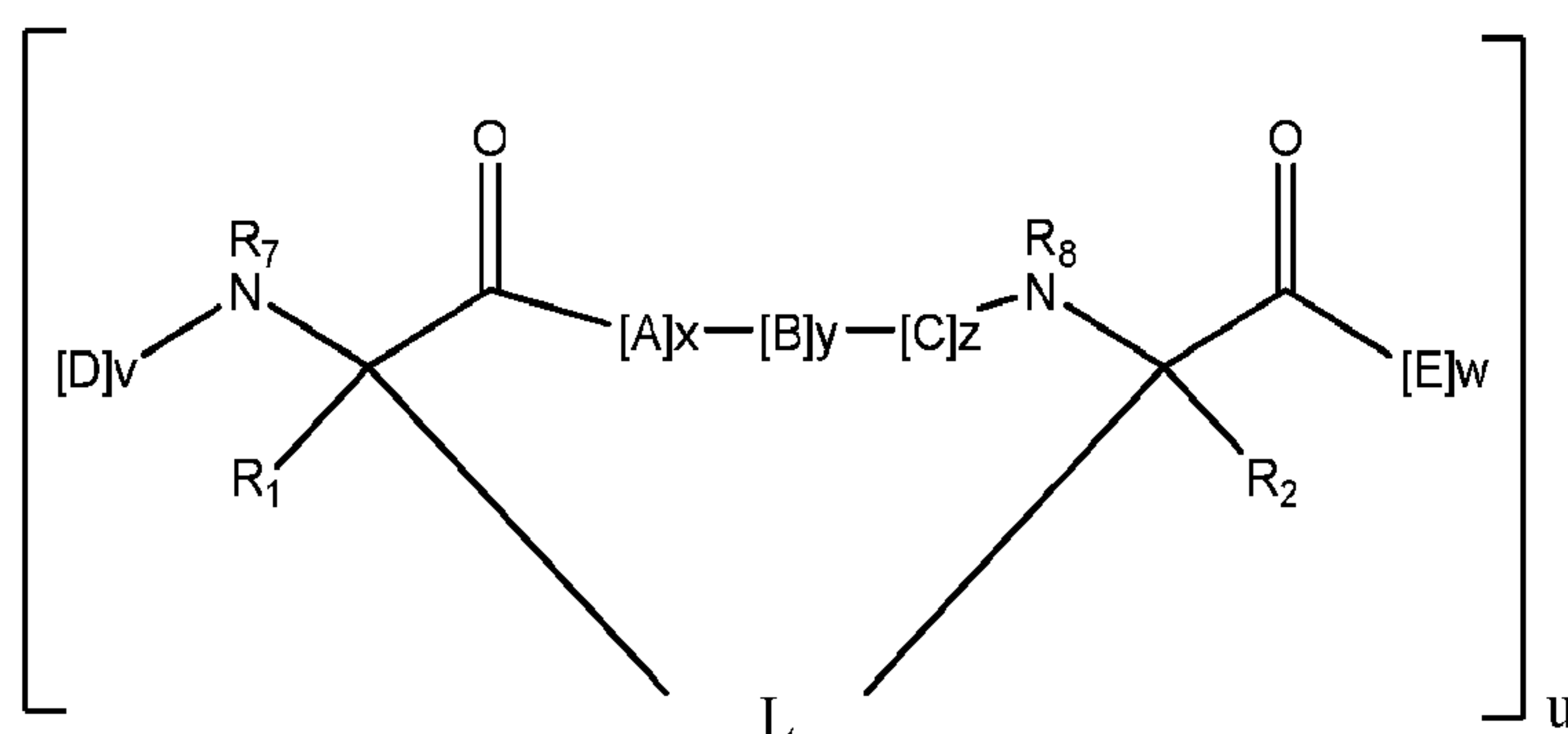
Formula I
