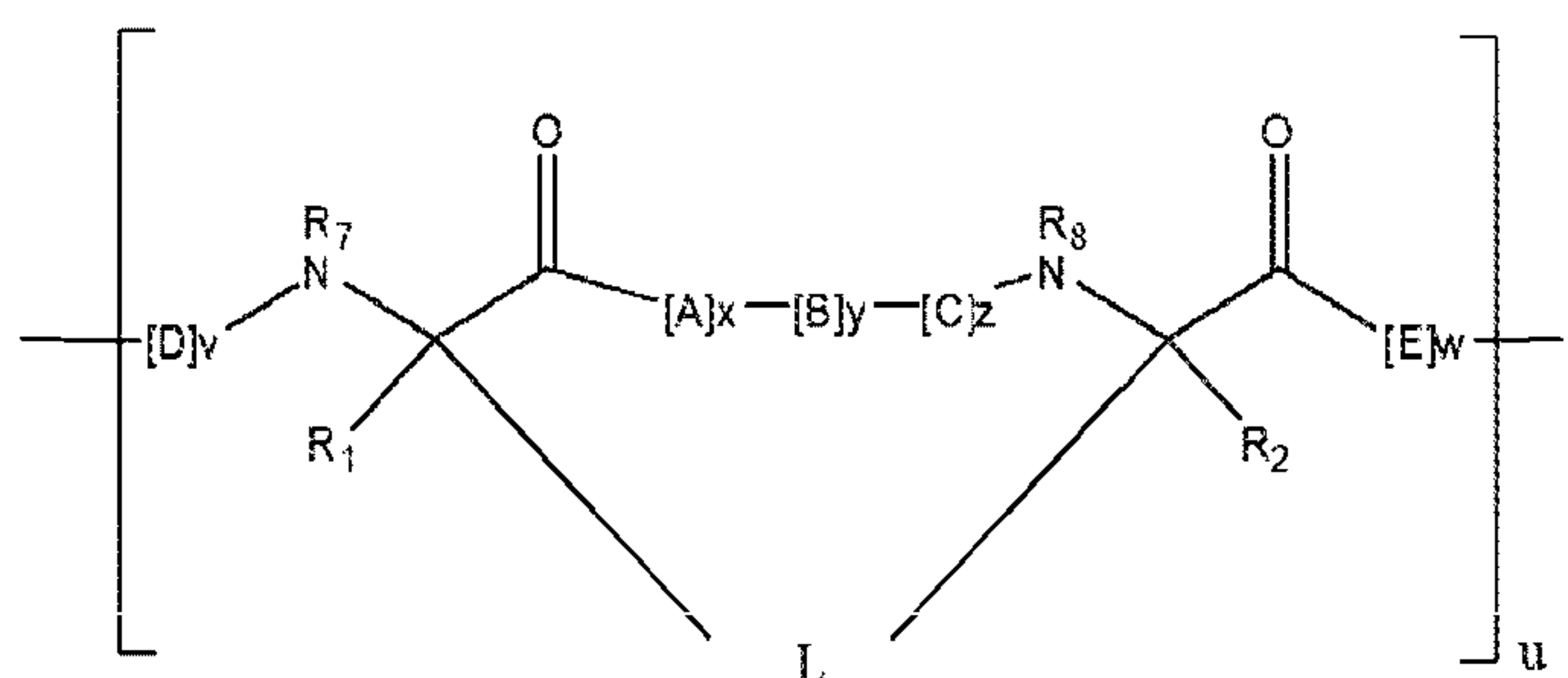
Formula (I)
