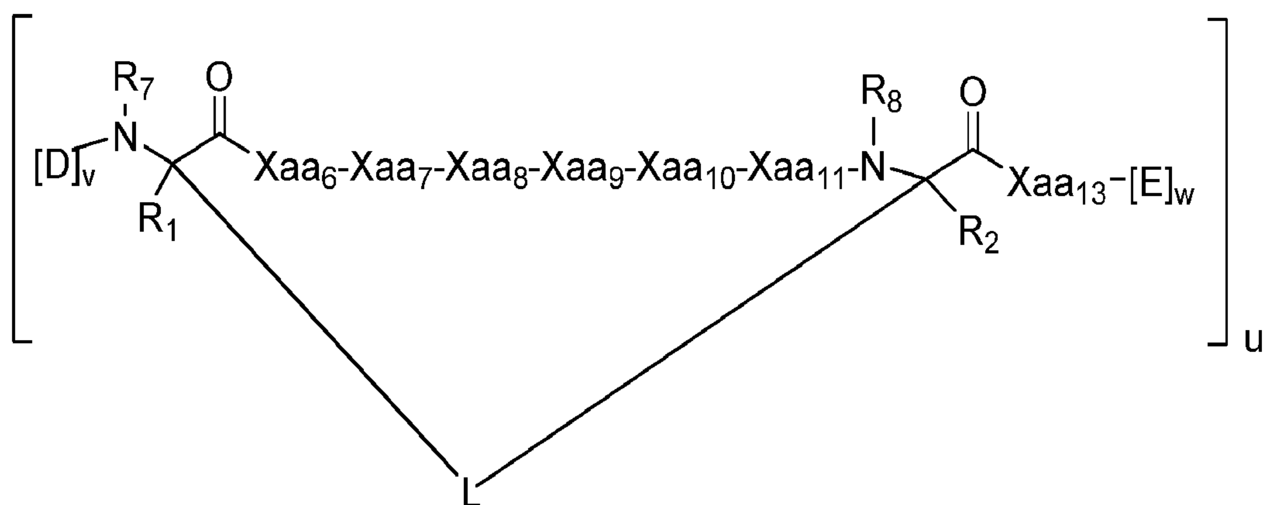
Formula (Ib)
