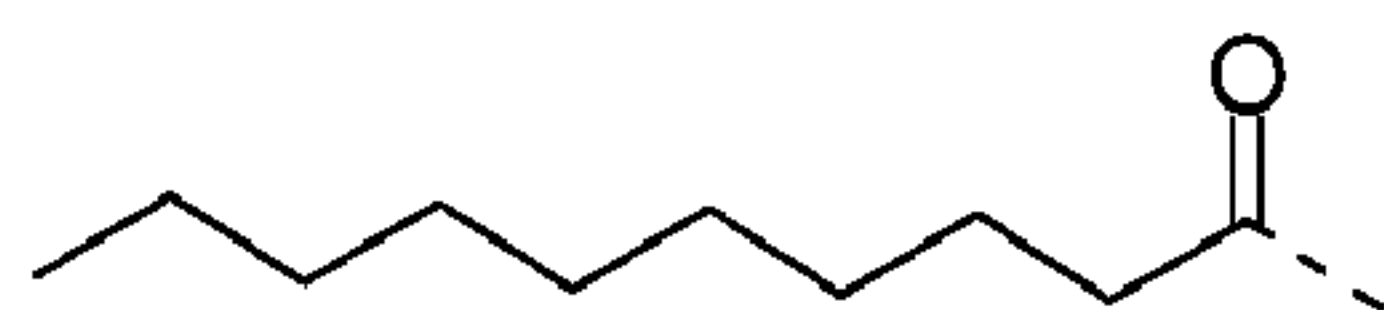
Decanoyl (Decac)
