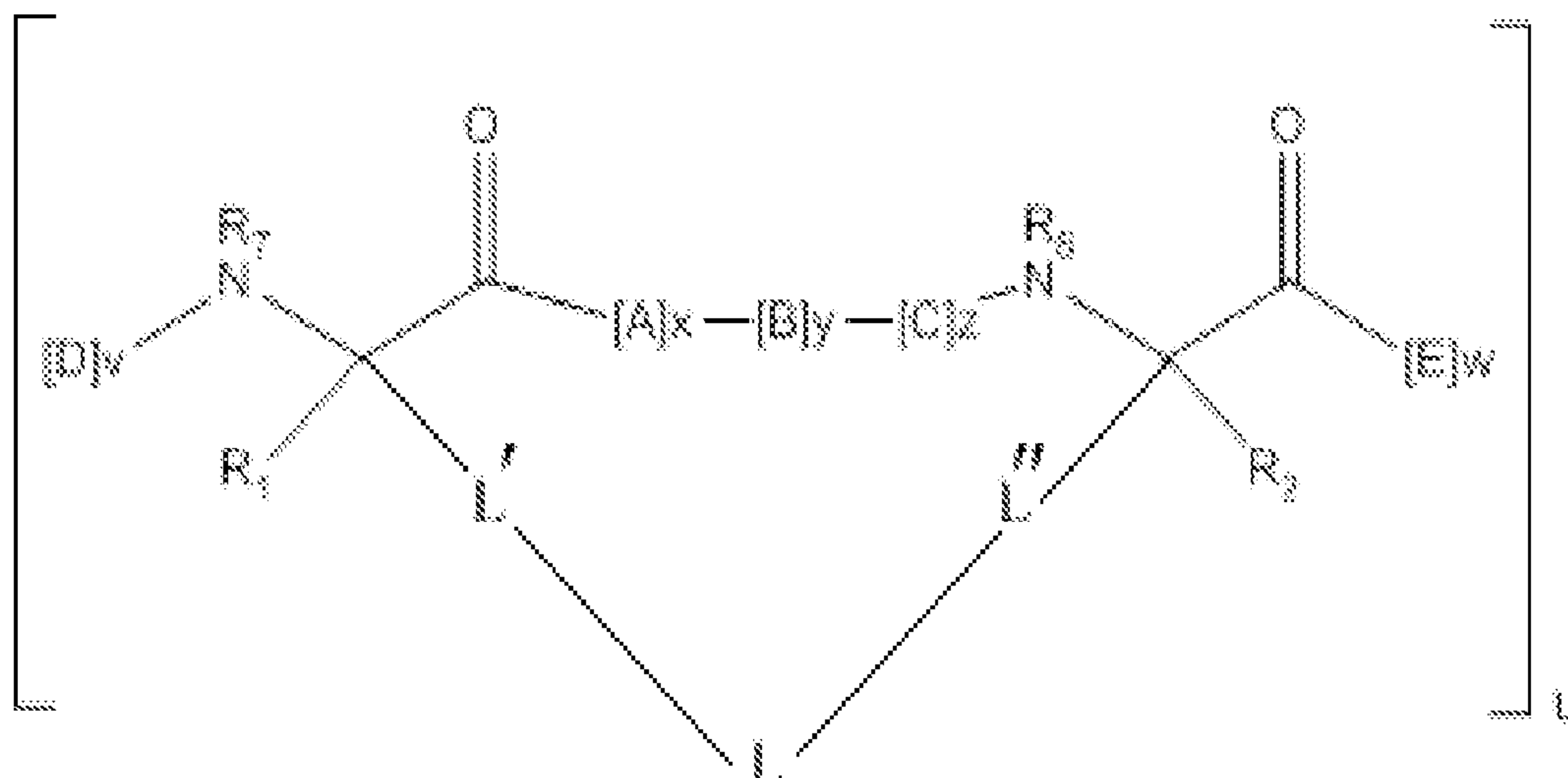
Formula (IX)
