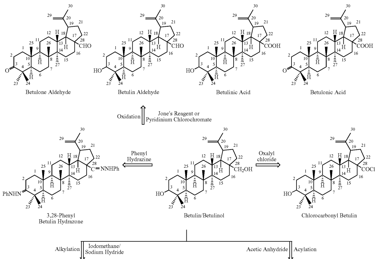
Scheme 1. Synthesis of Betulinol Derivatives
