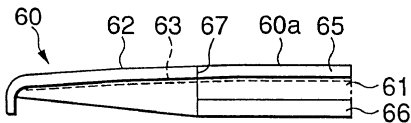
FIG.13 PRIOR ART
