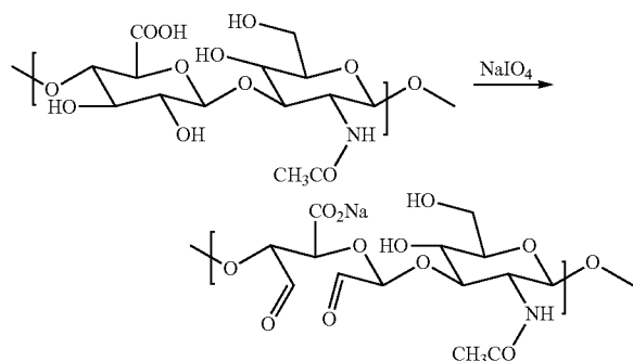
Scheme 3 Oxidation to a dialdehyde
