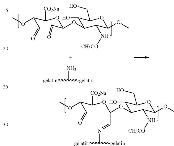
Scheme 4 Cross-linking reaction of the oxidized hyaluronan and gelatin
