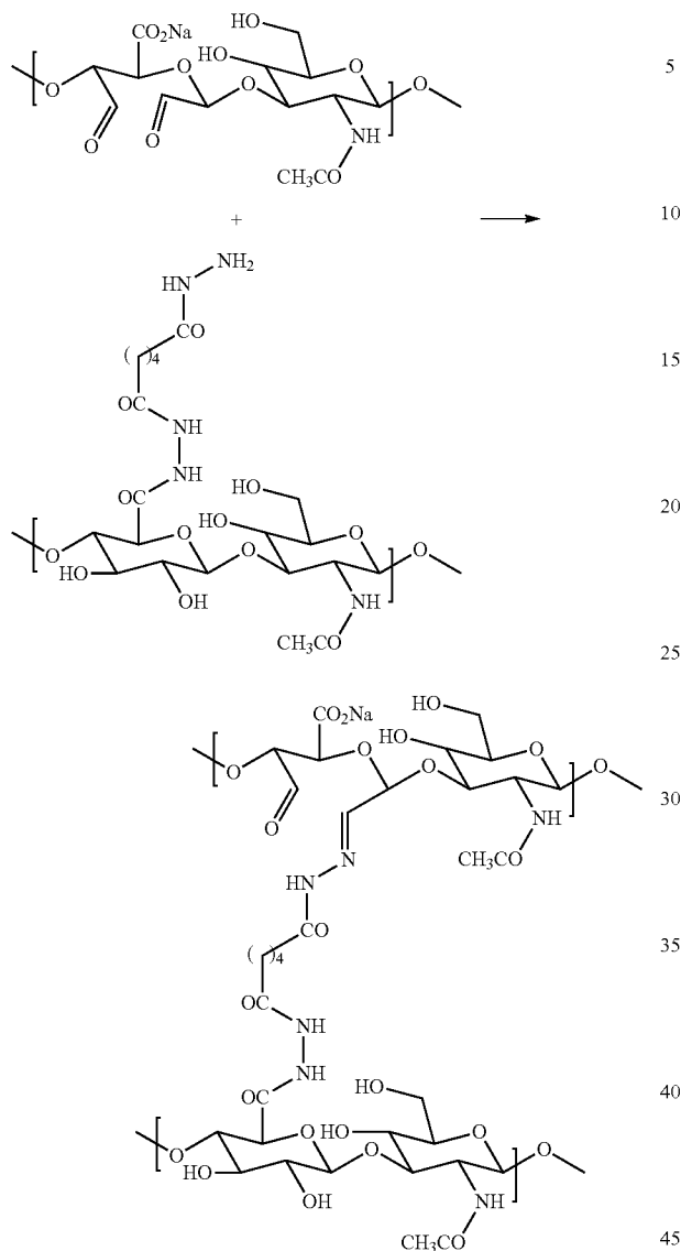
Scheme 5 Preparation of the cross-linked hyaluronan
