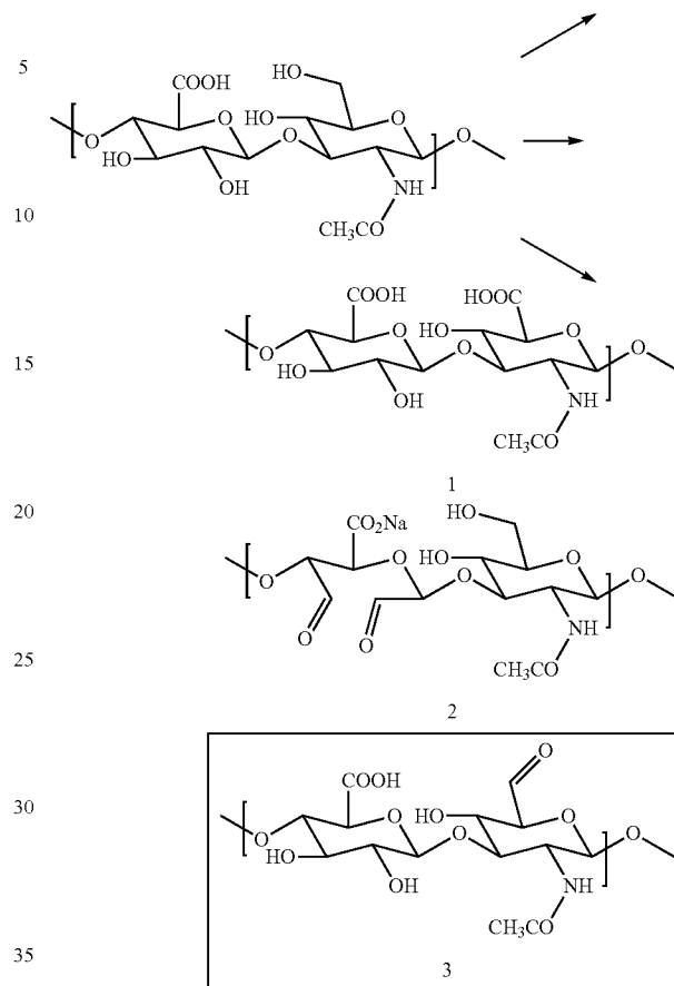
Scheme 6 Hyaluronan oxidation, reaction products
