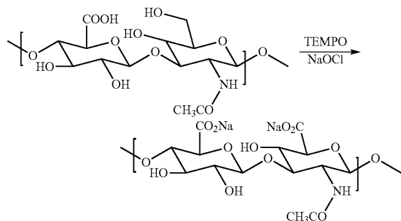
Scheme 2 Oxidation to a carboxylic acid
