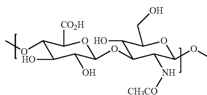
Scheme 1 The hyaluronic acid
