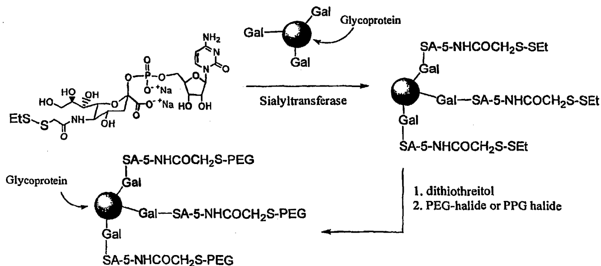
Scheme 6
