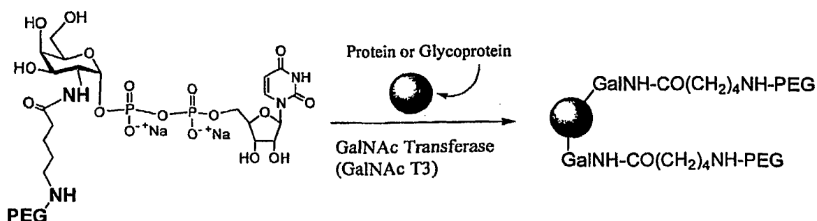
Scheme 7
