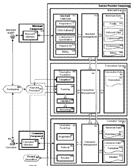
Fig. 1: Architecture of Transaction Settled Consumer Referral and Reward Service
