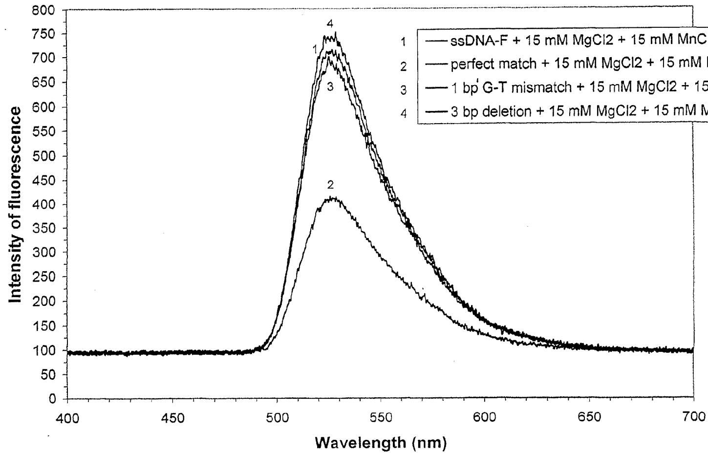
FIG. 5B. Binding of 15-mer antiparallel ssDNA-F probe (4 pmole) (33% GC) and 50-mer dsDNA (0.4 pmole) in the presence of divalent cations (after 1 hr)
