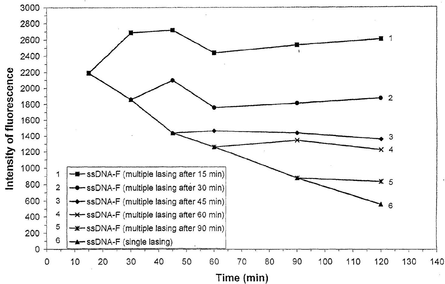
FIG. 6A. Effect of multiple laser treatment on cationic quench of 15-mer antiparallel ssDNA-F (4 pmole) by 10 mM MgCl 2 + 10 mM MnCl 2
