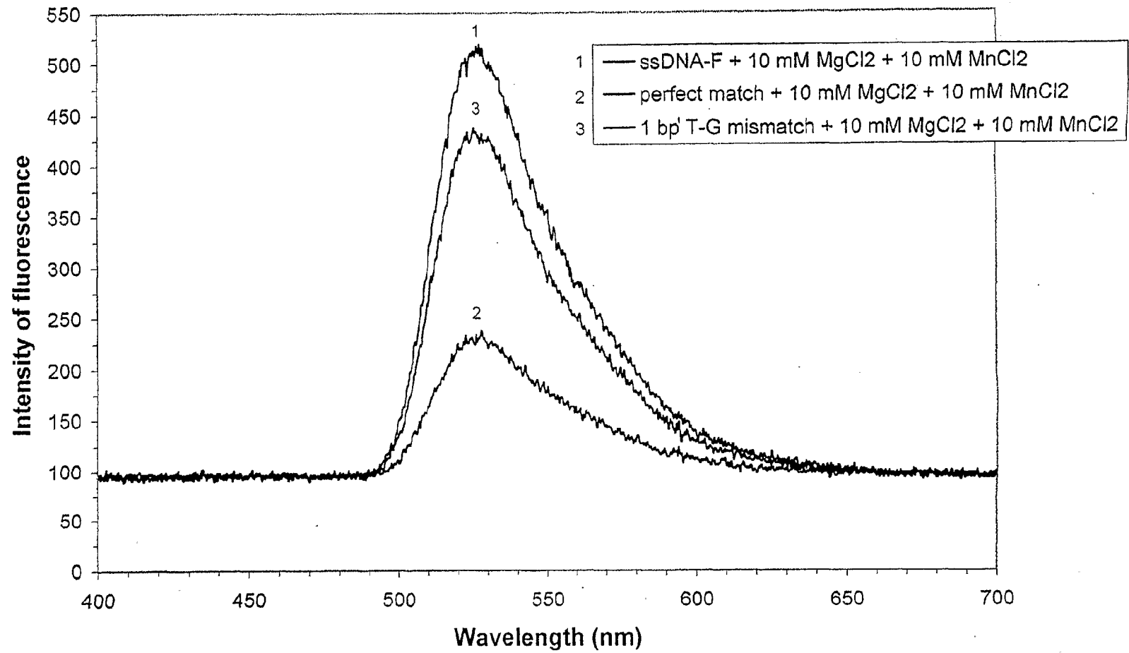
FIG. 5C. Binding of 15-mer antiparallel ssDNA-F probe (4 pmole) (53% GC) and 50-mer dsDNA (0.4 pmole) in the presence of divalent cations (after 1 hr)
