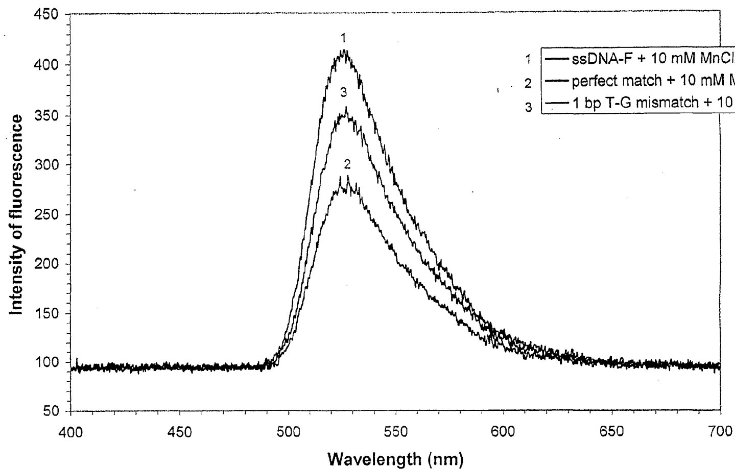
FIG. 4. Binding of 15-mer antiparallel ssDNA-F probe (4 pmole) (53% GC) and 50-mer dsDNA (0.4 pmole) in the presence of divalent cations (after 1 hr)
