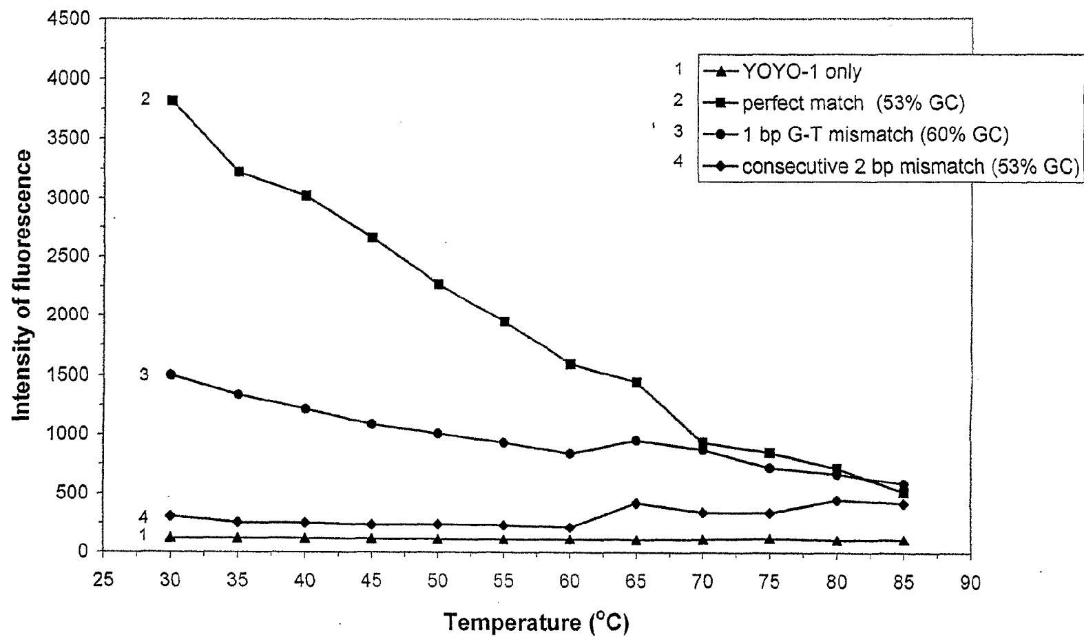
FIG. 2A. Binding of 15-mer antiparallel ssDNA to 50-mer dsDNA with YOYO-1 without prior denaturation of dsDNA
