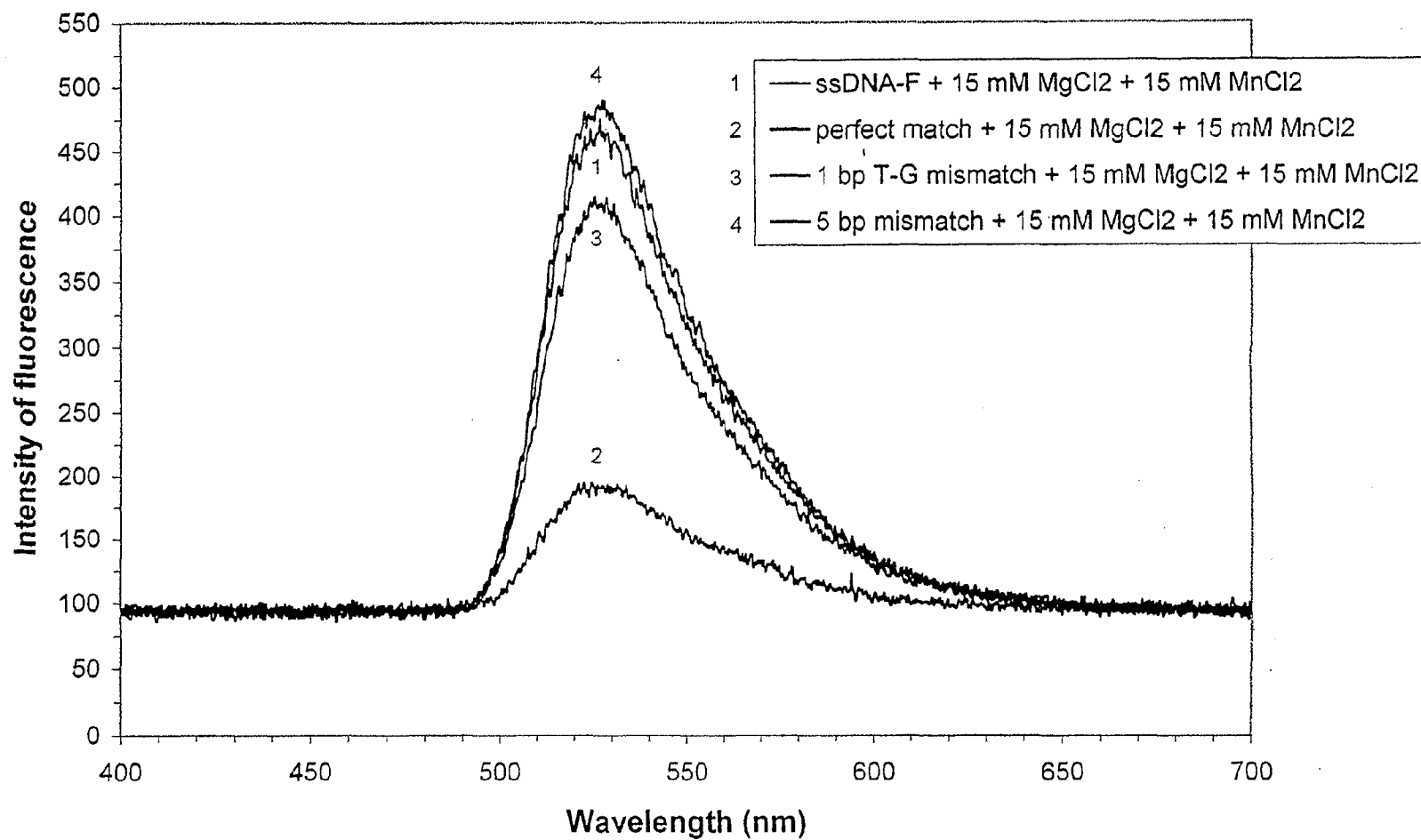
FIG. 5D. Binding of 15-mer antiparallel ssDNA-F probe (4 pmole) (53% GC) and 50-mer dsDNA (0.4 pmole) in the presence of divalent cations (after 1 hr)
