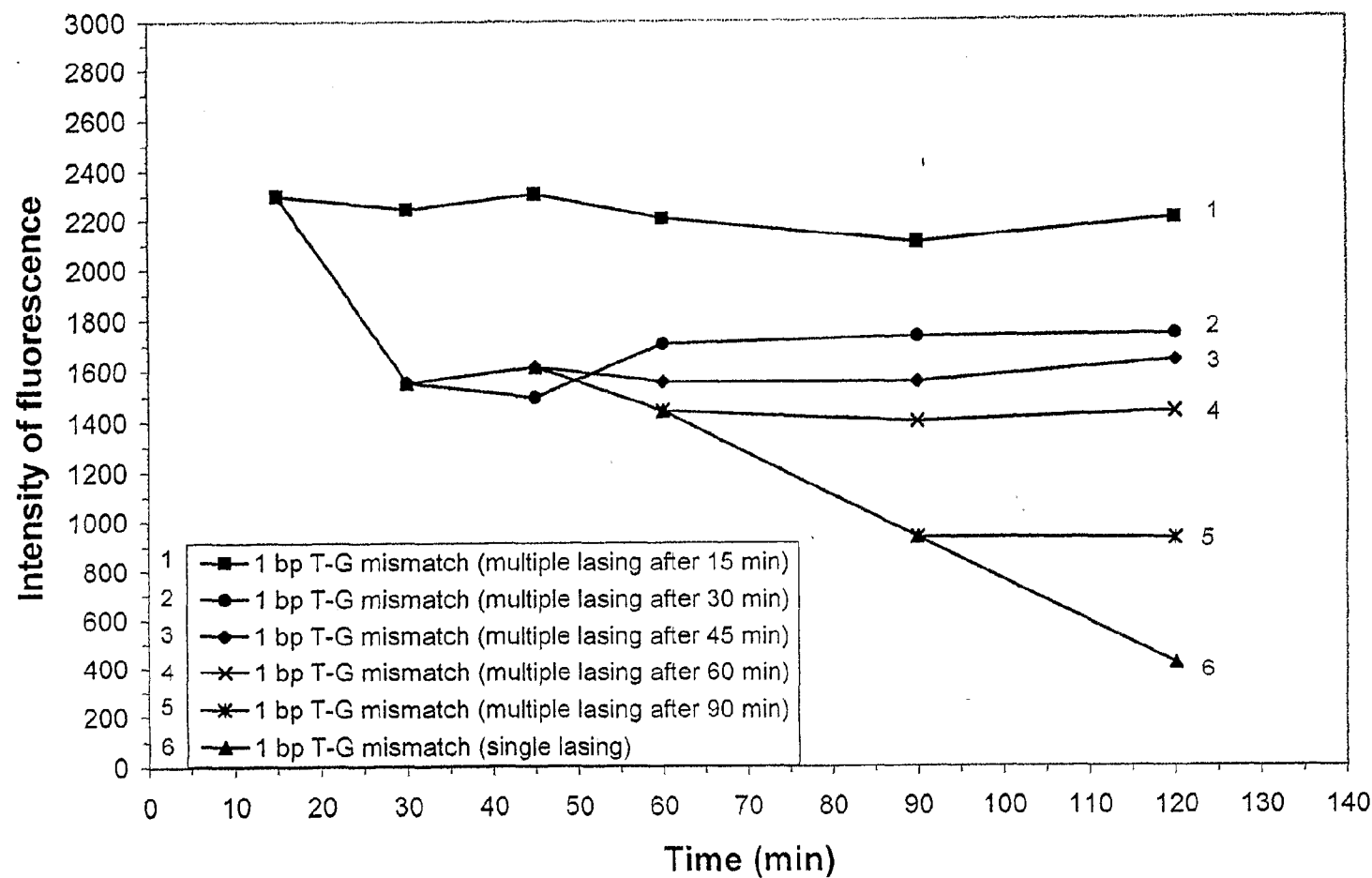
FIG. 6C. Effect of multiple laser treatment on complex formation between antiparallel 15-mer ssDNA-F (4 pmole) + 50-mer dsDNA (0.4 pmole) resulting in a 1 bp T-G mismatch in the presence of 10 mM MgCl 2 + 10 mM MnCl 2
