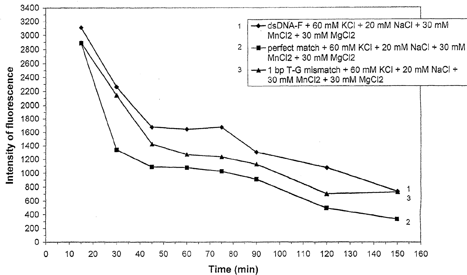
FIG. 9A. Binding of 15-mer dsDNA-F (4 pmole) (53% GC) and 50-mer dsDNA (0.4 pmole) in the presence of monovalent and divalent cations over time
