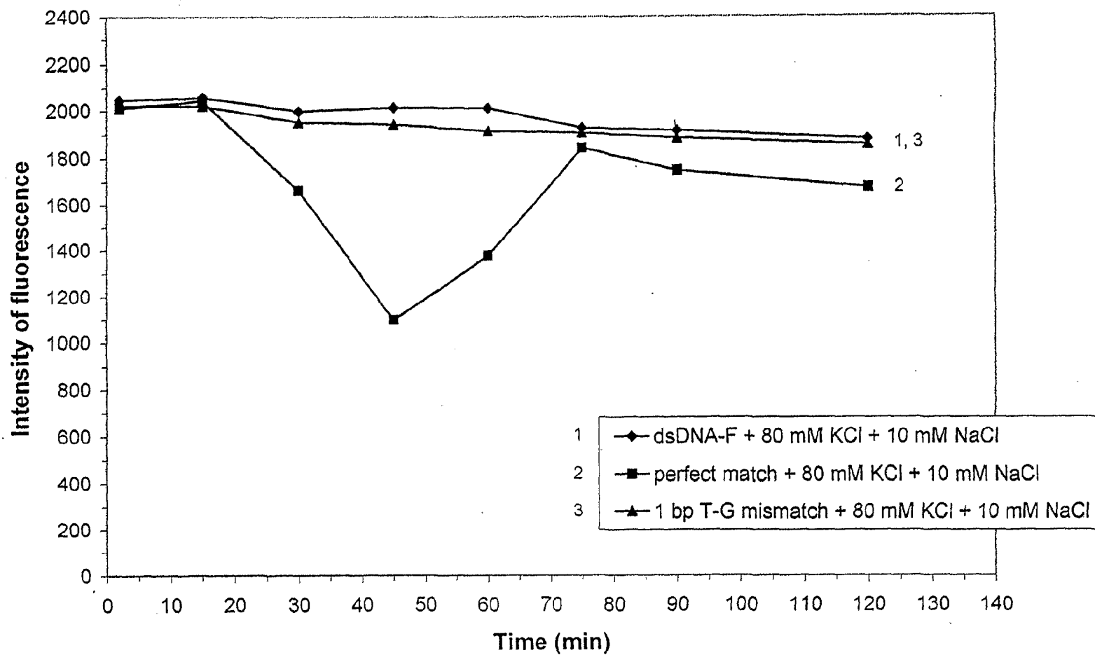
FIG. 7C. Binding of 15-mer dsDNA-F (4 pmole) (53% GC) and 50-mer dsDNA (0.4 pmole) in the presence of 80 mM KCl + 10 mM NaCl over time
