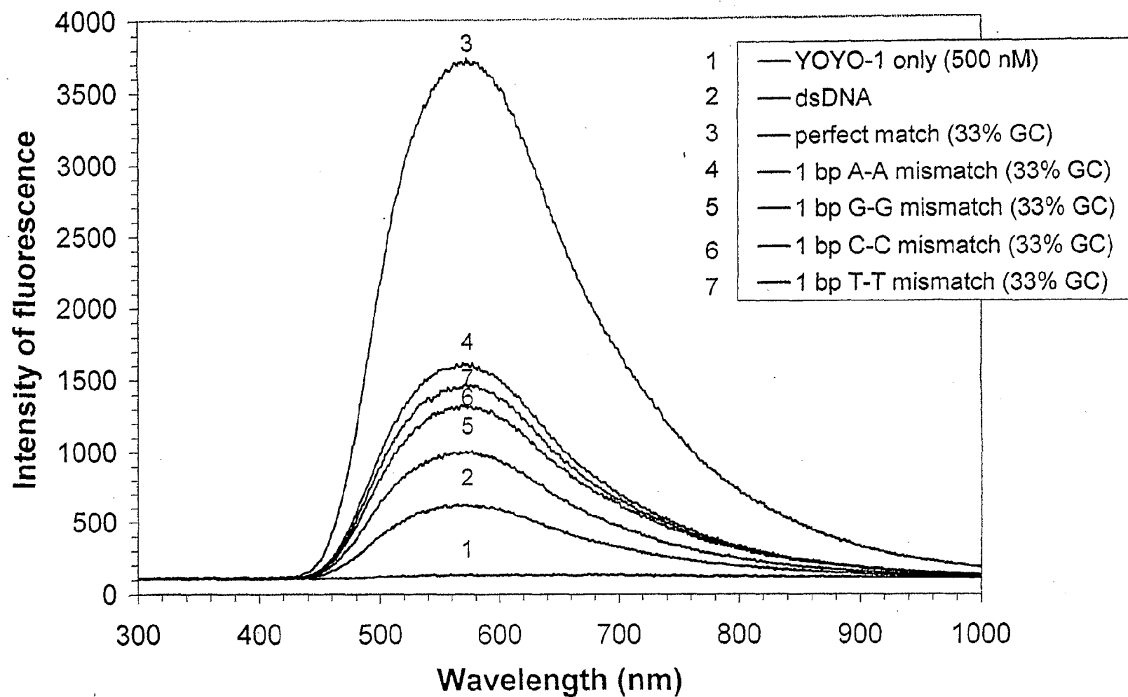
FIG. 12C. Binding of 15-mer sense ssDNA to 50-mer dsDNA with YOYO-1
