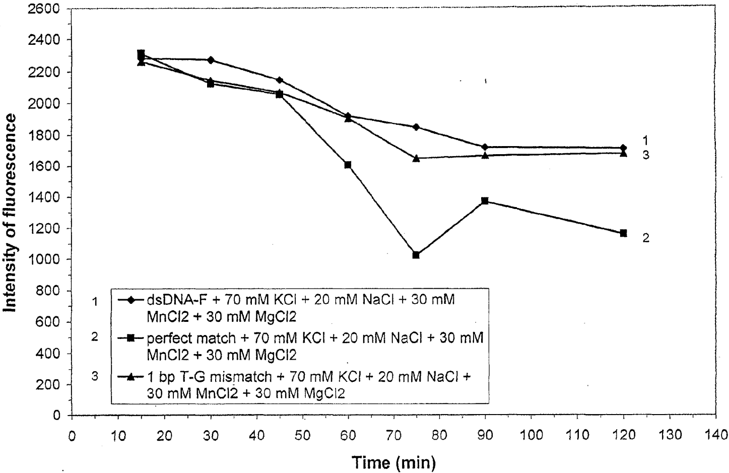
FIG. 9B. Binding of 15-mer dsDNA-F (4 pmole) (53% GC) and 50-mer dsDNA (0.4 pmole) in the presence of monovalent and divalent cations over time
