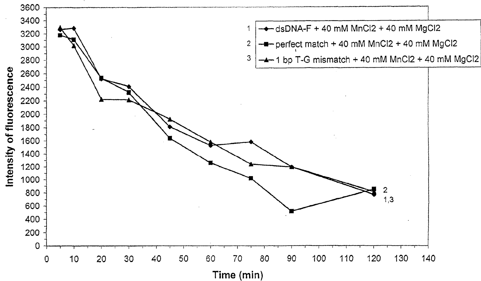
FIG. 8B. Binding of 15-mer dsDNA-F (4 pmole) (53% GC) and 50-mer dsDNA (0.4 pmole) in the presence of 40 mM \text{MnCl}_2 + 40 mM \text{MgCl}_2 over time
