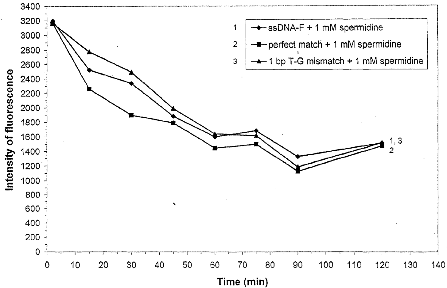
FIG. 10. Binding of 15-mer antiparallel ssDNA-F (2 pmole) (53% GC) and 50-mer dsDNA (0.2 pmole) in the presence of 1 mM spermidine over time
