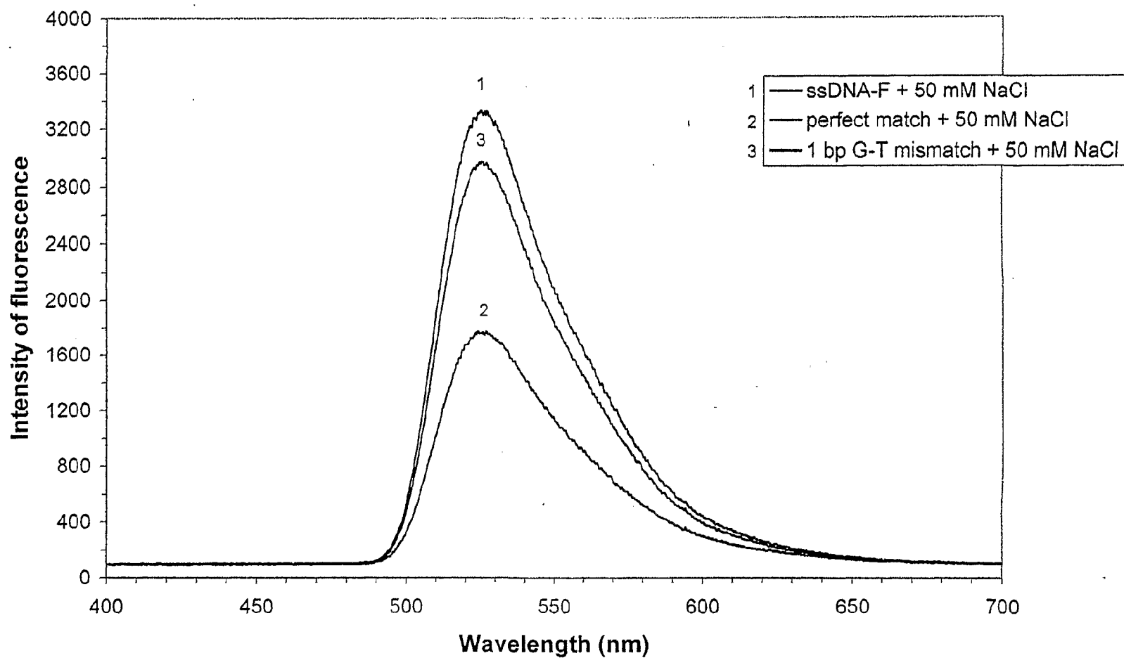
FIG. 3. Binding of 15-mer antiparallel ssDNA-F probe (4 pmole) (33% GC) and 50-mer dsDNA (0.4 pmole) in the presence of 50 mM NaCl (after 1 hr)
