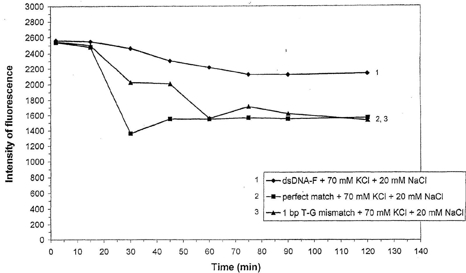
FIG. 7B. Binding of 15-mer dsDNA-F (4 pmole) (53% GC) and 50-mer dsDNA (0.4 pmole) in the presence of 70 mM KCl + 20 mM NaCl over time
