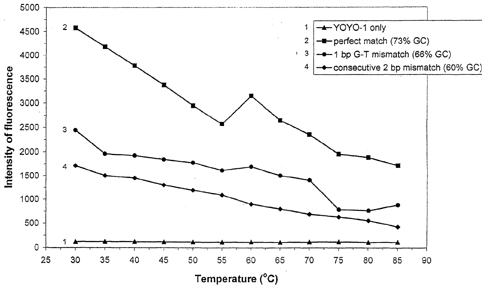
FIG. 2B. Binding of 15-mer antiparallel ssDNA to 50-mer dsDNA with YOYO-1 without prior denaturation of dsDNA
