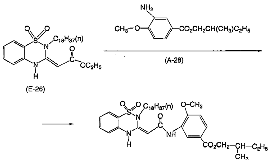
Exemplified compound (C-28)
