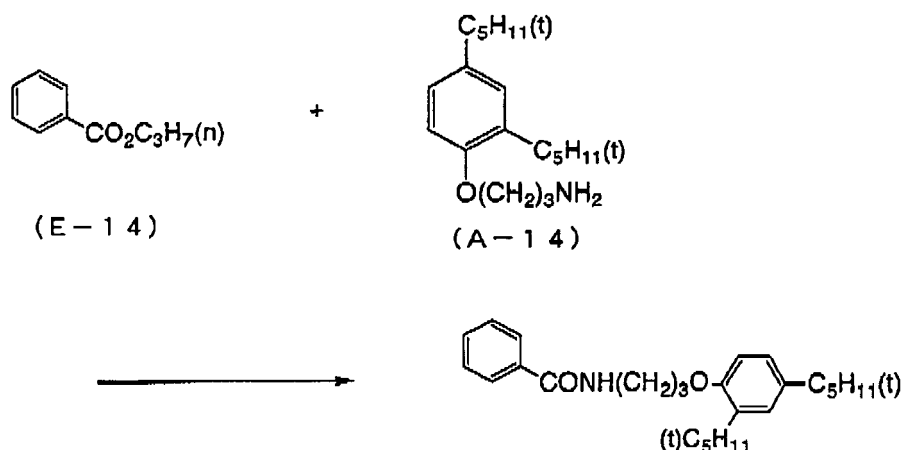
Exemplified compound (C-14)
