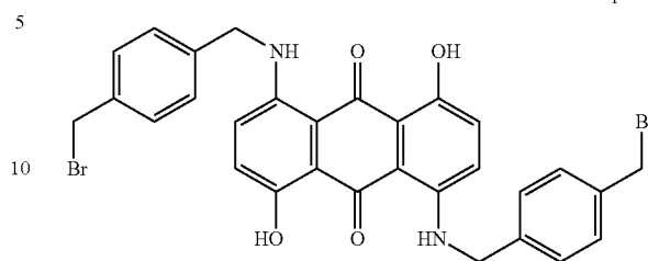
Compound 1
