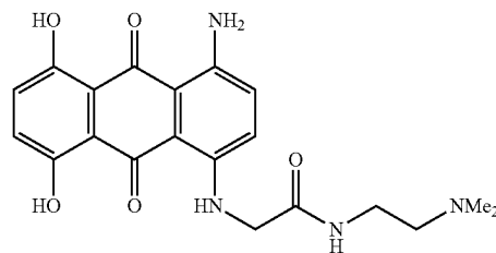
Compound 20
