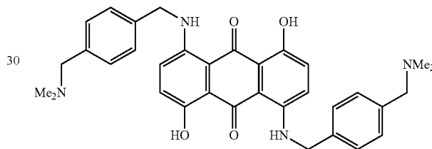
Compound 2
