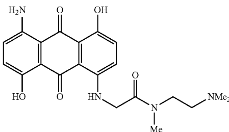
Compound 18
