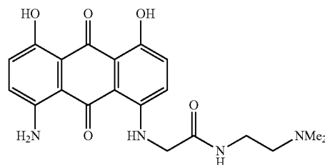
Compound 19
