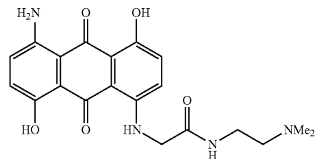
Compound 9
