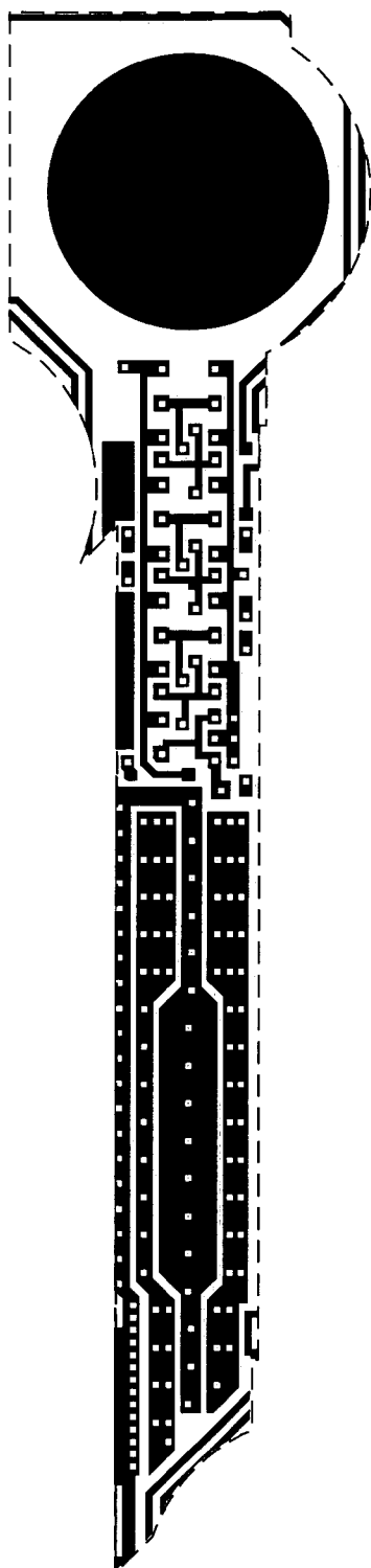
Metal 1 mask
