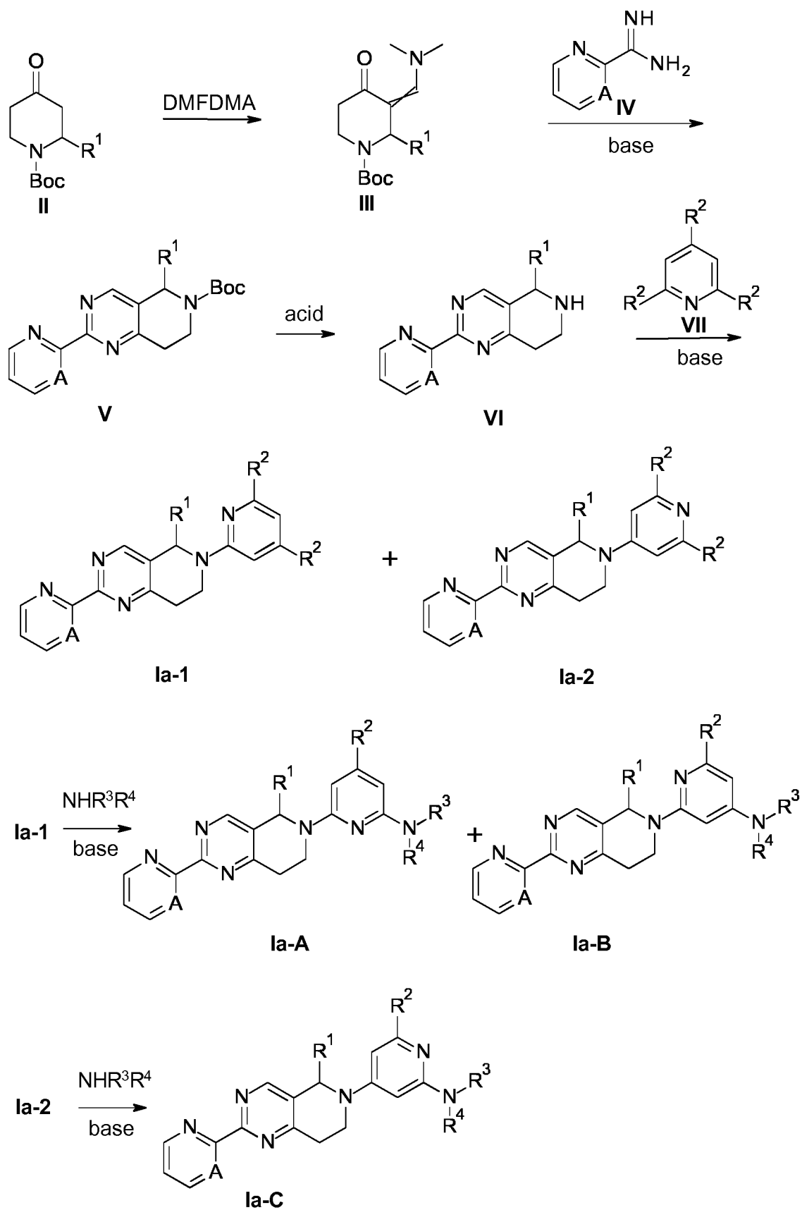
Scheme 1
