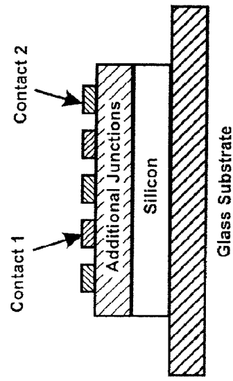
2. Single-Crystal Silicon (Longitudinal Backside Contacts)
