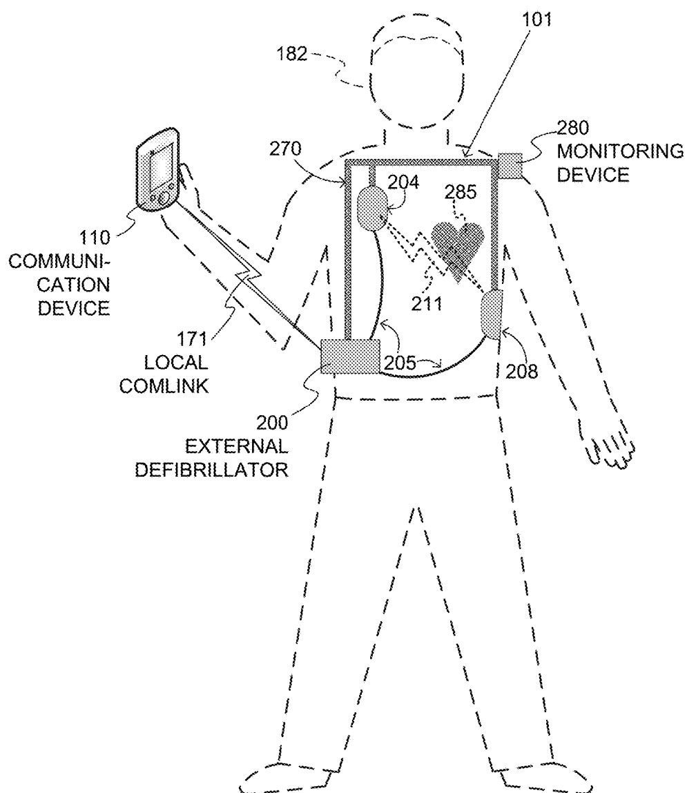
WEARABLE DEFIBRILLATOR SYSTEM & MOBILE COMMUNICATION DEVICE
