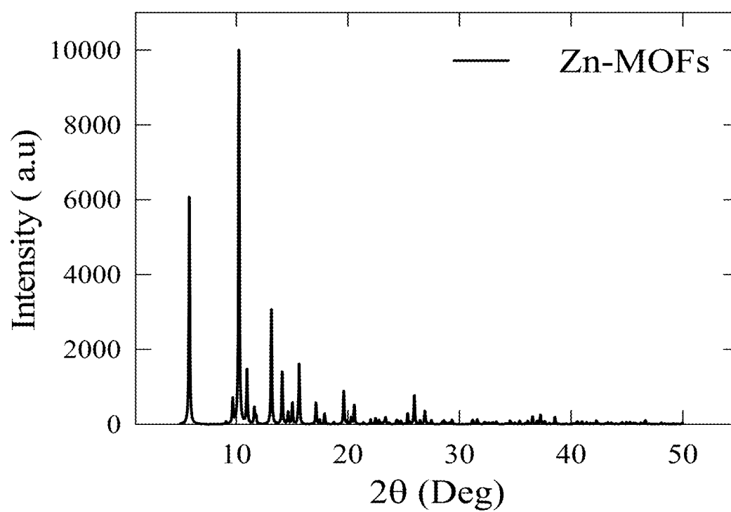
Fig. 5. XRD pattern of Zn-MOFs
