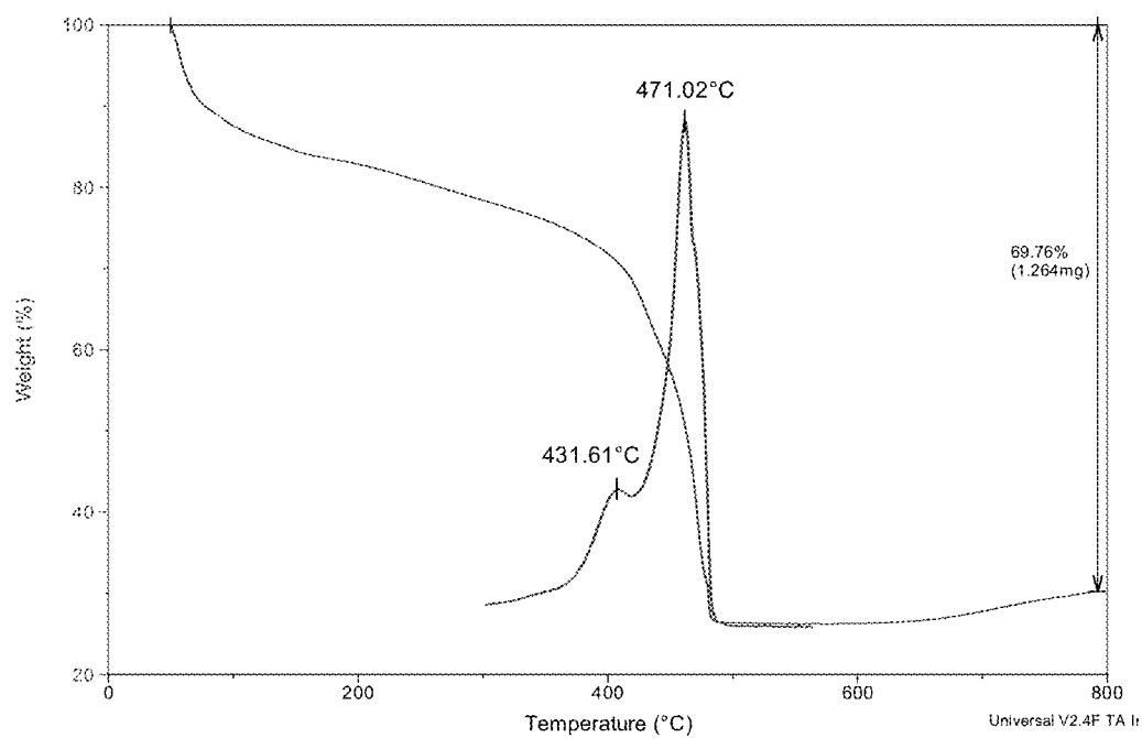
Fig. 6: TGA curve of Zn-MOFs
