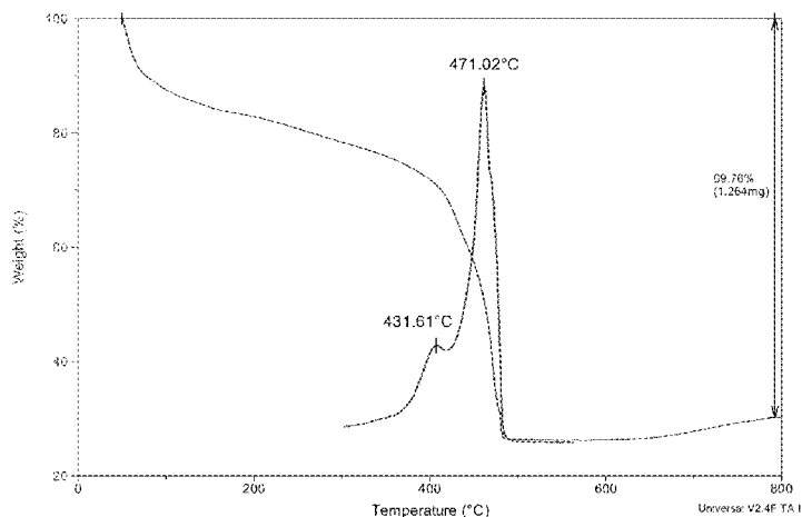
TGA curve of Zn-MOFs
