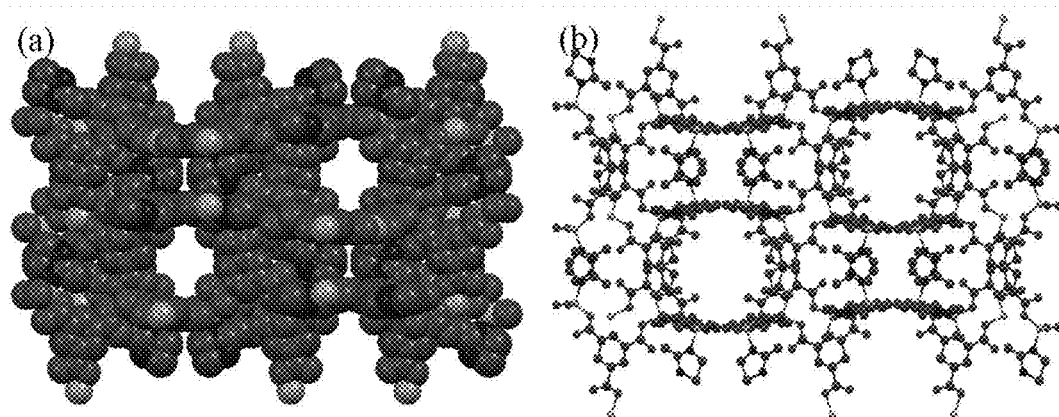
Figure 3: Packing diagram of Zn-MOFs
