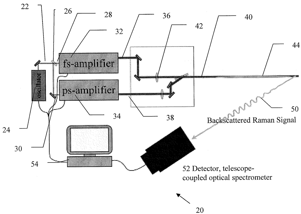
FIG. 1 – Experimental Apparatus
