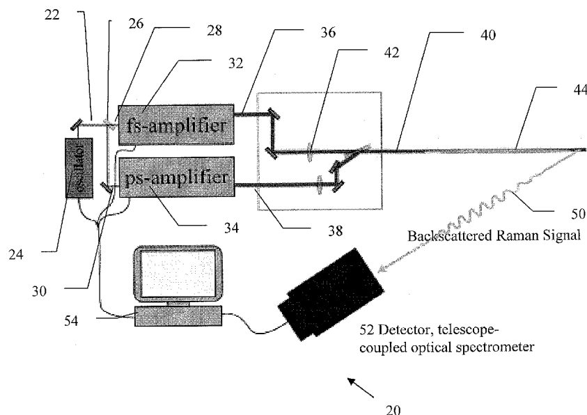
FIG. 1 – Experimental Apparatus
