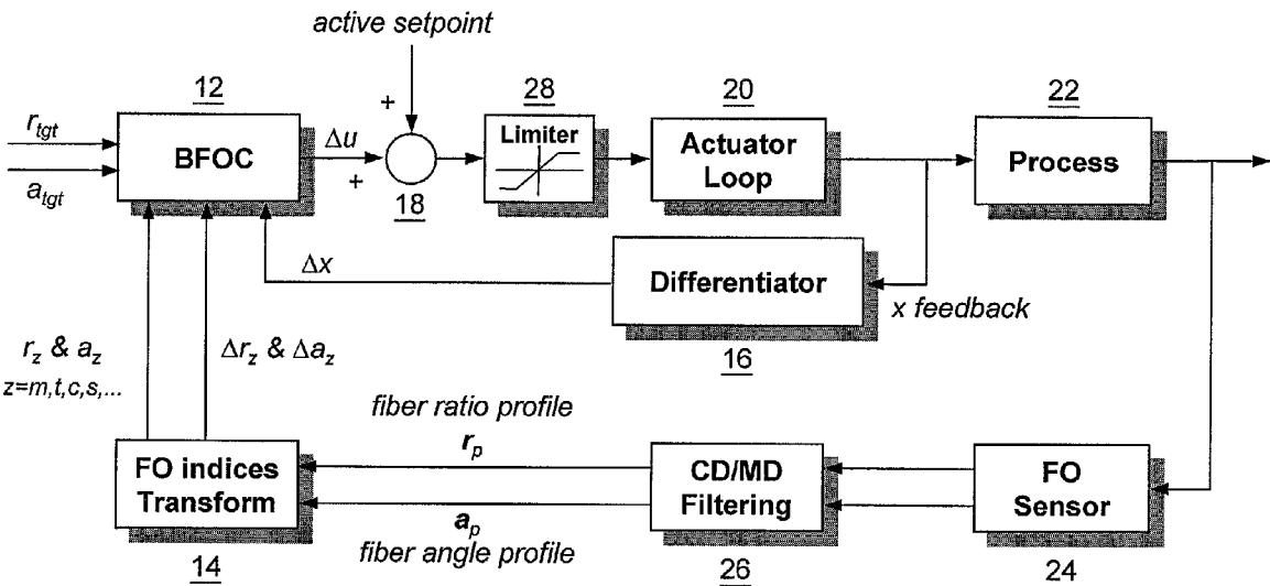
Block diagram of base FO control (BFOC) system (10)
