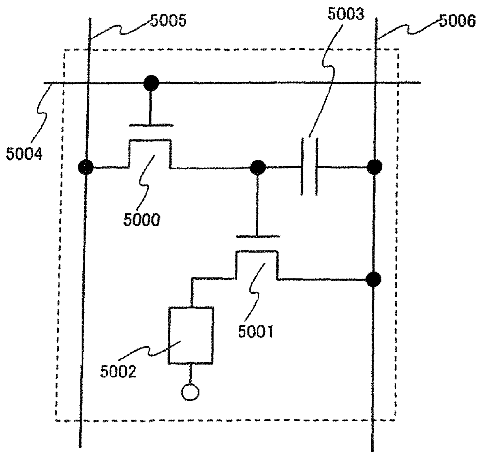
Fig. 18 PRIOR ART
