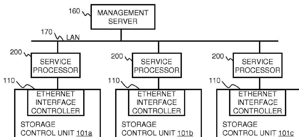
FIG. 2 Service Processor Arrangement
