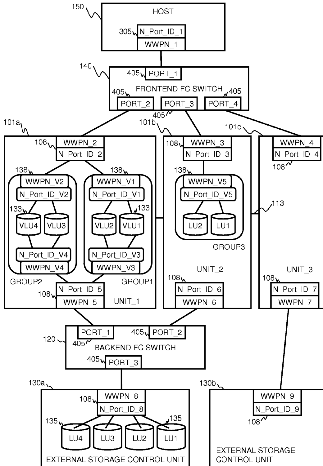
FIG. 13 Explanatory Drawing of Port and Volume Configuration
