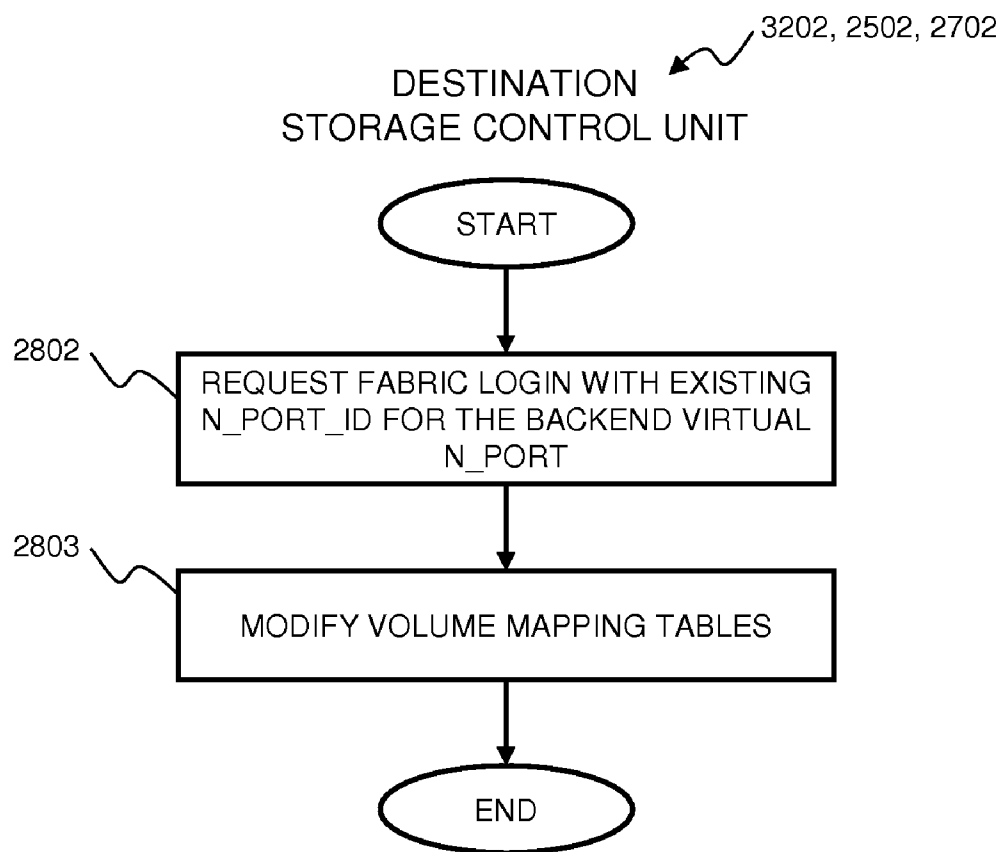
FIG. 26 Flowchart of Backend Virtual N_Port Transfer
