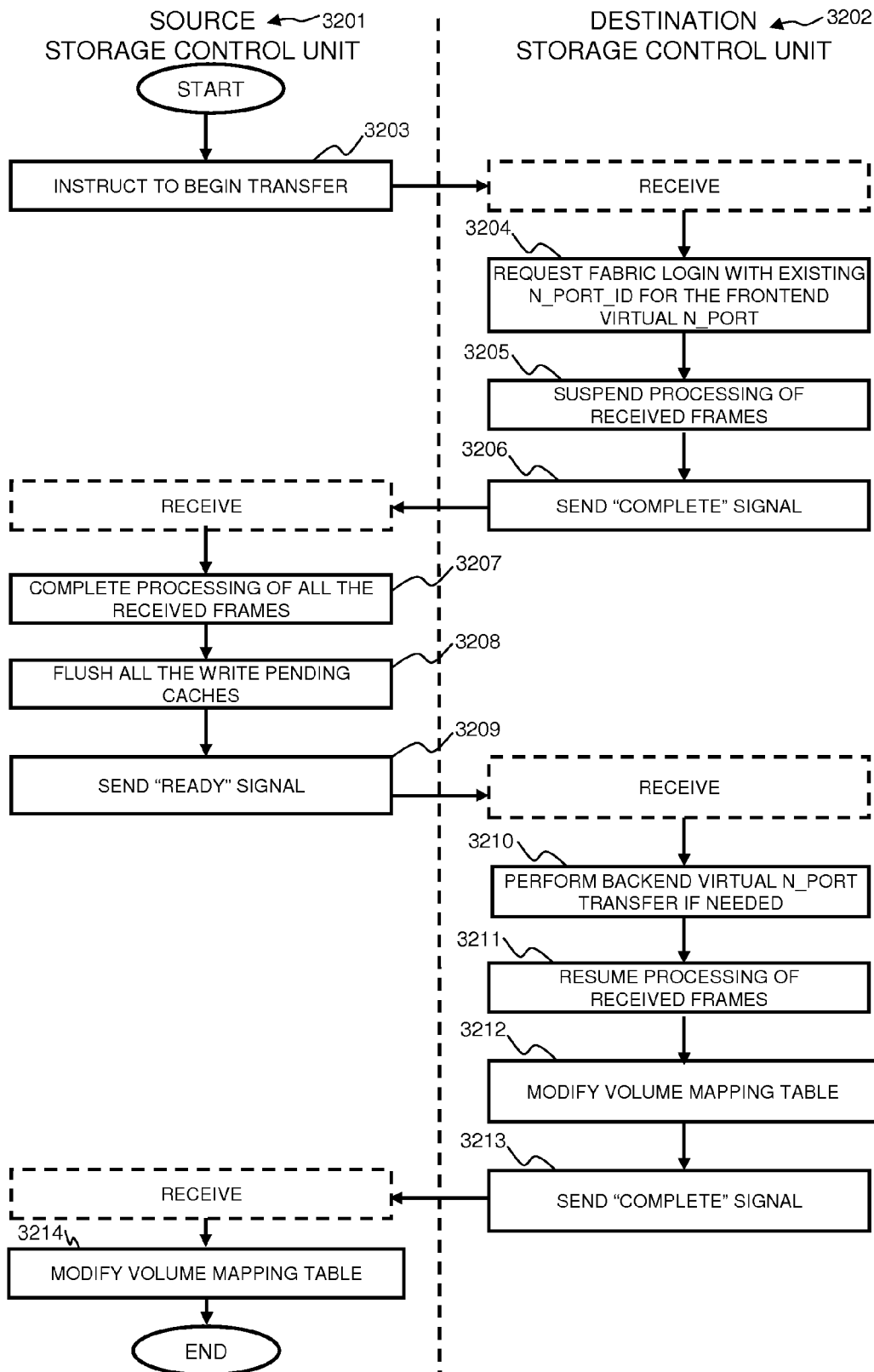
FIG. 24A Flowchart of Frontend Virtual N_Port Transfer
