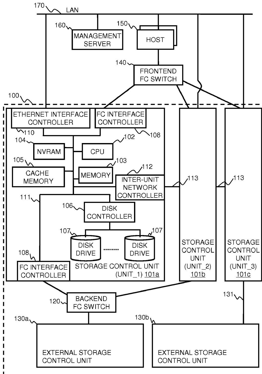
FIG. 1 System Configuration
