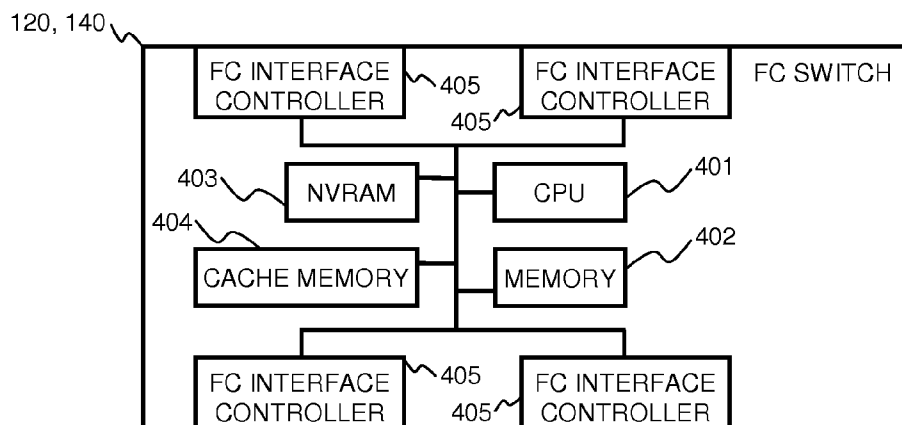
FIG. 4 Configuration of FC Switch
