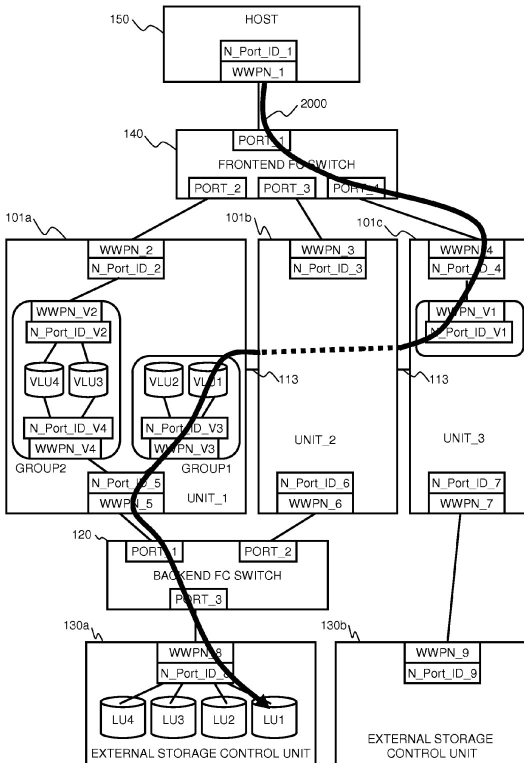
FIG. 19 Volume Accessing Path In Case That Only Frontend Virtual N_Port is Transferred to Another Unit
