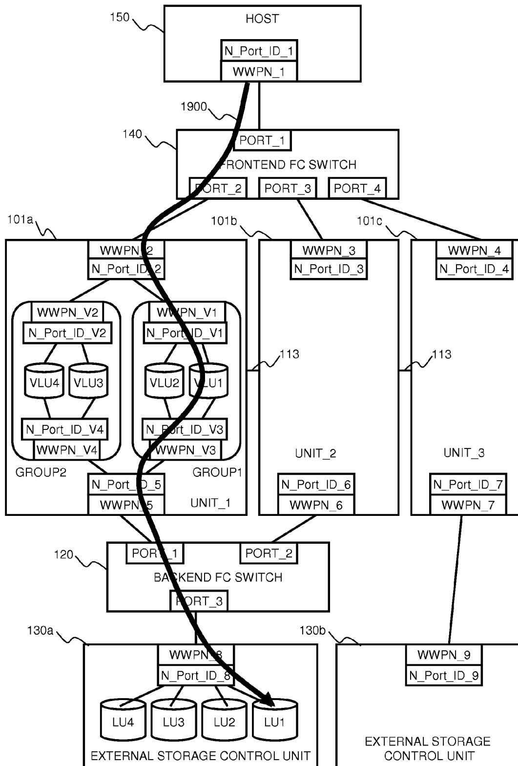
FIG. 18 Volume Accessing Path Before Port Transfer
