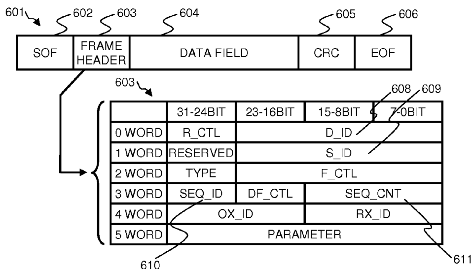
FIG. 6 Structure of a Frame (Related Art)
