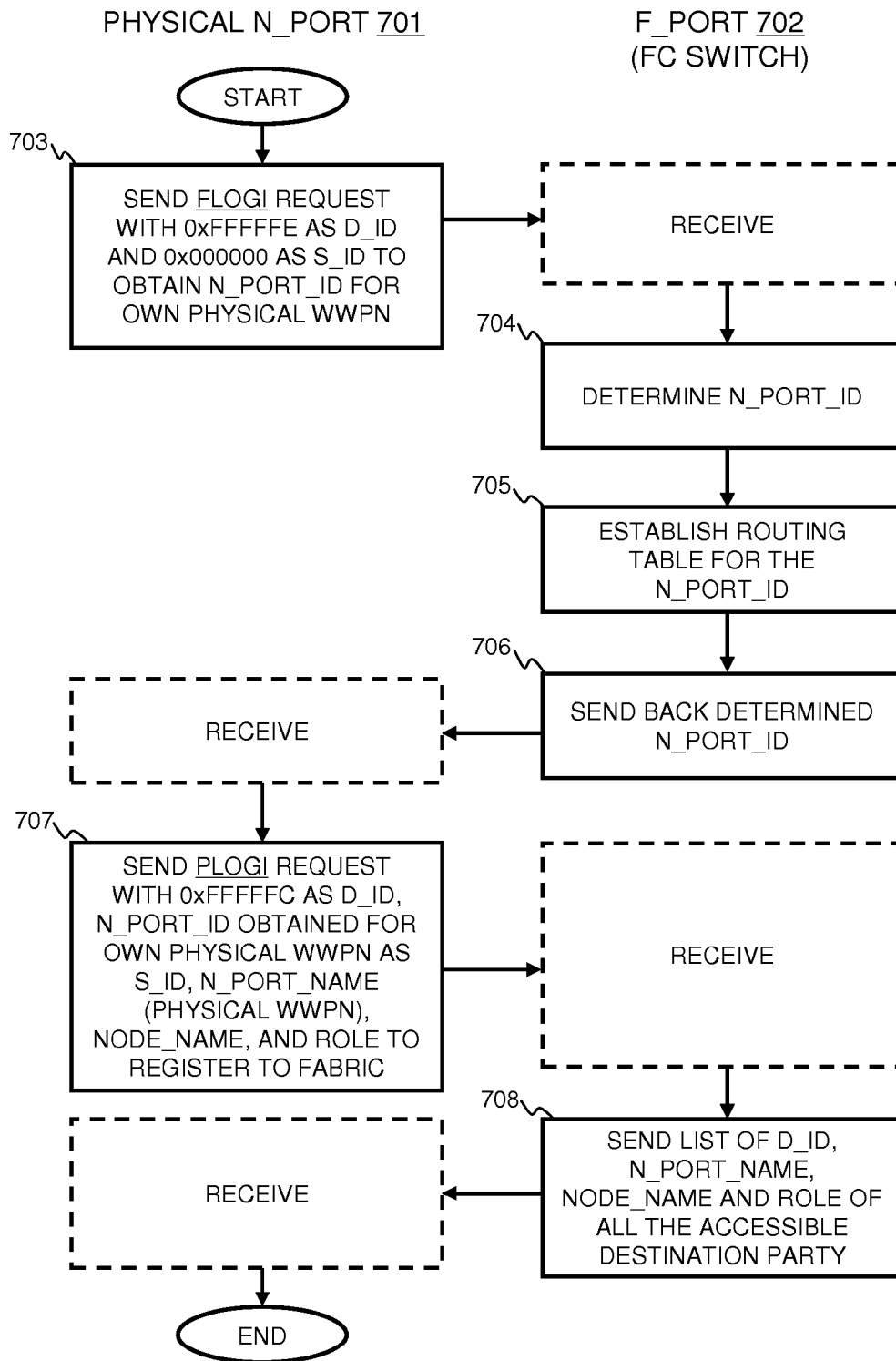
FIG. 7 Fabric Login Procedure for Physical N_Port (Related Art)
