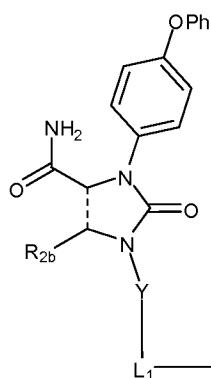
(IIIa)
