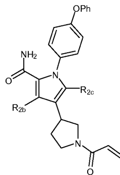
(XVd)
