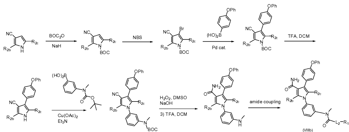
Scheme 6
