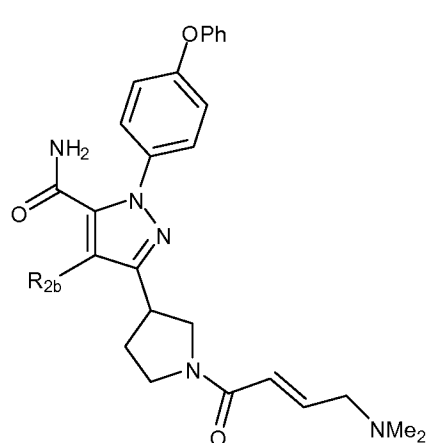
(XVIIIc)
