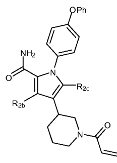
(XVI d)
