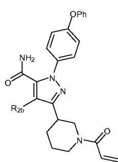
(XVIc)
