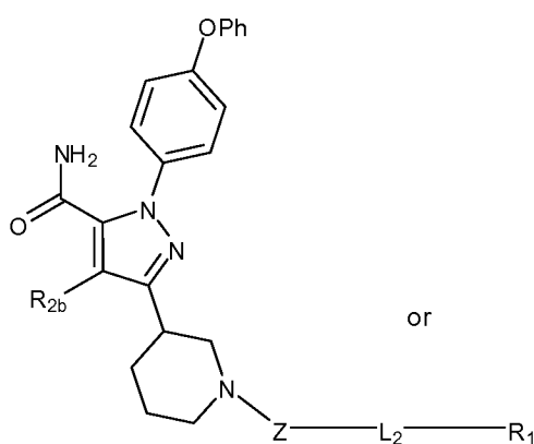
(Vc)
