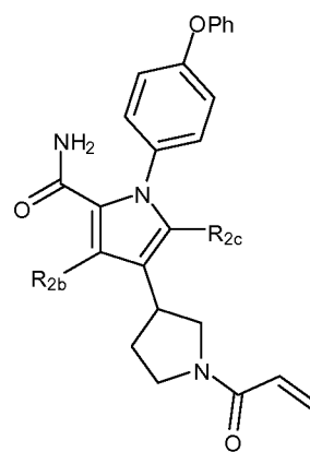
(XVd)
