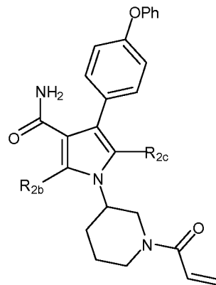
(XVIb)
