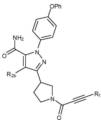
(XIIc)
