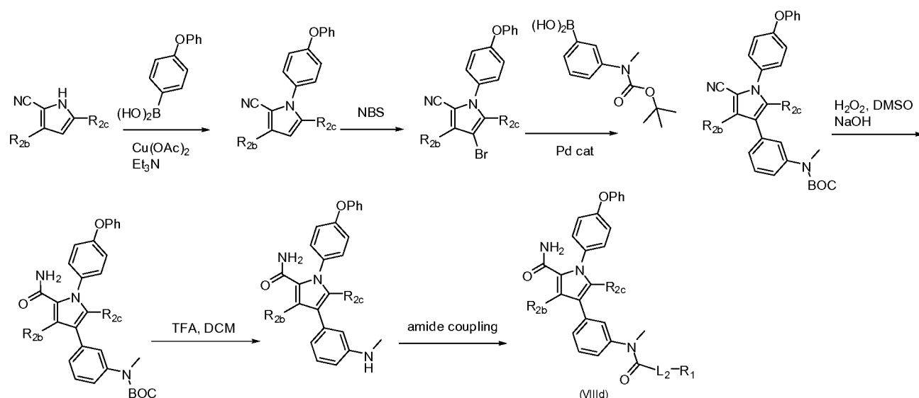
Scheme 8
