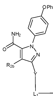
(IIIc)
