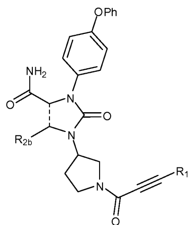
(XIIa)
