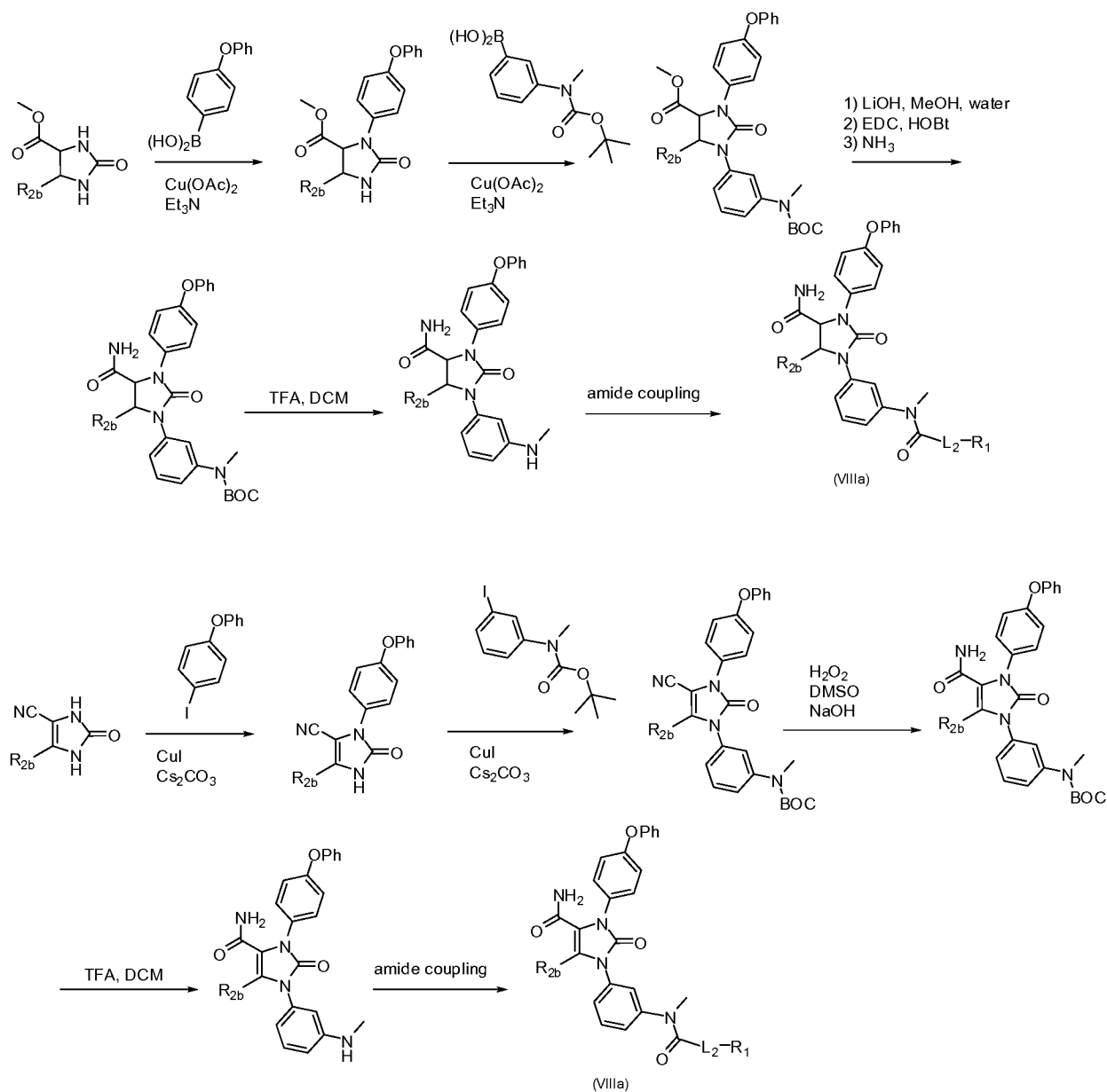
Scheme 5
