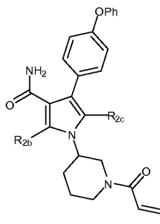
(XVIb)
