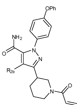
(XVIc)
