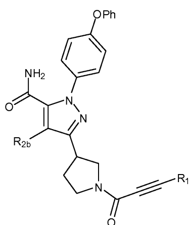
(XIIc)
