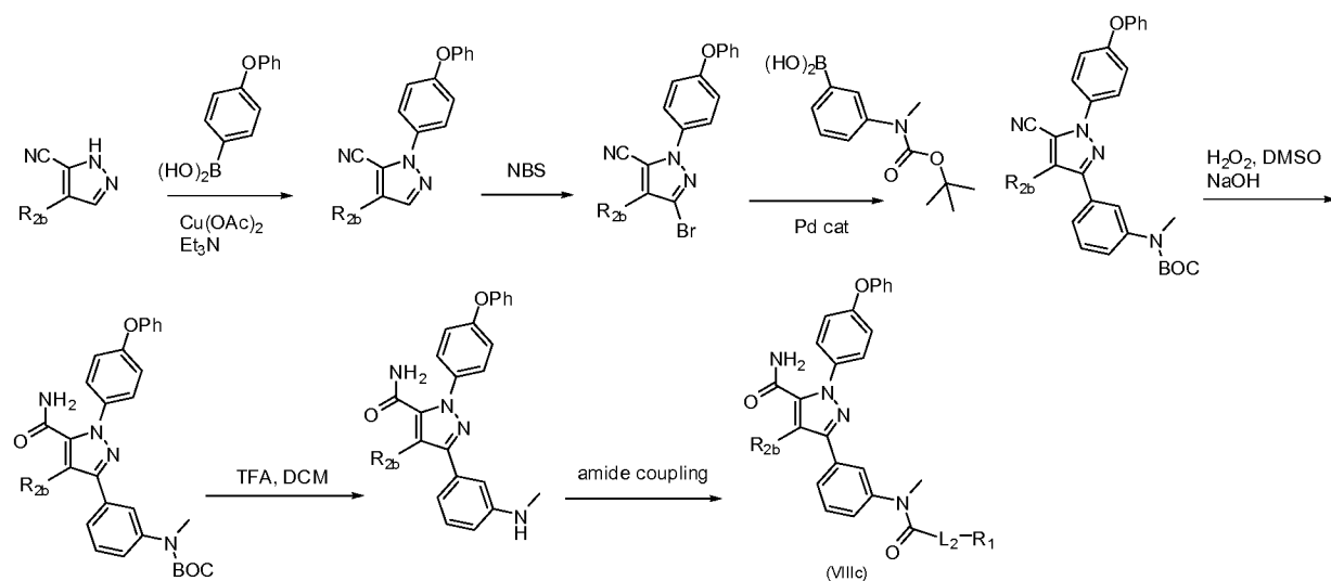
Scheme 7
