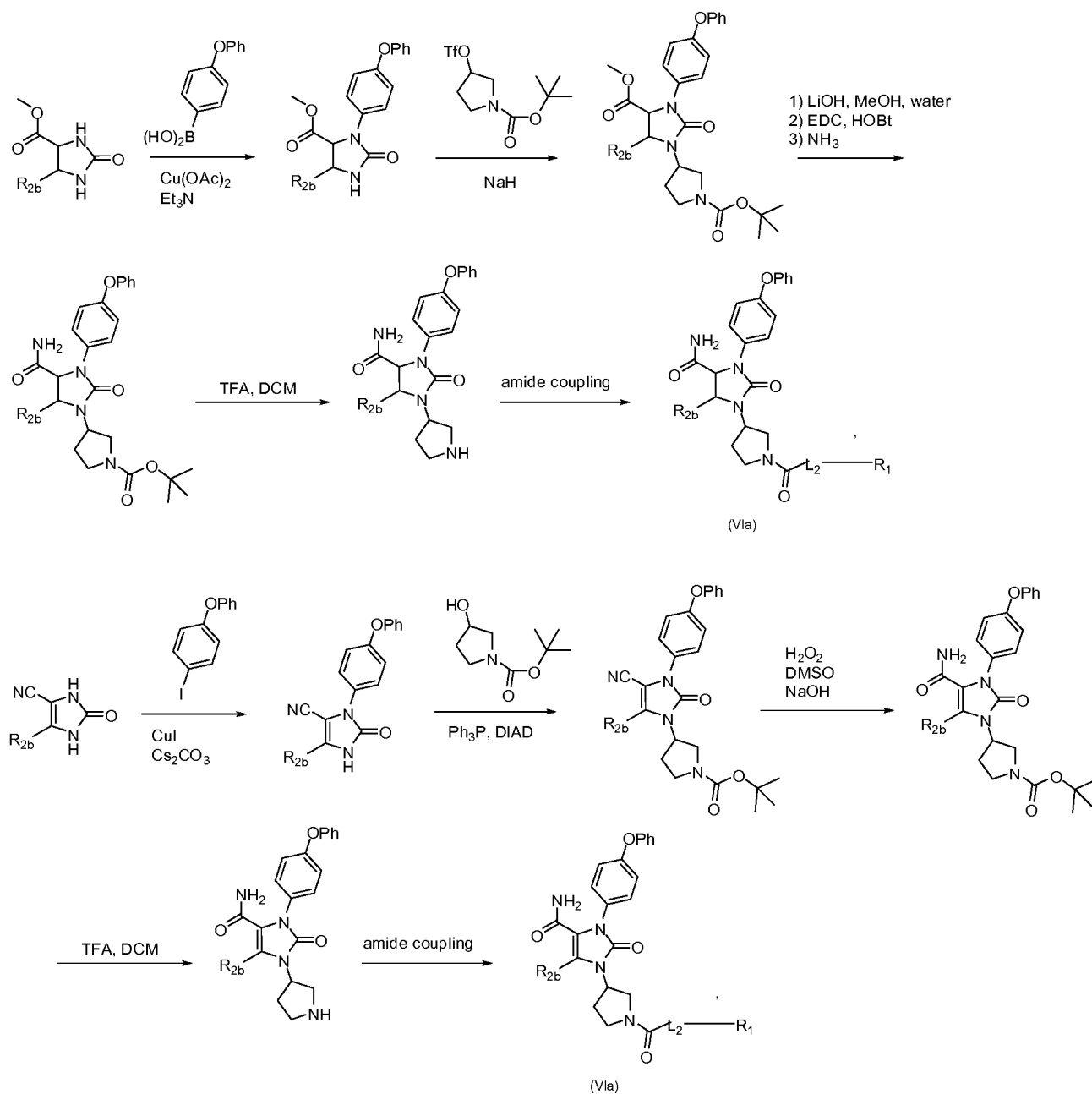
Scheme 1
