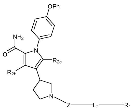
(IVd)
