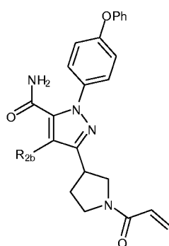
(XVc)
