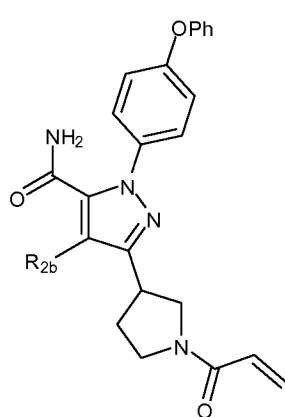
(XVc)
