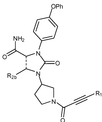
(XIIa)
