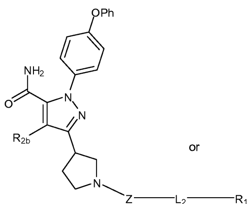
(IVc)
