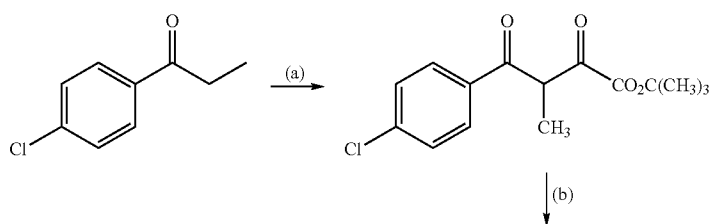
Scheme 8
