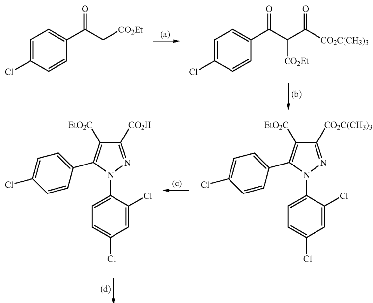
Scheme 11
