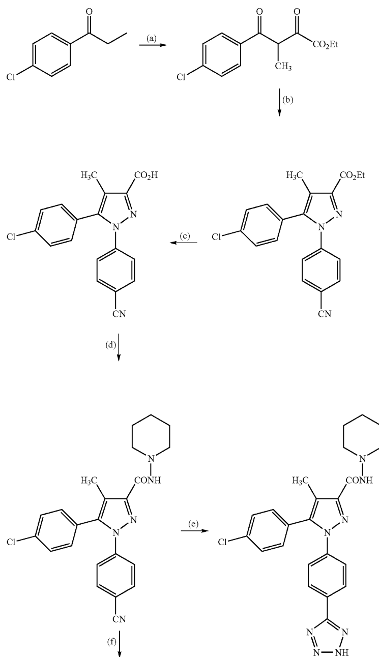
Scheme 10
