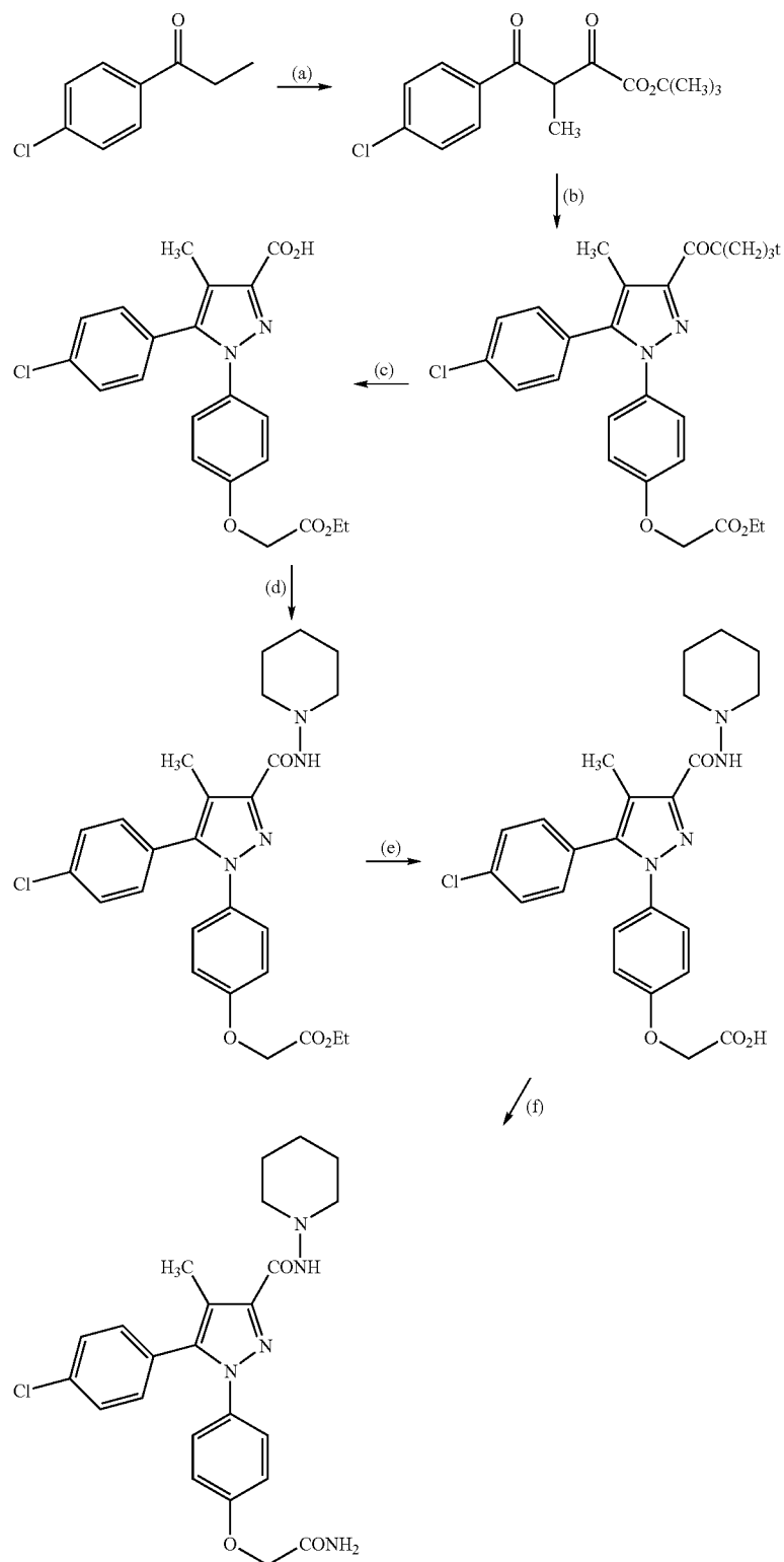
Scheme 9
