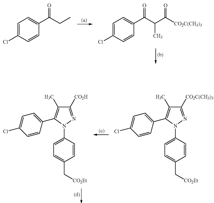
Scheme 7
