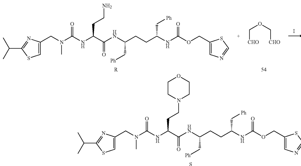
Scheme 21
