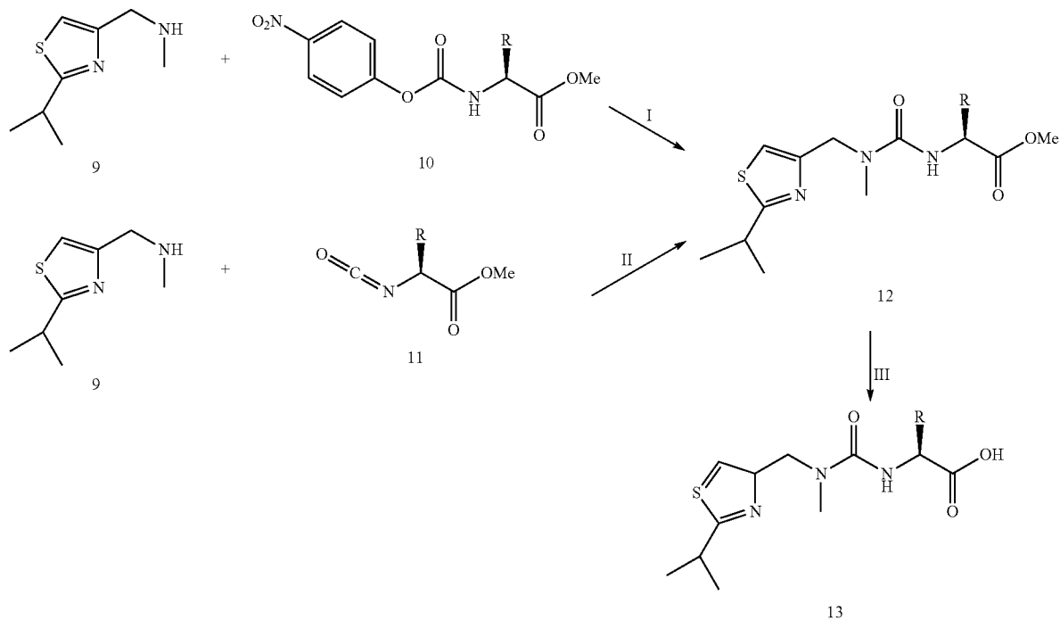
Scheme 6
