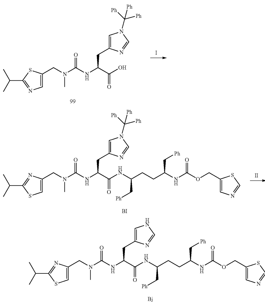
Scheme 49
