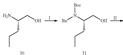
Scheme 14
