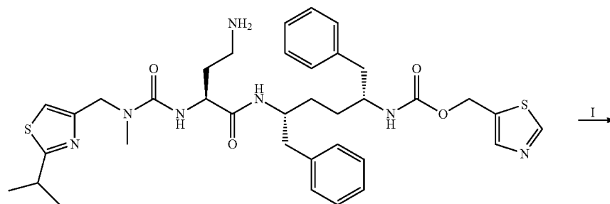
Scheme 66
