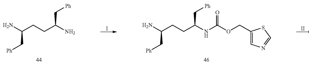
Scheme 76
