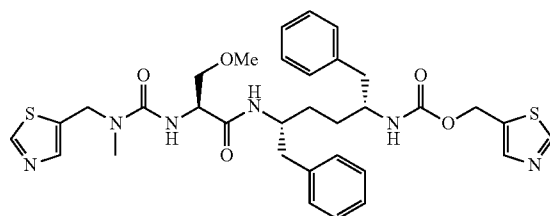
Scheme 68
