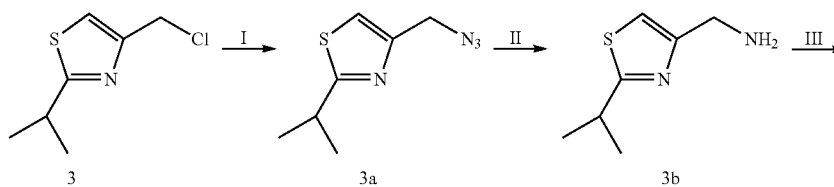
Scheme 10
