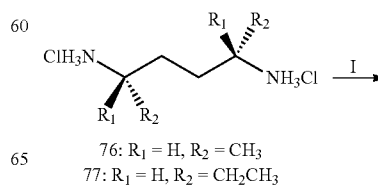
Scheme 32
