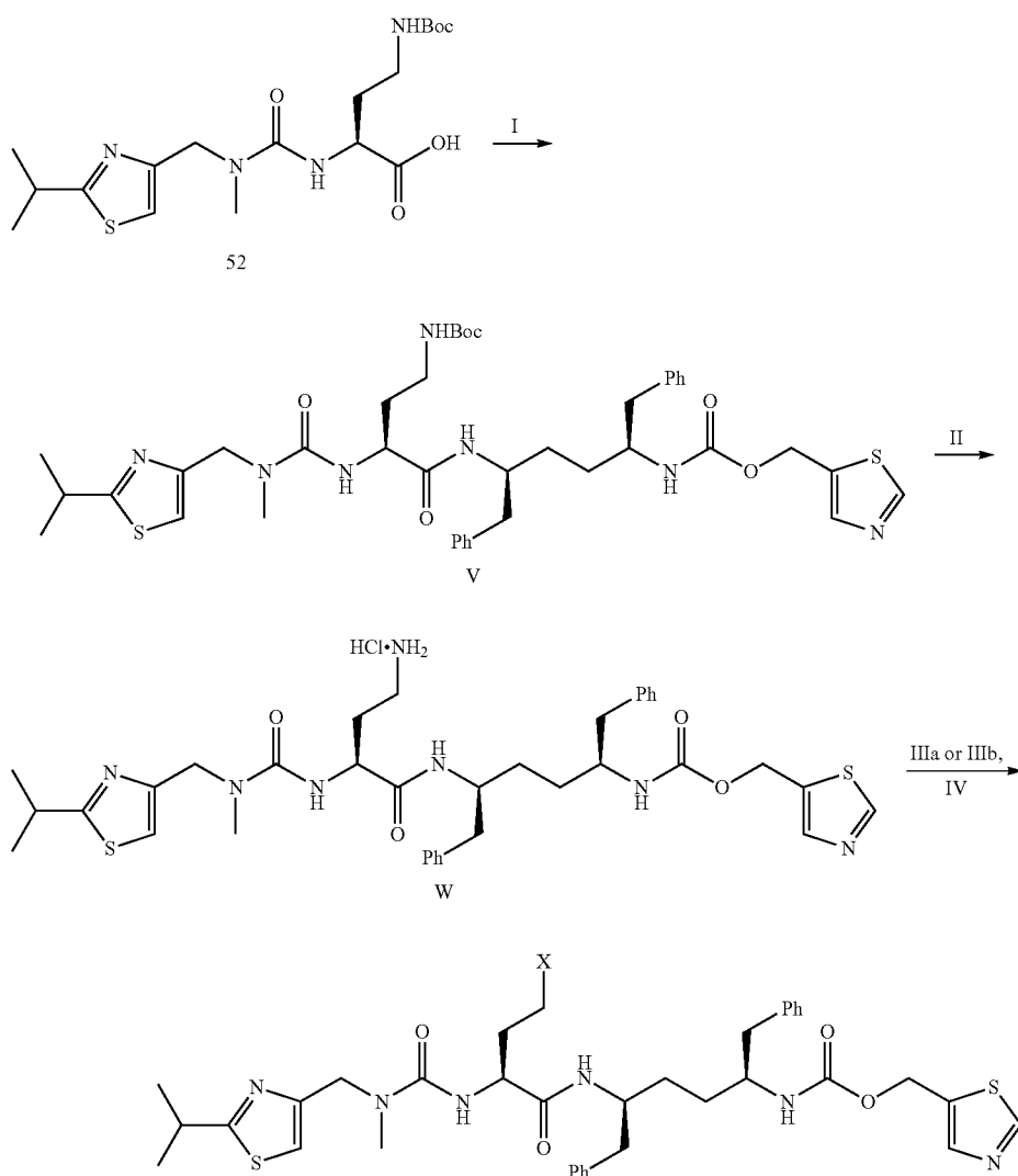
Scheme 25
