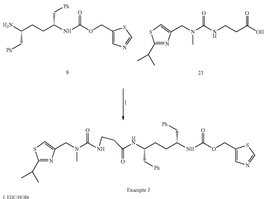
Scheme 9
