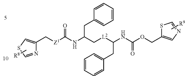
Formula IB
