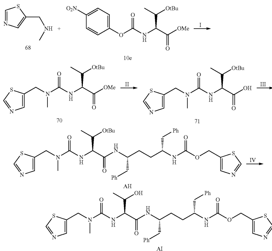
Scheme 29
