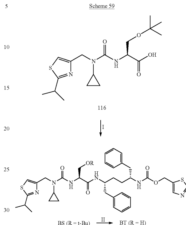
Scheme 59
