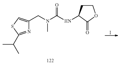
Scheme 23
