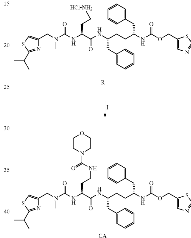
Scheme 63
