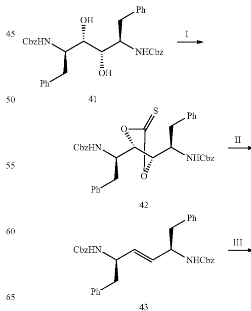
Scheme 16
