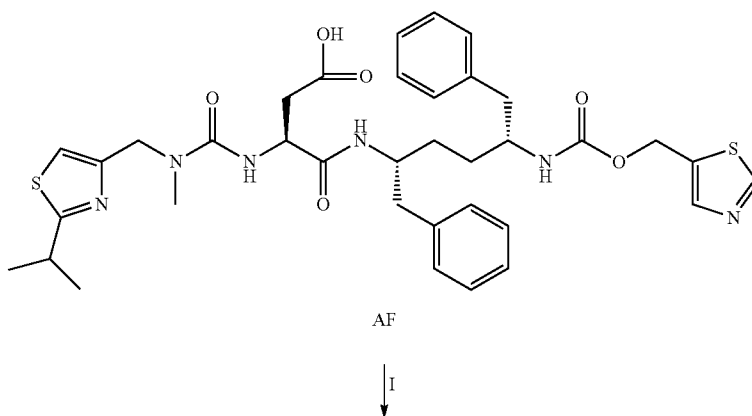
Scheme 65
