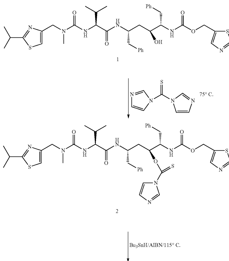
Scheme 1
