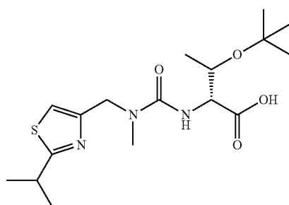
Scheme 57
