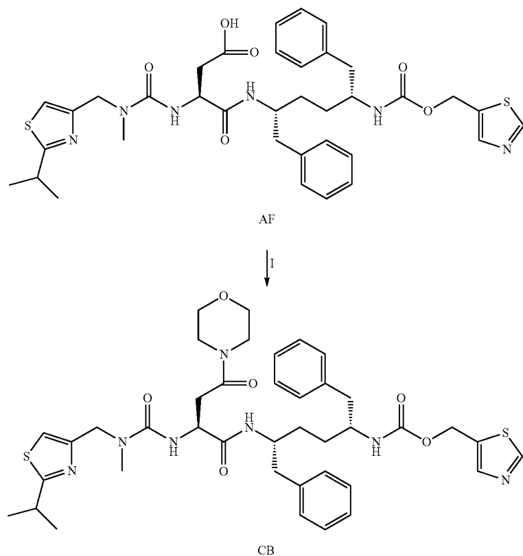
Scheme 64
