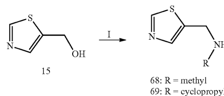
Scheme 28
