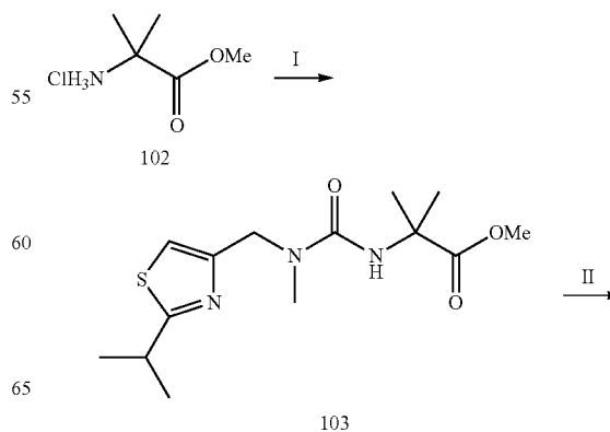
Scheme 50
