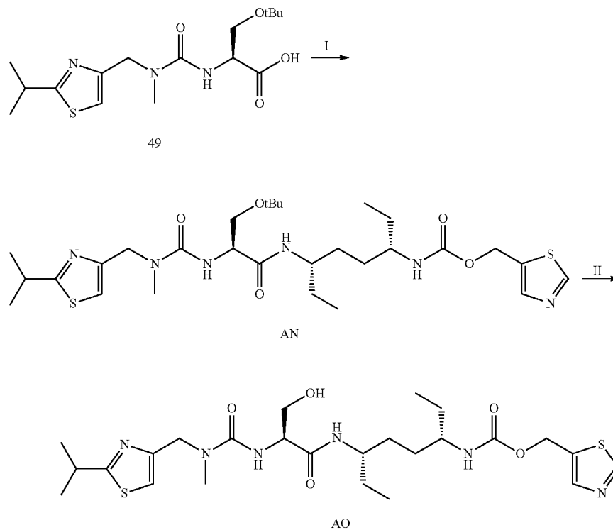
Scheme 33
