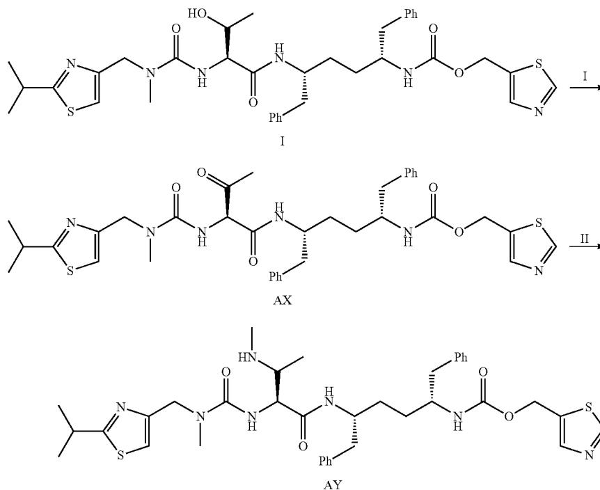
Scheme 41
