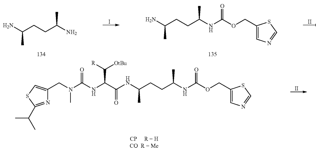
Scheme 77
