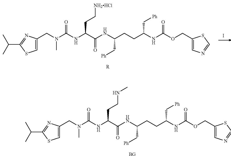
Scheme 47
