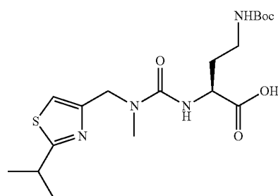
Scheme 58
