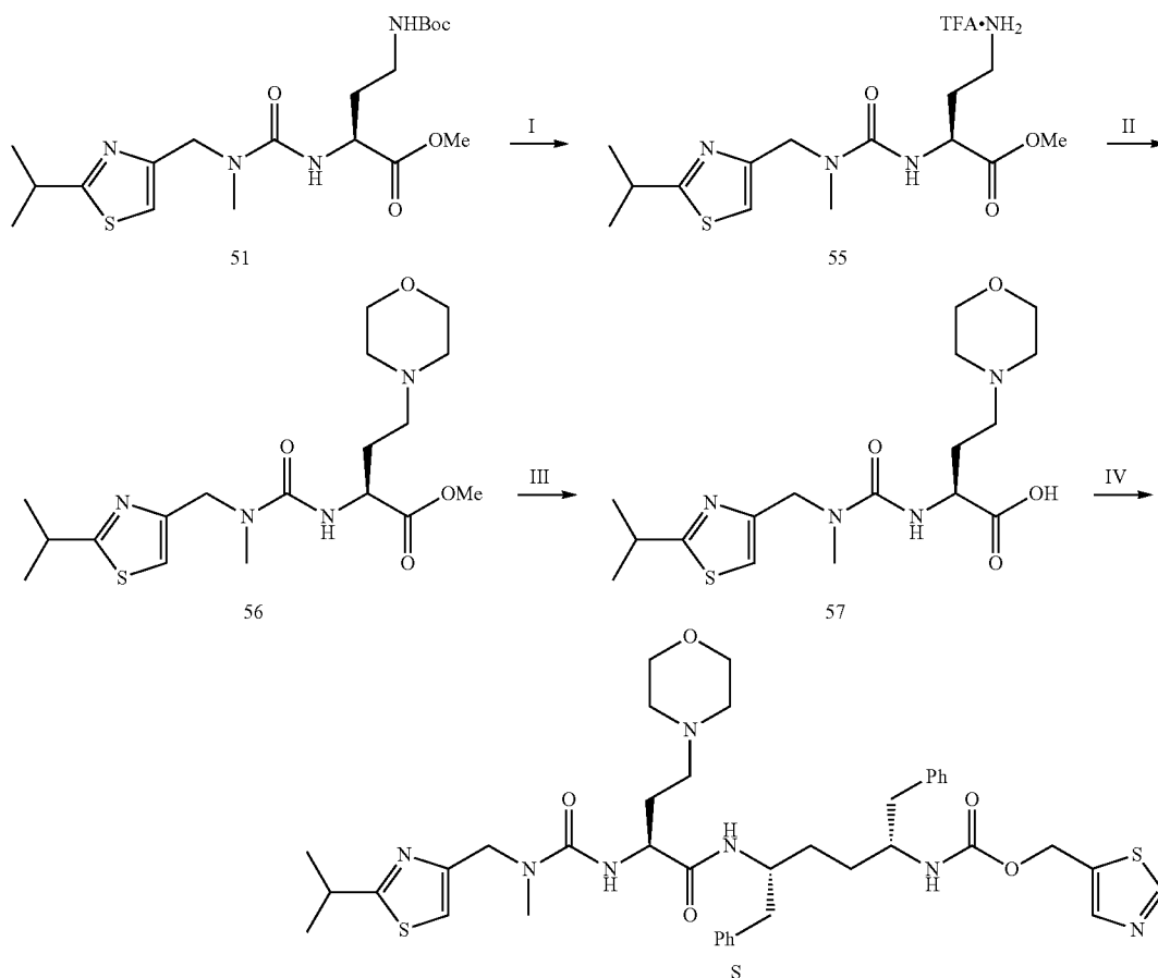
Scheme 22
