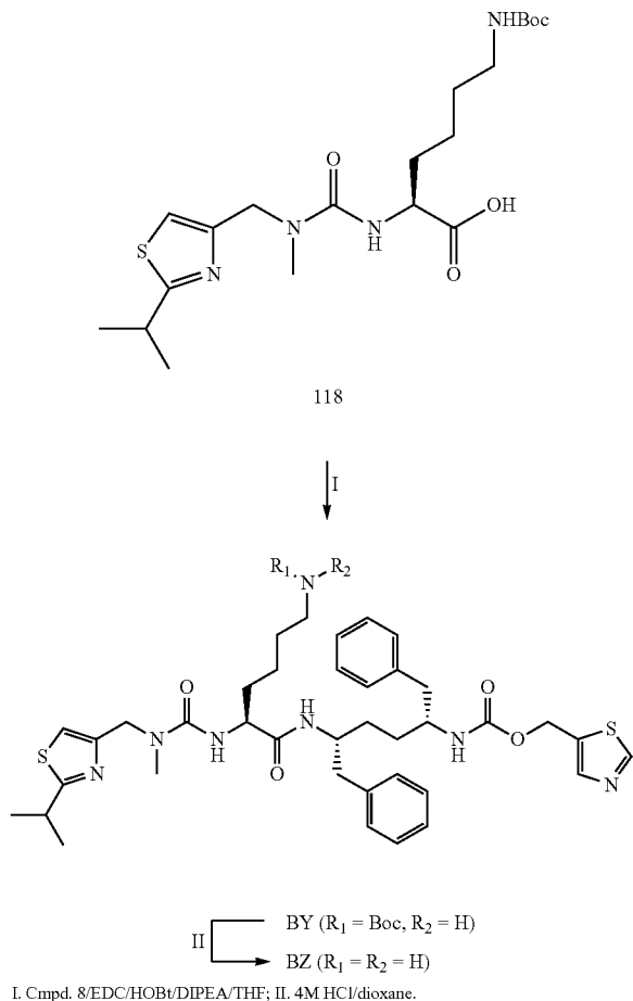
Scheme 62
