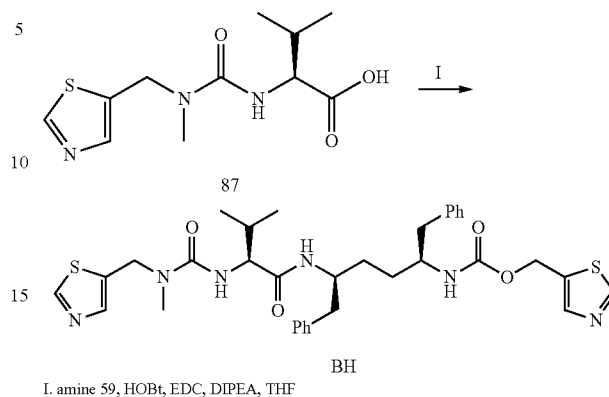
Scheme 48
