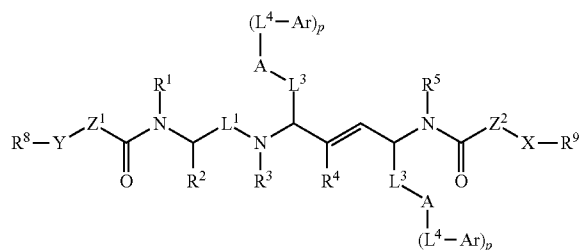
Formula IID
