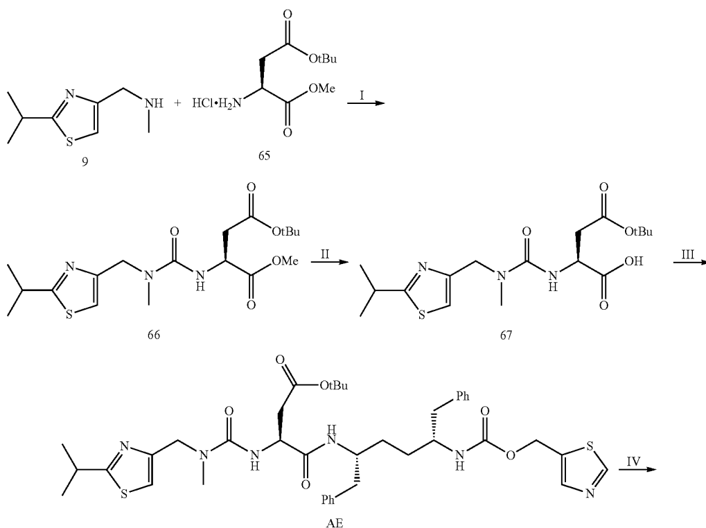
Scheme 27
