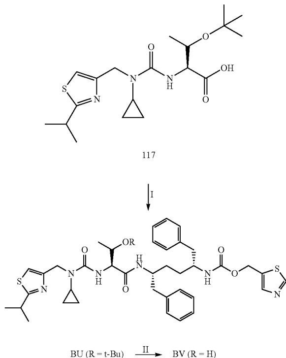
Scheme 60
