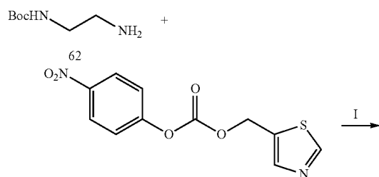
Scheme 26
