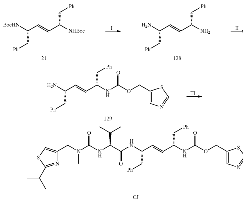
Scheme 73
