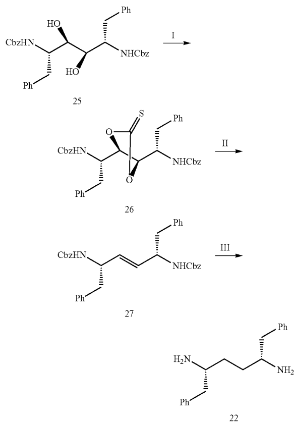
Scheme 12
