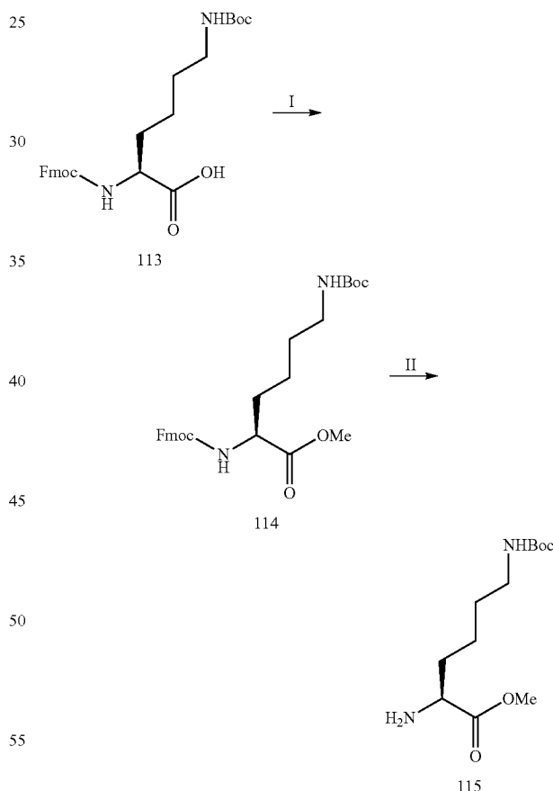
Scheme 53
