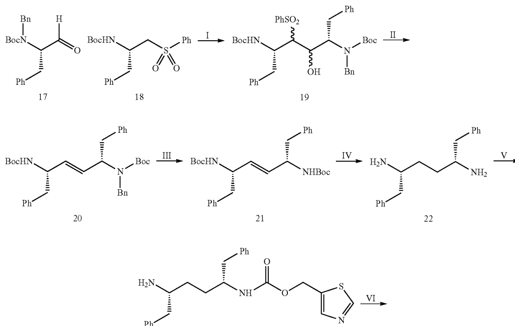
Scheme 8
