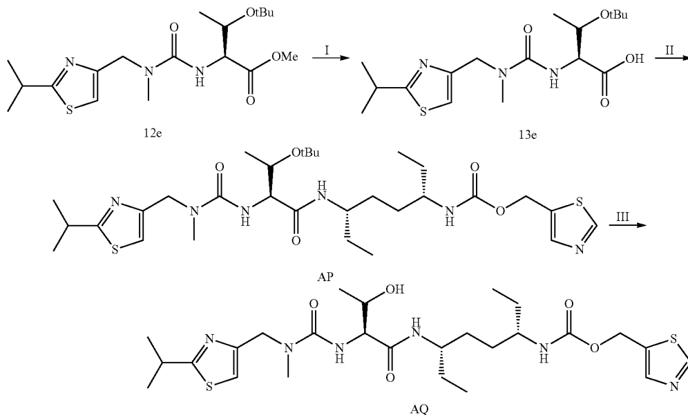
Scheme 34
