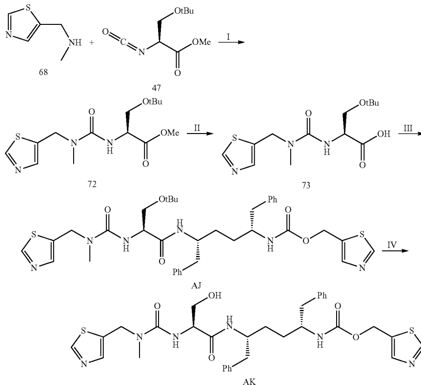
Scheme 30
