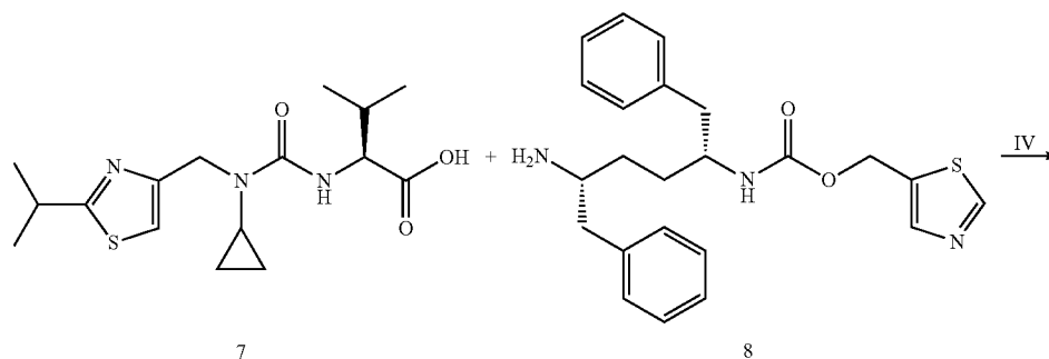
Scheme 5
