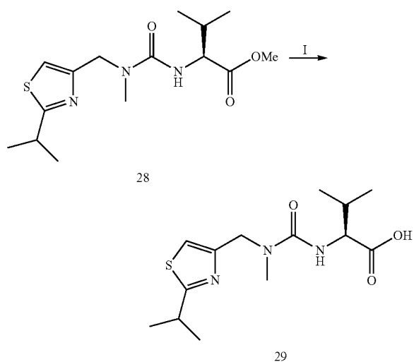
Scheme 13
