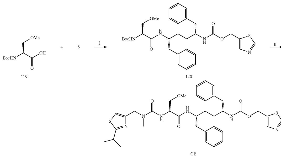
Scheme 67
