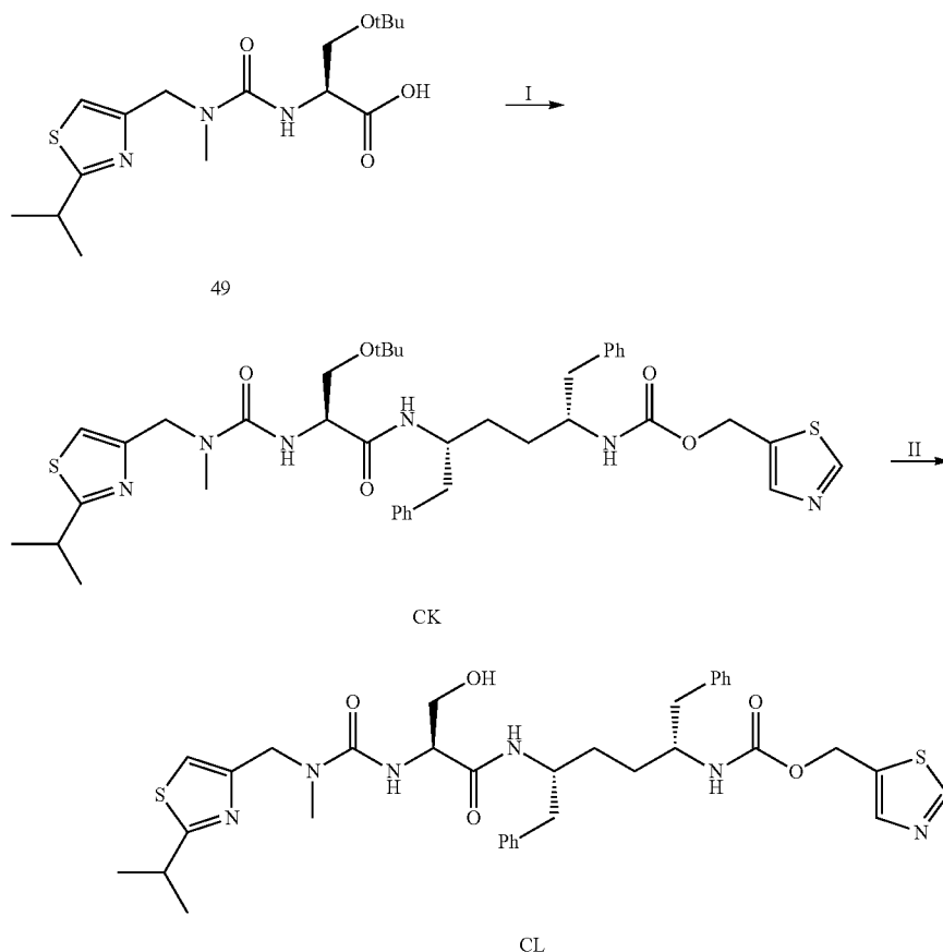
Scheme 74
