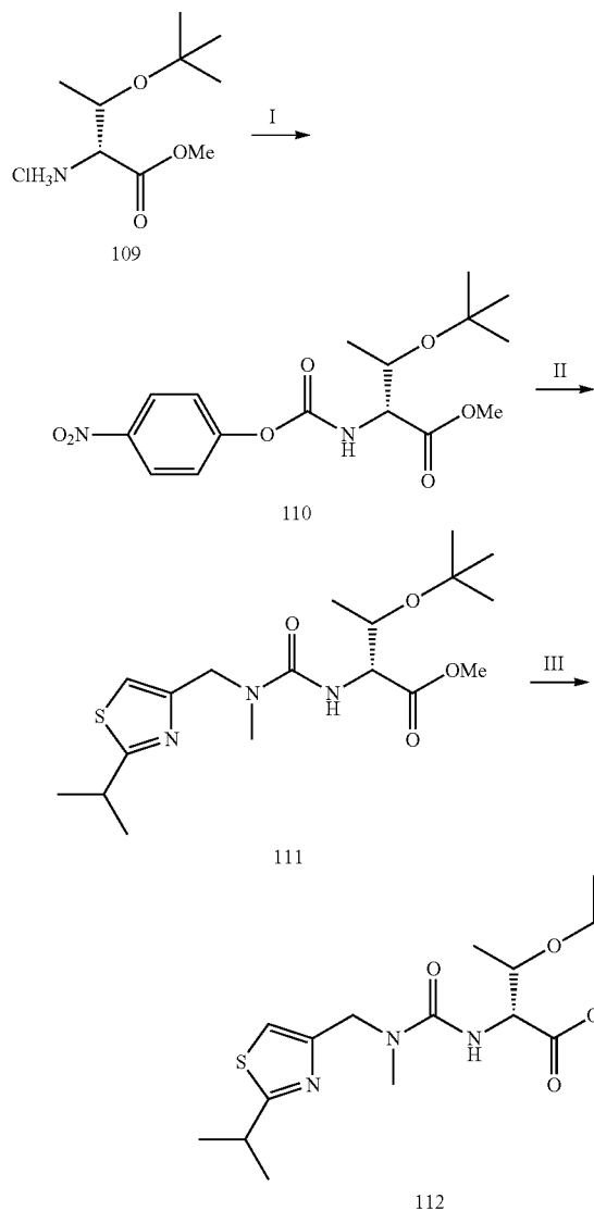
Scheme 52
