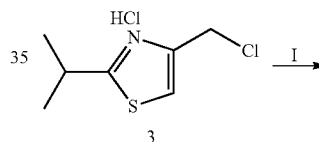
Scheme 3
