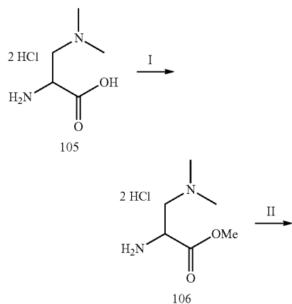
Scheme 51
