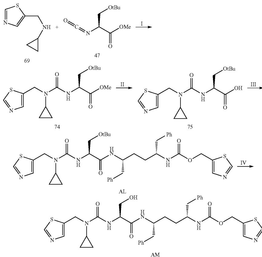
Scheme 31
