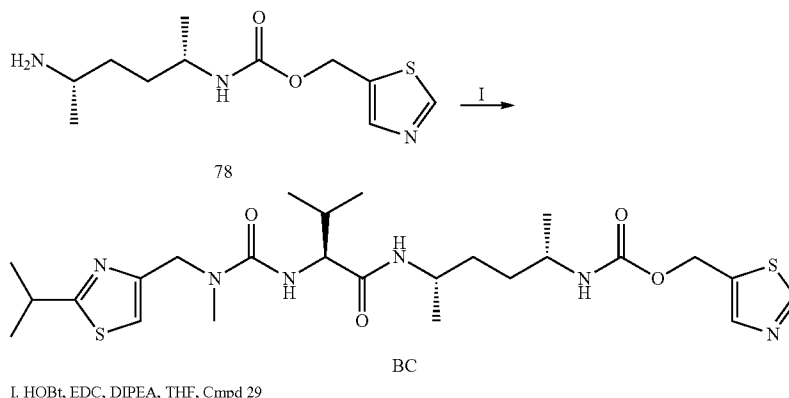
Scheme 44
