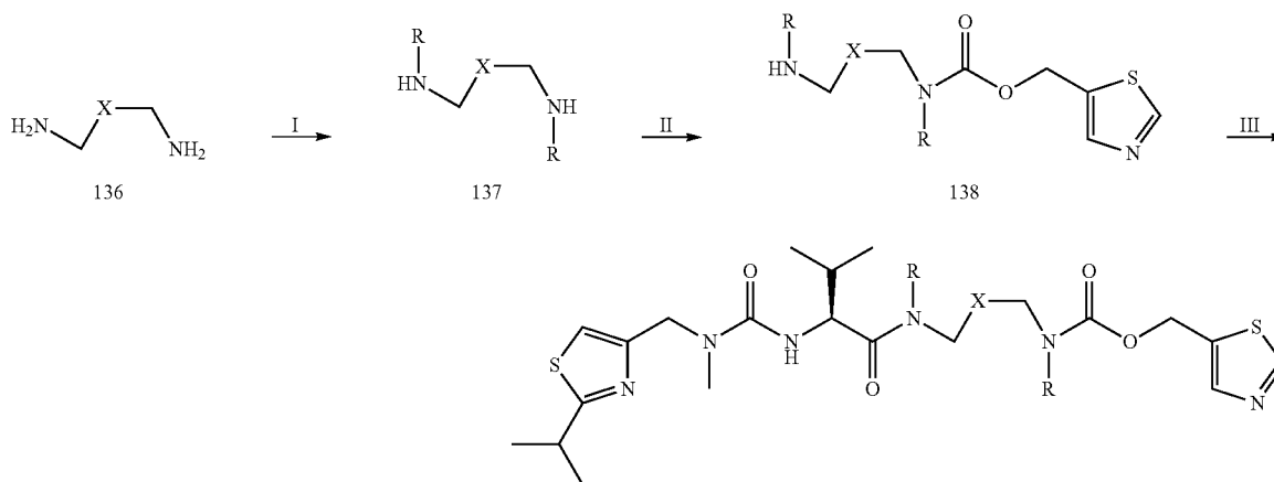
Scheme 78
