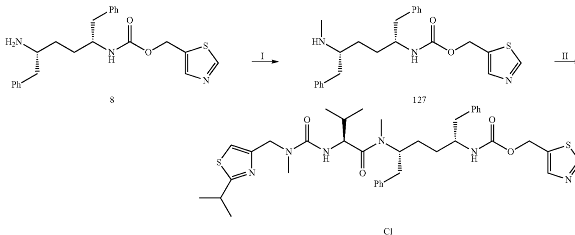
Scheme 72
